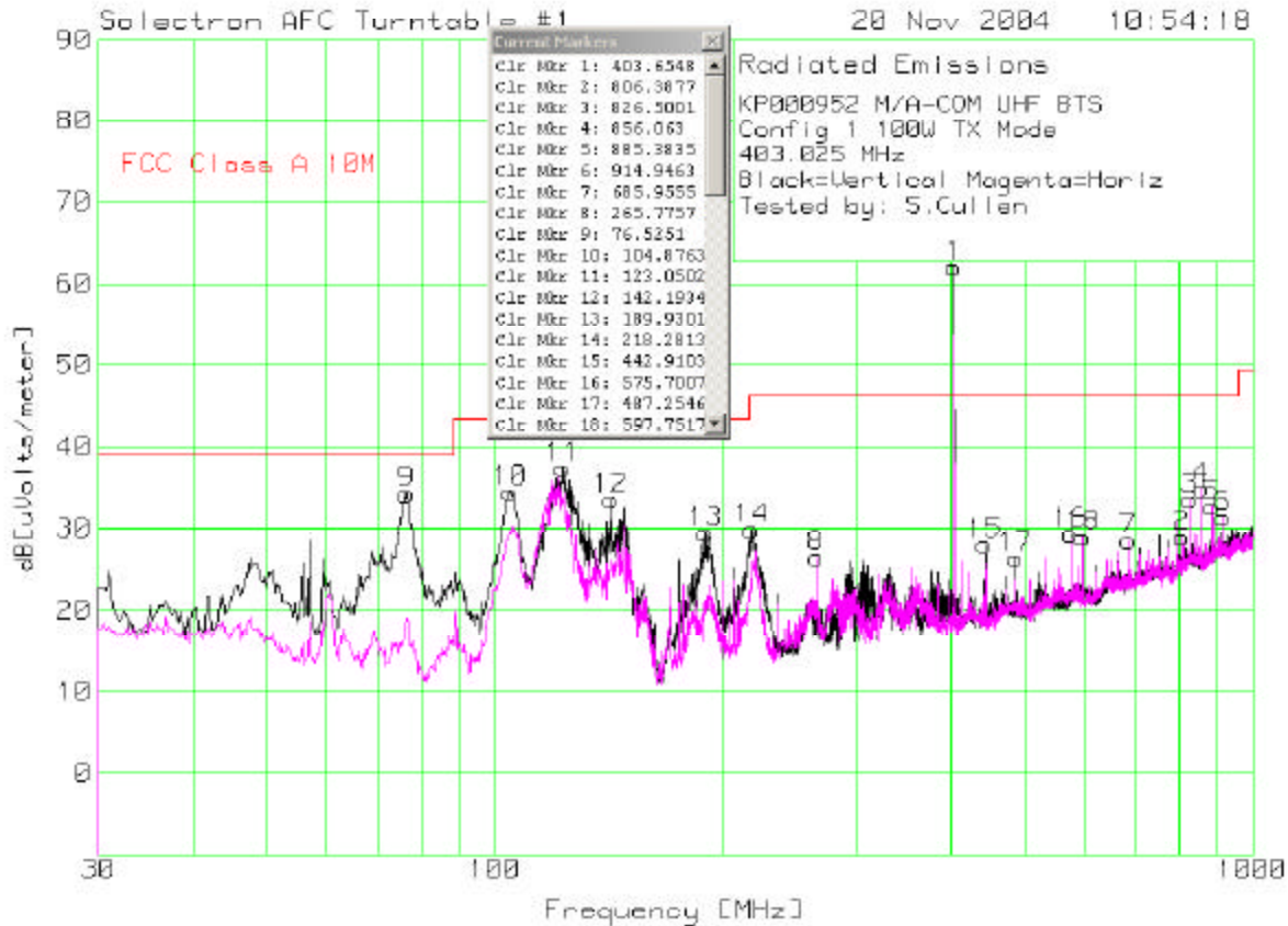
Figure 7-16: Field Strength with 100 W Tx, 30 MHz to 1 GHz (Tx at 403.025 MHz)
