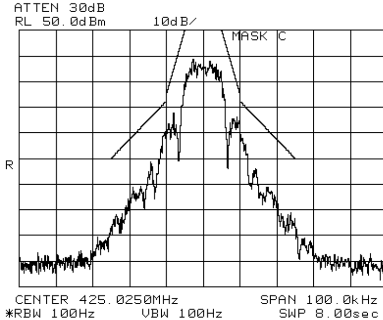
Figure 7-12: 2 Level 9600 baud Signal with +/- 3 kHz Deviation, 425.025 MHz
