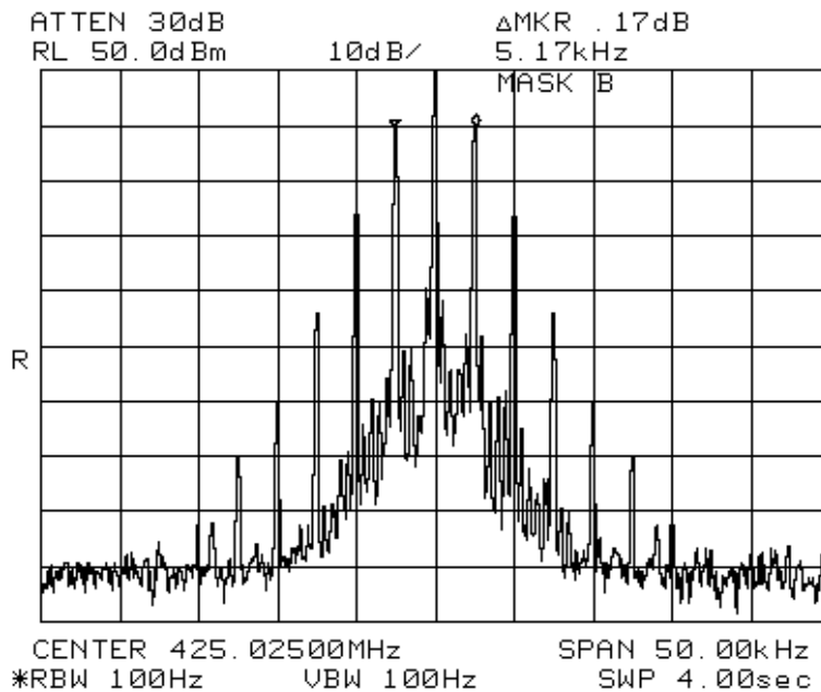
Figure 7-29: 2500 Hz Audio Signal Narrowband, 425.025 MHz
