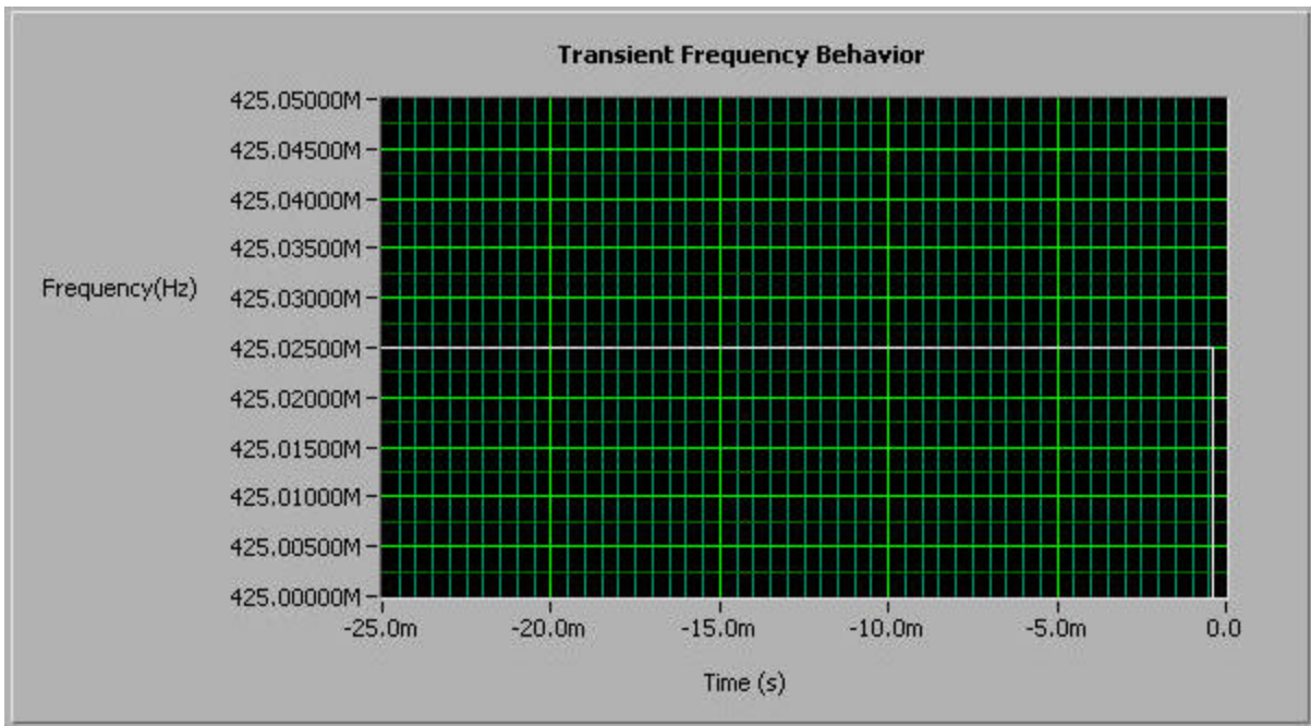
Figure 7-25 Transient Frequency Behavior, Tx at 425.025 MHz, Wideband, Transmitter off
