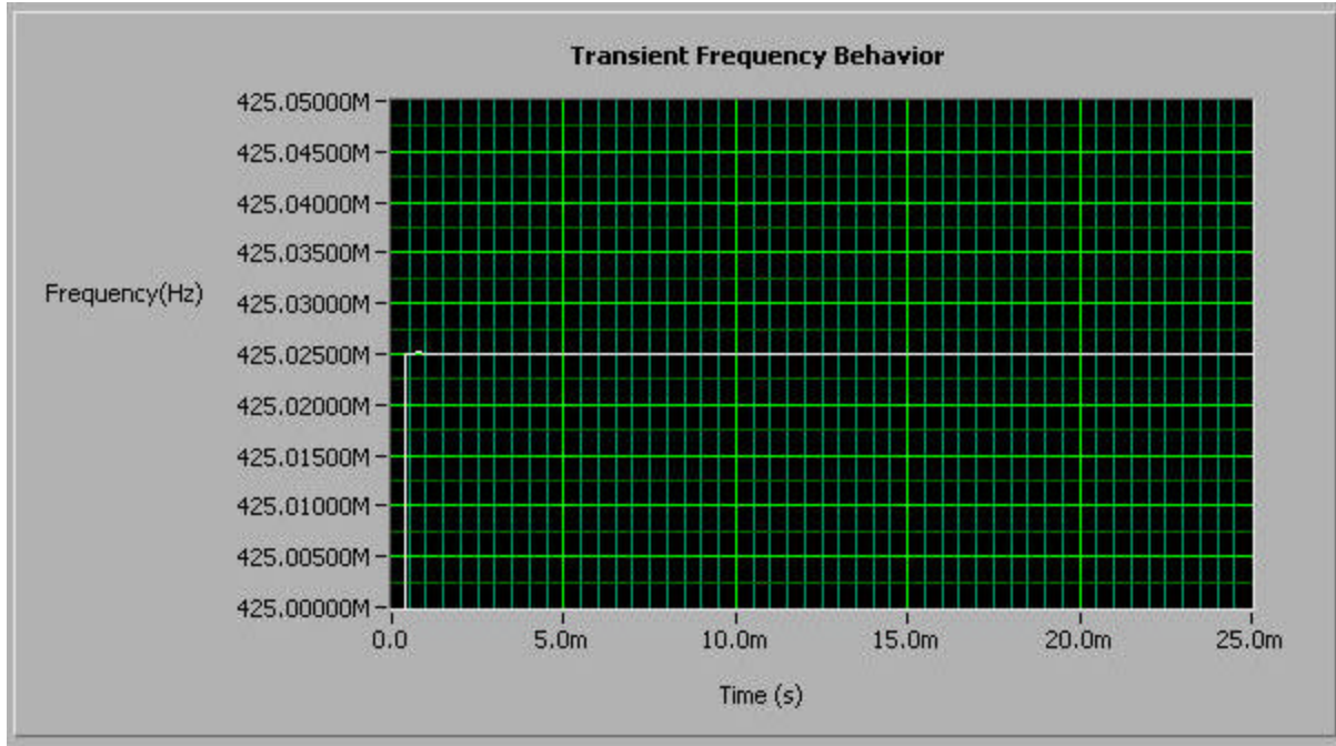
Figure 7-24 Transient Frequency Behavior, Tx at 425.025 MHz, Wideband, Transmitter on
