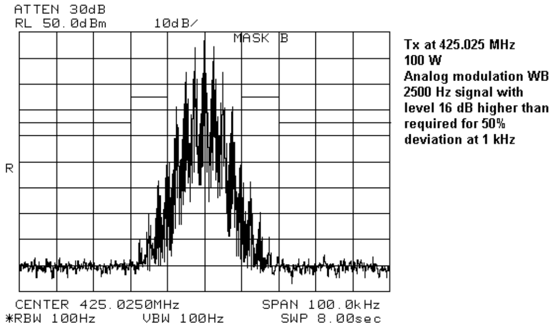
Figure 7-10: 2500 Hz Audio Signal Wideband, 425.025 MHz
