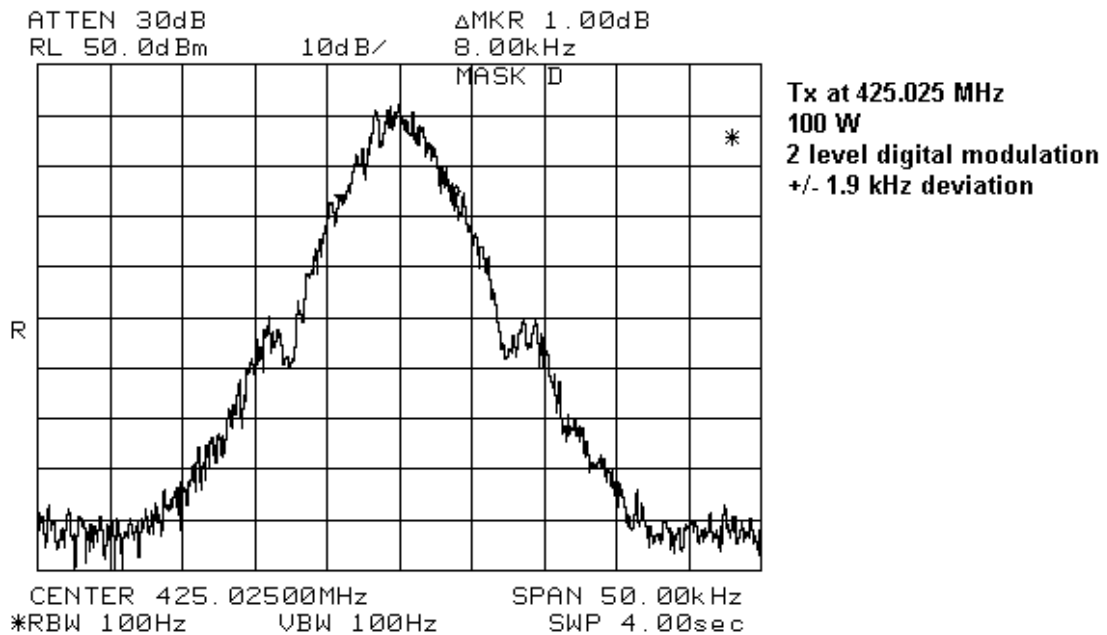
Figure 7-31: 2 Level 9600 baud Signal with +/- 1.9 kHz Deviation, 425.025 MHz
