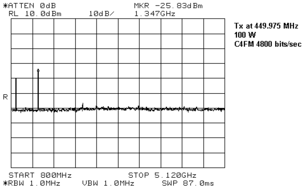
Figure 7-7: Tx at 449.975 MHz, 100 W Power, 800 MHz to 5.12 GHz
