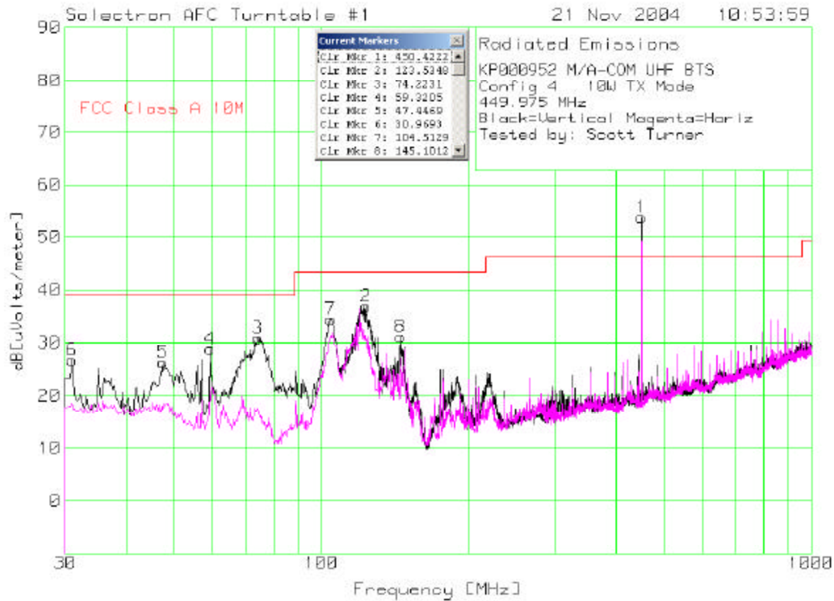
Figure 7-22: Field Strength with 10 W Tx, 30 MHz to 1 GHz (Tx at 449.975 MHz)
