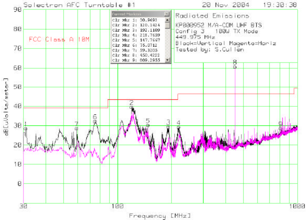
Figure 7-20: Field Strength with 100 W Tx, 30 MHz to 1 GHz (Tx at 449.975 MHz)
