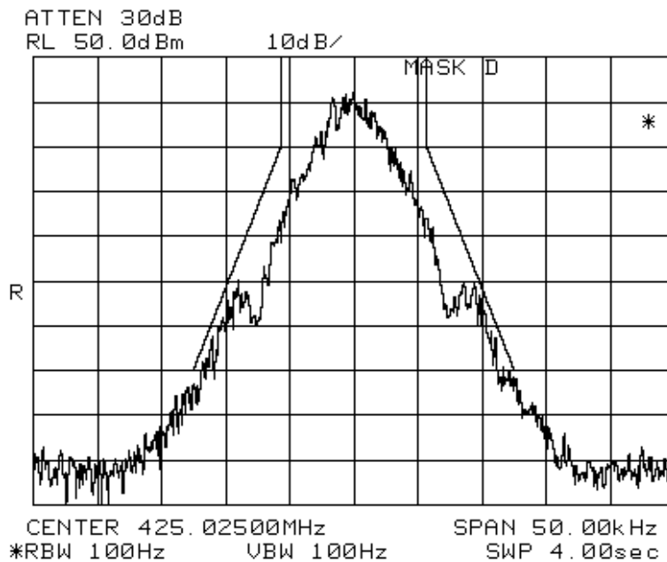
Figure 7-13: 2 Level 9600 baud Signal with +/- 1.9 kHz Deviation, 425.025 MHz
