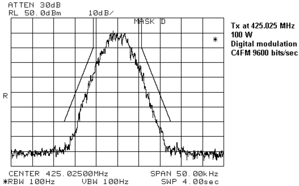
Figure 7-14: C4FM / 9600 bits/second Signal, 425.025 MHz
