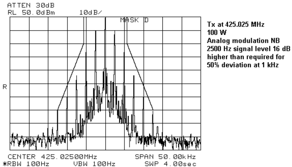
Figure 7-11: 2500 Hz Audio Signal Narrowband, 425.025 MHz
