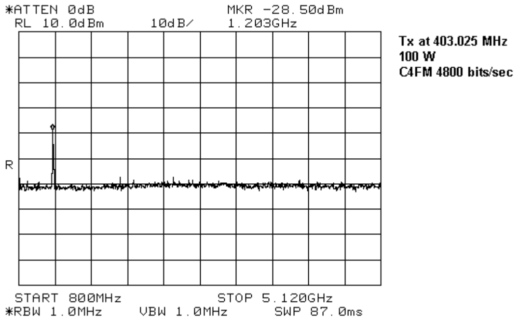
Figure 7-3: Tx at 403.025 MHz, 100 W Power, 800 MHz to 5.12 GHz
