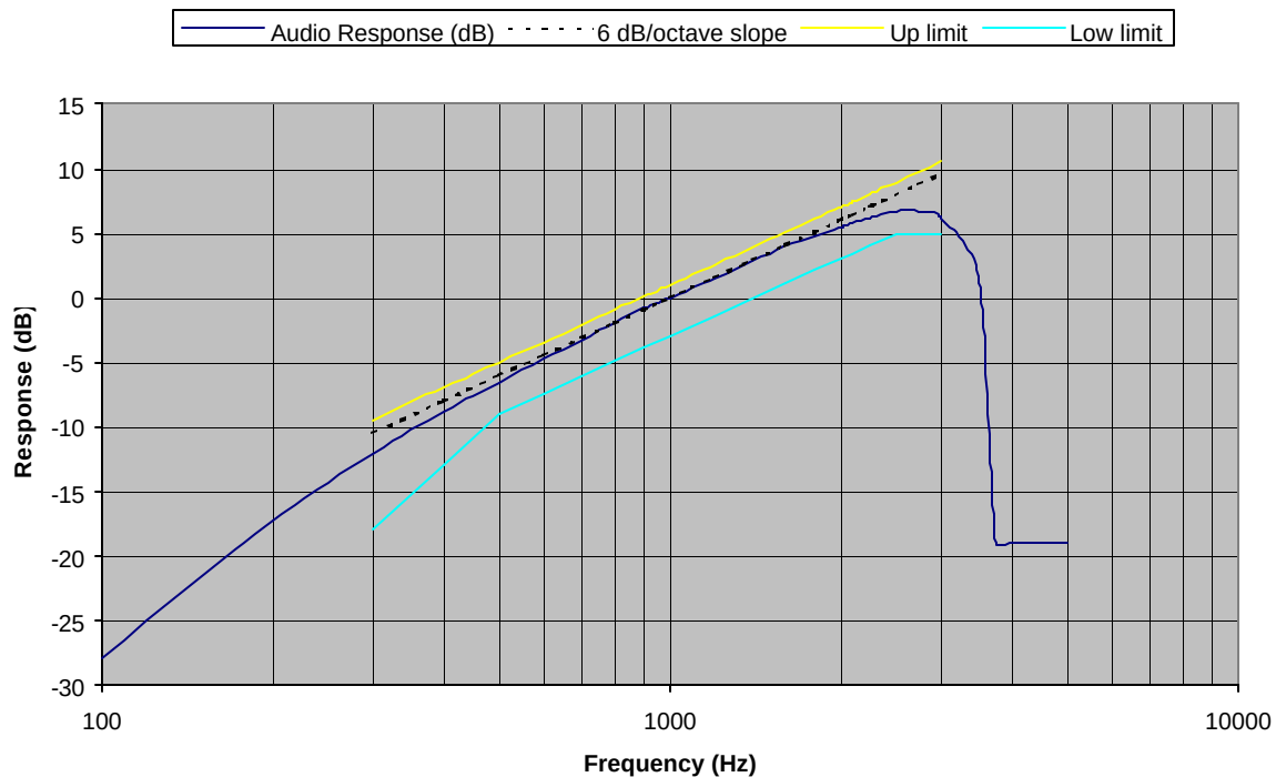
Figure 5-1: Audio Frequency Response Results
