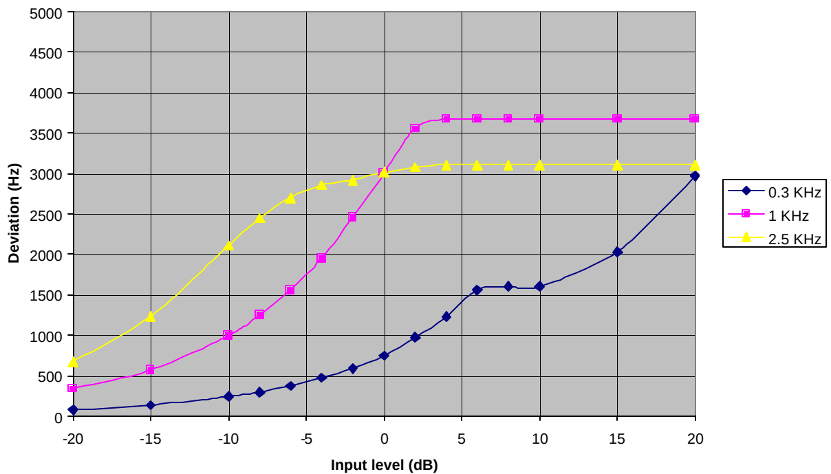
Figure 5-3 Modulation Limiting, Positive Peak (25 kHz channel)
