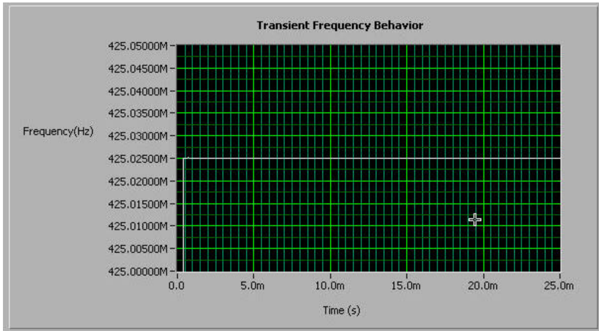
Figure 7-26 Transient Frequency Behavior, Tx at 425.025 MHz, Narrowband, Transmitter on
