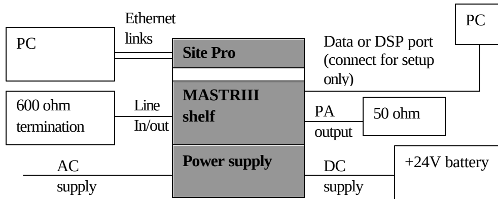
Figure 3-3: System Configuration
