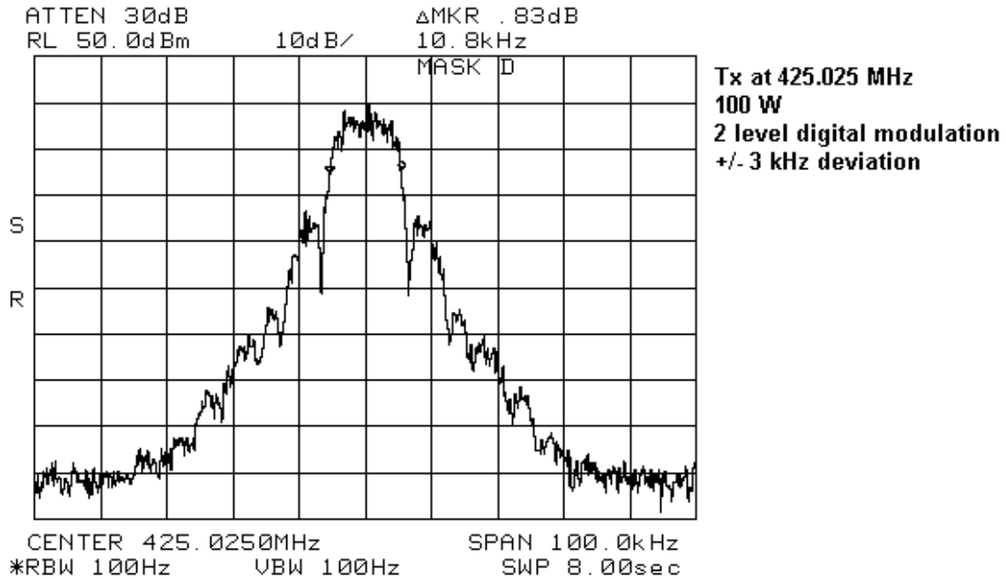
Figure 7-30: 2 Level 9600 baud Signal with +/- 3 kHz Deviation, 425.025 MHz
