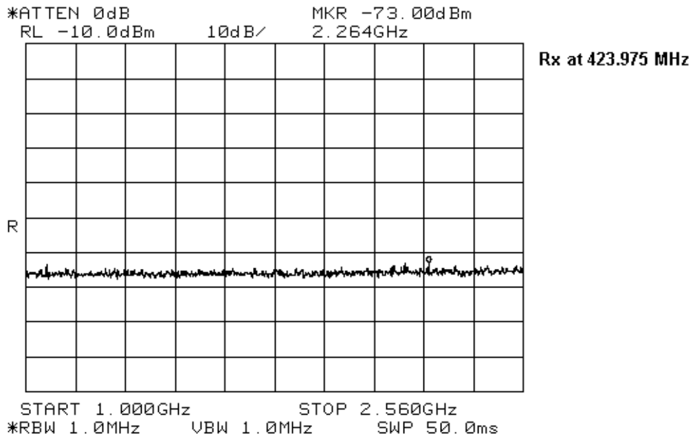
Figure 7-35: Rx at 423.975 MHz, 1 GHz to 2.56 GHz
