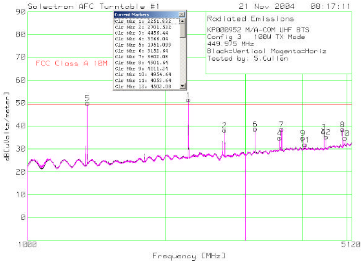
Figure 7-21: Field Strength with 100 W Tx, 1 GHz to 5.12 GHz, (Tx at 449.975 MHz)
