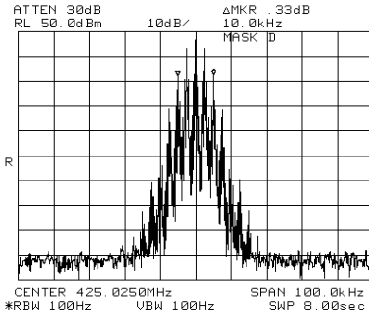
Figure 7-28: 2500 Hz Audio Signal Wideband, 425.025 MHz
