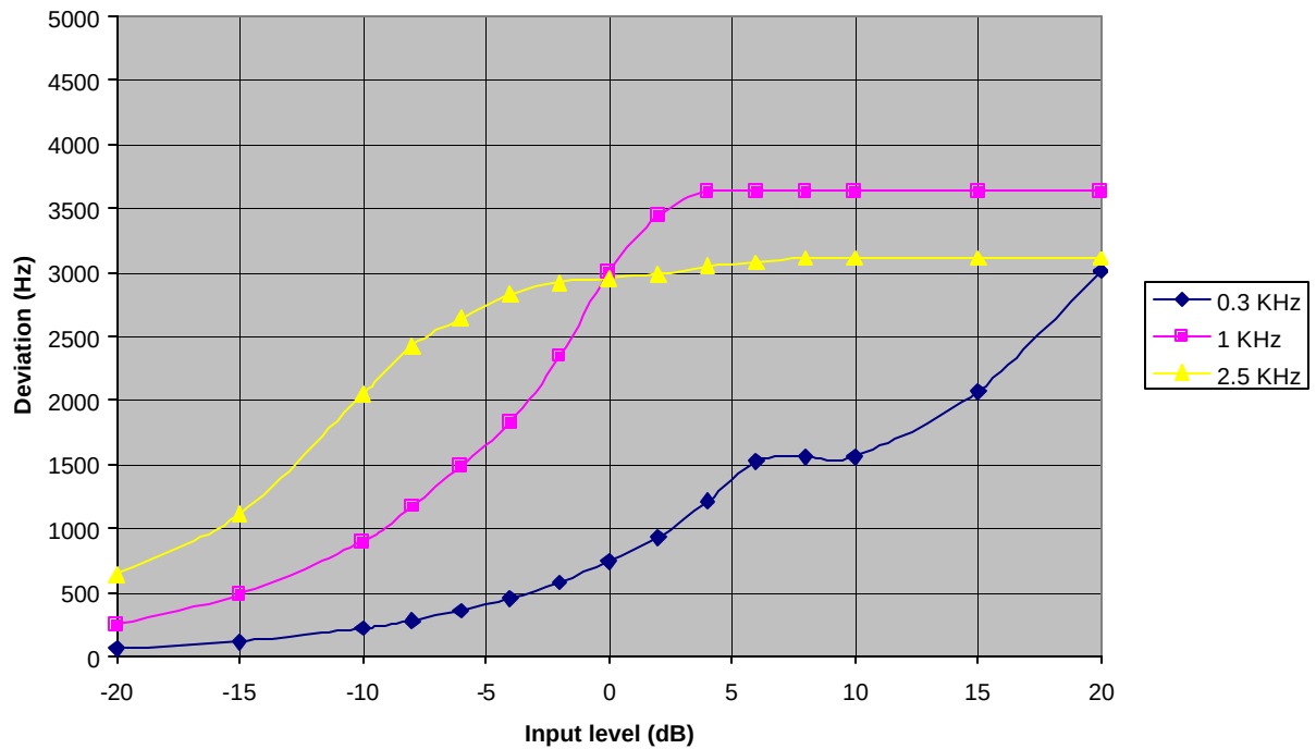
Figure 5-5 Modulation Limiting, Positive Peak (12.5 kHz channel)
