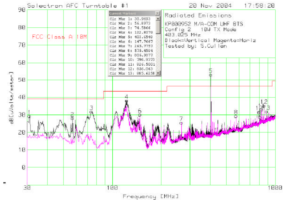
Figure 7-18: Field Strength with 10 W Tx, 30 MHz to 1 GHz (Tx at 403.025 MHz)
