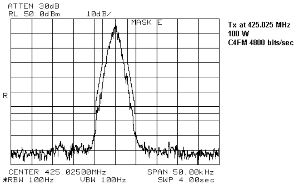
Figure 7-15: C4FM / 4800 bits/second Signal, 425.025 MHz
