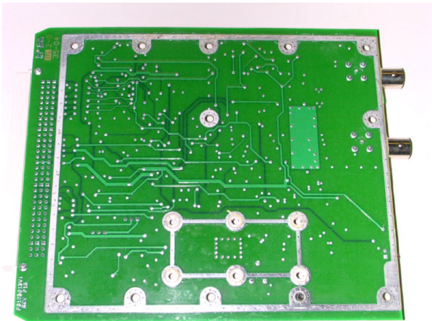
Tx Synthesizer 470-512 MHz (secondary side)
