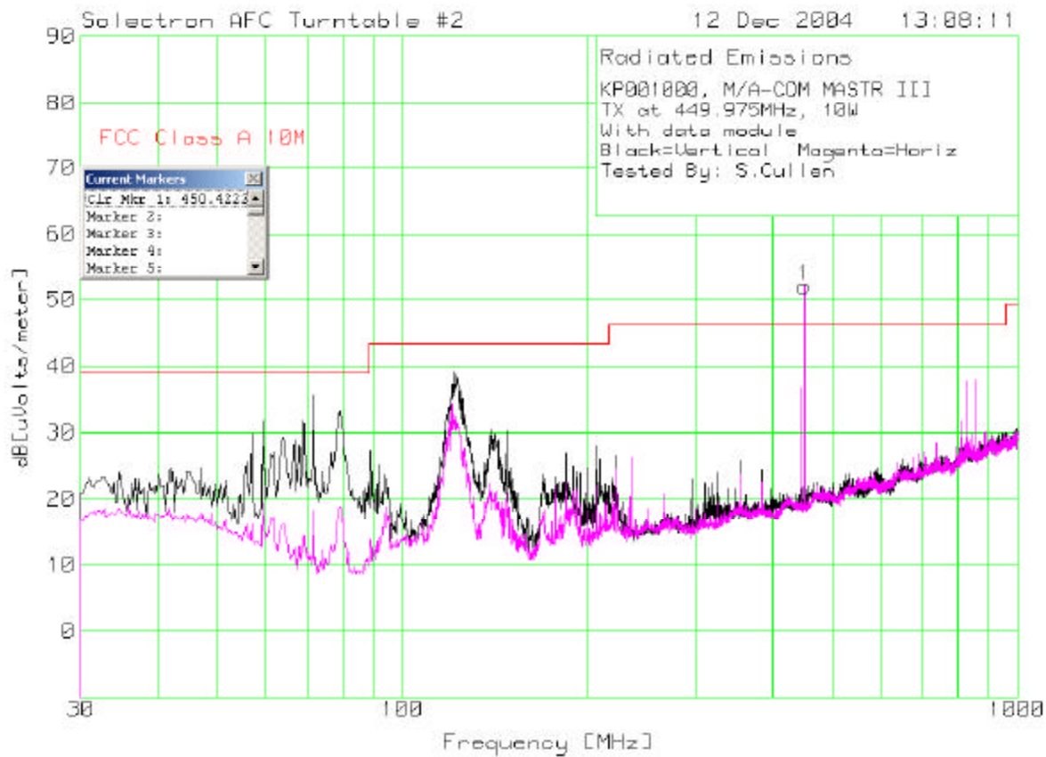
Figure 7-17: Field Strength with 10 W Tx, 30 MHz to 1 GHz (Tx at 449.975 MHz)
