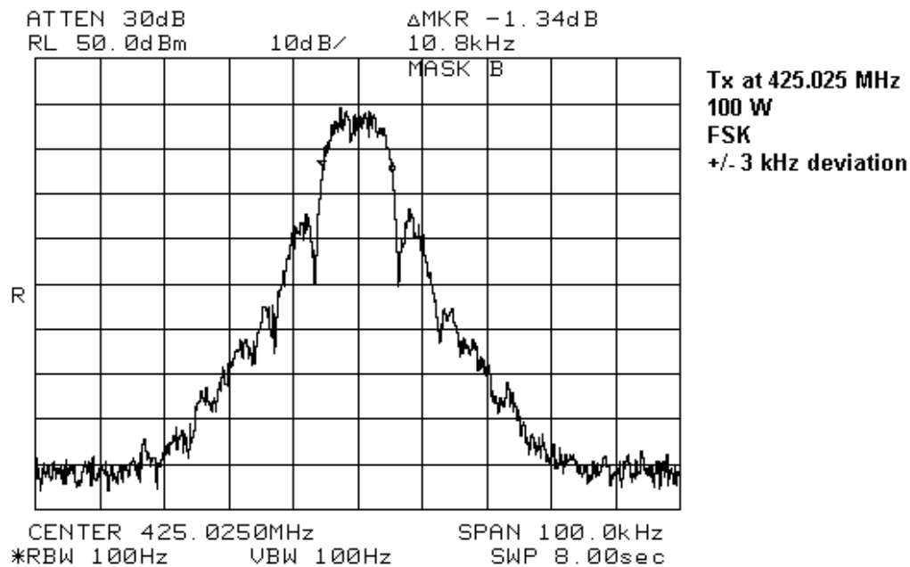
Figure 7-21: 2 Level 9600 baud Signal with +/- 3 kHz Deviation, 425.025 MHz
