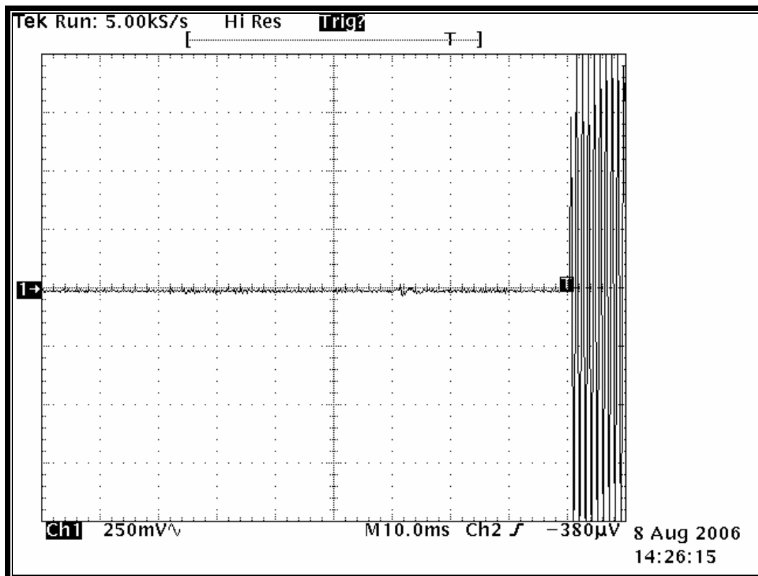
Plot 12-3: Transient Frequency Behavior – 459.800 MHz; Narrow Band; High Power; Carrier ON Time
