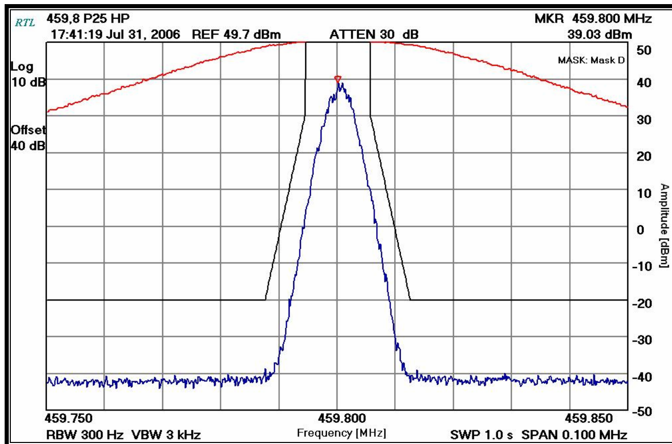
Plot 7-6: Occupied Bandwidth - 459.800 MHz; P25; High Power
