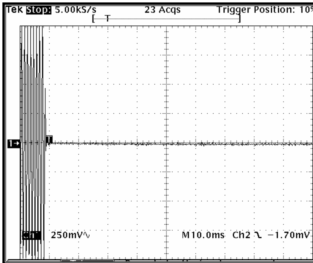
Plot 12-4: Transient Frequency Behavior – 459.800 MHz; Narrow Band; High Power; Carrier OFF Time
