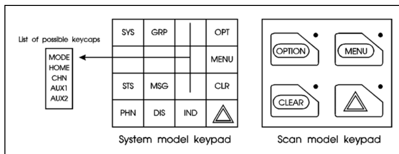
Figure 8-3: Standard M7100 IP Keycaps Configuration
