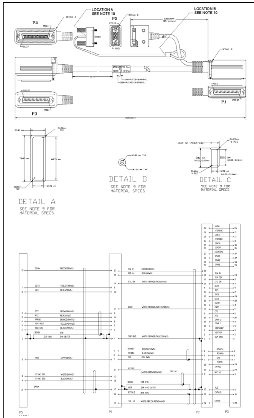
Figure 12-5: Dual Radio Control Cable (CA101288V10)
