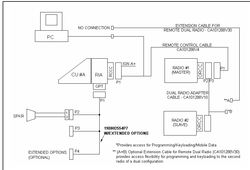
Figure 12-2: M7100 Dual Radio Remote Mount/Remote Mount Installation Configuration
