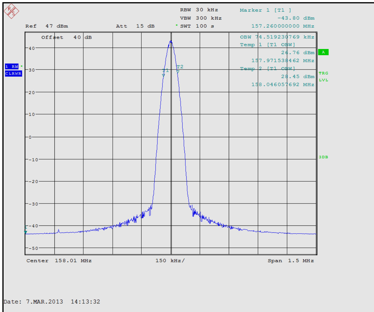
Plot 5-1: Occupied Bandwidth – 158.01 MHz; Analog (FCC Part 22)
