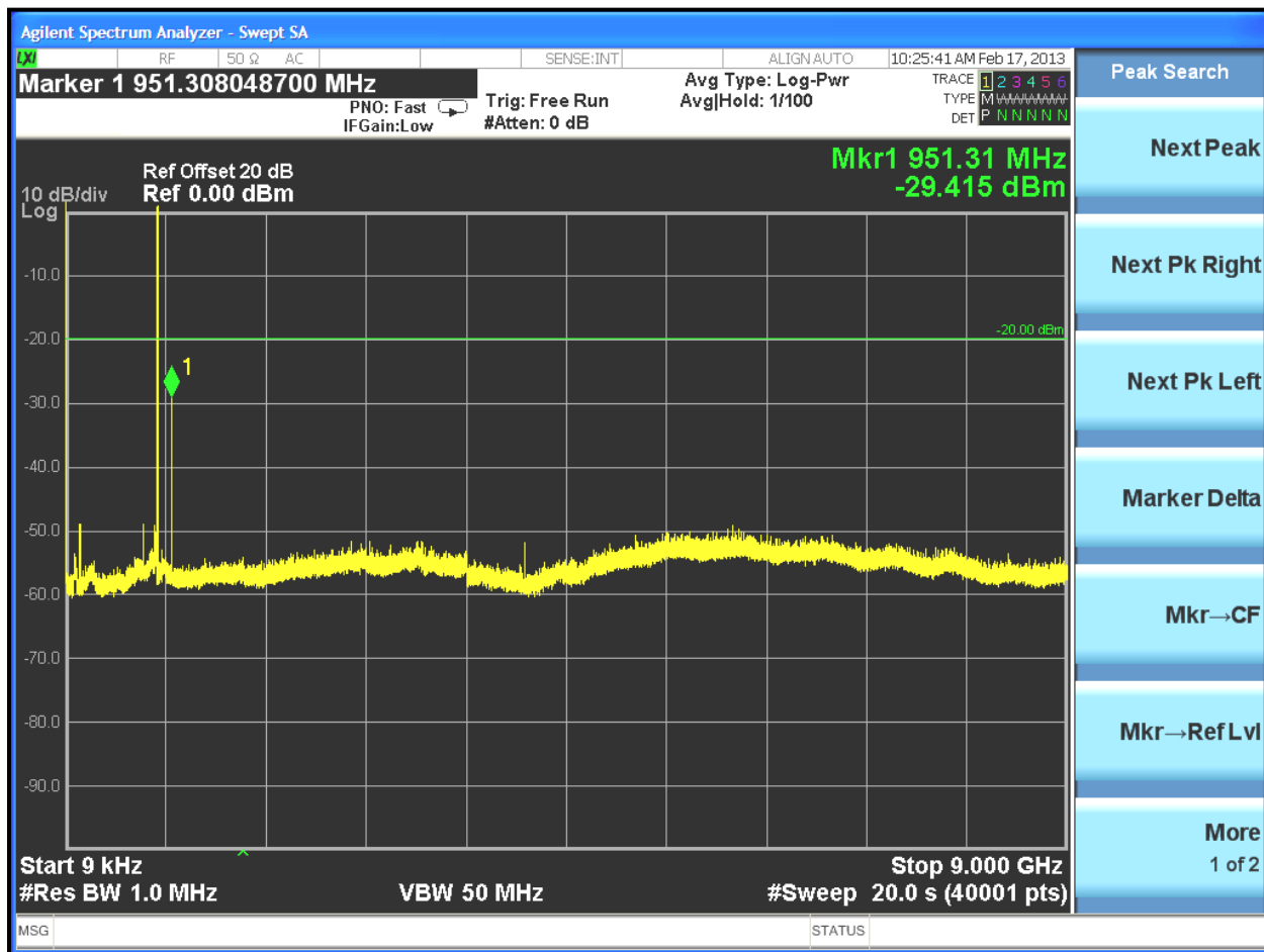
Plot 5-8: Conducted Spurious Emissions – H-CPM TDMA; 823.9875 MHz
