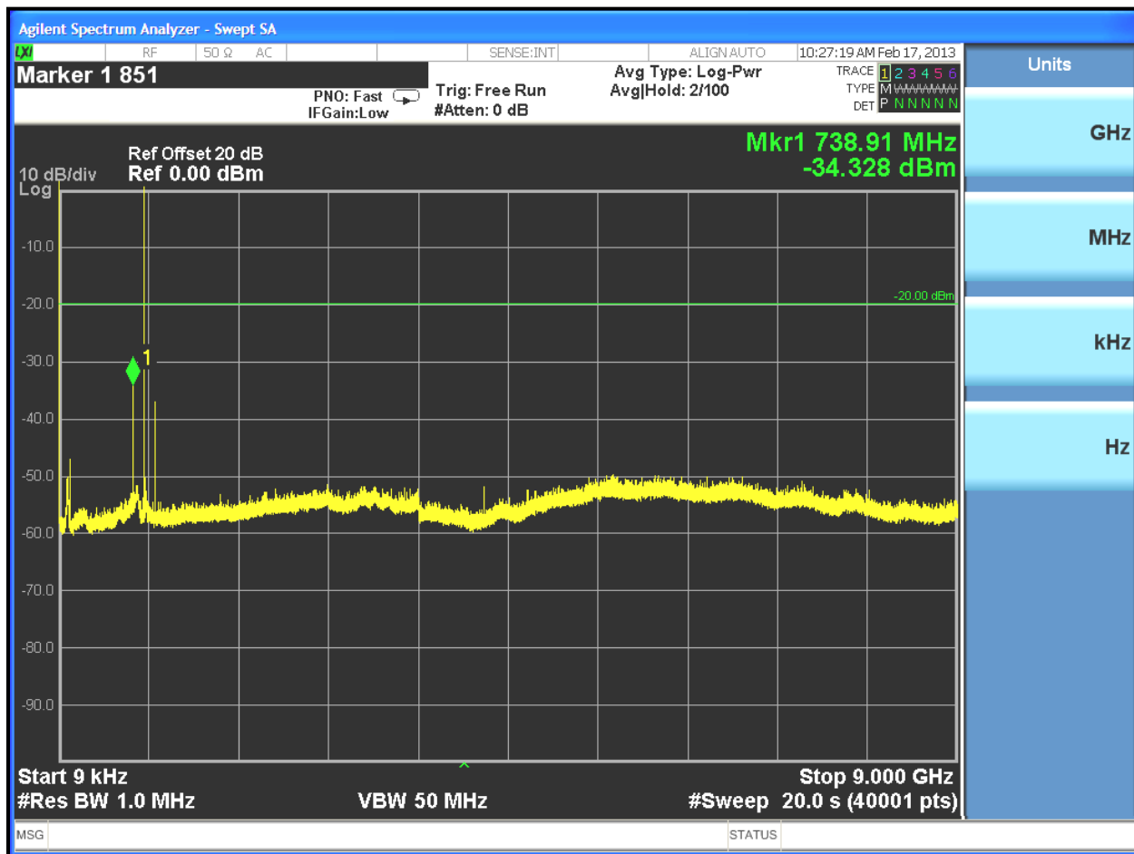
Plot 5-9: Conducted Spurious Emissions – H-CPM TDMA; 851.0125 MHz
