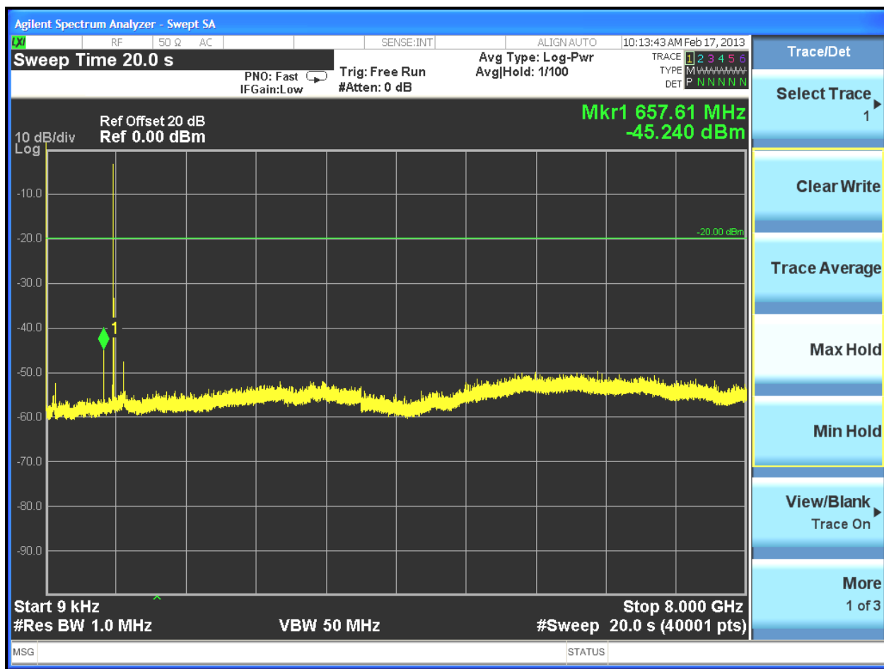
Plot 5-1: Conducted Spurious Emissions – H-CPM TDMA; 770.00625 MHz
