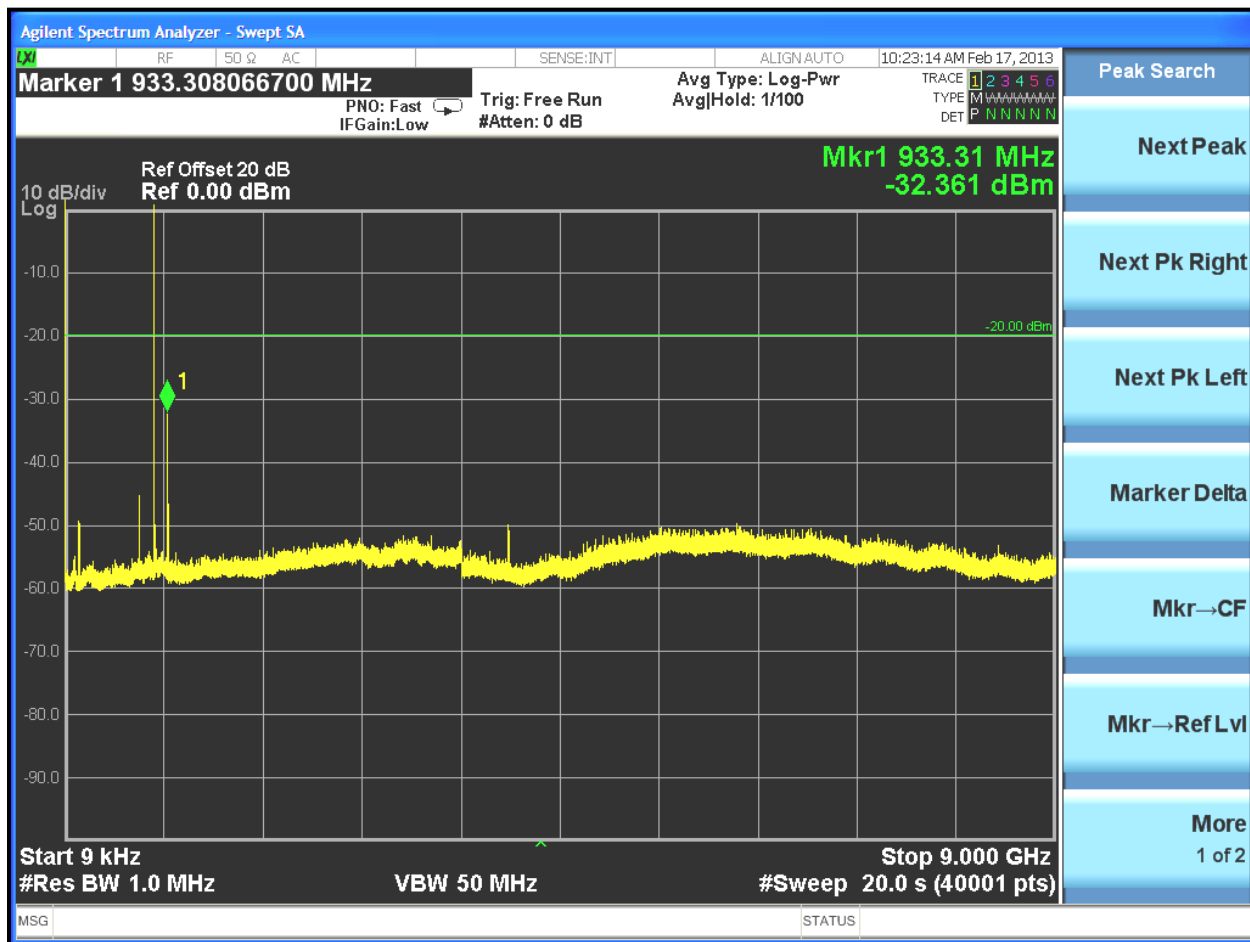
Plot 5-6: Conducted Spurious Emissions – H-CPM TDMA; 806.0125 MHz
