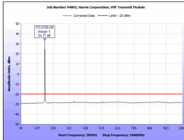
Plot 61. Spurious Emissions at Antenna Terminals, below 1GHz, 174MHz HDQPSK, 100W
