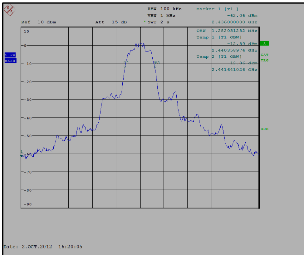
Plot 6-5: 20 dB Bandwidth - 2441 MHz (EDR)
