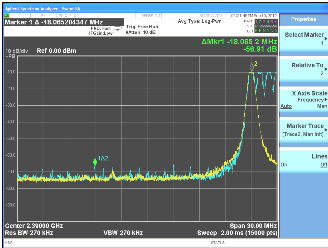
Plot 5-1: Lower Band Edge TX Frequency - 2402 MHz
