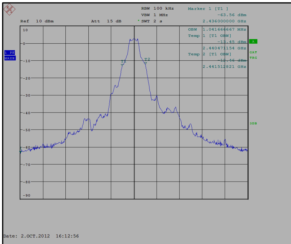
Plot 6-2: 20 dB Bandwidth - 2441 MHz (SDR)
