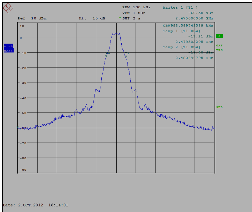
Plot 6-3: 20 dB Bandwidth - 2480 MHz (SDR)
