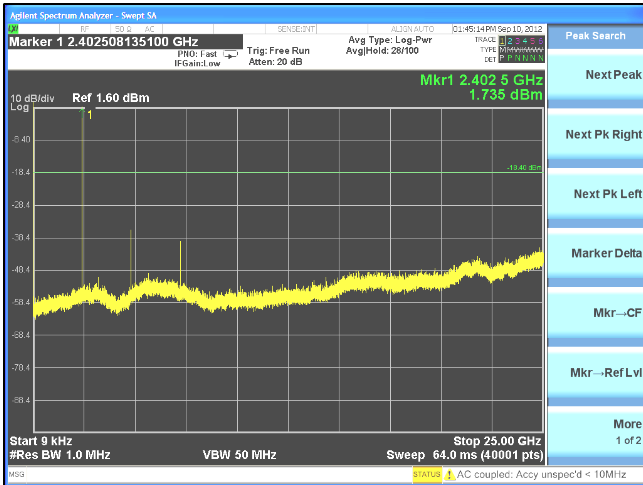
Plot 4-1: Antenna Conducted Spurious TX Frequency - 2402 MHz
