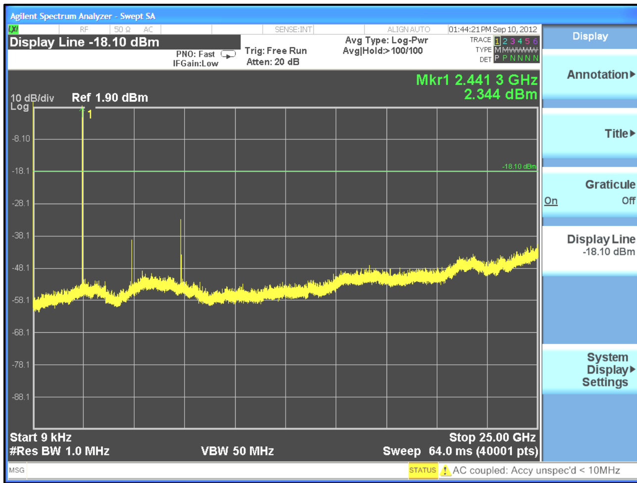
Plot 4-2: Antenna Conducted Spurious TX Frequency - 2441 MHz
