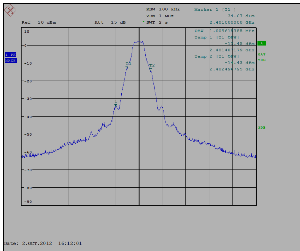
Plot 6-1: 20 dB Bandwidth - 2402 MHz (SDR)
