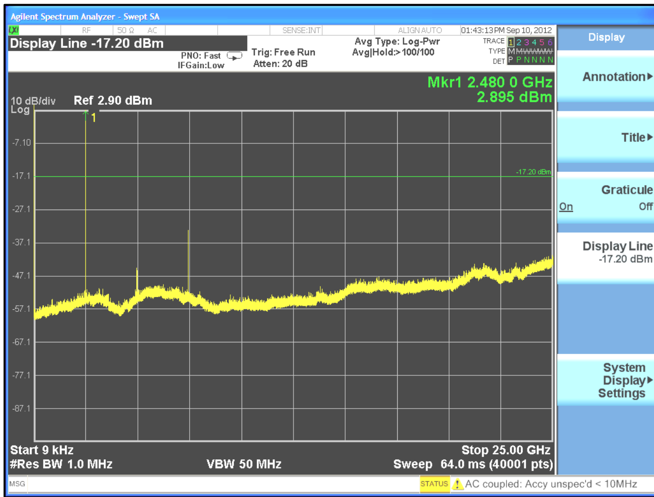
Plot 4-3: Antenna Conducted Spurious TX Frequency - 2480 MHz
