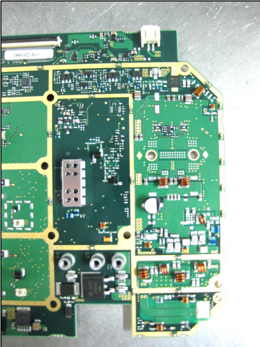
Photograph 18: PCB - Right Side
