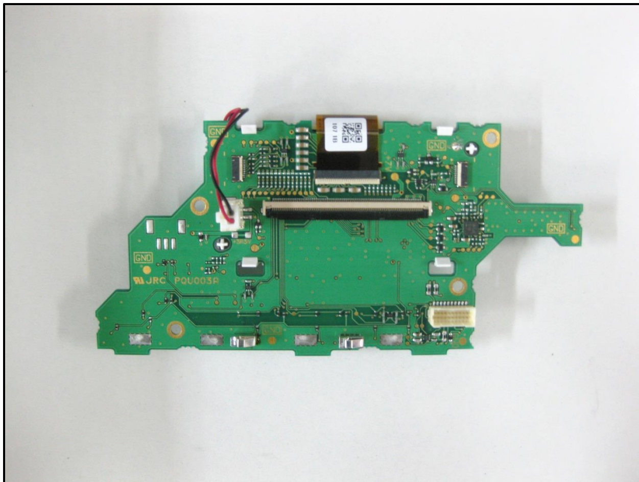
Photograph 23: Solder Side
