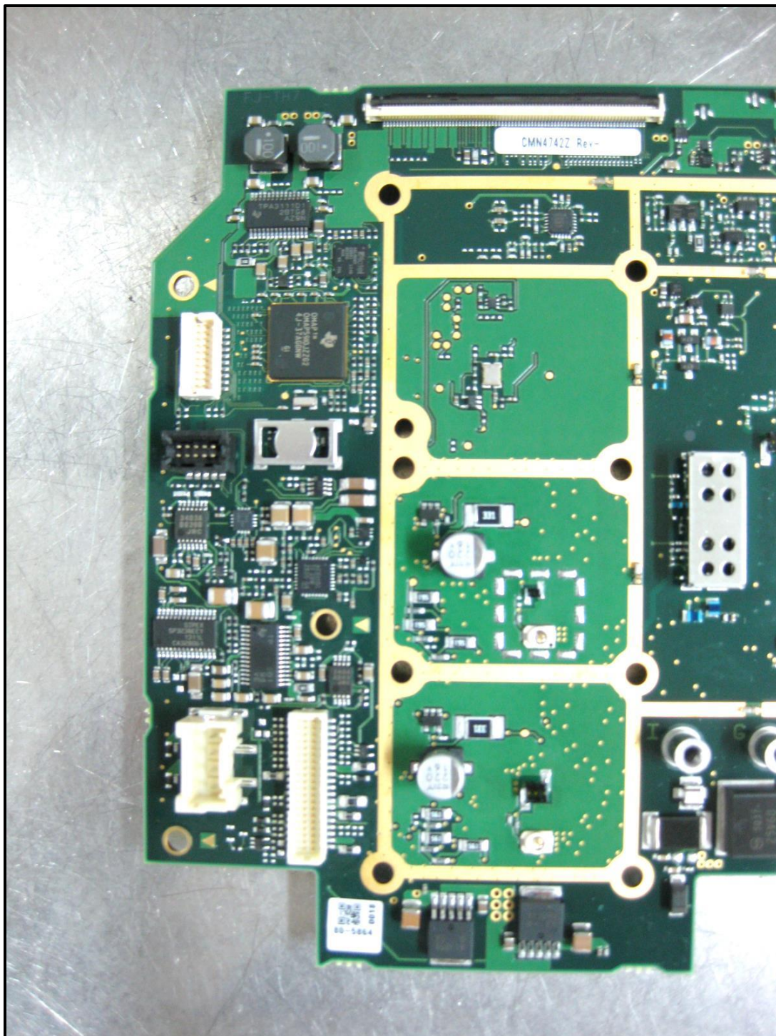
Photograph 17: PCB – Left Side
