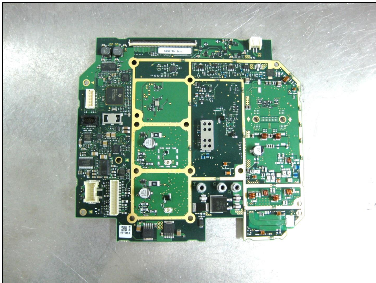
Photograph 15: PCB Side
