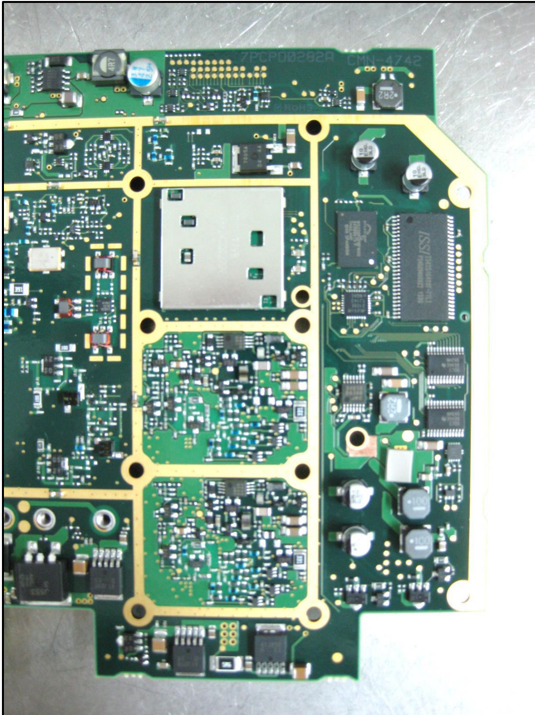
Photograph 20: Solder – Right Side
