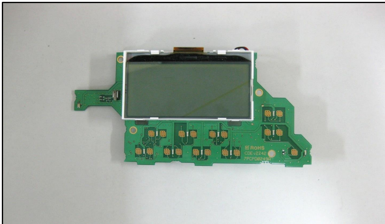
Photograph 22: PCB Side
