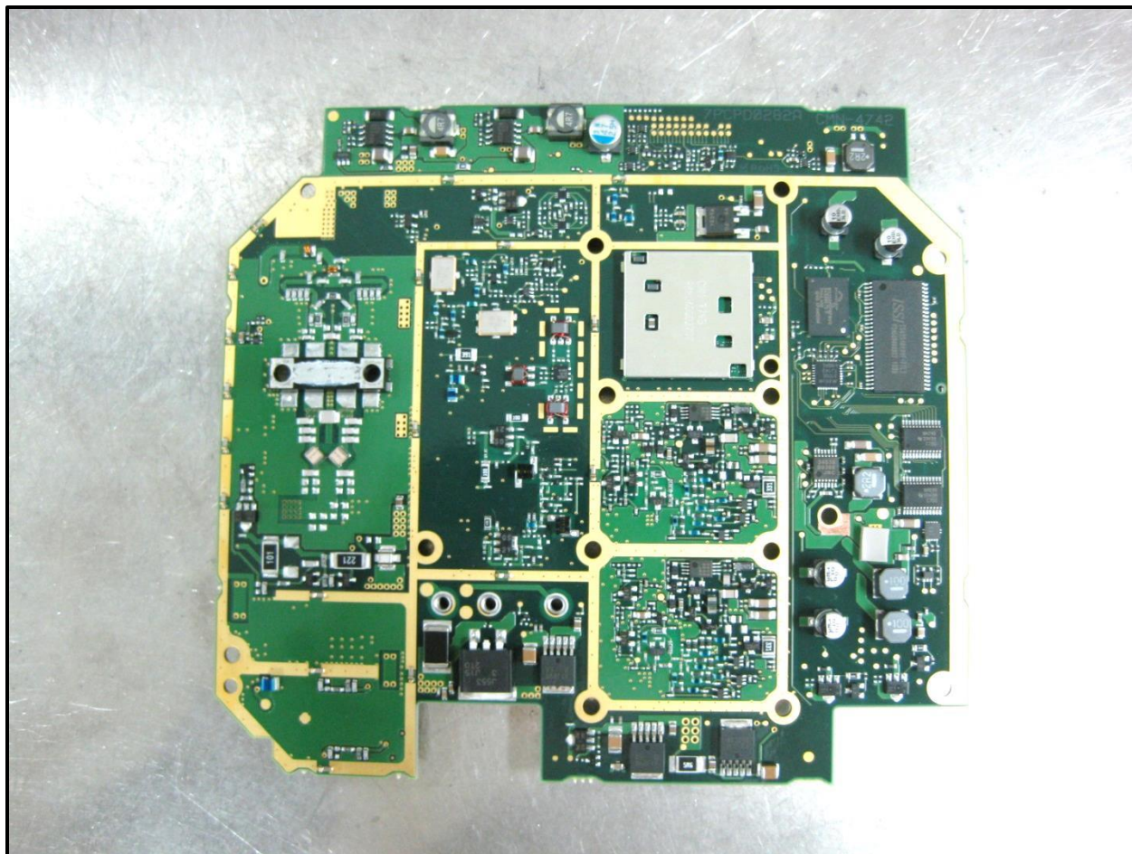
Photograph 16: Solder Side
