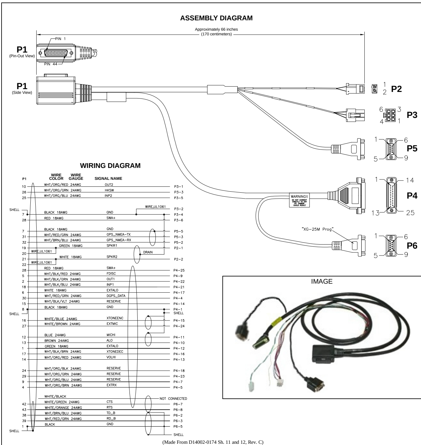
Figure 11-1: Option Cable 14002-0174-08
