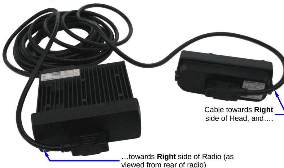
Figure 8-3: Left Side/Right Side Remote Control Cable Orientation
