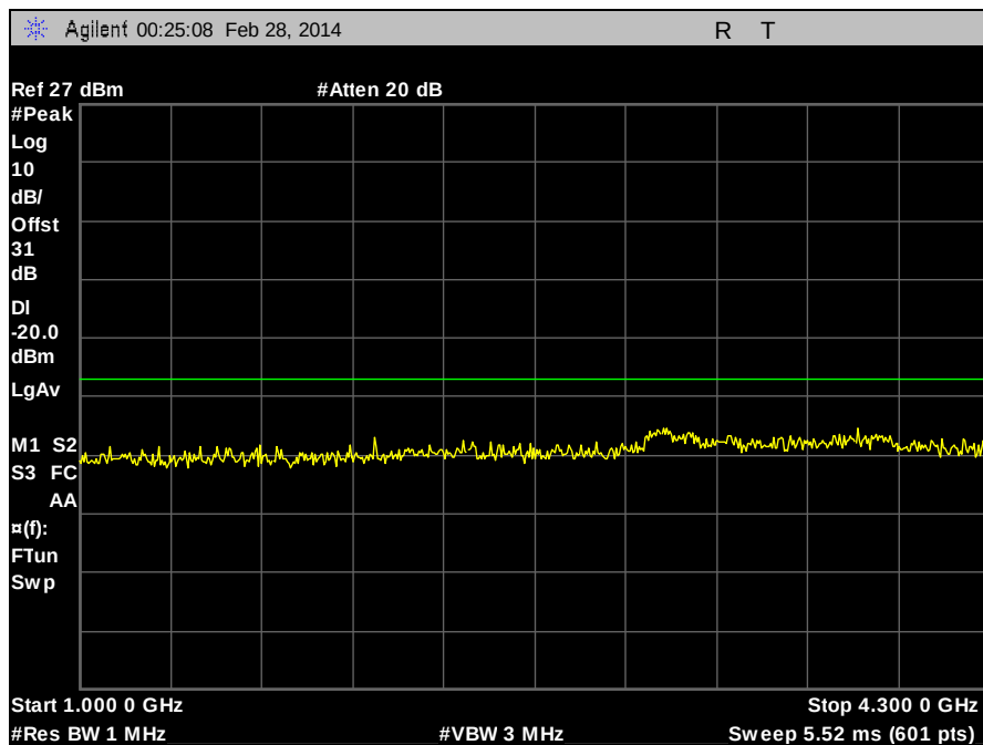
Plot 96. Part 90, Conducted Spurious Emissions, 426 MHz, HDQPSK, 100 W, 1 GHz – 4.3 GHz
