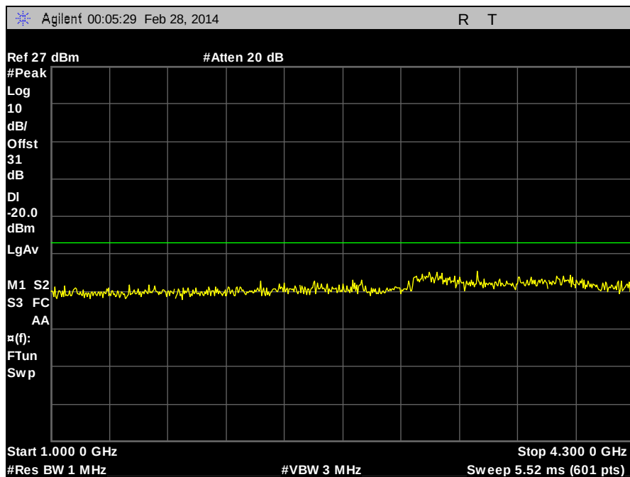
Plot 100. Part 90, Conducted Spurious Emissions, 430 MHz, CQPSK, 10 W, 1 GHz – 4.3 GHz
