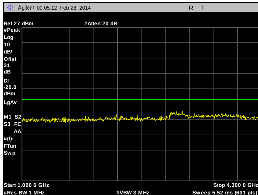
Plot 98. Part 90, Conducted Spurious Emissions, 430 MHz, C4FM, 10 W, 1 GHz – 4.3 GHz
