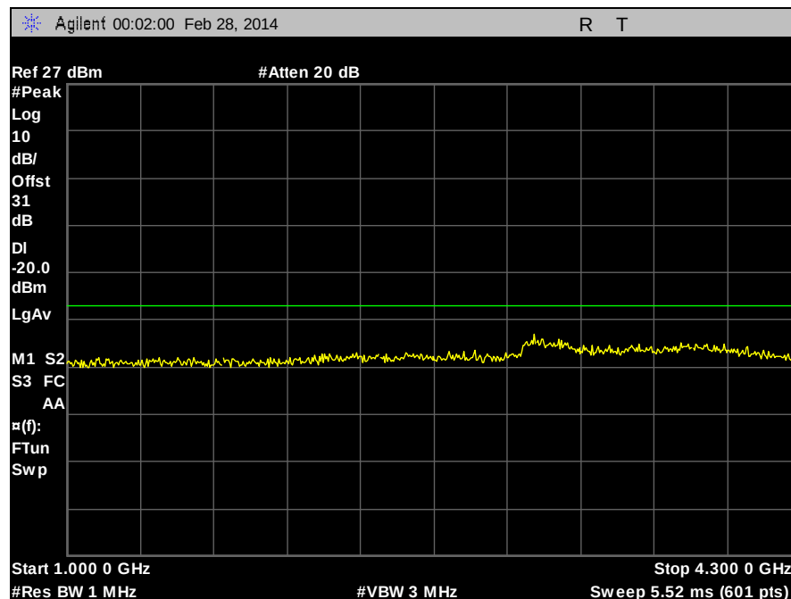
Plot 104. Part 90, Conducted Spurious Emissions, 430 MHz, C4FM, 100 W, 1 GHz – 4.3 GHz
