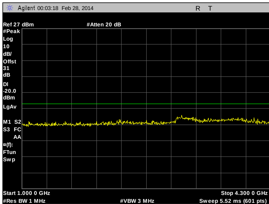
Plot 108. Part 90, Conducted Spurious Emissions, 430 MHz, HDQPSK, 100 W, 1 GHz – 4.3 GHz
