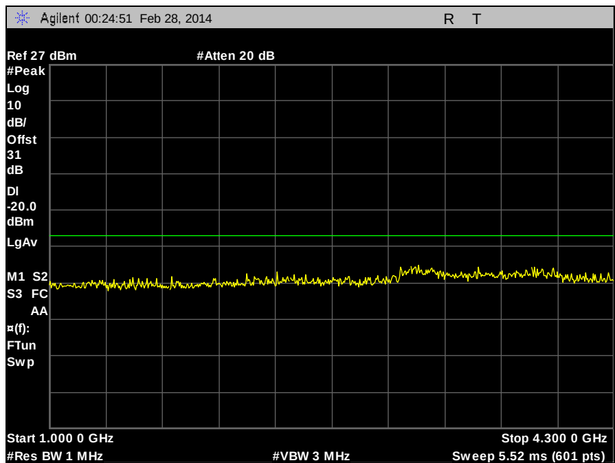
Plot 94. Part 90, Conducted Spurious Emissions, 426 MHz, CQPSK, 100 W, 1GHz – 4.3 GHz
