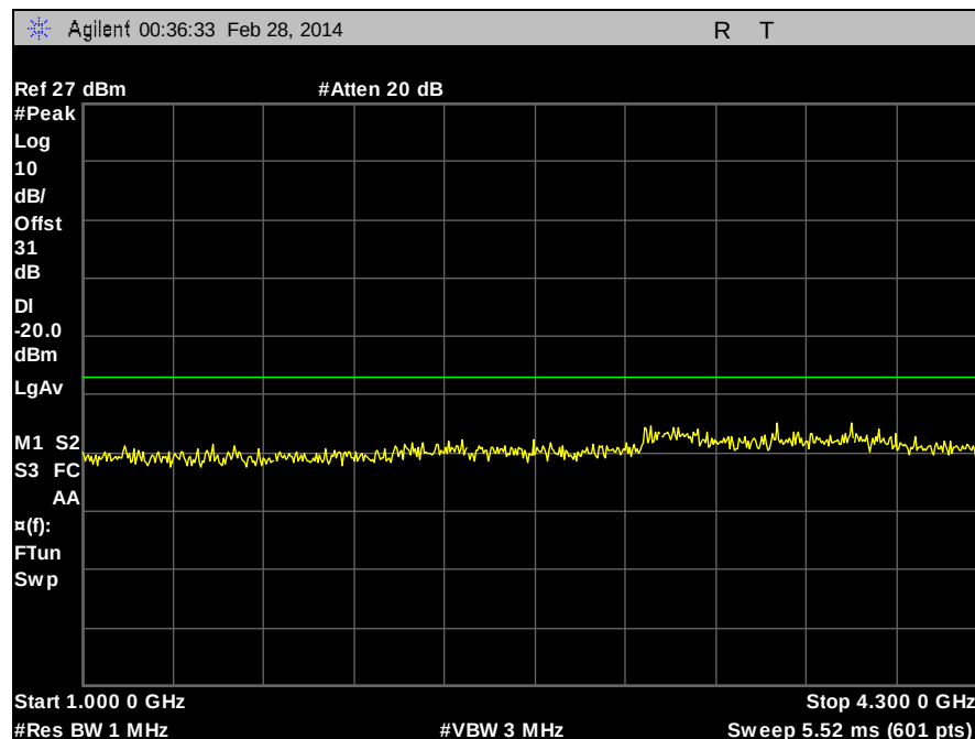
Plot 82. Part 90, Conducted Spurious Emissions, 423 MHz, CQPSK, 100 W, 1 GHz – 4.3 GHz
