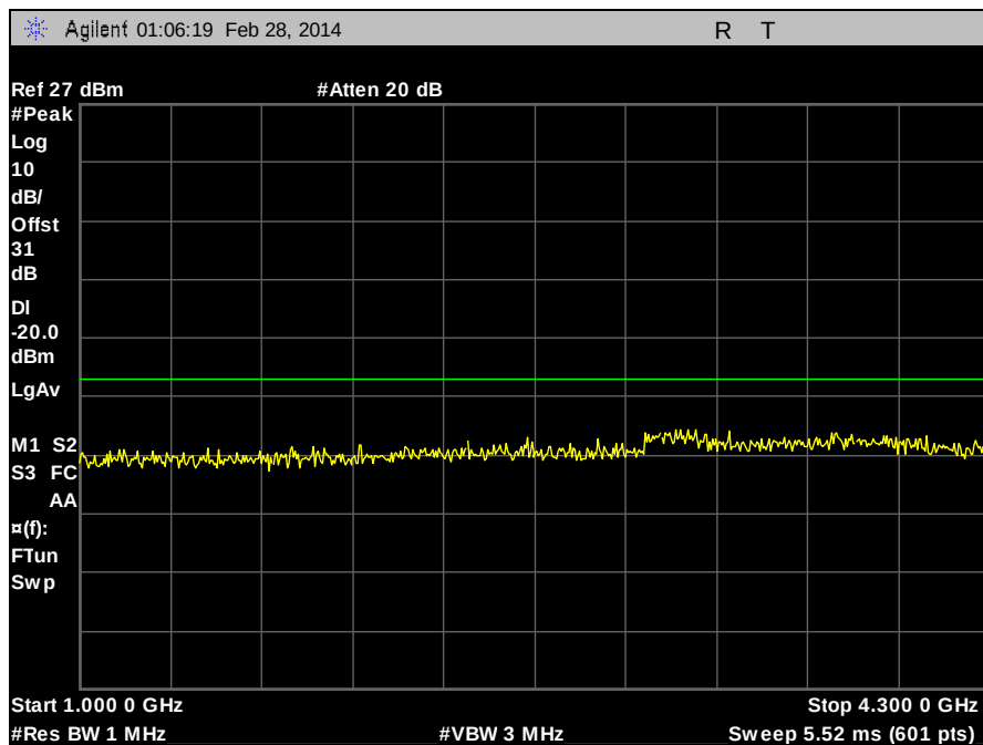
Plot 72. Part 90, Conducted Spurious Emissions, 420 MHz, HDQPSK, 100 W, 1 GHz – 4.3 GHz
