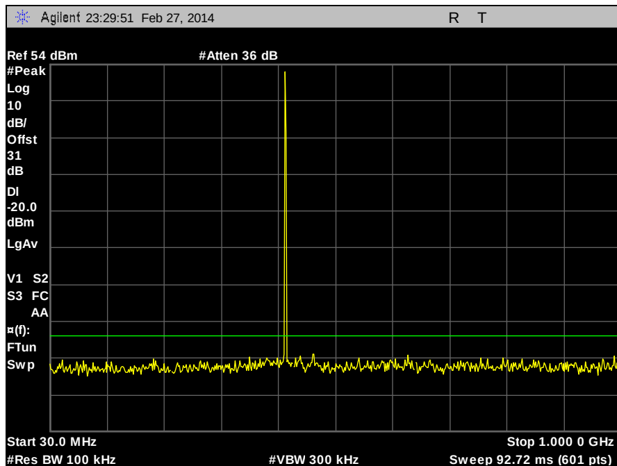
Plot 107. Part 90, Conducted Spurious Emissions, 430 MHz, HDQPSK, 100 W, 30 MHz – 1 GHz
