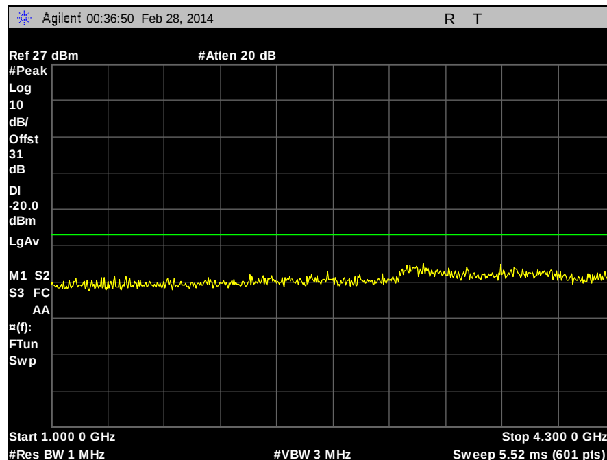
Plot 78. Part 90, Conducted Spurious Emissions, 423 MHz, HDQPSK, 10 W, 1 GHz – 4.3 GHz
