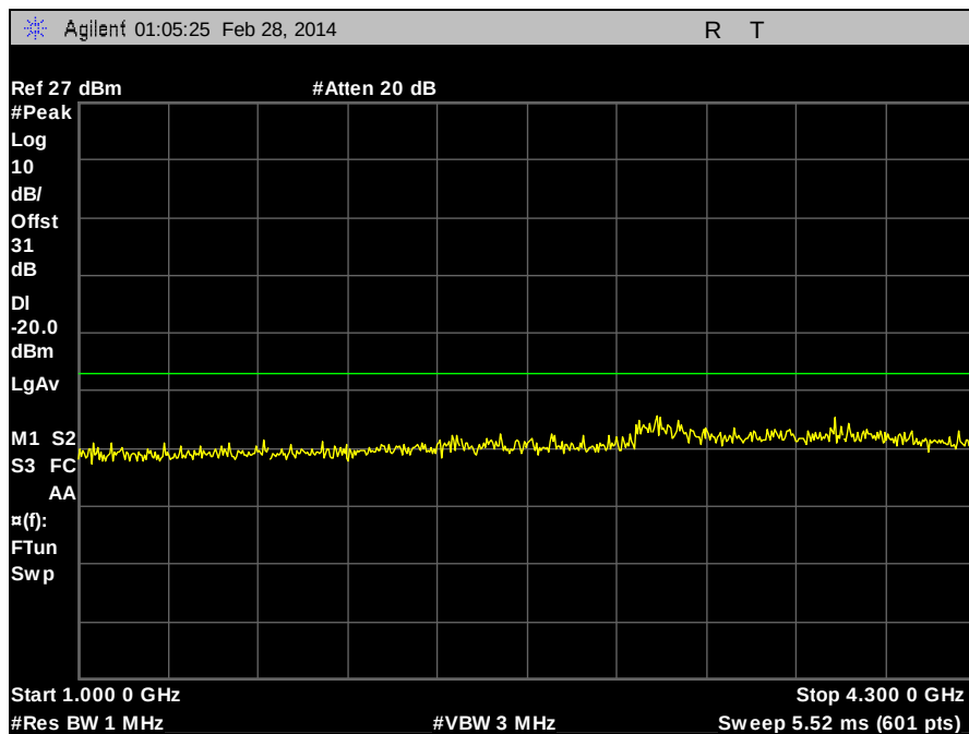
Plot 68. Part 90, Conducted Spurious Emissions, 420 MHz, C4FM, 100 W, 1 GHz – 4.3 GHz
