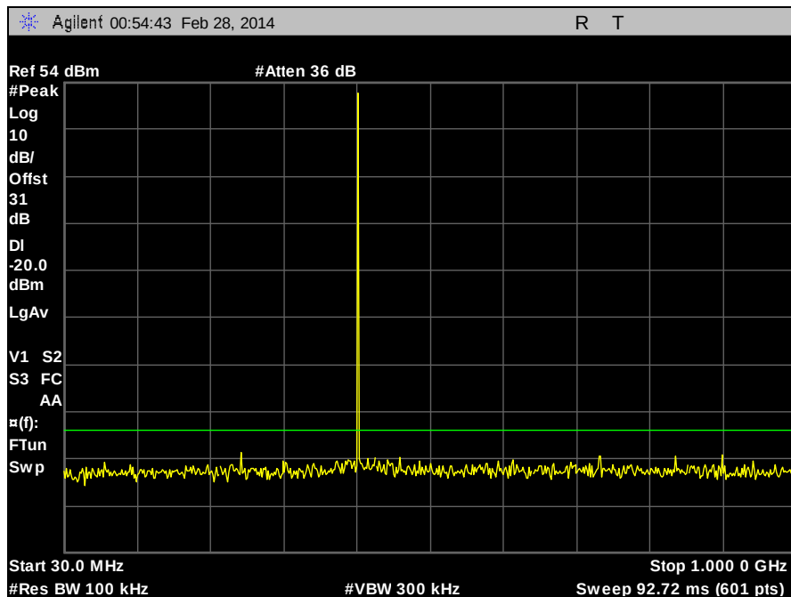
Plot 71. Part 90, Conducted Spurious Emissions, 420 MHz, HDQPSK, 100 W, 30 MHz – 1 GHz
