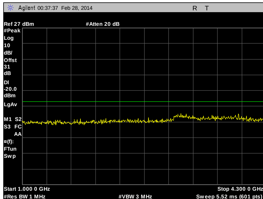
Plot 84. Part 90, Conducted Spurious Emissions, 423 MHz, HDQPSK, 100 W, 1 GHz – 4.3 GHz
