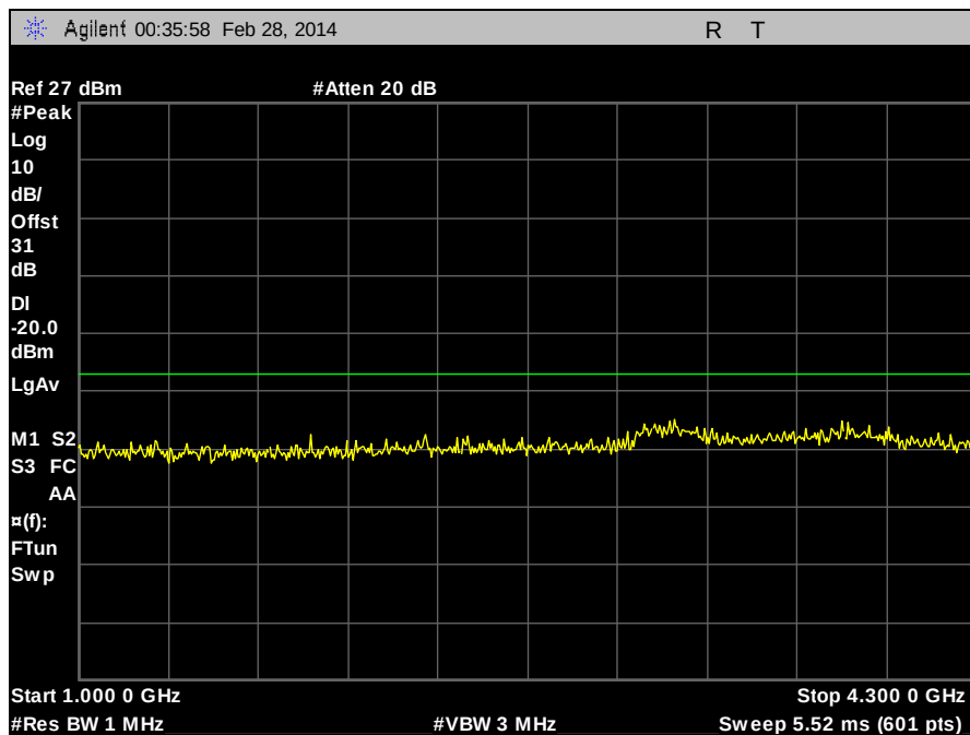
Plot 80. Part 90, Conducted Spurious Emissions, 423 MHz, C4FM, 100 W, 1 GHz – 4.3 GHz
