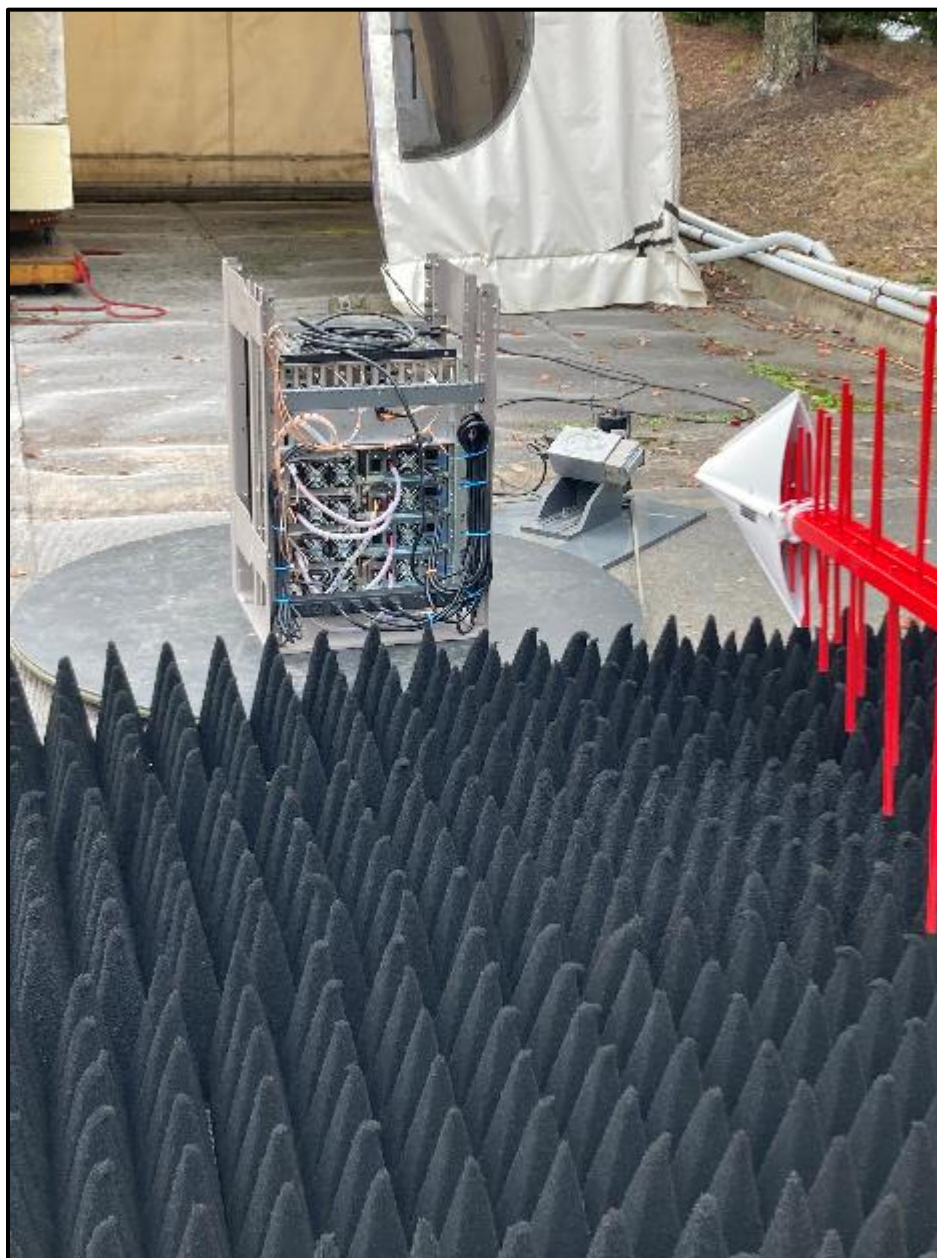
Photograph 4: Radiated Emissions – Back View (Above 1 GHz)
