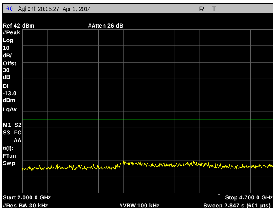
Plot 134. Part 22, Conducted Spurious Emissions, 463 MHz, C4FM, 10 W, 2 GHz – 4.7 GHz
