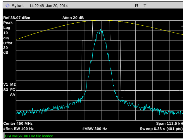
Plot 37. Part 90, Emission Mask, 450 MHz, C4FM, 10 W
