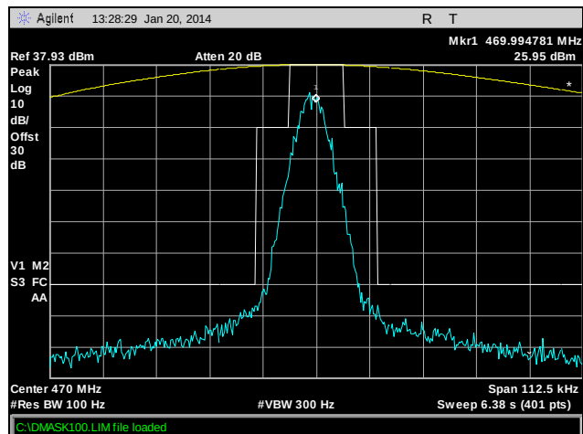
Plot 55. Part 90, Emission Mask, 470 MHz, C4FM, 10 W
