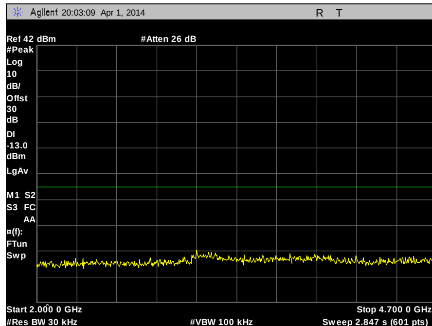
Plot 112. Part 22, Conducted Spurious Emissions, 450 MHz, CQPSK, 10 W, 2 GHz – 4.7 GHz
