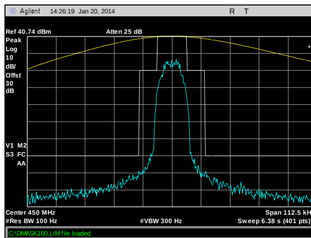
Plot 38. Part 90, Emission Mask, 450 MHz, CQPSK, 10 W
