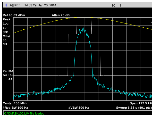
Plot 39. Part 90, Emission Mask, 450 MHz, HDQPSK, 10 W
