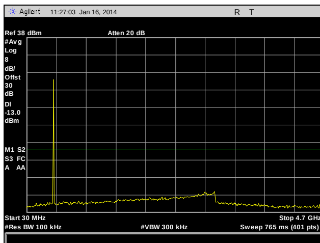
Plot 157. Part 80, Conducted Spurious Emissions, 450 MHz, C4FM, 10 W, 30 MHz – 4.7 GHz
