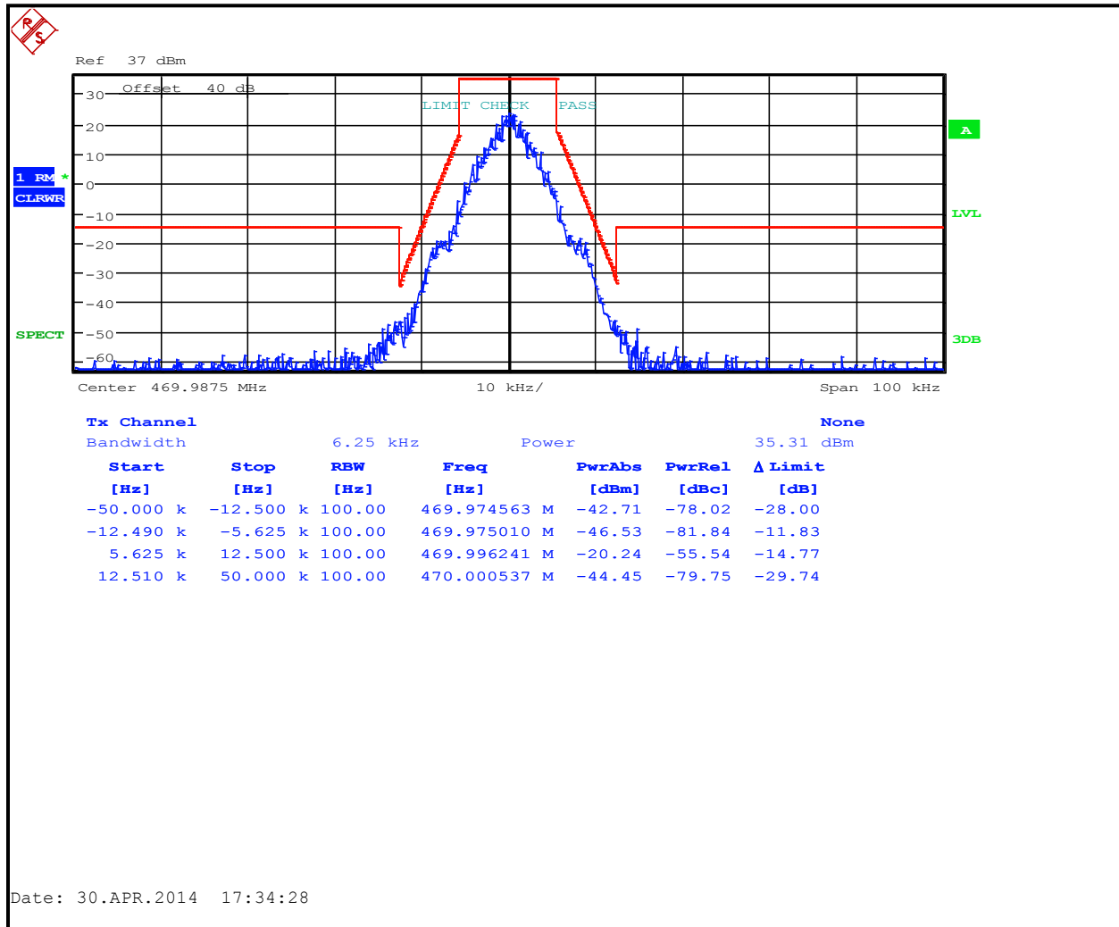
Plot 7-12: Occupied Bandwidth – 469.9875 MHz; Narrowband 2-level 9600 FSK; Mask D
