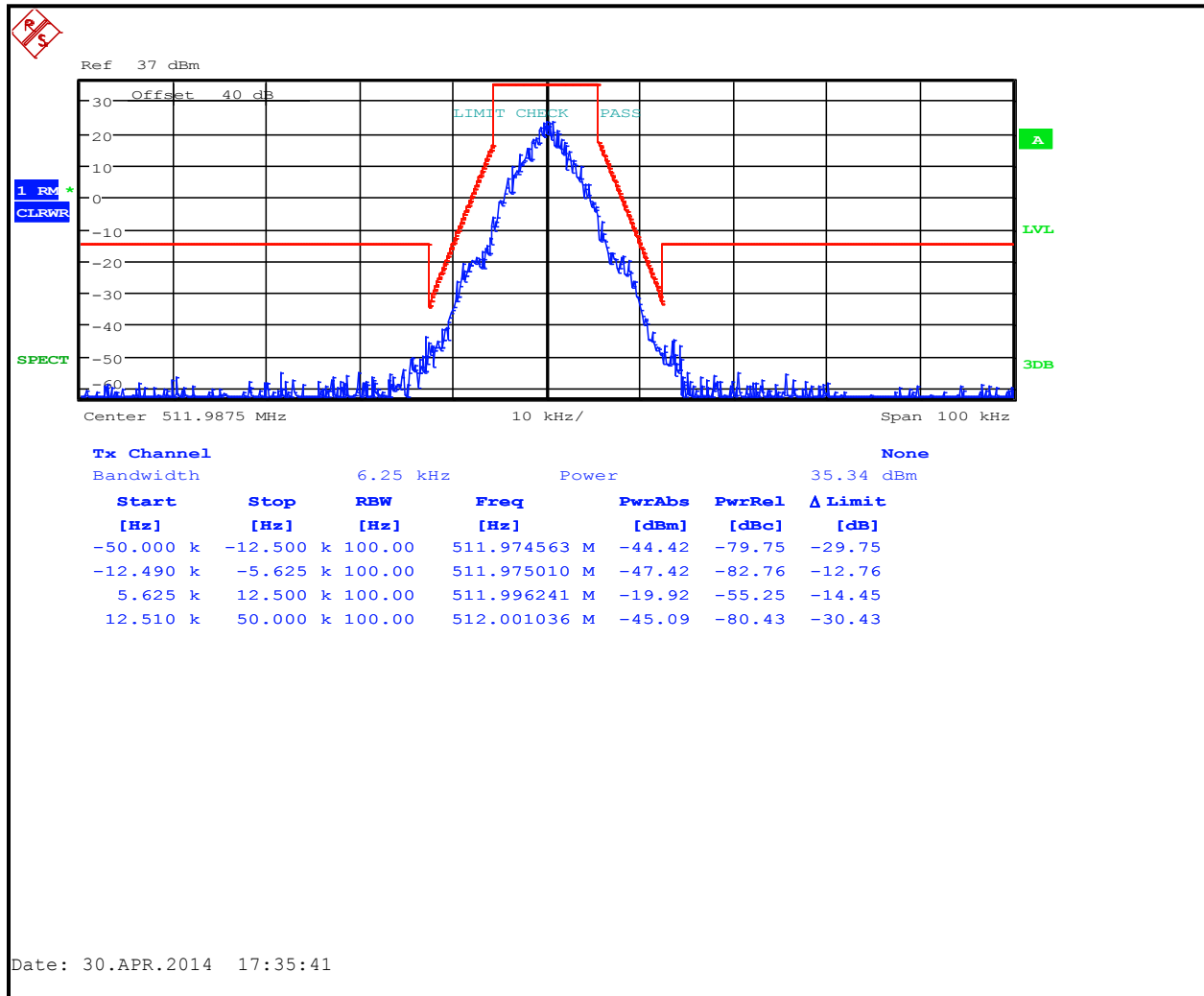
Plot 7-13: Occupied Bandwidth – 511.9875 MHz; Narrowband 2-level 9600 FSK; Mask D
