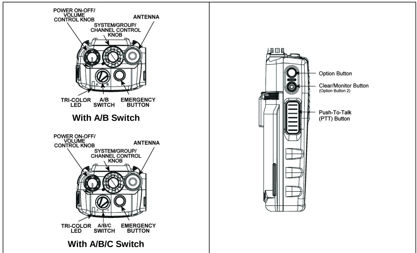
Figure 9-1: Top View
