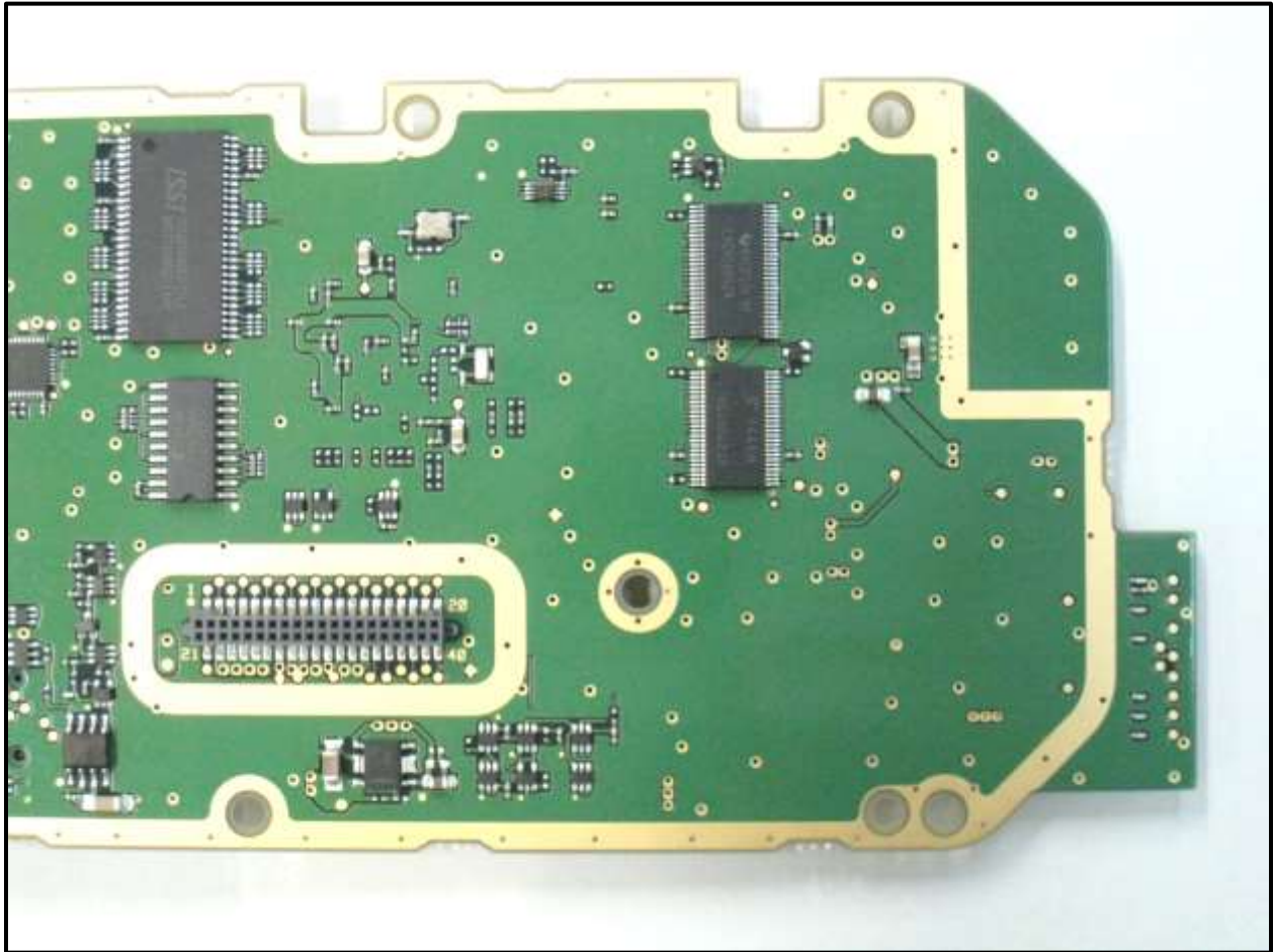
Photograph 36: PK Board – Solder Side; Right Side
