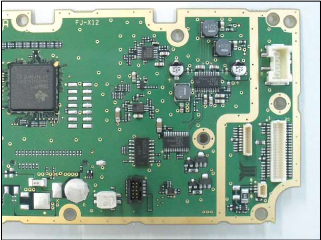
Photograph 33: PK Board – Component Side; Right Side
