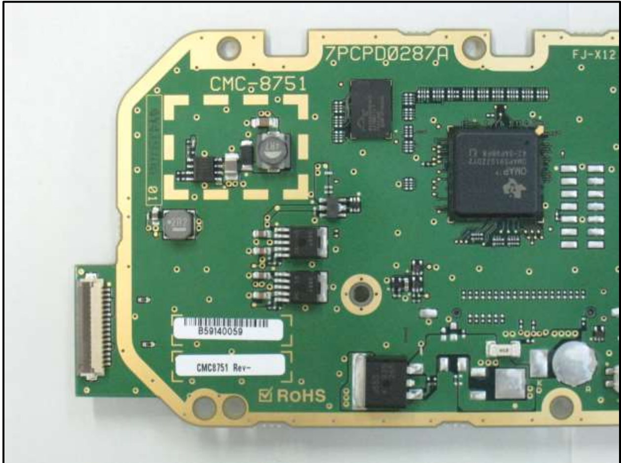
Photograph 32: PK Board – Component Side; Left Side
