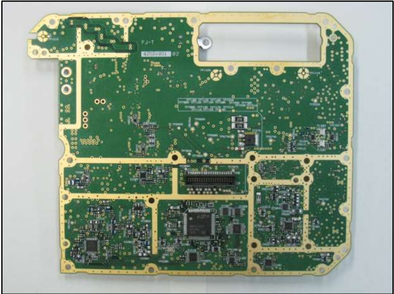
Photograph 26: RF Processor – Solder Side
