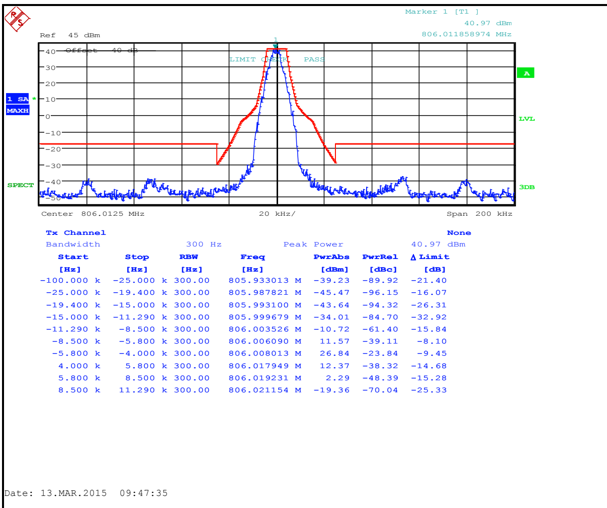
Plot 8-16: Occupied Bandwidth – 806.0125 MHz; P25; Mask H
