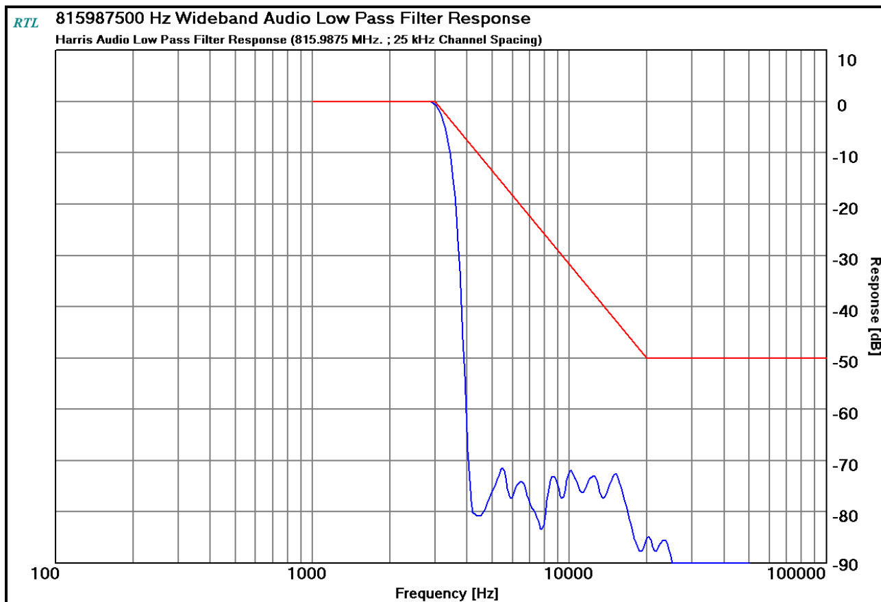
Plot 10-27: Modulation Characteristics – Audio Low Pass Filter – 815.9875 MHz
