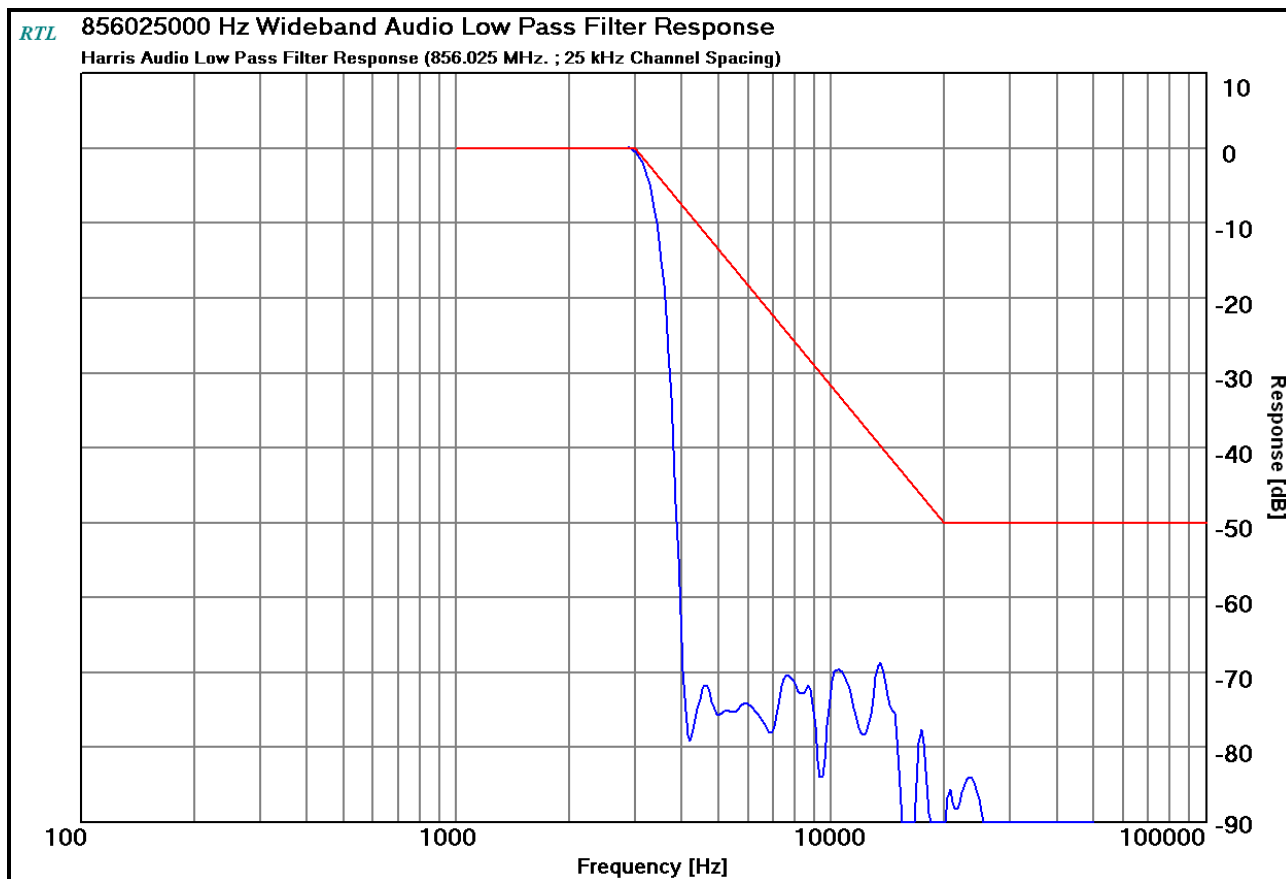
Plot 10-29: Modulation Characteristics – Audio Low Pass Filter – 856.0250 MHz
