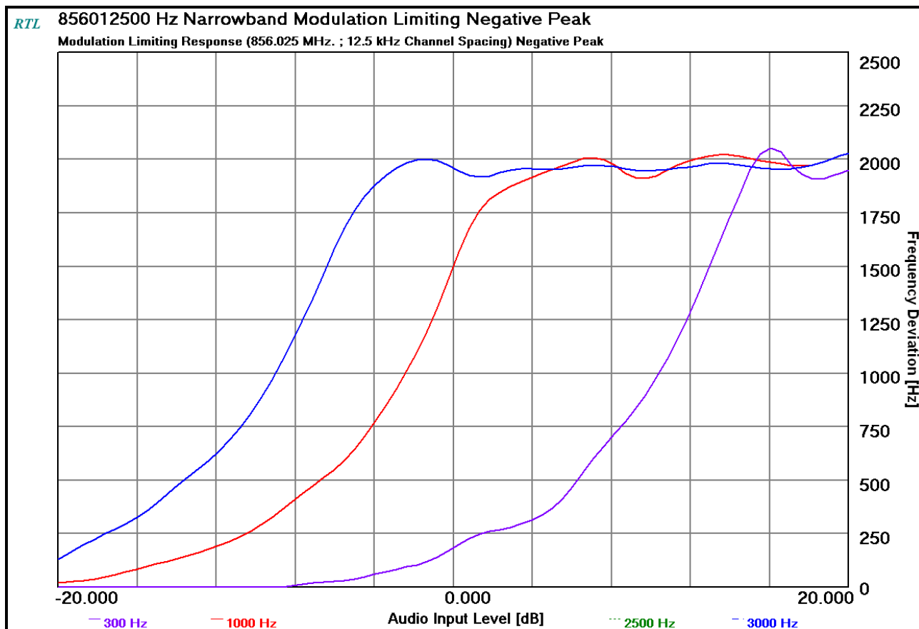
Plot 10-58: Modulation Characteristics – Modulation Limiting - 856.0250 MHz; Negative Peak; NB
