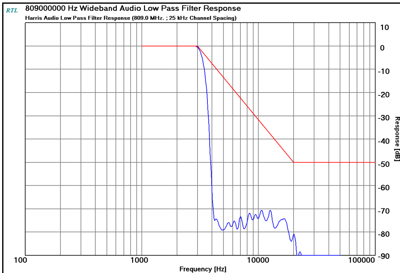
Plot 10-26: Modulation Characteristics – Audio Low Pass Filter – 809.0000 MHz
