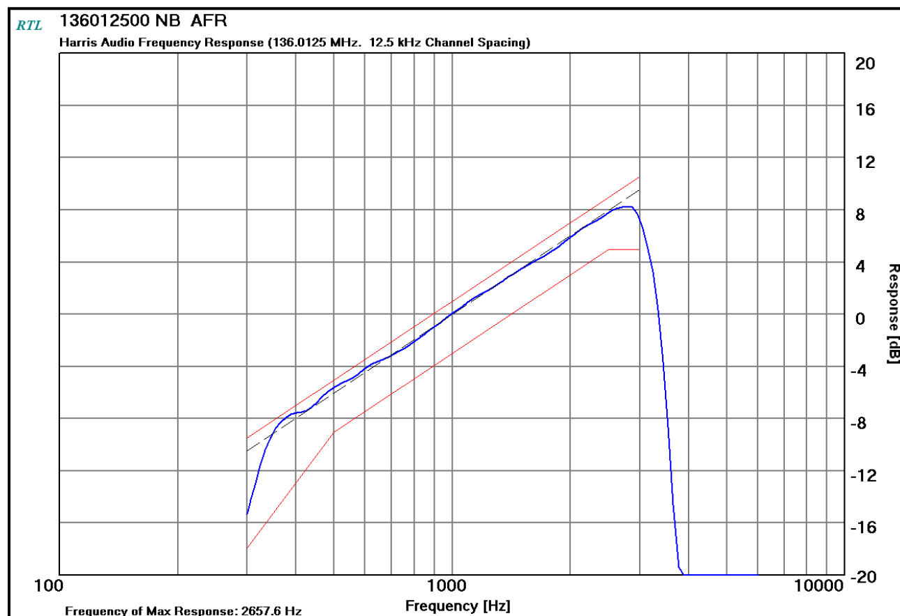
Plot 10-1: Modulation Characteristics - Audio Frequency Response – 136.0125 MHz
