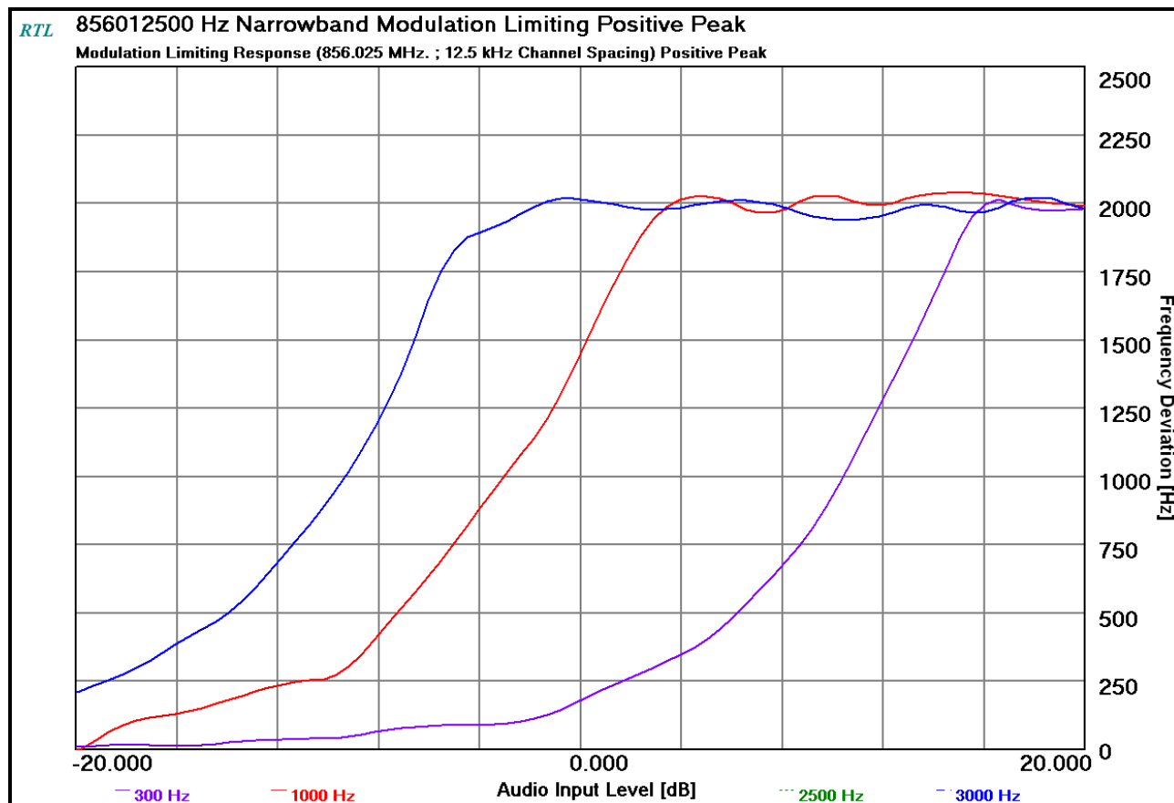
Plot 10-57: Modulation Characteristics – Modulation Limiting - 856.0250 MHz; Positive Peak; NB
