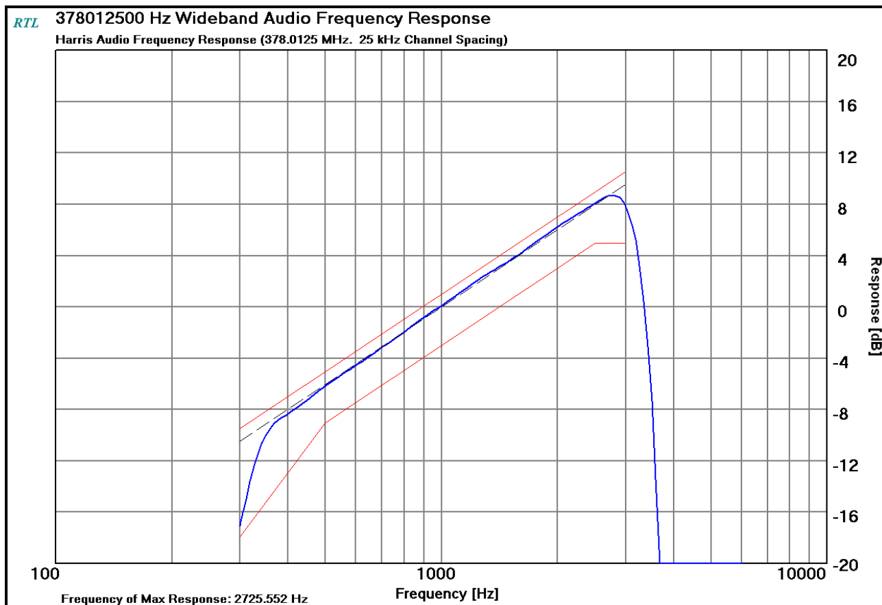
Plot 10-4: Modulation Characteristics - Audio Frequency Response – 378.0125 MHz
