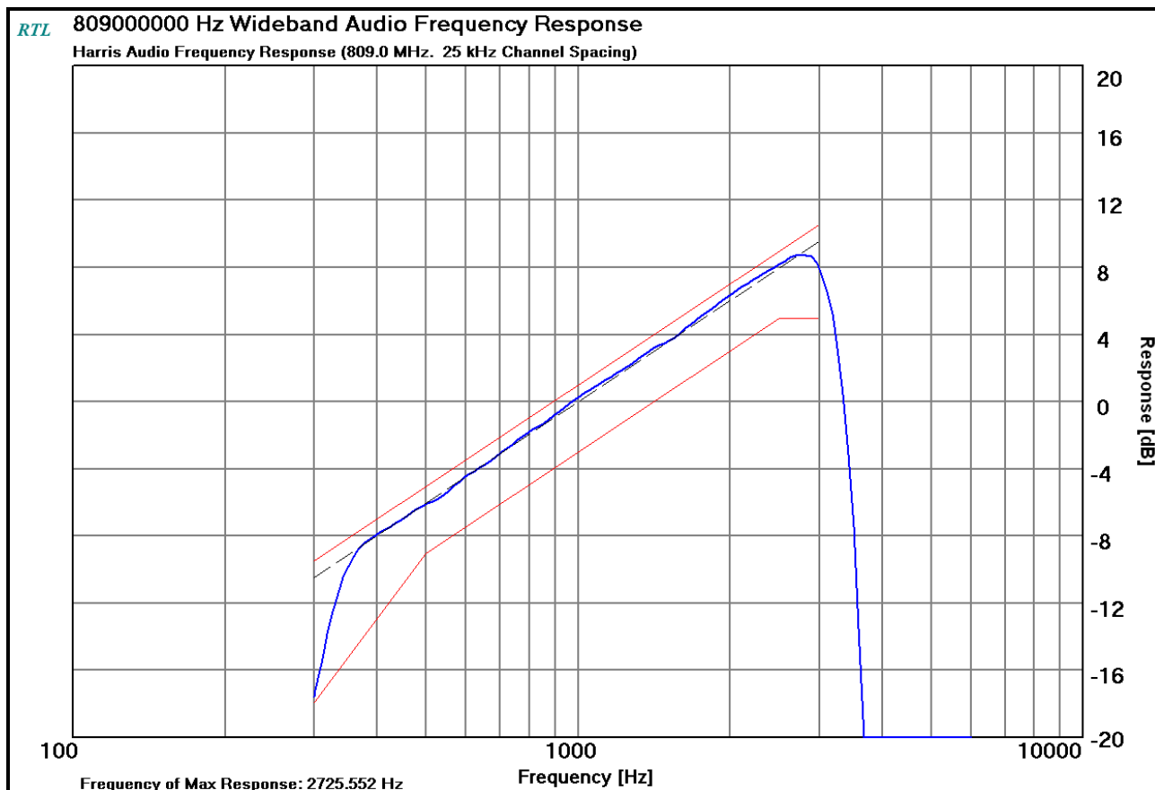
Plot 10-11: Modulation Characteristics - Audio Frequency Response – 809.0000 MHz
