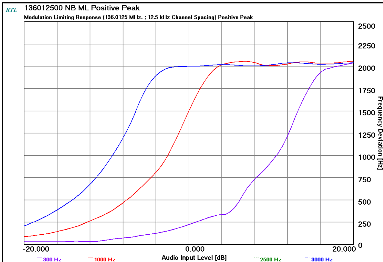
Plot 10-31: Modulation Characteristics – Modulation Limiting – 136.0125 MHz; Positive Peak; NB
