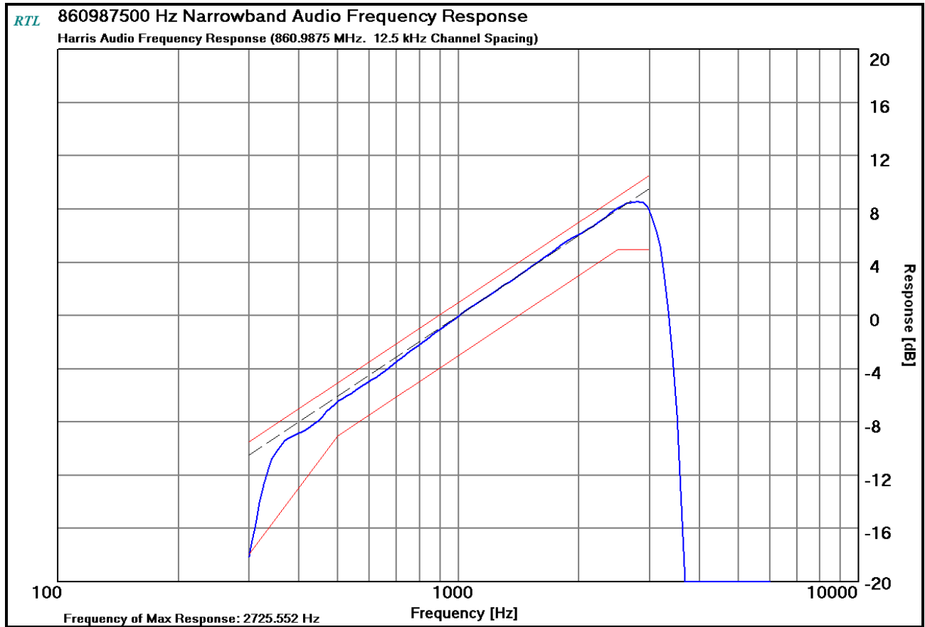
Plot 10-15: Modulation Characteristics - Audio Frequency Response – 860.9875 MHz
