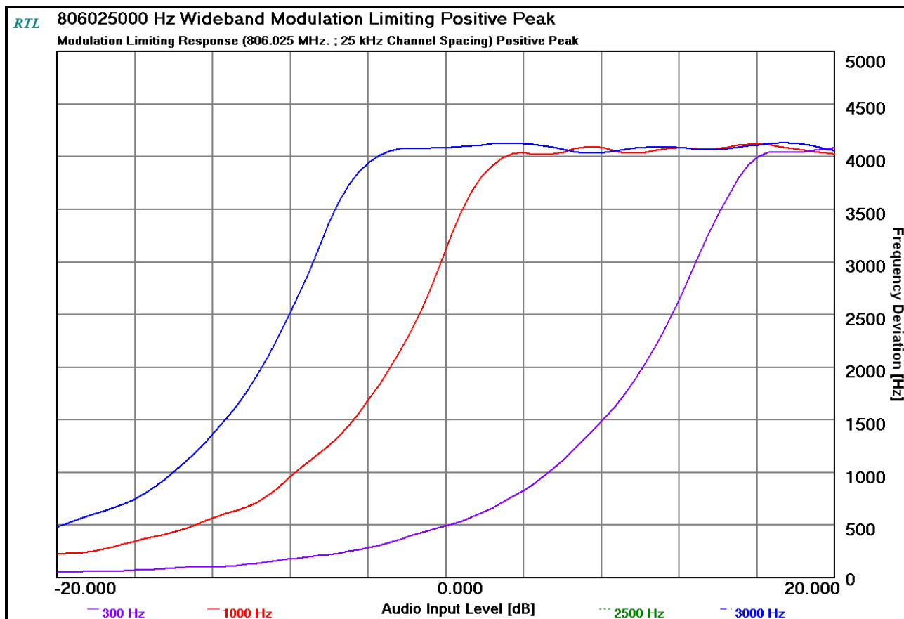
Plot 10-73: Modulation Characteristics – Modulation Limiting – 806.0250 MHz; Positive Peak; WB
