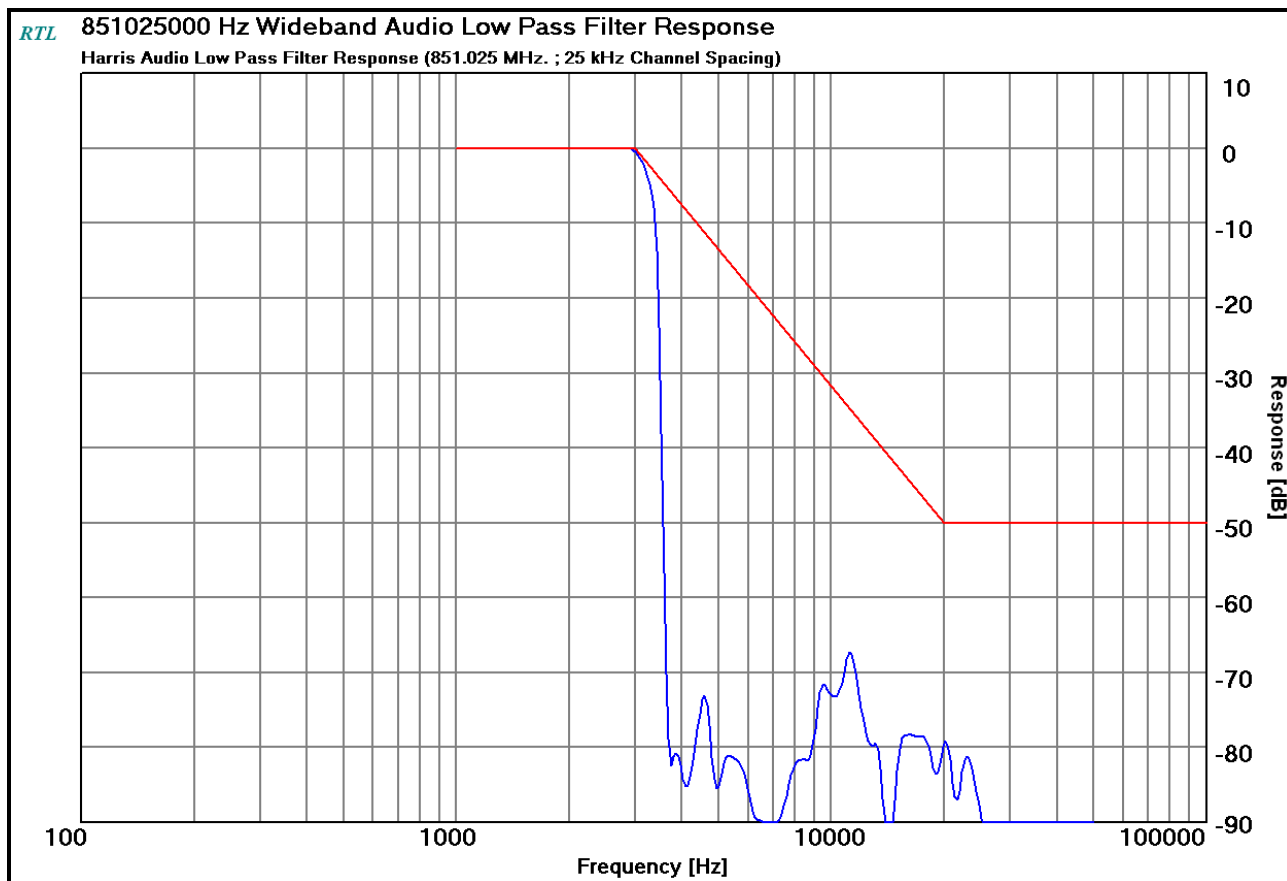
Plot 10-28: Modulation Characteristics – Audio Low Pass Filter – 851.0250 MHz
