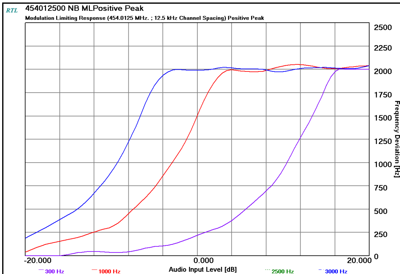
Plot 10-39: Modulation Characteristics – Modulation Limiting – 454.0125 MHz; Positive Peak; NB
