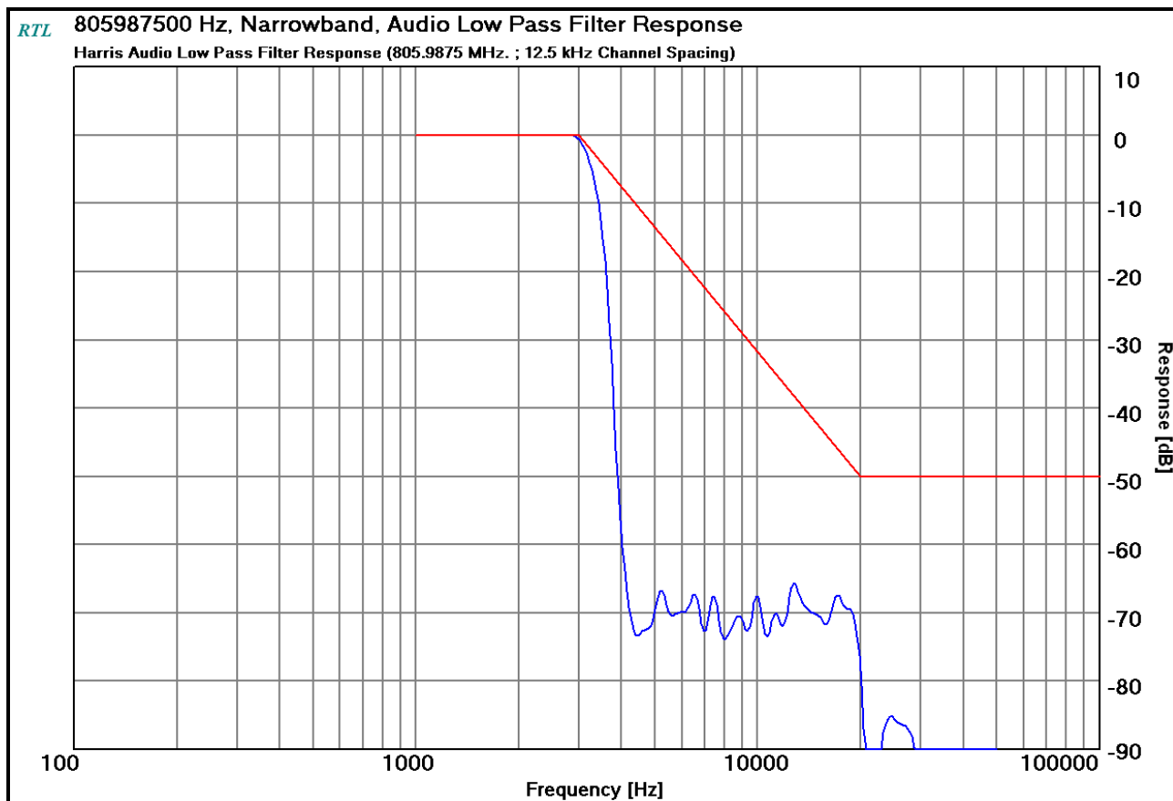
Plot 10-24: Modulation Characteristics – Audio Low Pass Filter – 805.9875 MHz
