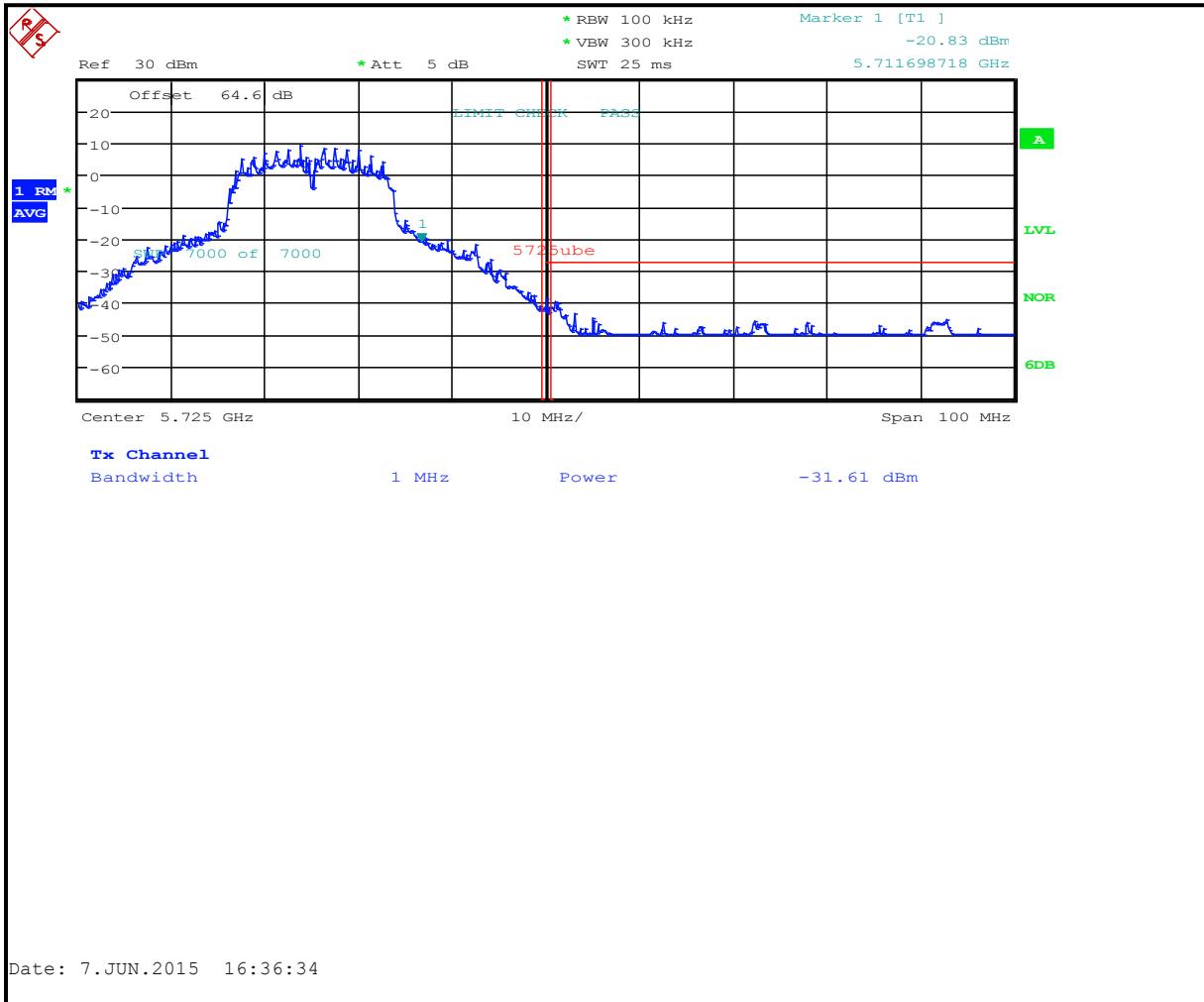
Plot 6-28: Upper Band Edge: Measurement Channel 140 (5700 MHz, 802.11n, Average)
