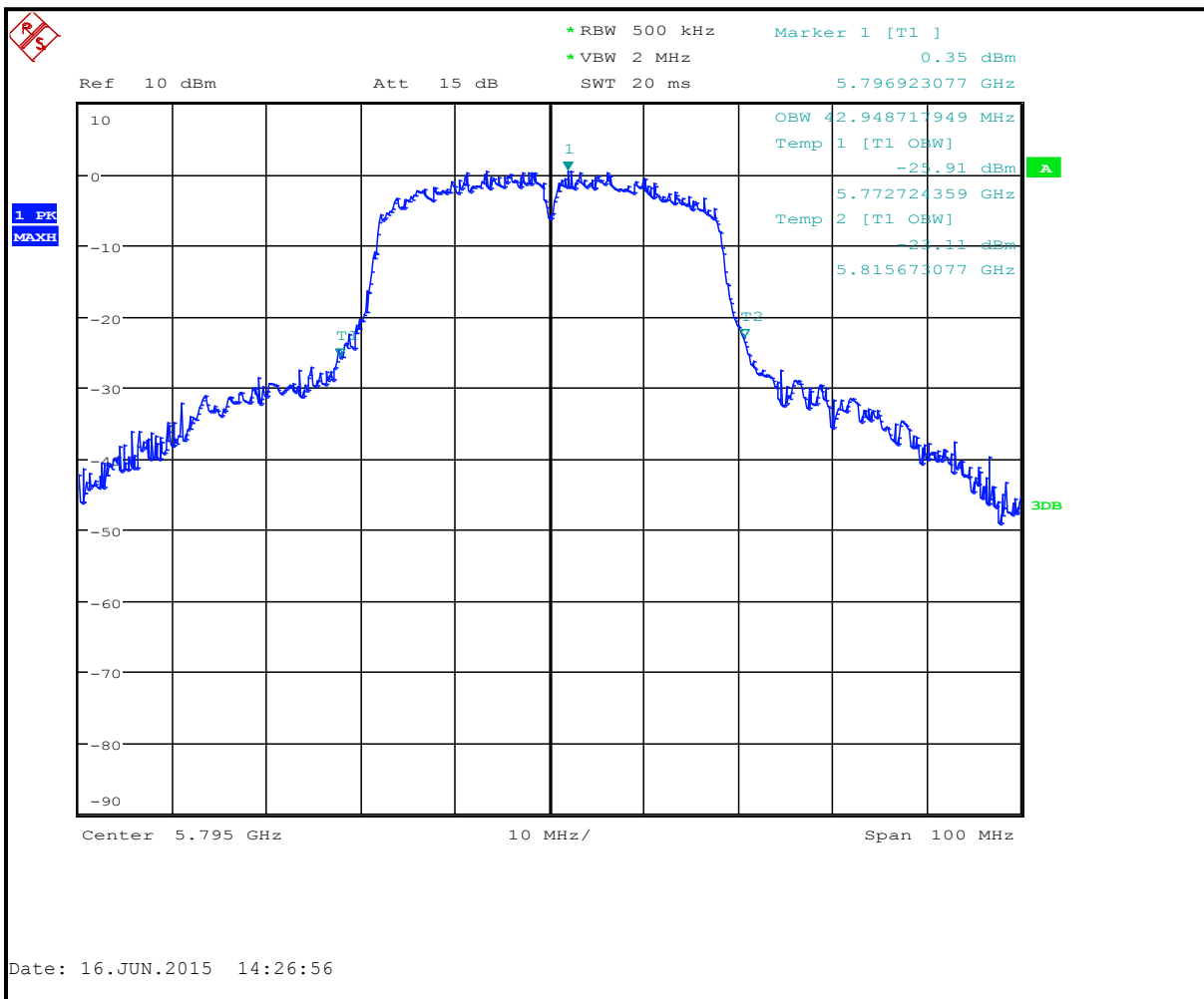
Plot 8-51: 26 dB Bandwidth (Frequency 5795 MHz) - 802.11n (40 MHz BW)
