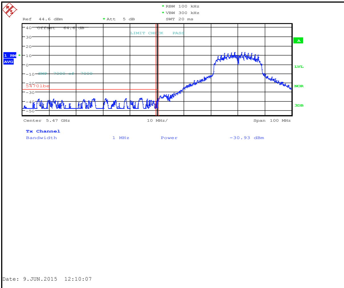
Plot 6-18: Lower Band Edge: Measurement Channel 100 (5500 MHz, 802.11a, Average)
