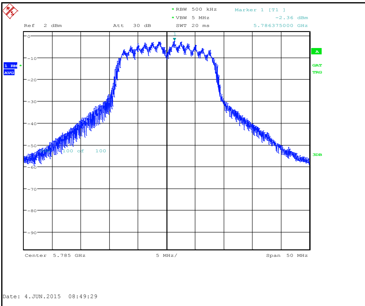
Plot 4-25: Power Spectral Density: Channel 157 (5785 MHz) 802.11n 65 Mbps
