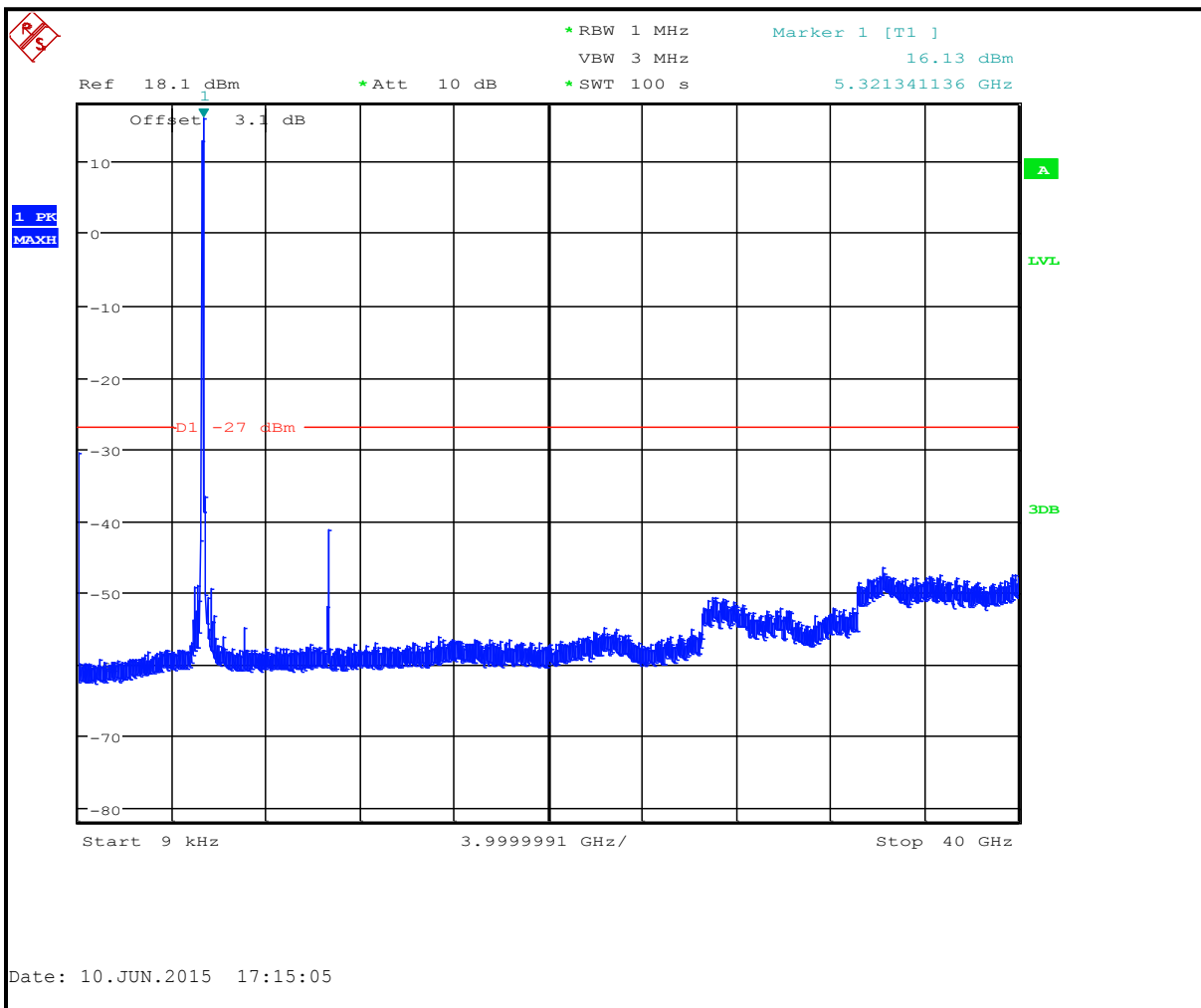
Plot 7-9: Undesirable Emissions Channel 64 (5320 MHz)
