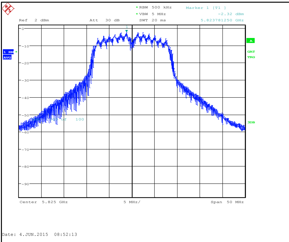
Plot 4-26: Power Spectral Density: Channel 165 (5825 MHz) 802.11n 65 Mbps
