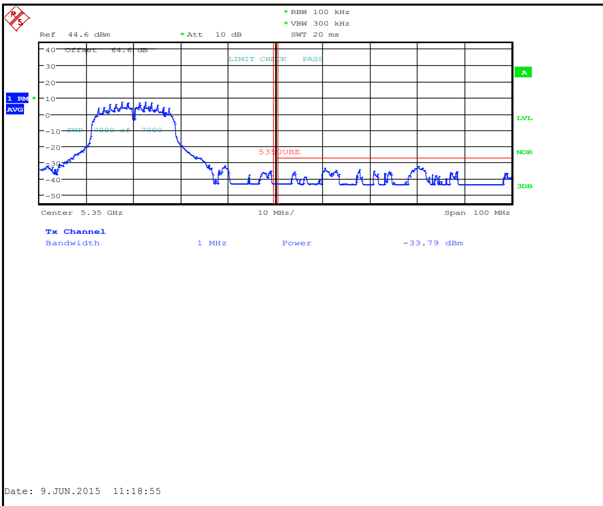
Plot 6-10: Upper Band Edge: Measurement Channel 64 (5320 MHz, 802.11a, Average)
