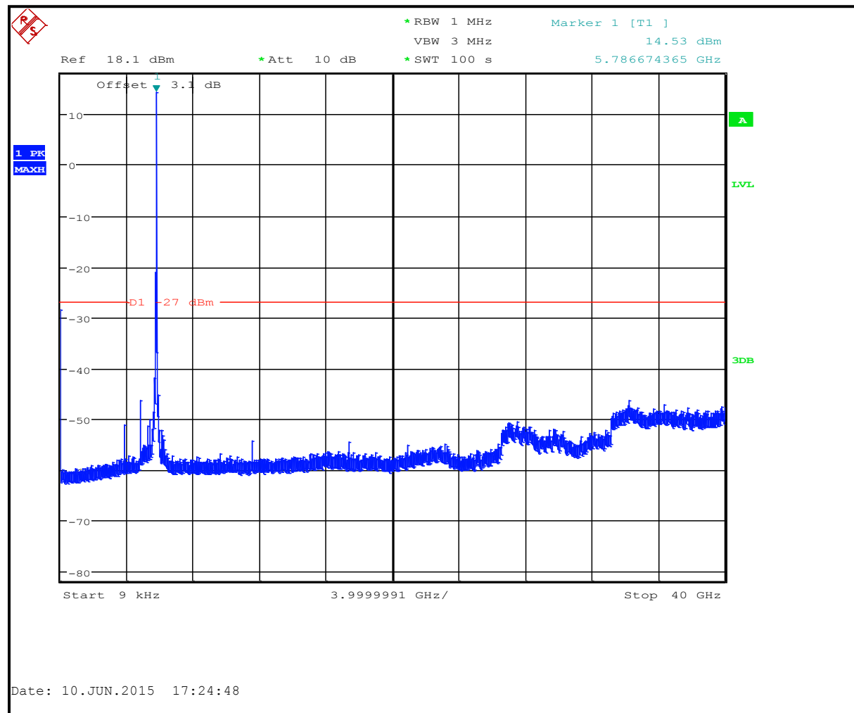
Plot 7-14: Undesirable Emissions Channel 157(5785 MHz)
