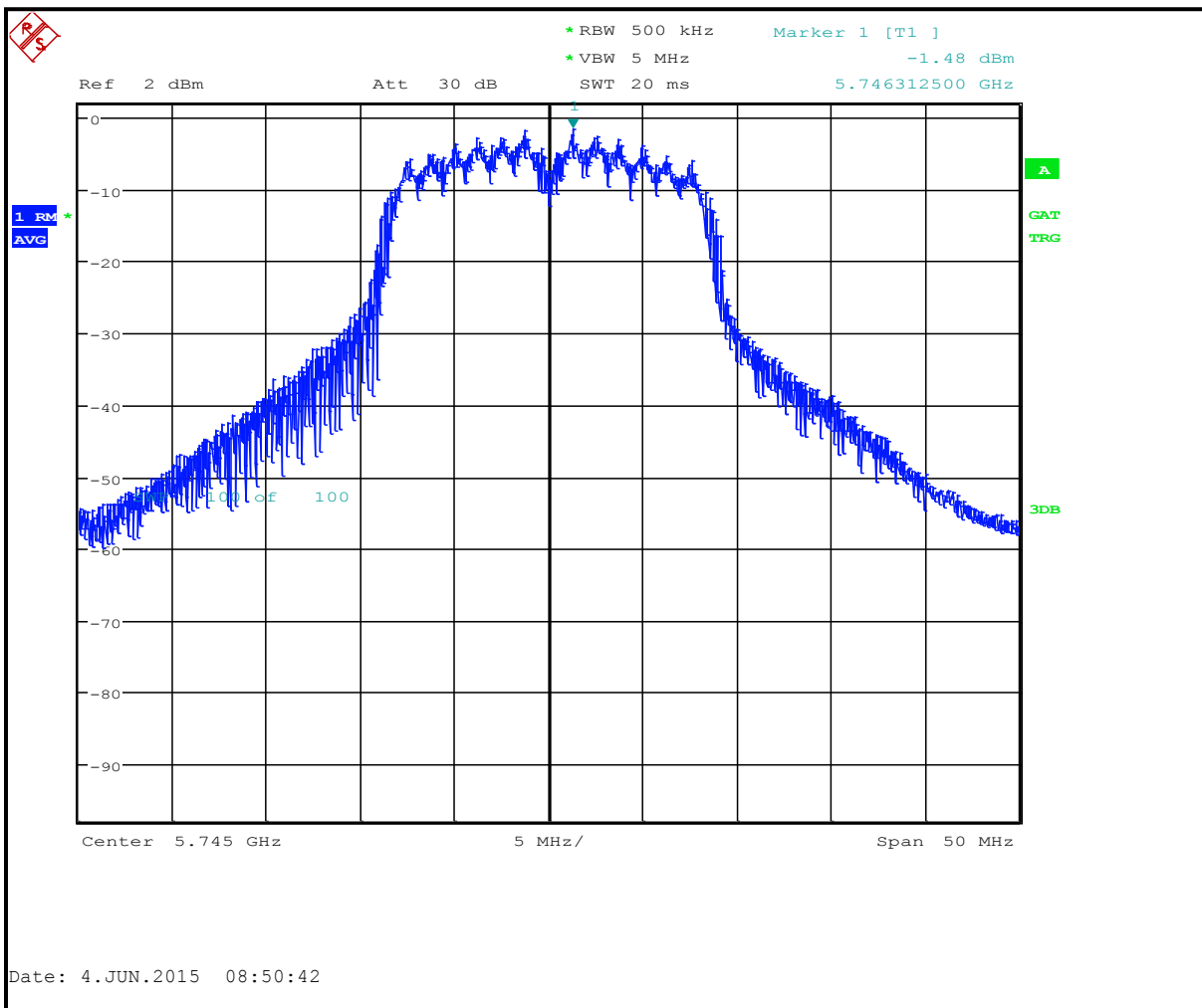
Plot 4-24: Power Spectral Density: Channel 149 (5745 MHz) 802.11n 65 Mbps
