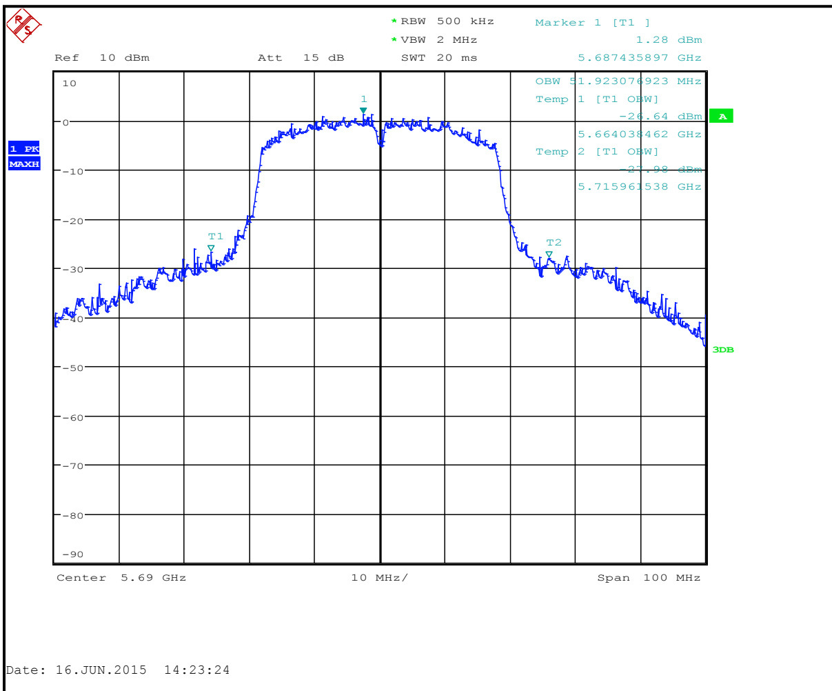
Plot 8-49: 26 dB Bandwidth (Frequency 5690 MHz) - 802.11n (40 MHz BW)
