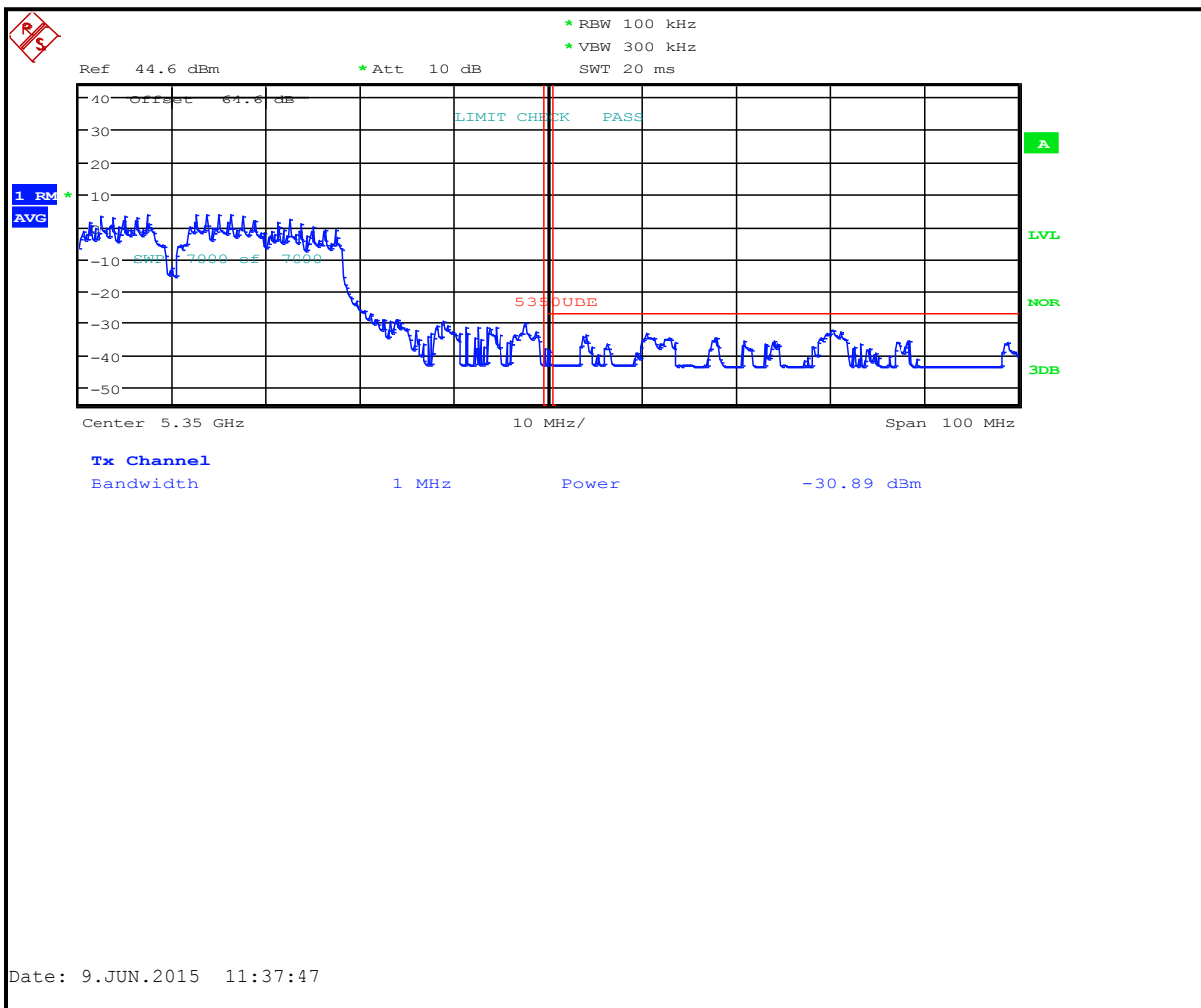
Plot 6-16: Upper Band Edge: Measurement Channel 64 (5320 MHz, 40 MHz BW, 802.11n, Average)
