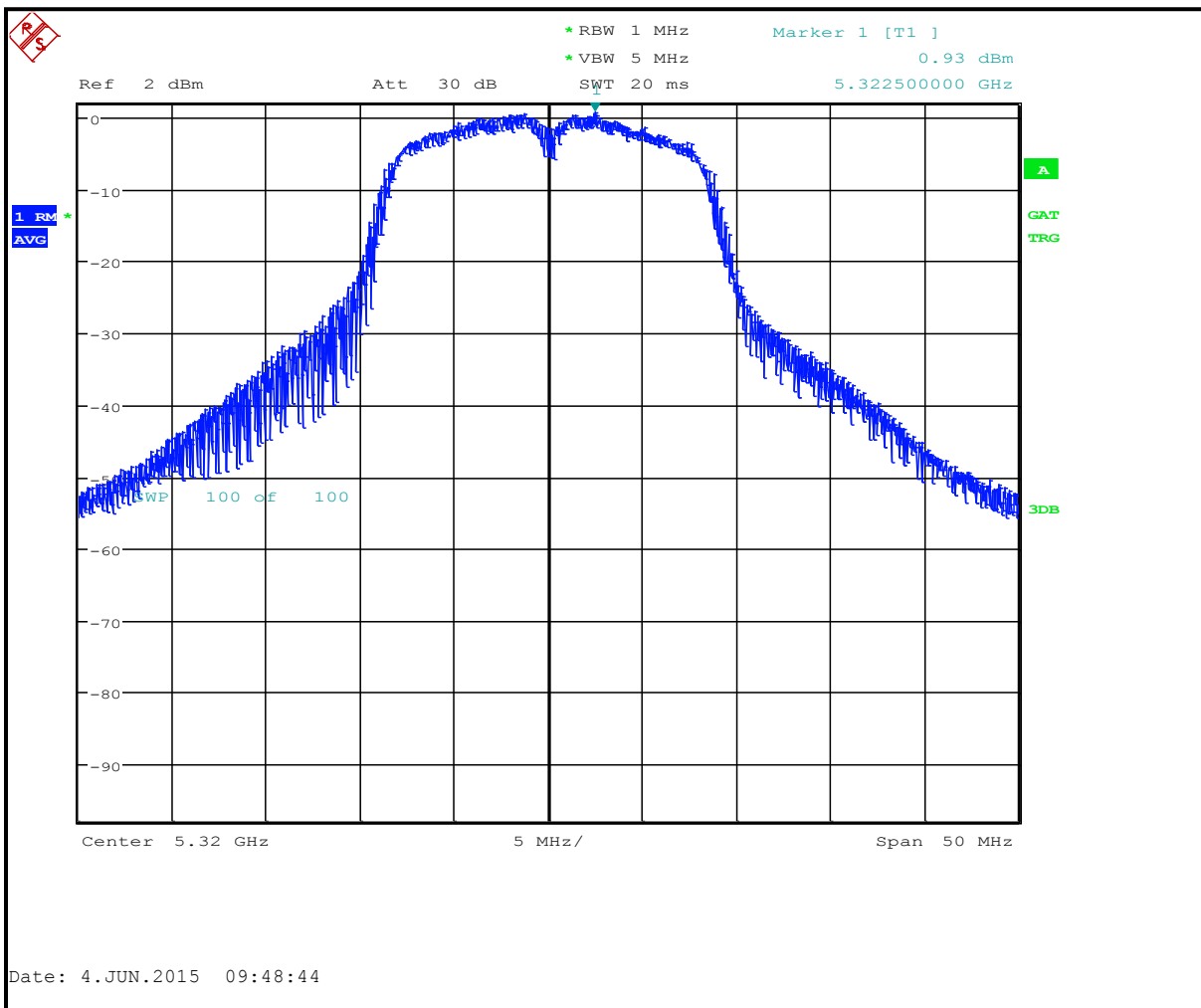
Plot 4-20: Peak Power Spectral Density: Channel 64 (5320 MHz) 802.11n 65 Mbps
