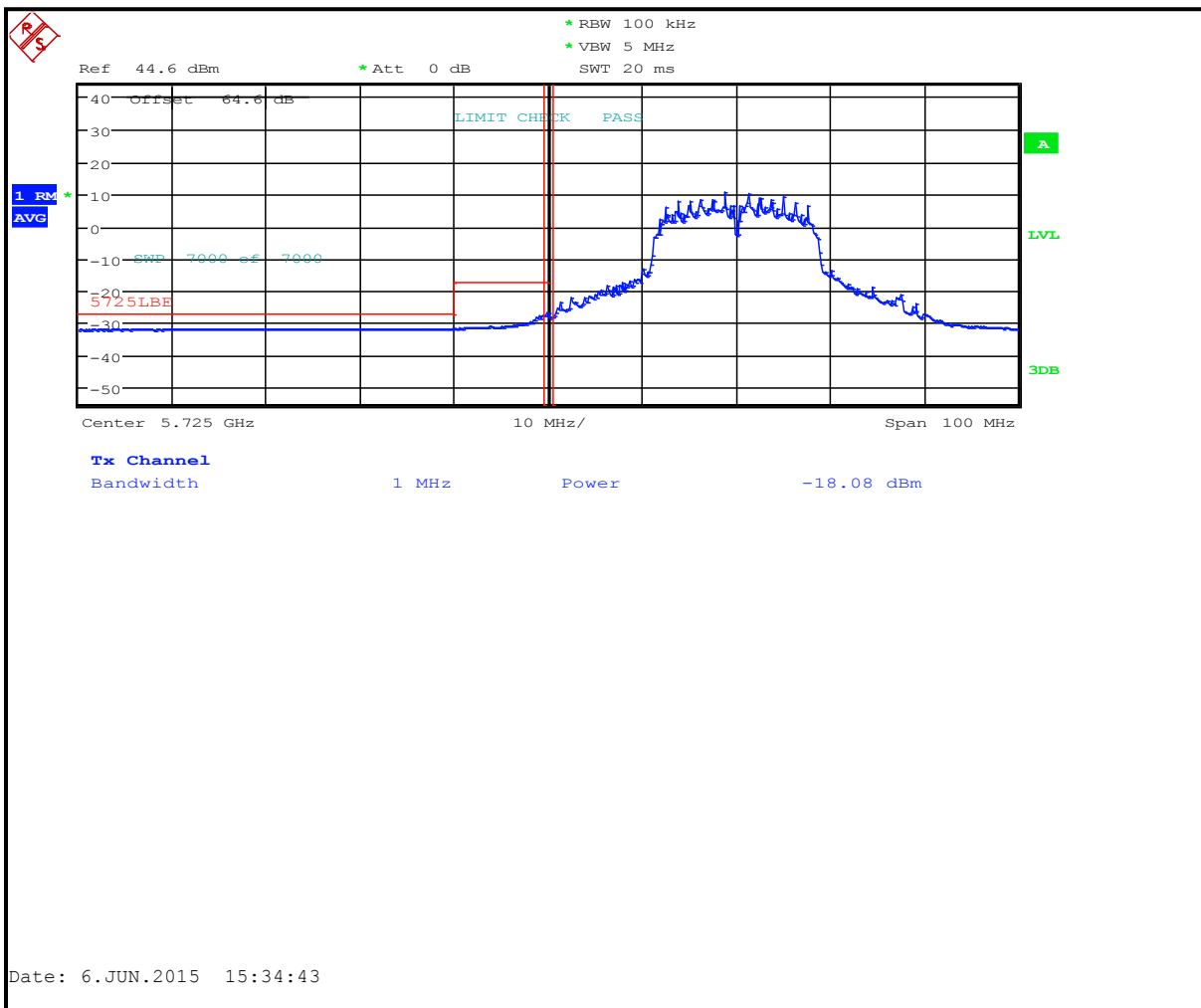
Plot 6-36: Lower Band Edge: Measurement Channel 149 (5745 MHz, 802.11n, Average)
