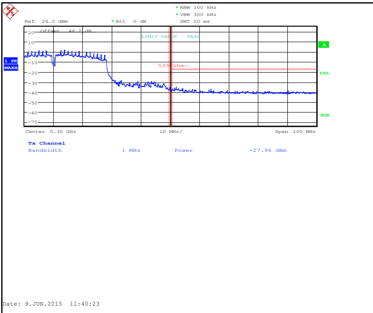
Plot 6-15: Upper Band Edge: Measurement Channel 64 (5320 MHz, 40 MHz BW, 802.11n, Peak)
