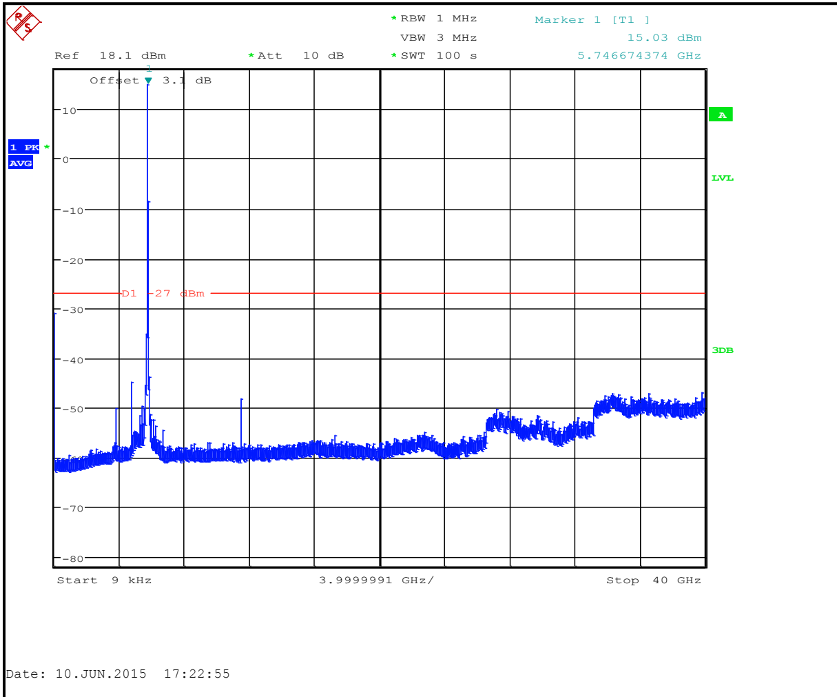
Plot 7-13: Undesirable Emissions Channel 149 (5745 MHz)
