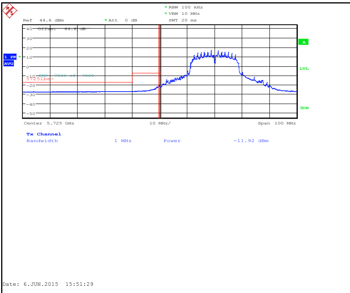
Plot 6-33: Lower Band Edge: Measurement Channel 149 (5745 MHz, 802.11a, Peak)
