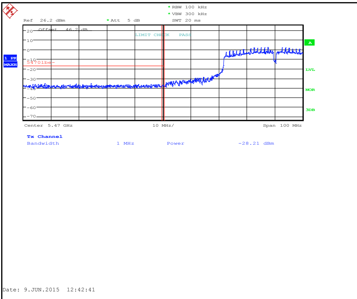
Plot 6-21: Lower Band Edge: Measurement Channel 100 (5500 MHz, 40 MHz BW, 802.11a, Peak)
