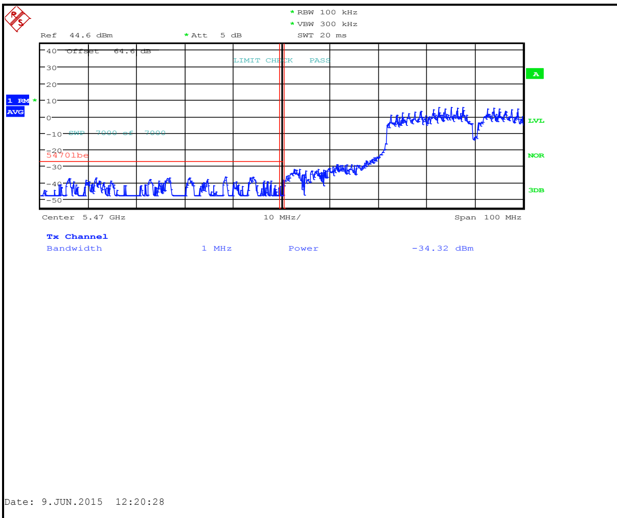
Plot 6-22: Lower Band Edge: Measurement Channel 100 (5500 MHz, 40 MHz BW, 802.11a, Average)
