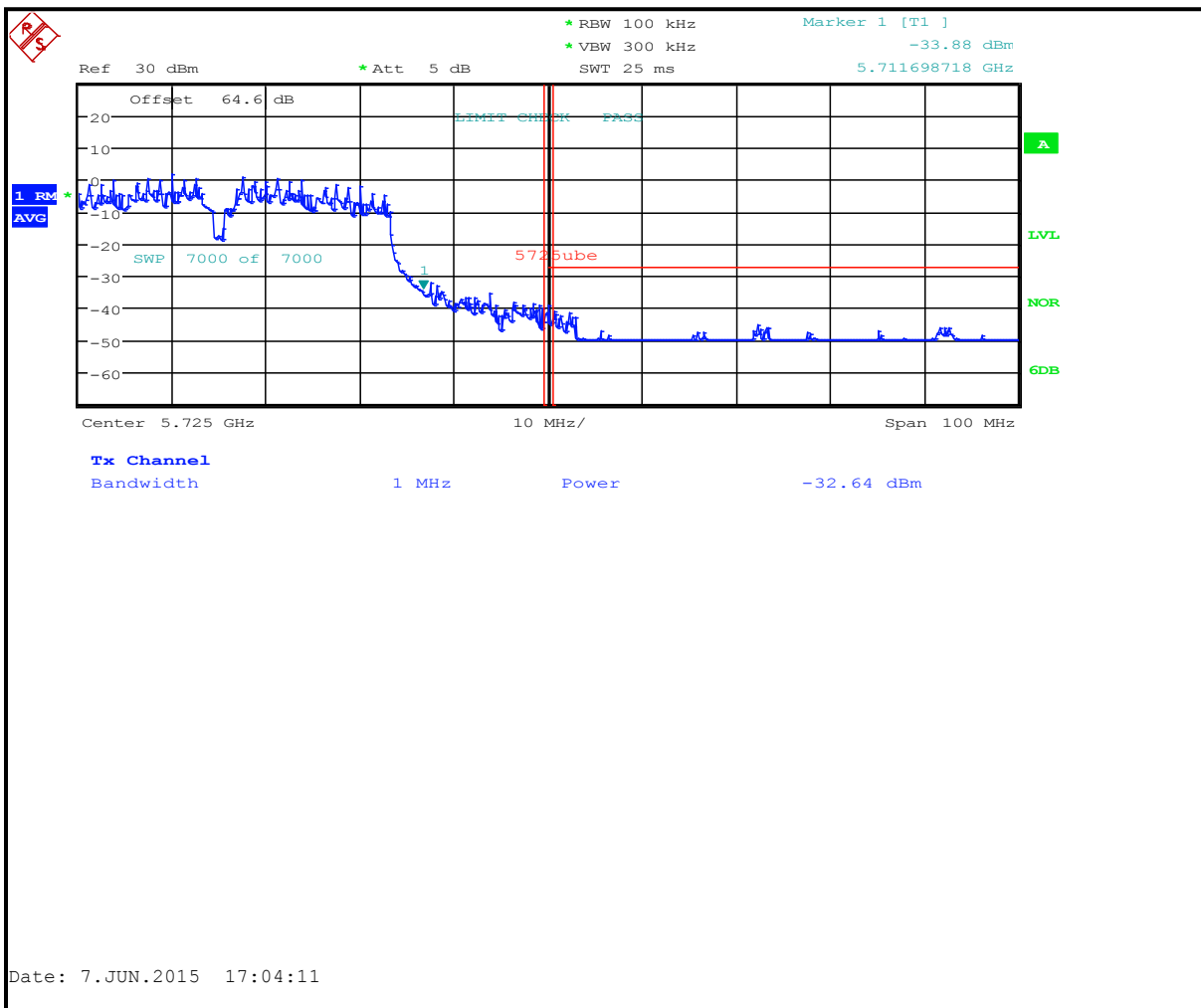
Plot 6-32: Upper Band Edge: Measurement Channel 140 (5700 MHz, 40 MHz BW, 802.11n, Average)
