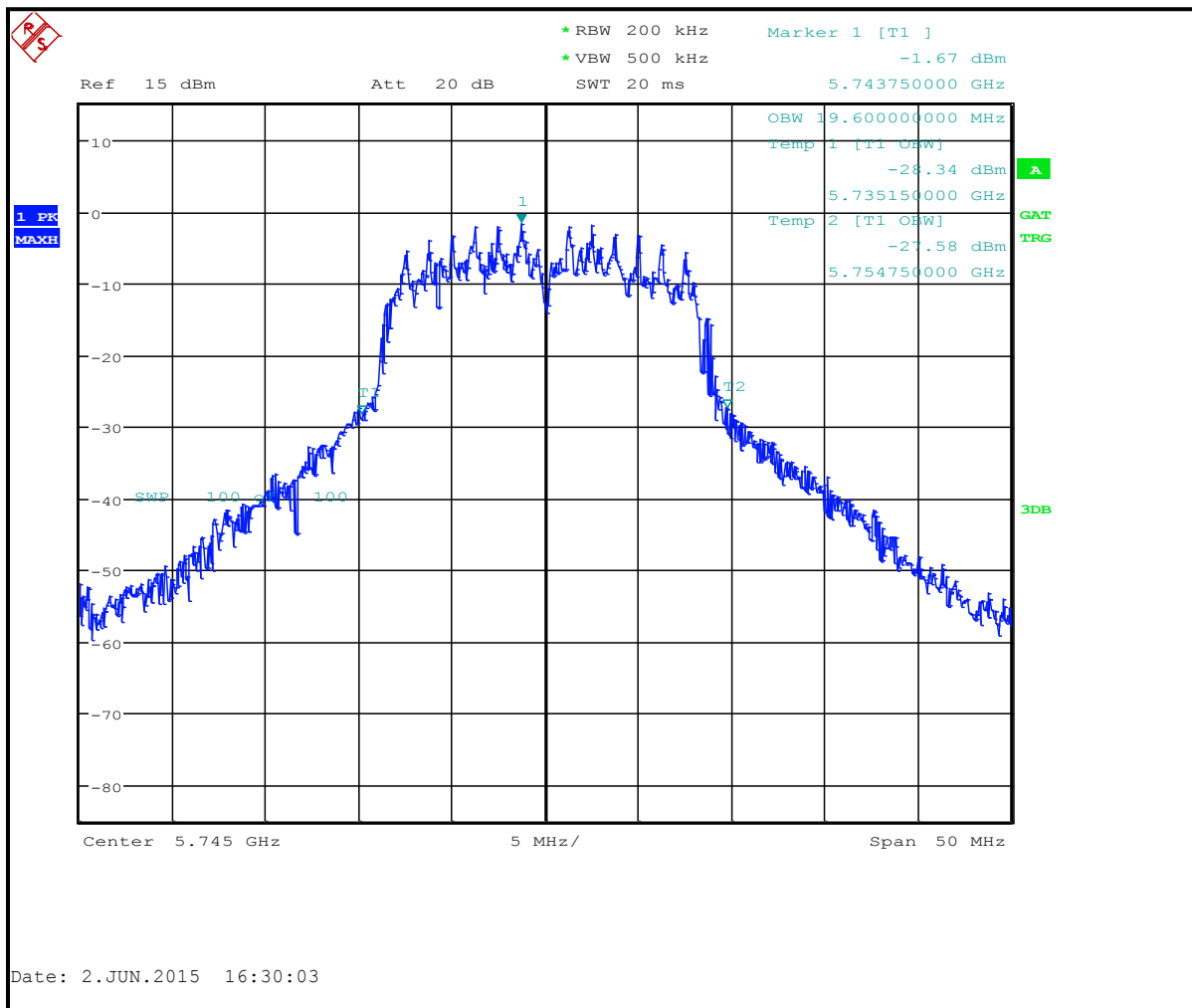
Plot 8-11: 26 dB Bandwidth Channel 149 (TX Frequency 5745 MHz) - 802.11a
