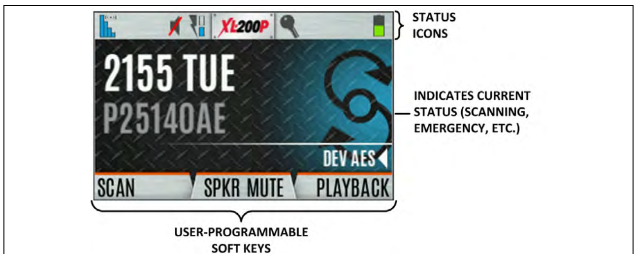
Figure 4-4: Sample Idle Front Display
