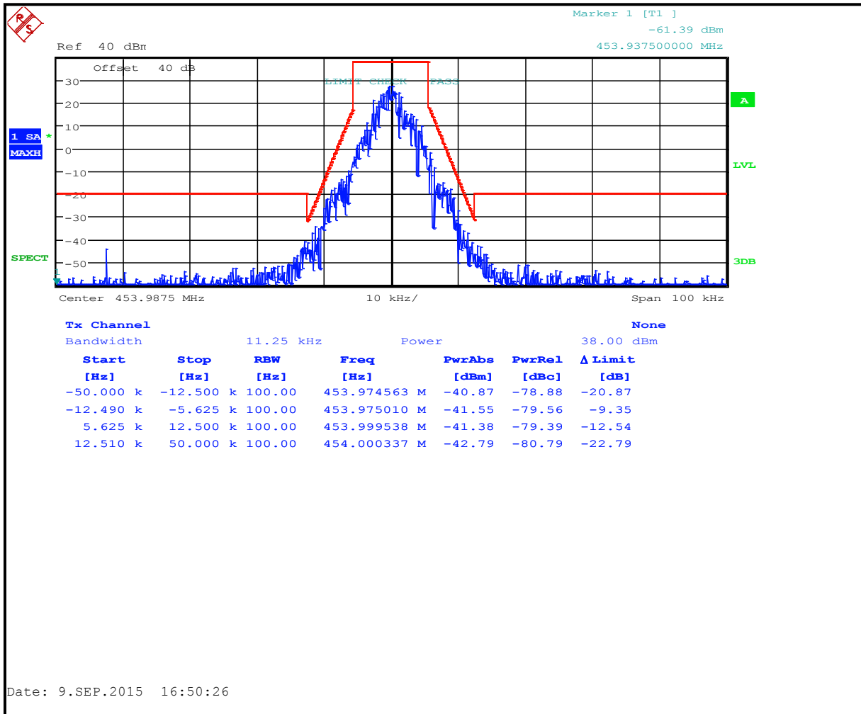
Plot 7-16: Occupied Bandwidth – 453.9875 MHz; Narrowband 2-level 9600 FSK; Mask D
