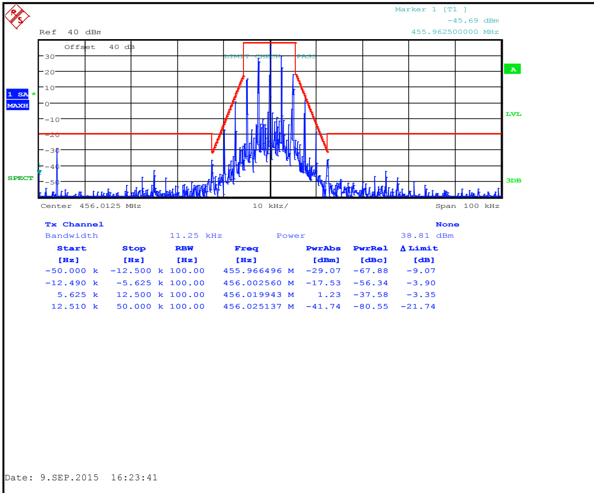
Plot 7-11: Occupied Bandwidth – 456.0125 MHz; Narrowband Analog; Mask D
