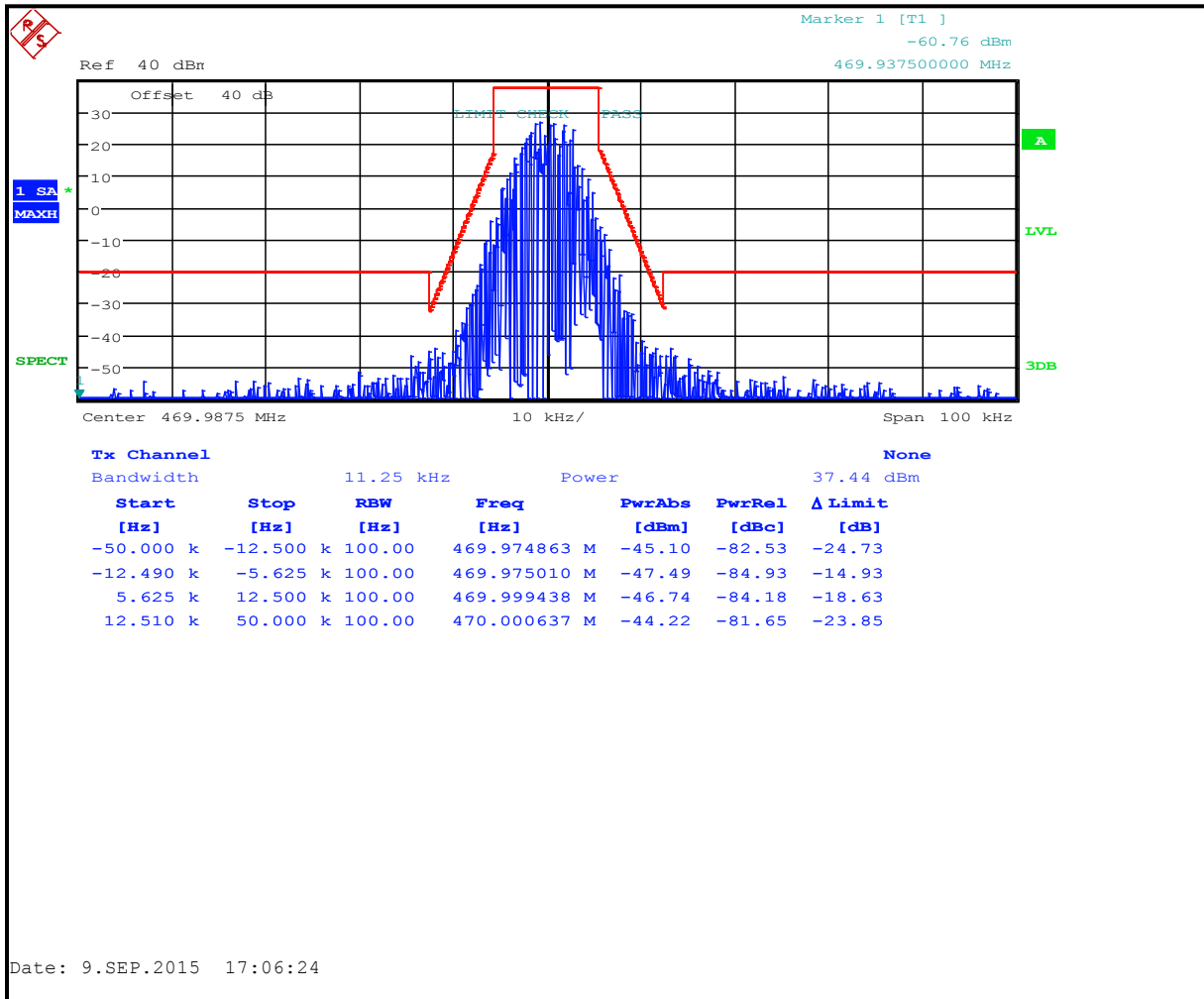
Plot 7-26: Occupied Bandwidth – 469.9875 MHz; Narrowband H-CPM TDMA; Mask D
