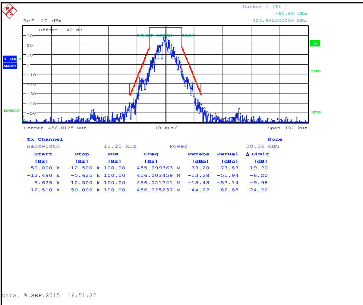
Plot 7-18: Occupied Bandwidth – 456.0125 MHz; Narrowband 2-level 9600 FSK; Mask D
