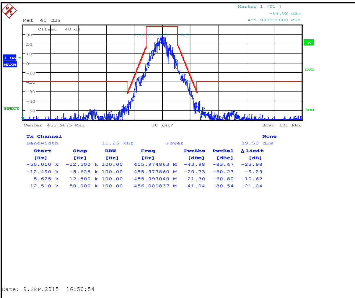
Plot 7-17: Occupied Bandwidth – 455.9875 MHz; Narrowband 2-level 9600 FSK; Mask D
