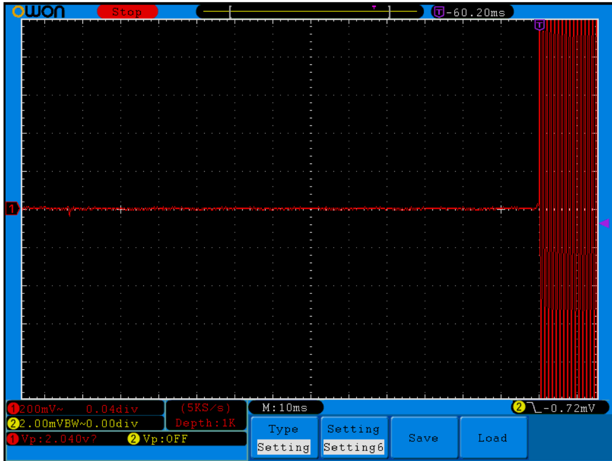
Plot 9-2: Transient Frequency Behavior – NB; Carrier Off Time; 450.0125 MHz
