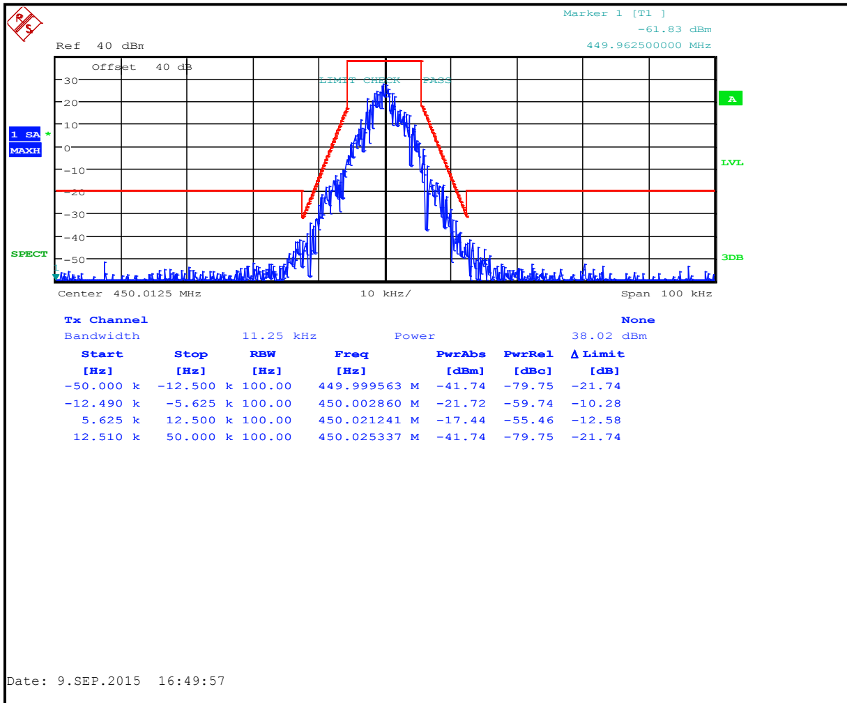
Plot 7-15: Occupied Bandwidth – 450.0125 MHz; Narrowband 2-level 9600 FSK; Mask D
