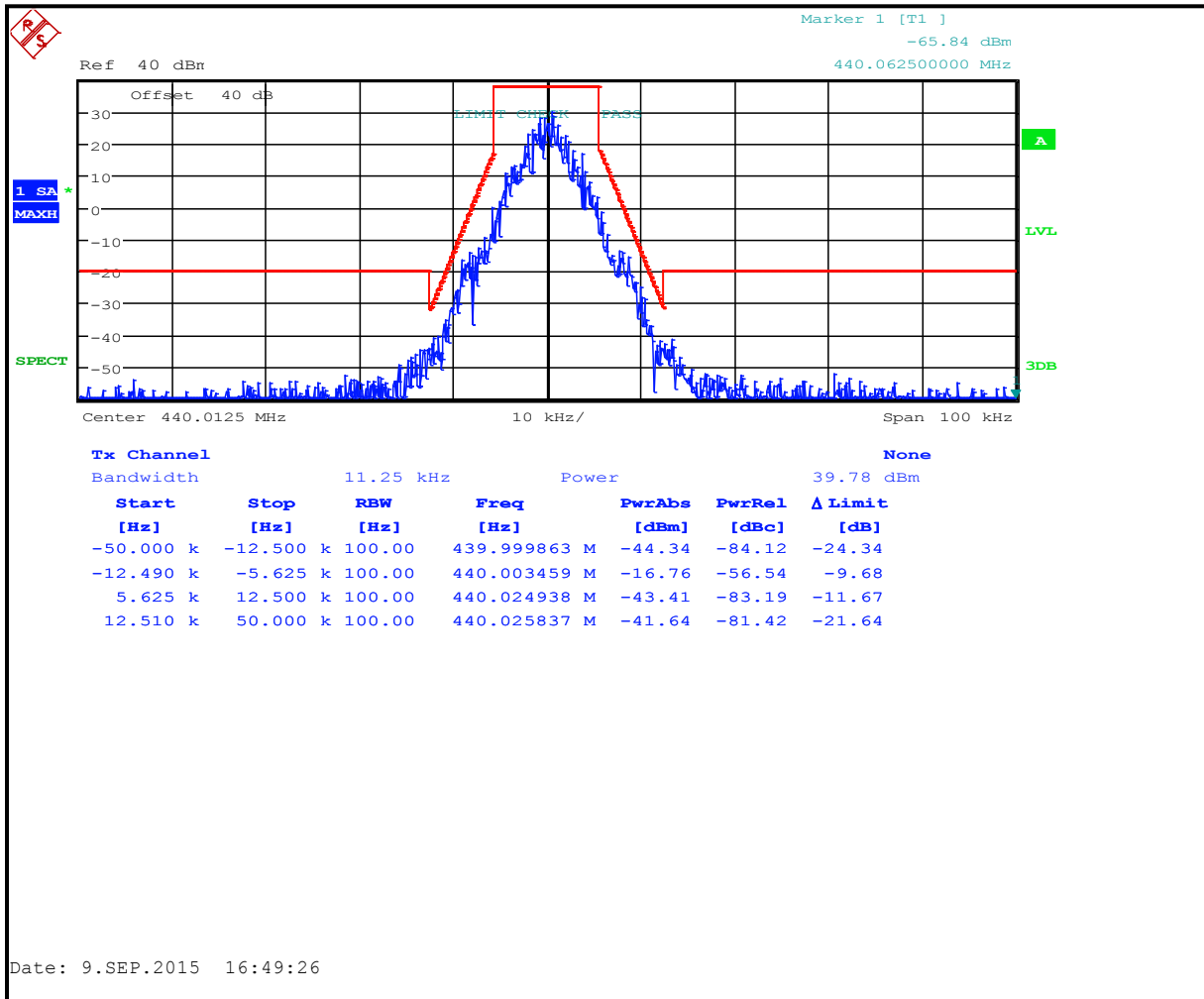
Plot 7-14: Occupied Bandwidth – 440.0125 MHz; Narrowband 2-level 9600 FSK; Mask D
