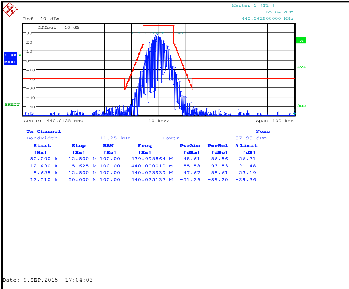
Plot 7-21: Occupied Bandwidth – 440.0125 MHz; Narrowband H-CPM TDMA; Mask D
