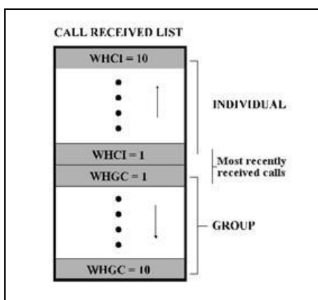
Figure 7-11: WHC Individual Call Display
