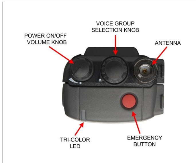
Figure 7-1: Top View
