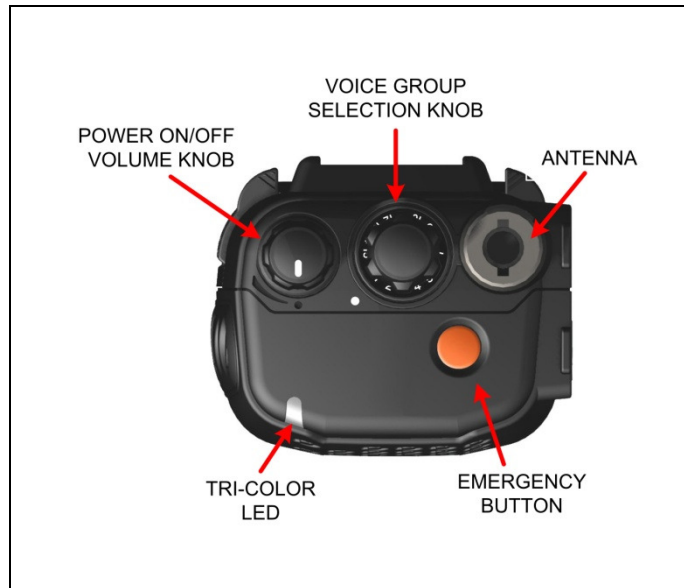
Figure 8-1: Top View
