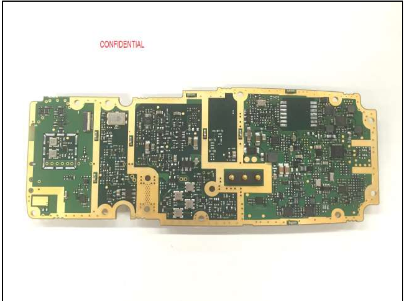
Photograph 18: RF Main Board without GPS – Back View
