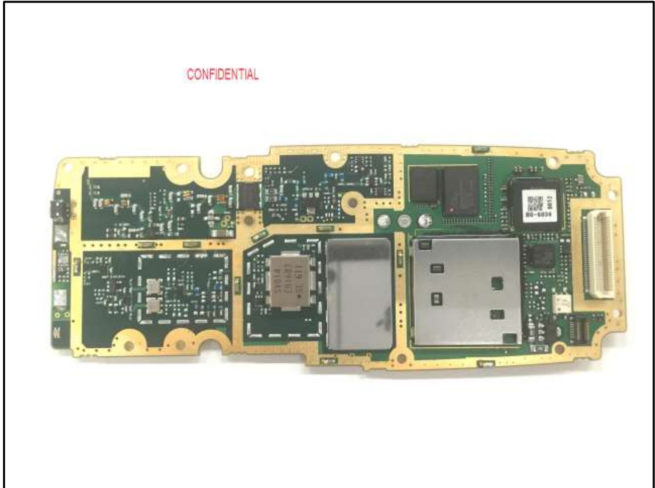
Photograph 16: RF Main Board without GPS – Top View
