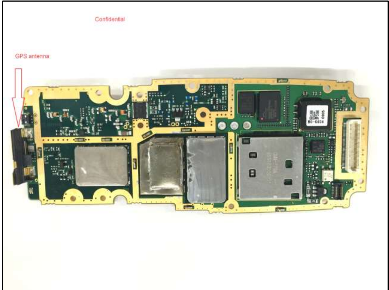
Photograph 15: RF Main Board with GPS – Top View
