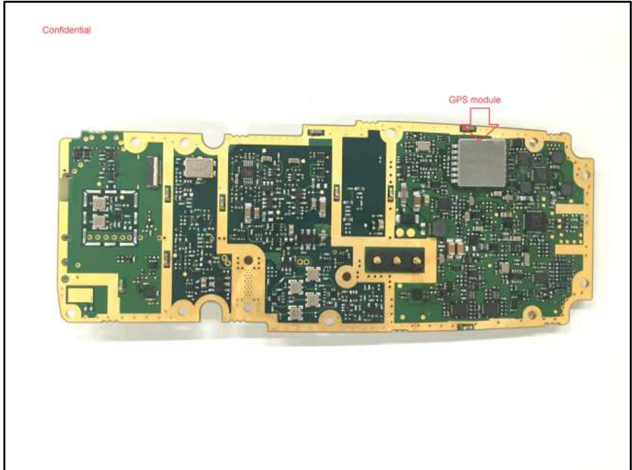
Photograph 17: RF Main Board with GPS – Back View
