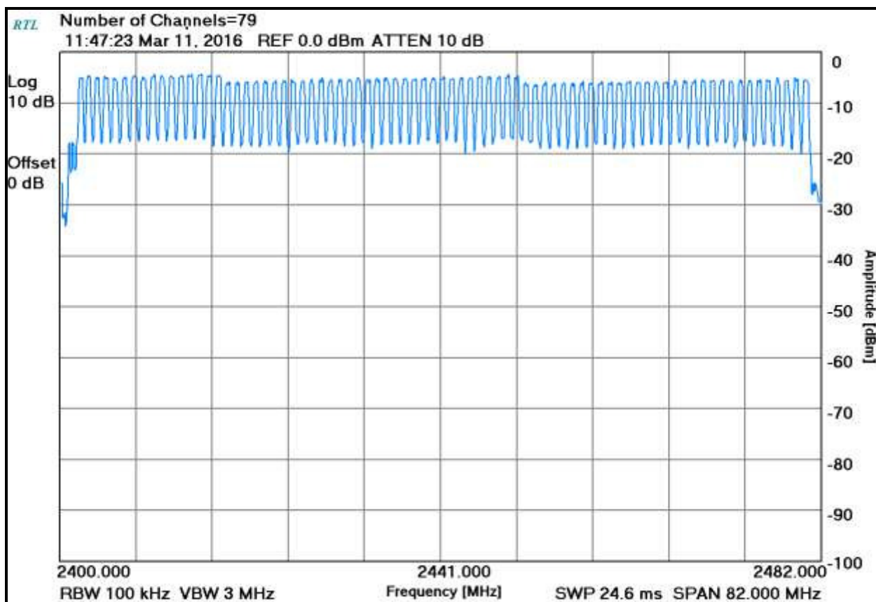
Plot 9-1: Number of Hopping Frequencies (2402 - 2480 MHz)
