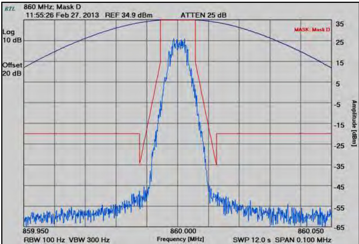
Plot 8-46: Occupied Bandwidth – 860.0000 MHz; H-CPM TDMA; Mask D
