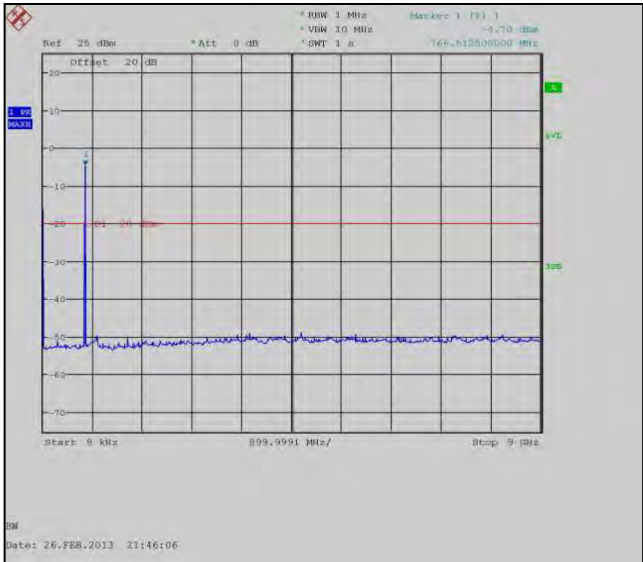
Plot 5-13: Conducted Spurious Emissions – H-CPM TDMA; 764.0125 MHz
