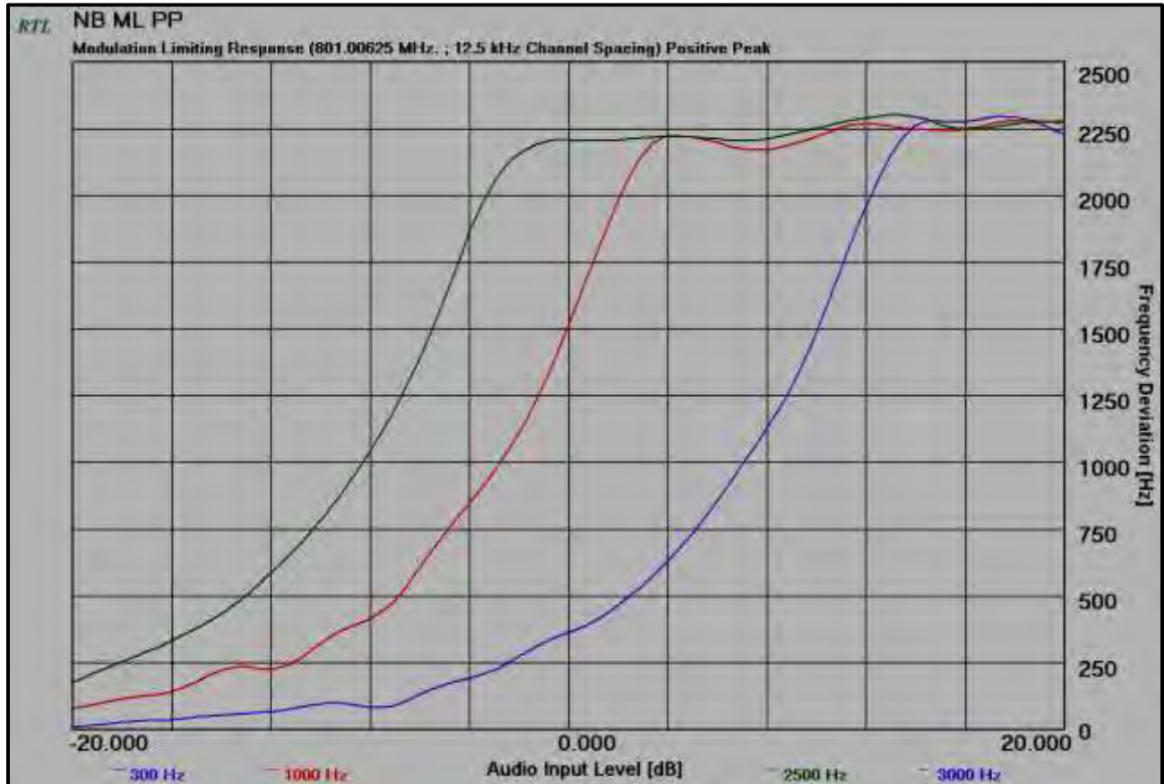
Plot 10-3: Modulation Characteristics – Modulation Limiting – 801.00625 MHz; NB, Positive Peak
