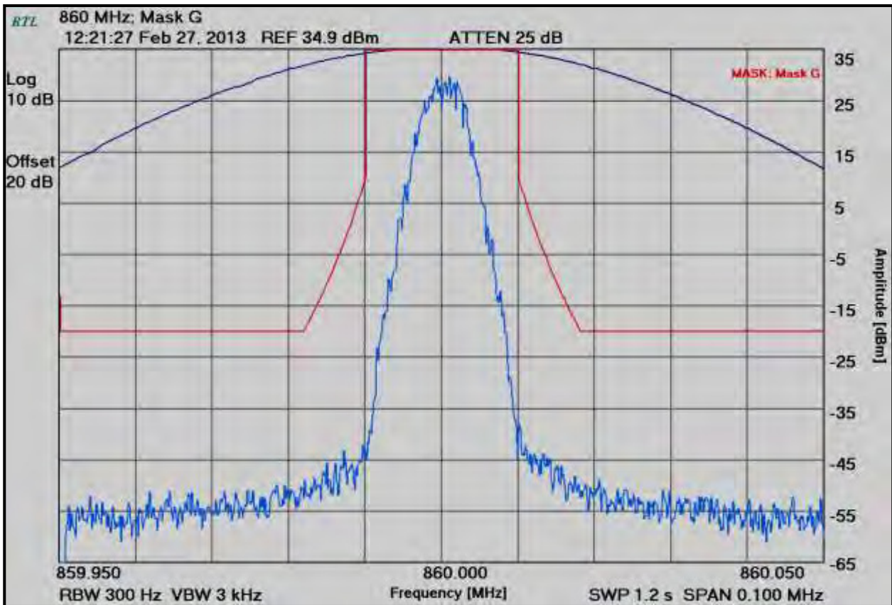
Plot 8-52: Occupied Bandwidth – 860.0000 MHz; H-CPM TDMA; Mask G
