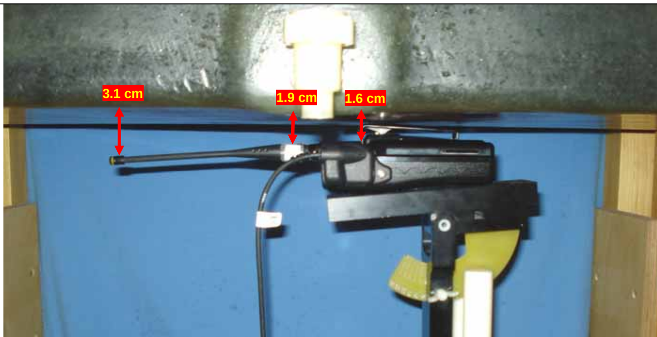
Body-worn Test Setup – Body-worn Acc. 5, Audio Acc. G3a, Antenna 1
