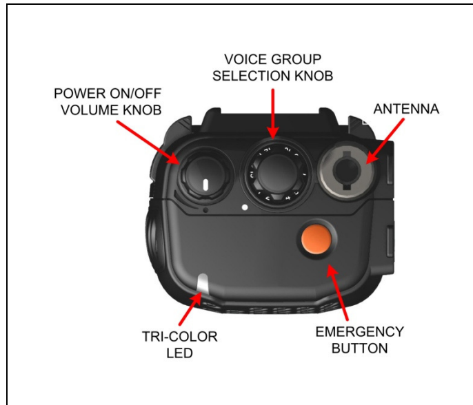
Figure 8-1: Top View
