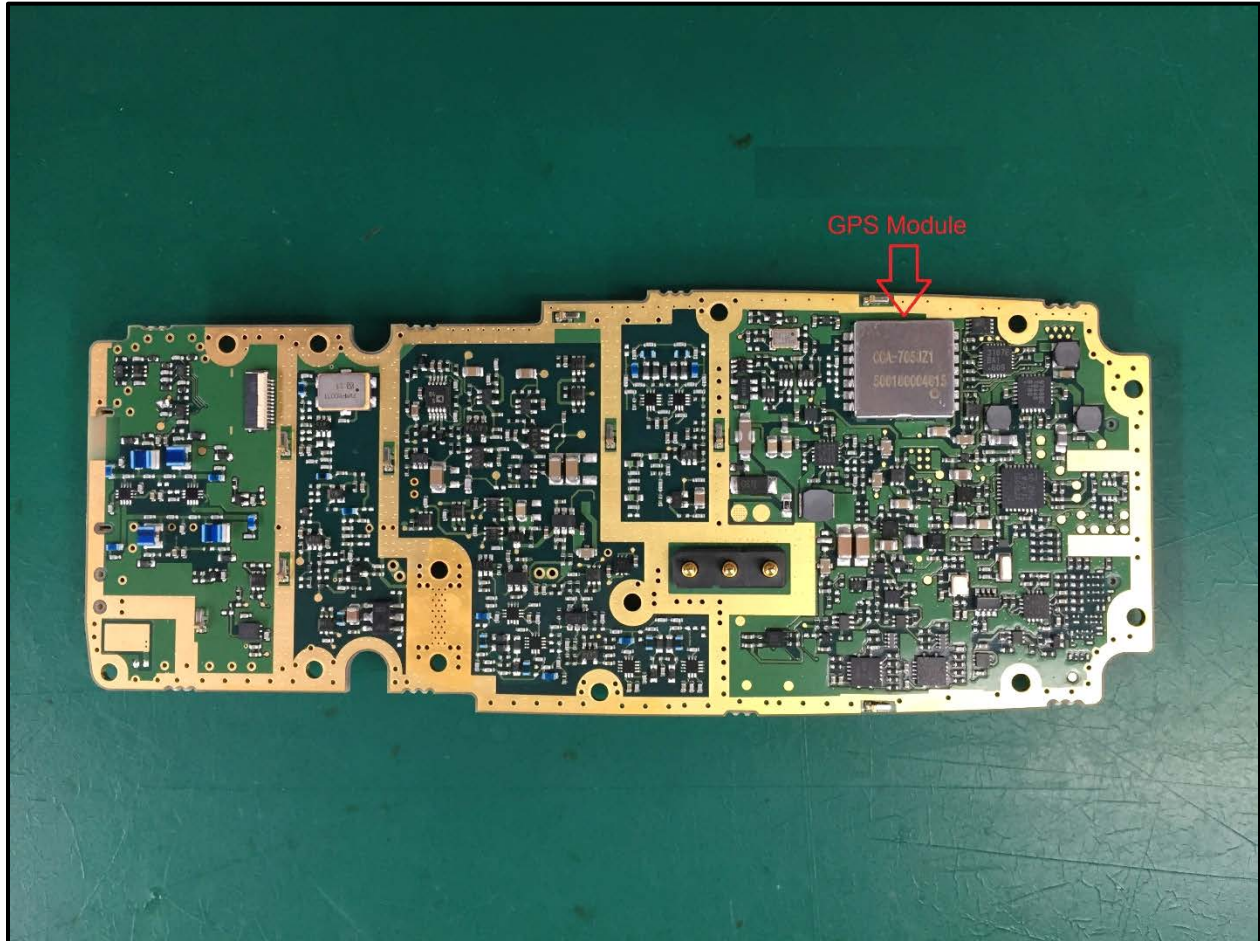
Photograph 16: RF Back View with GPS Module
