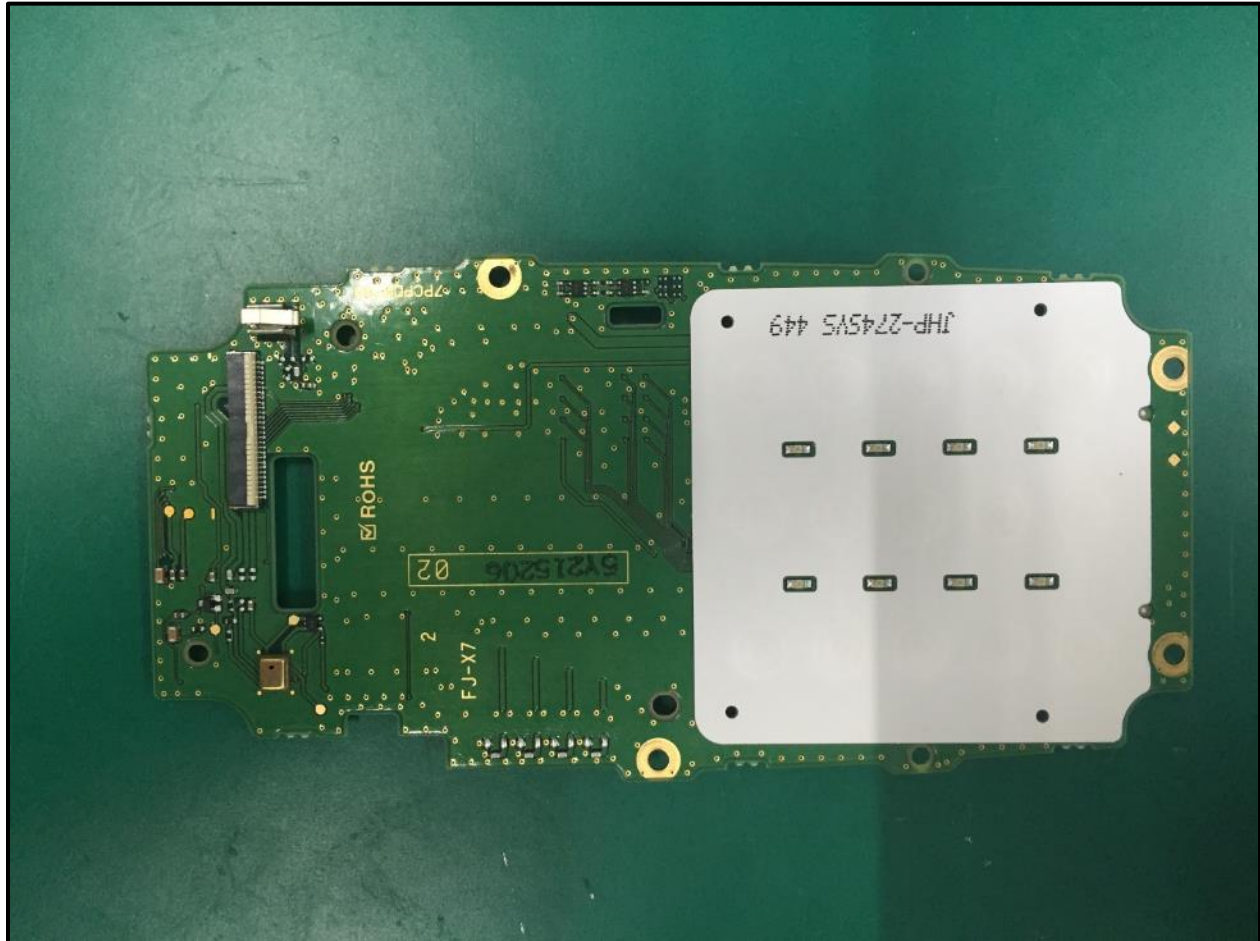
Photograph 13: Keypad
