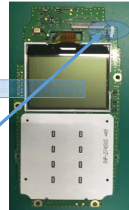
Display board
