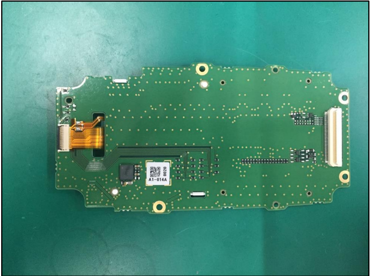
Photograph 14: Keypad Back with Cable
