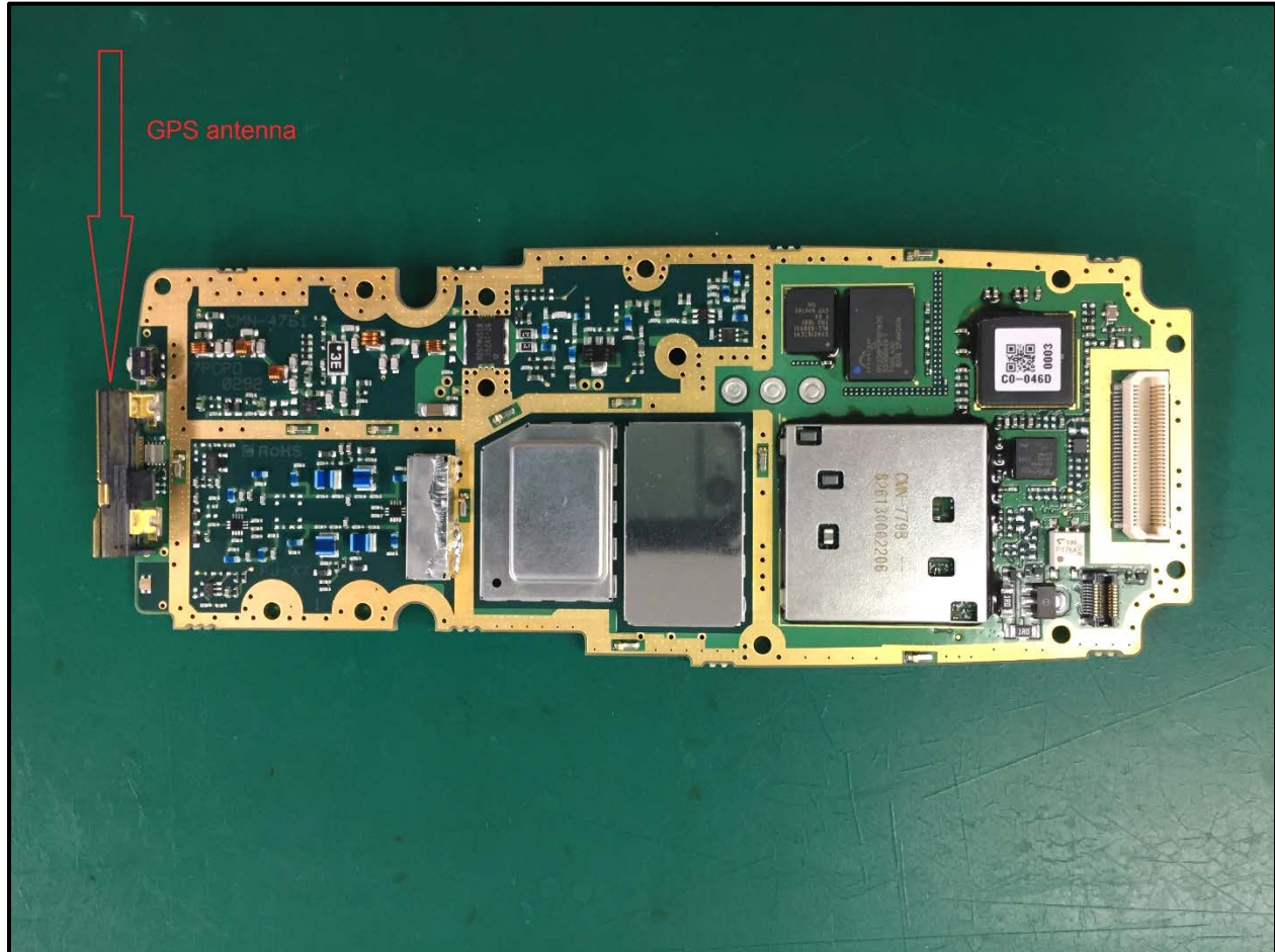
Photograph 15: RF Front View with GPS Antenna
