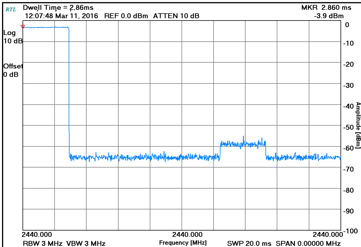
Plot 4-1: Pulse Width – 2.86ms
