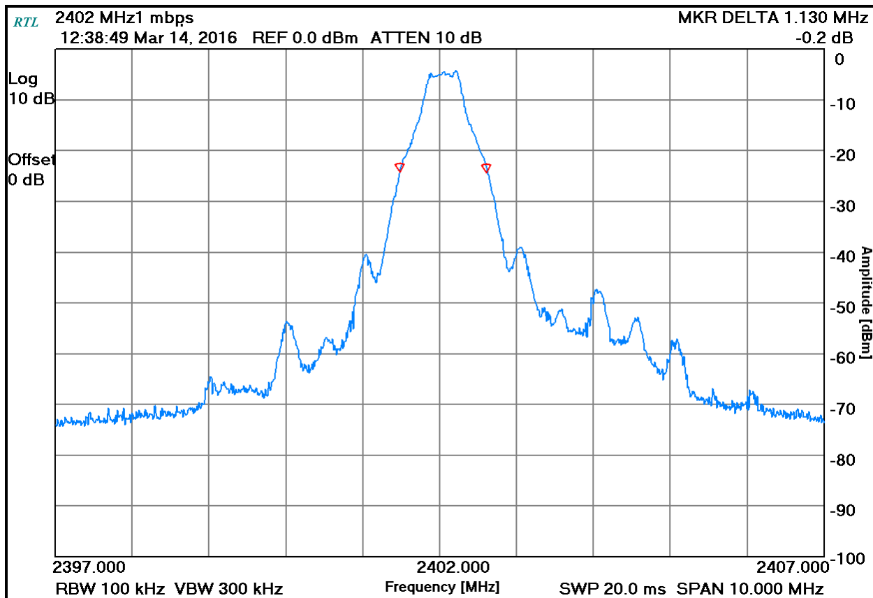
Plot 7-1: 20 dB Bandwidth - 2402 MHz; GFSK
