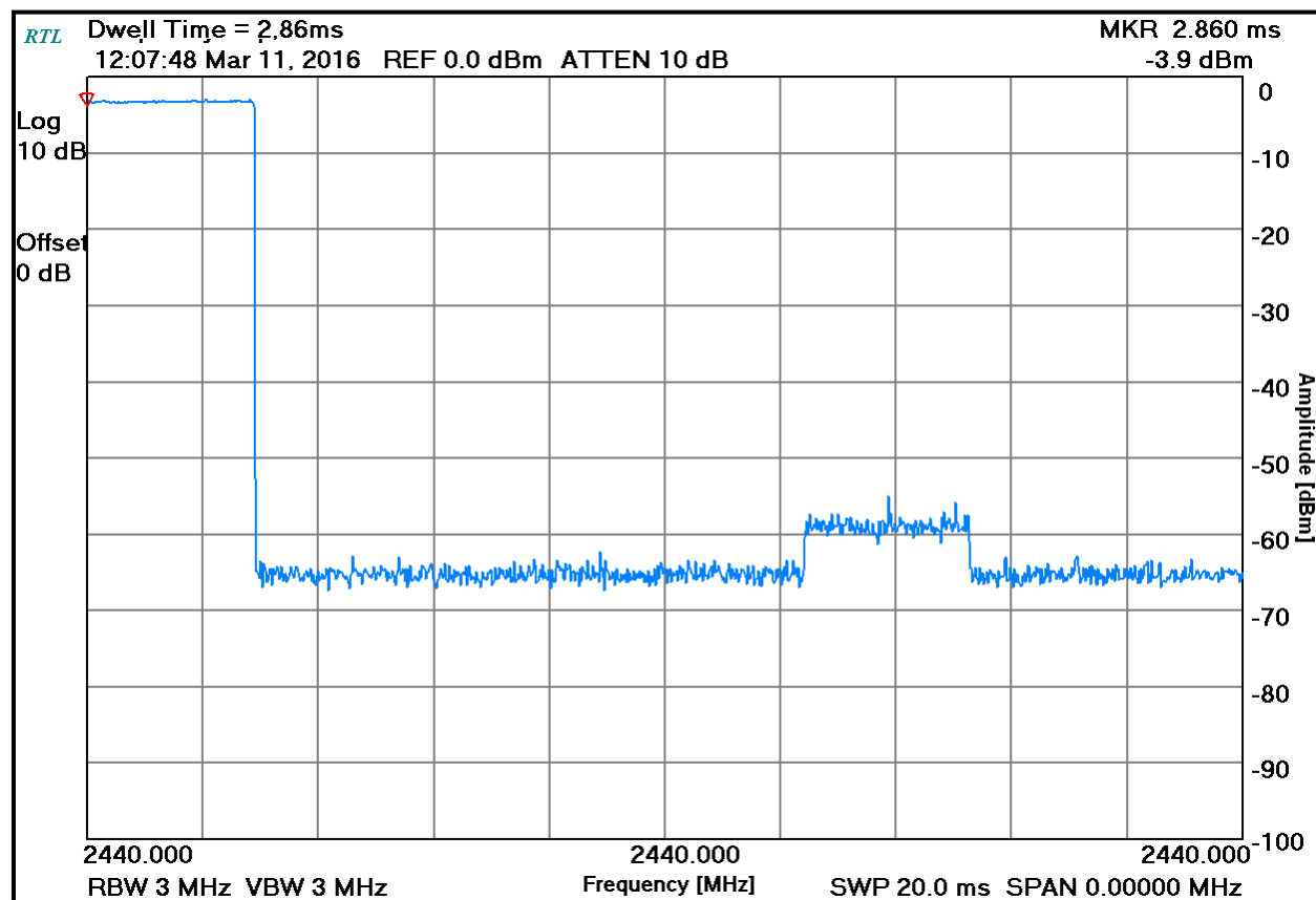
Plot 9-2: Time of Occupancy (Dwell Time)
