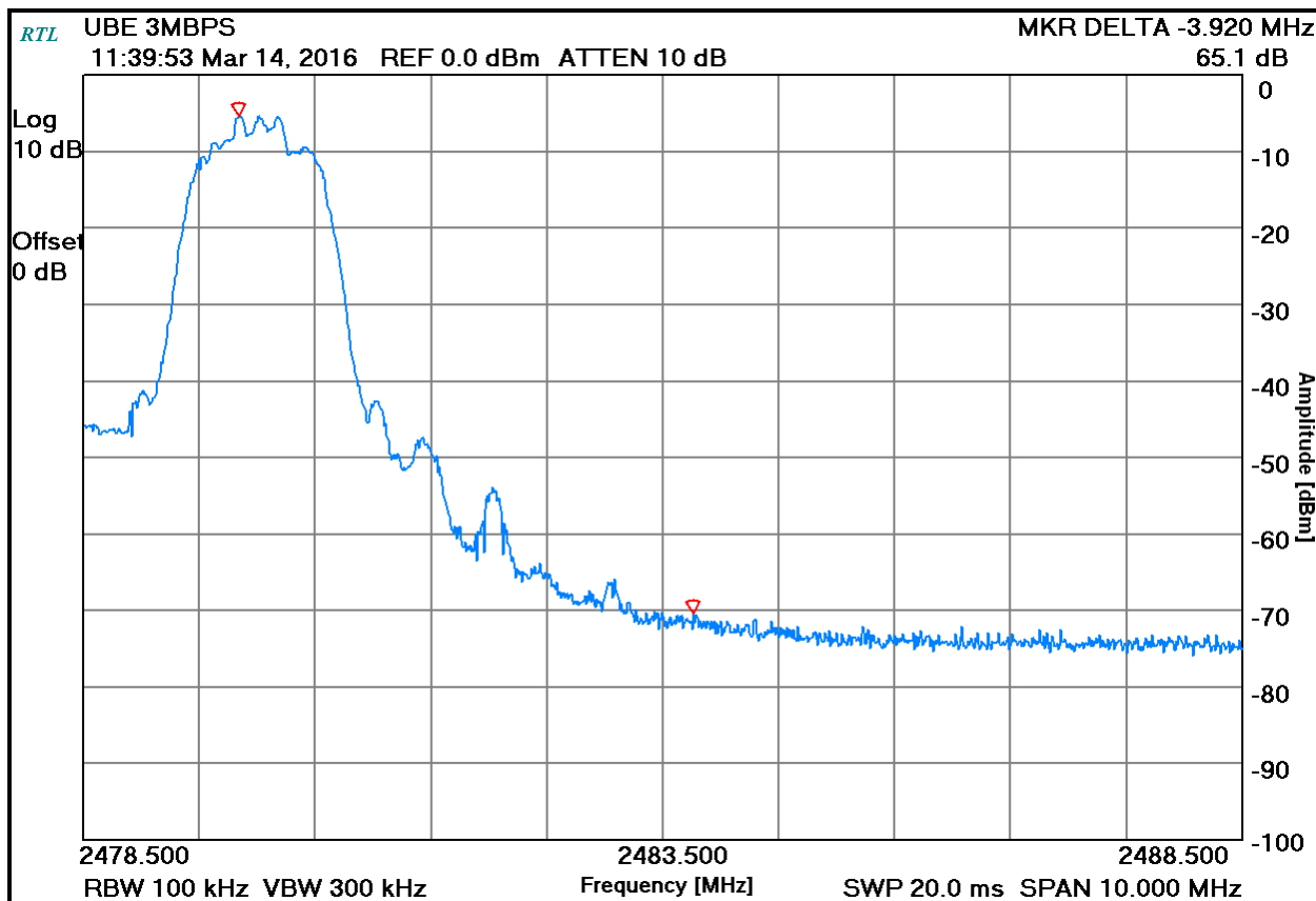
Plot 6-3: Upper Band Edge TX Frequency - 2480 MHz
