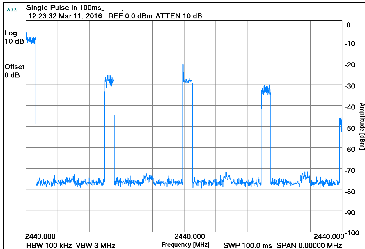
Plot 4-2: Single Pulse per 100ms
