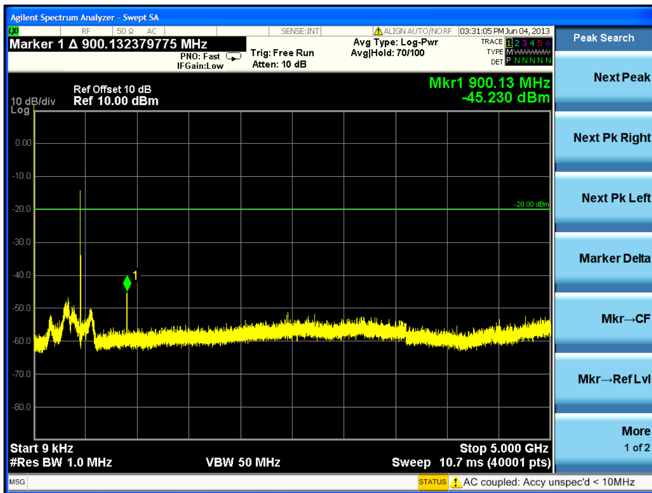
Plot 5-5: Spurious Emissions at Antenna Terminals – 450.0125 MHz
