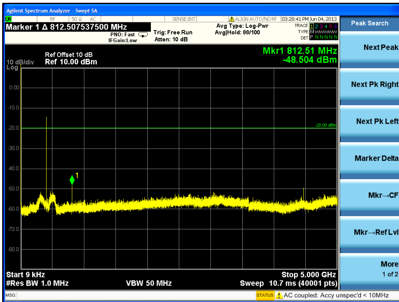
Plot 5-2: Spurious Emissions at Antenna Terminals – 406.1125 MHz
