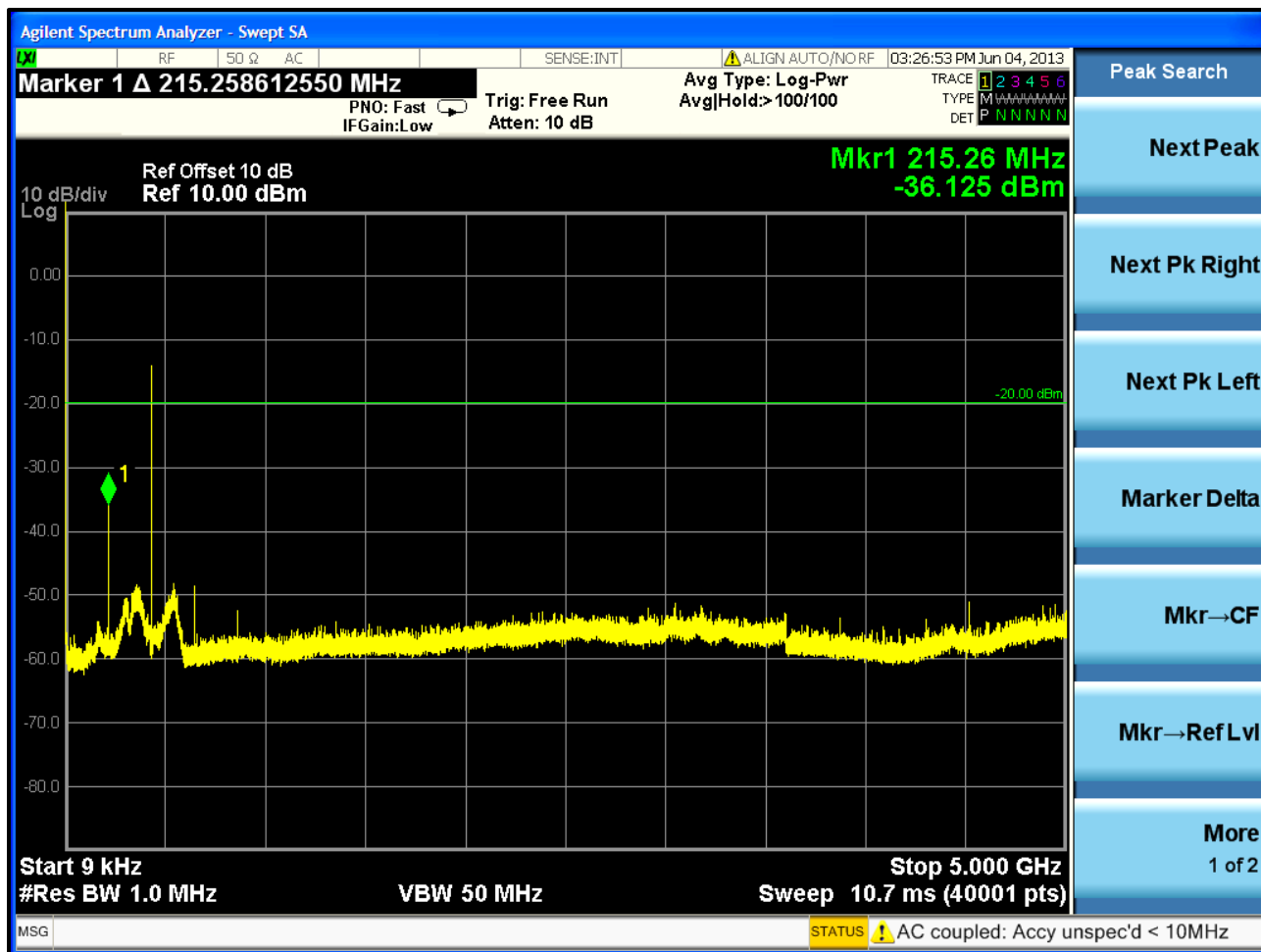
Plot 5-4: Spurious Emissions at Antenna Terminals – 429.9875 MHz
