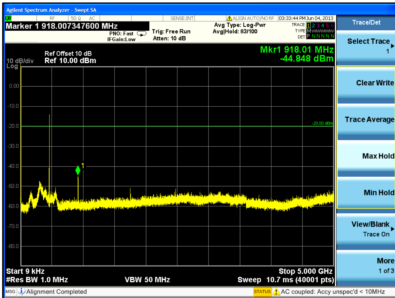
Plot 5-8: Spurious Emissions at Antenna Terminals – 458.9875 MHz
