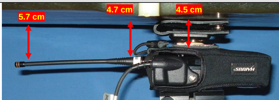
Body-worn Test Setup – Body-worn Acc. 1, Audio Acc. G8a, Antenna 3
