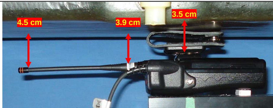
Body-worn Test Setup – Body-worn Acc. 6, Audio Acc. G8a, Antenna 4
