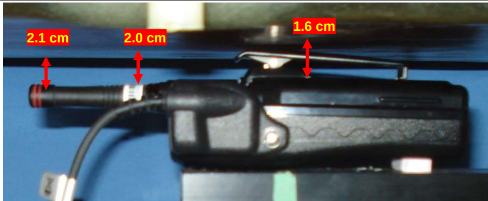
Body-worn Test Setup – Body-worn Acc. 5, Audio Acc. G8a, Antenna 2
