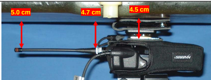
Body-worn Test Setup – Body-worn Acc. 1, Audio Acc. G8a, Antenna 4
