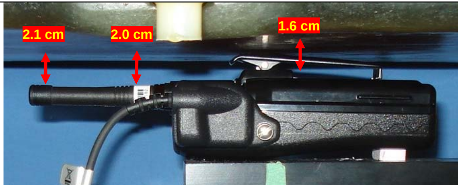
Body-worn Test Setup – Body-worn Acc. 5, Audio Acc. G8a, Antenna 1
