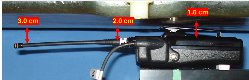
Body-worn Test Setup – Body-worn Acc. 5, Audio Acc. G8a, Antenna 3
