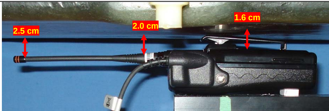
Body-worn Test Setup – Body-worn Acc. 5, Audio Acc. G8a, Antenna 4
