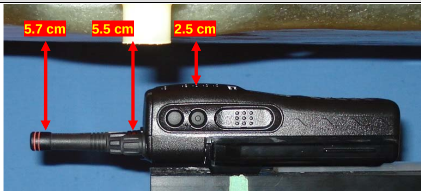
Face-Held Test Setup - Antenna 2
