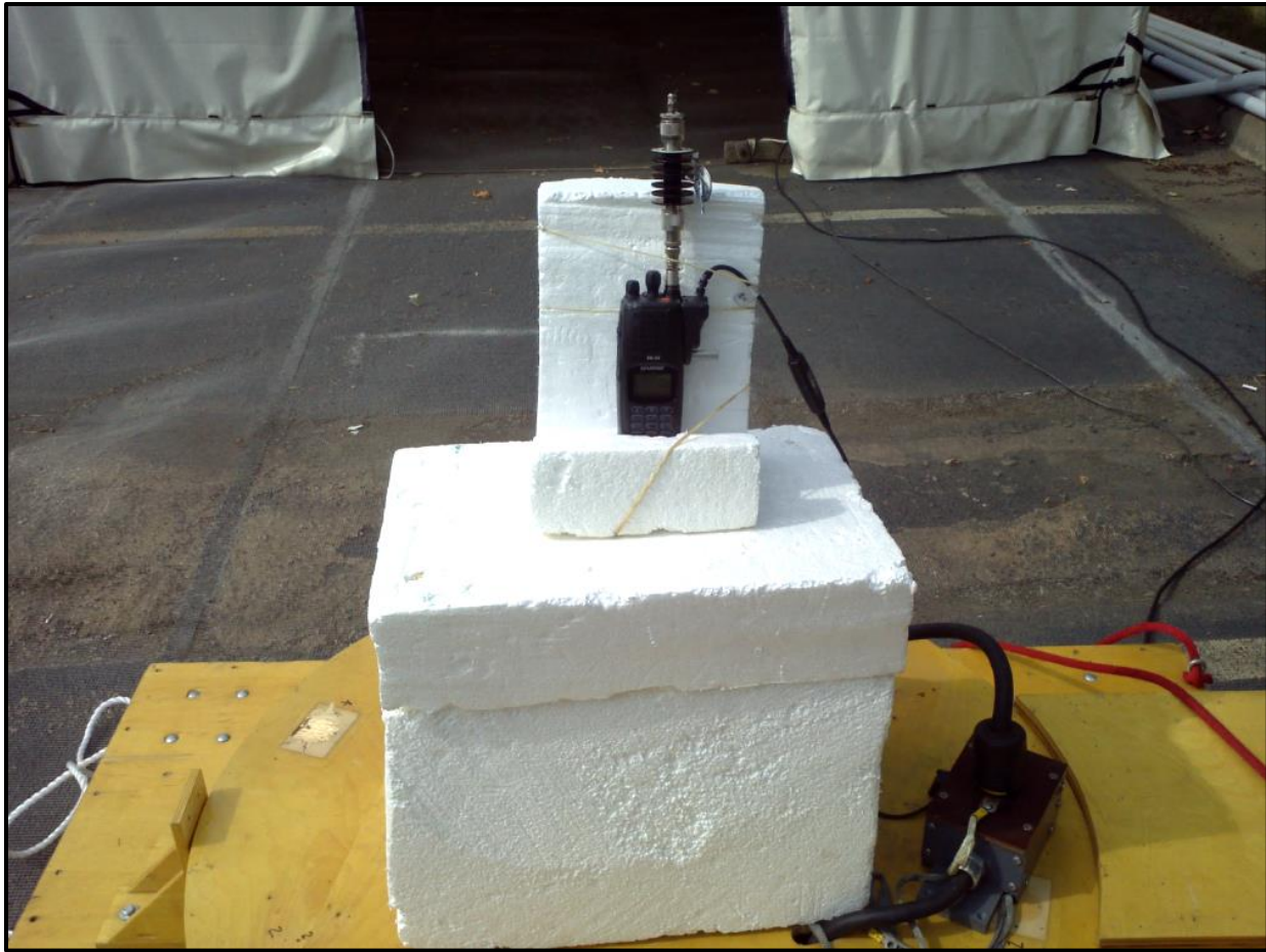
Photograph 4: Radiated Emissions (Spurious/Harmonics) – Front View
