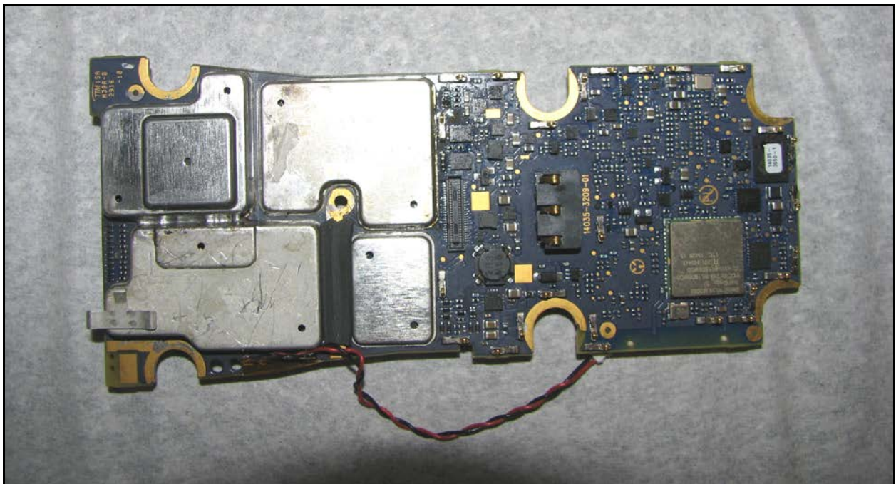
Main Board with Shields – Bottom
