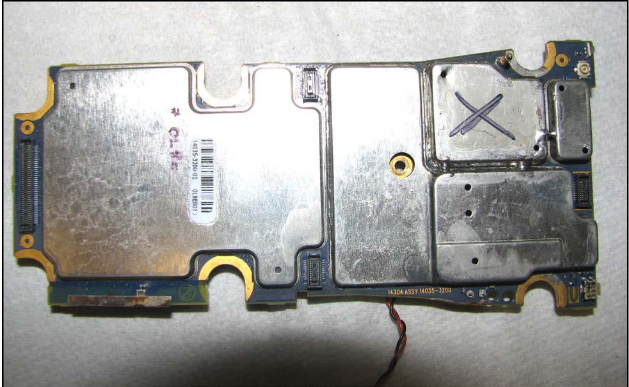
Main Board with Shields – Top
