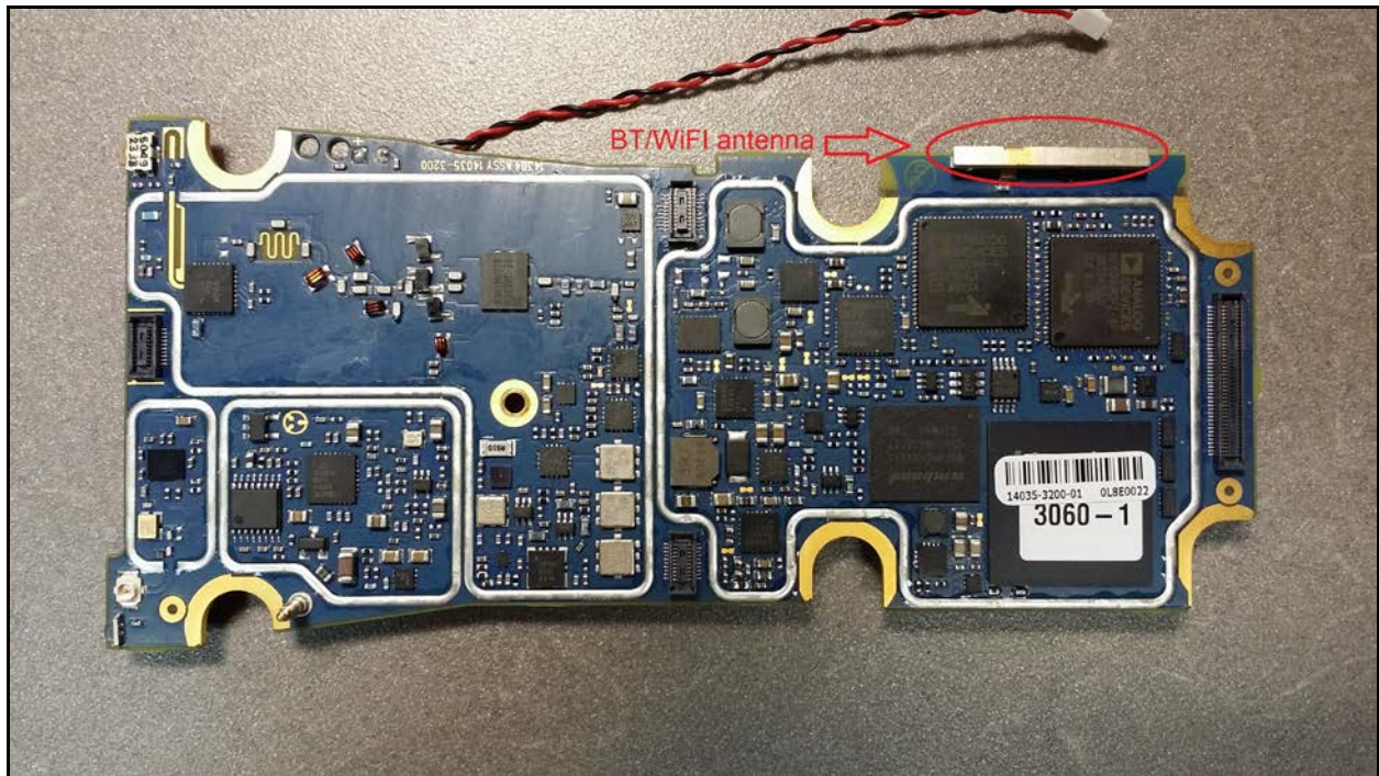
Main Board without Shields – Top, with BT/Wi-Fi Antenna
