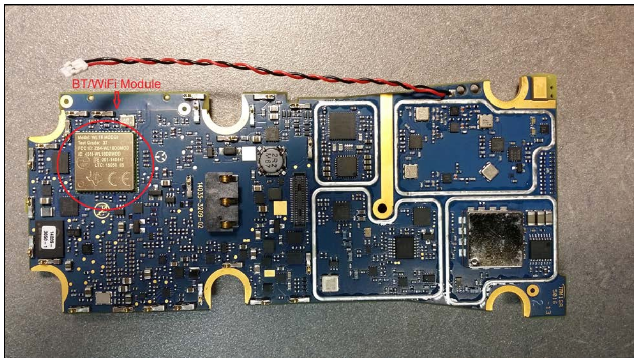
Main Board without Shields – Bottom, with BT/Wi-Fi Module
