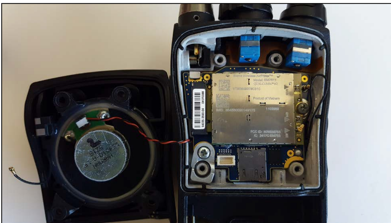
Rear Cover and Grounding Strap Removed; LTE Module
