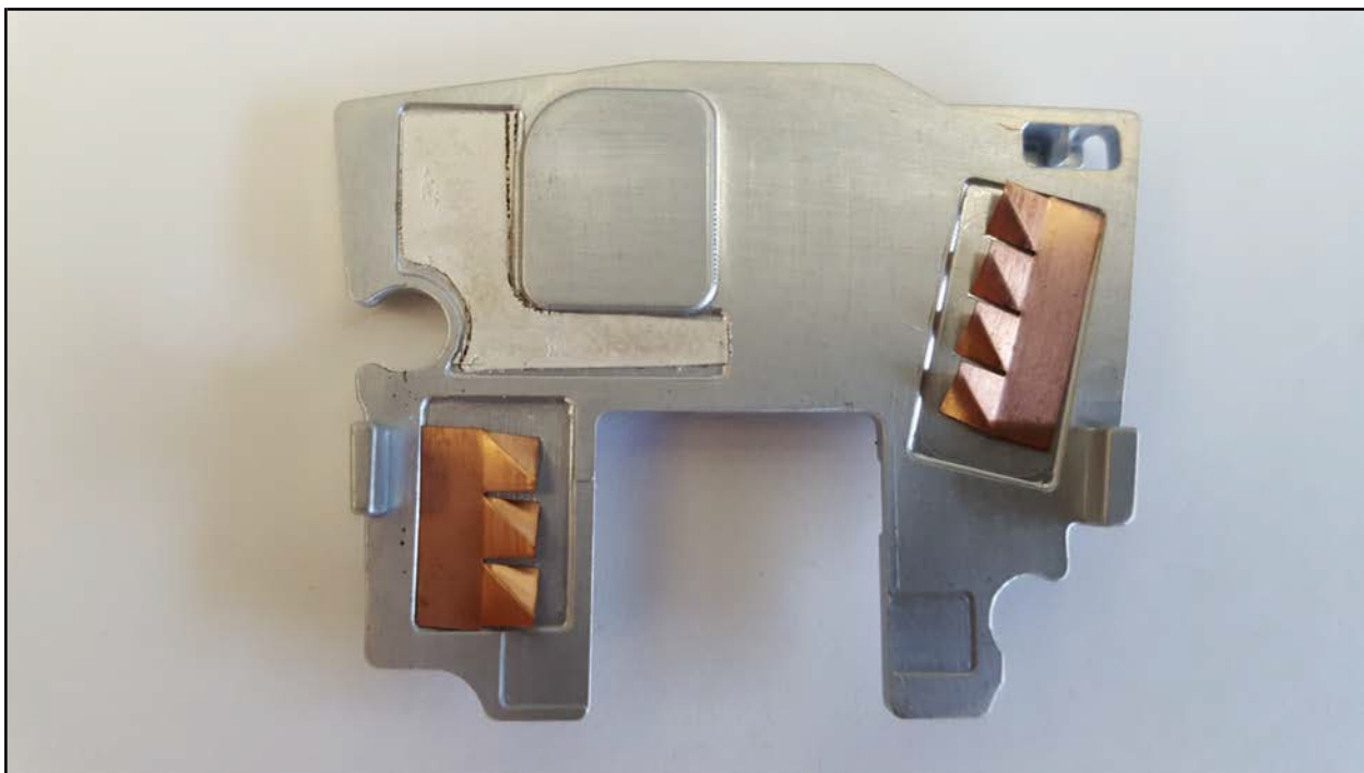
LTE Processor Shield – Bottom
