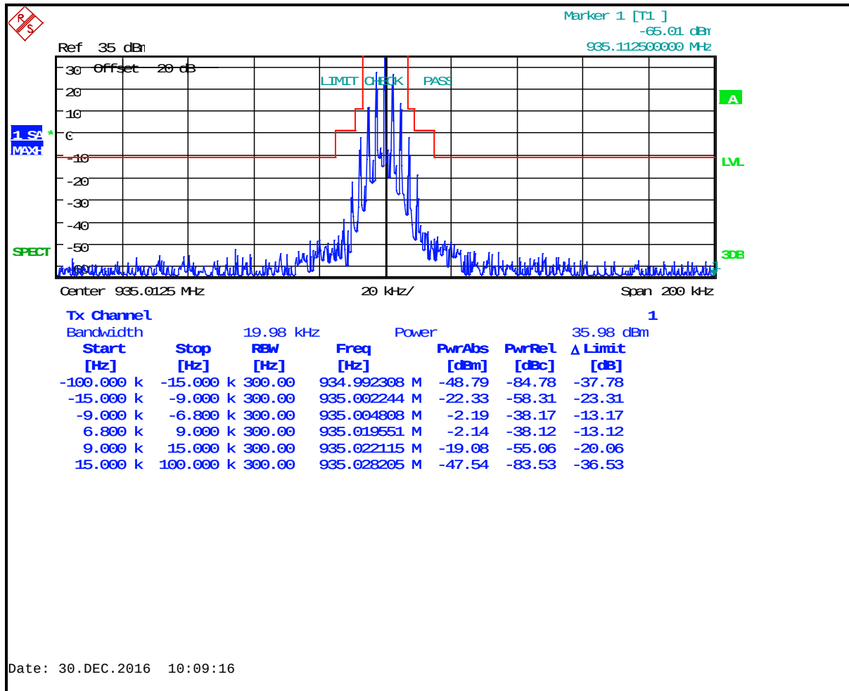
Plot 8-16: Occupied Bandwidth – 935.0125 MHz; NB Analog; Mask I
