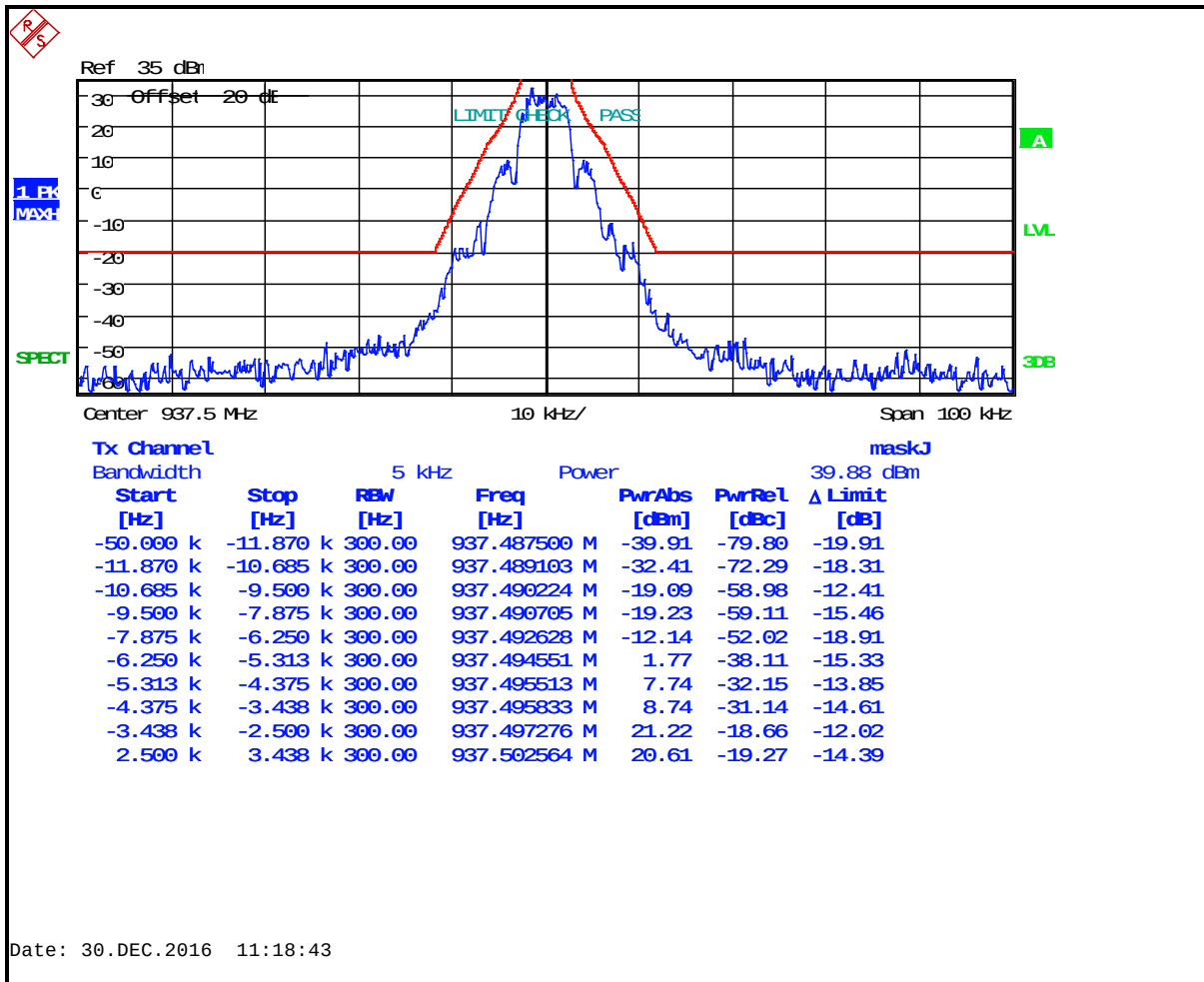
Plot 8-35: Occupied Bandwidth – 937.5 MHz; 2-Level FSK 4800 XNB; Mask J
