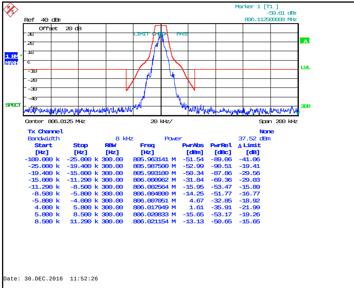
Plot 8-37: Occupied Bandwidth – 806.0125 MHz; 2-Level FSK 9600 NB; Mask H
