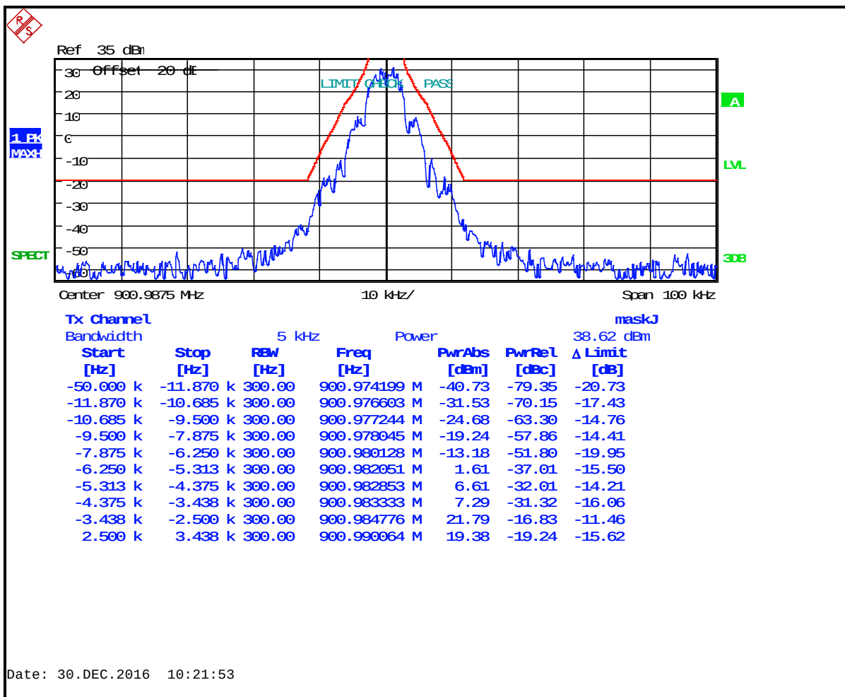
Plot 8-33: Occupied Bandwidth – 900.9875 MHz; 2-Level FSK 4800 XNB; Mask J
