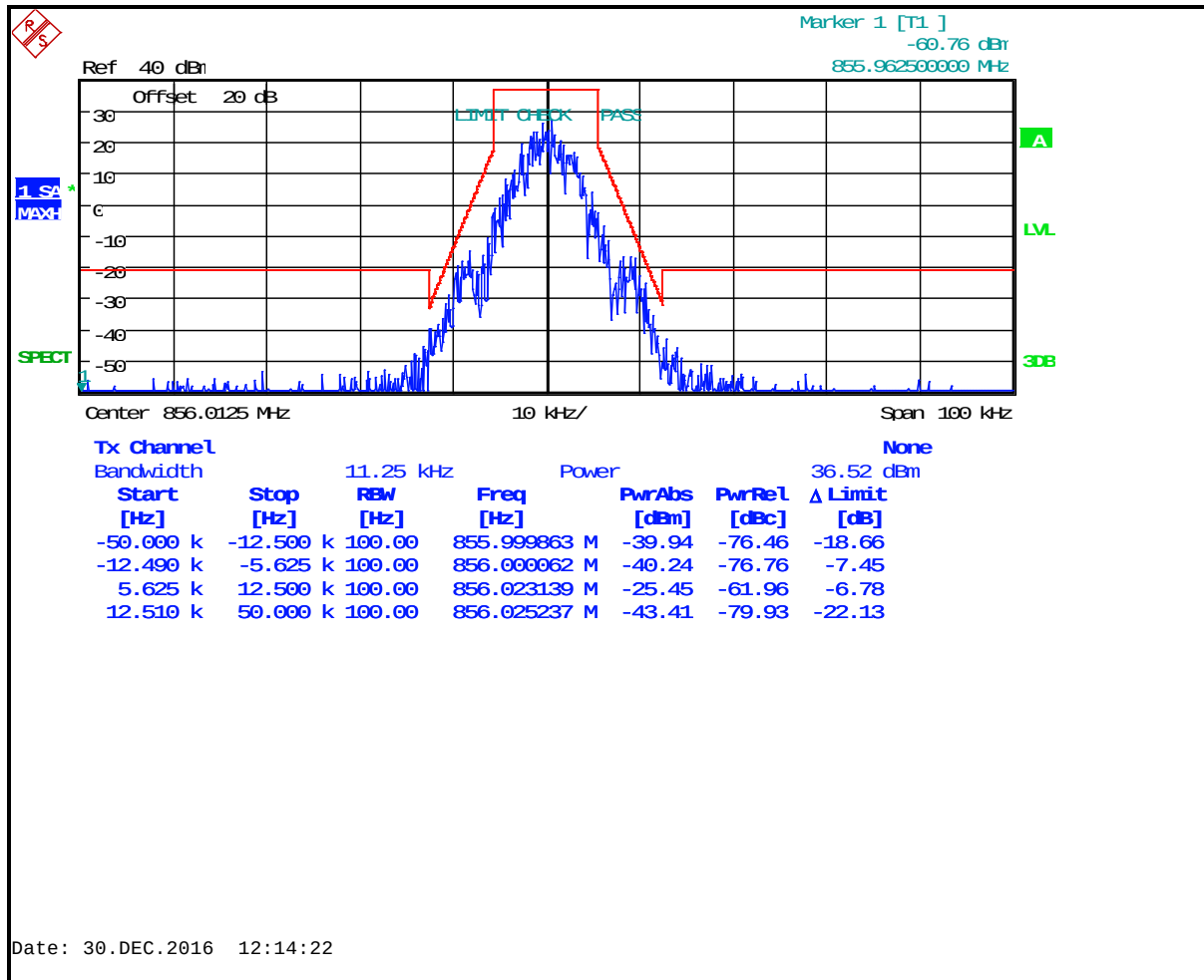
Plot 8-47: Occupied Bandwidth – 856.0125 MHz; 2-Level FSK 9600 NB; Mask D (IC)
