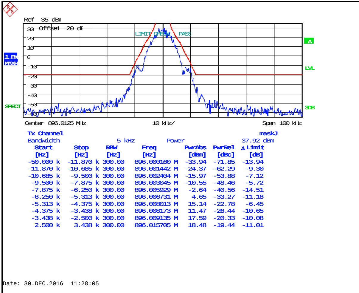
Plot 8-49: Occupied Bandwidth – 896.0125 MHz; 2-Level FSK 9600 NB; Mask J
