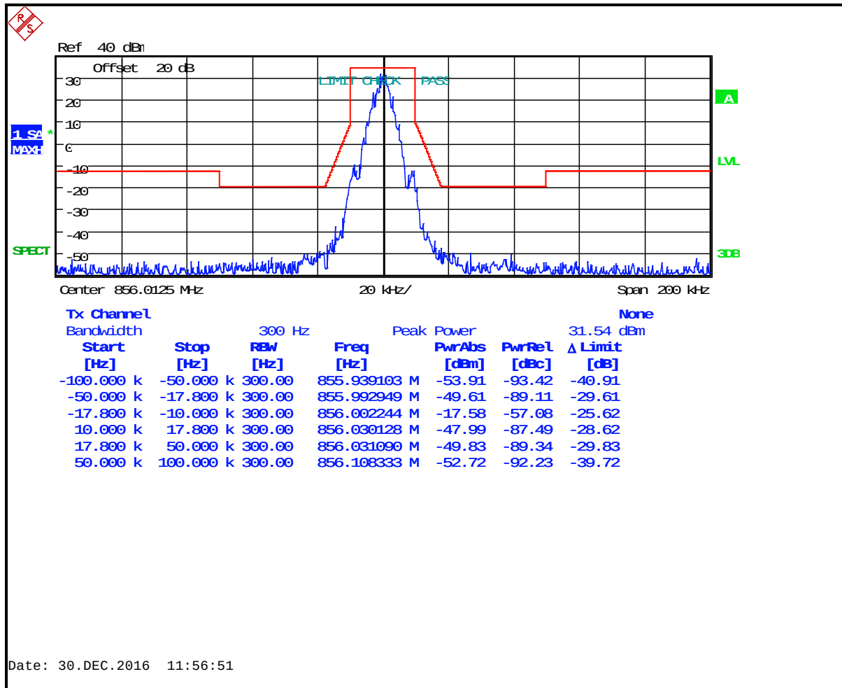
Plot 8-41: Occupied Bandwidth – 856.0125 MHz; 2-Level FSK 9600 NB; Mask G
