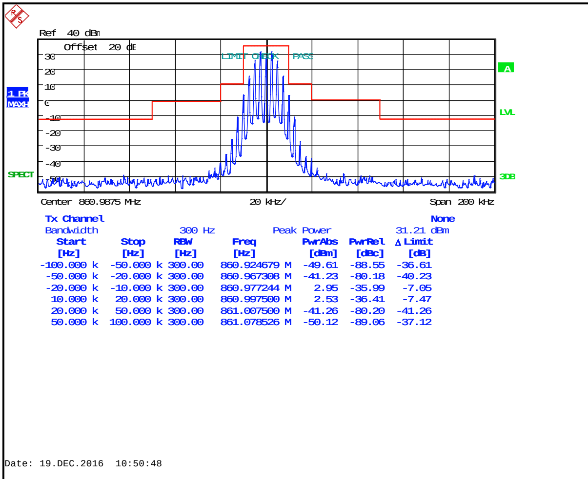
Plot 8-30: Occupied Bandwidth – 860.9875 MHz; WB Analog; Mask B
