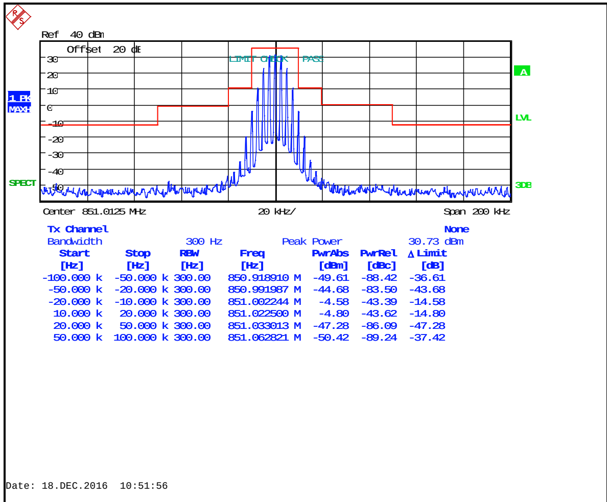
Plot 8-28: Occupied Bandwidth – 851.0125 MHz; WB Analog; Mask B
