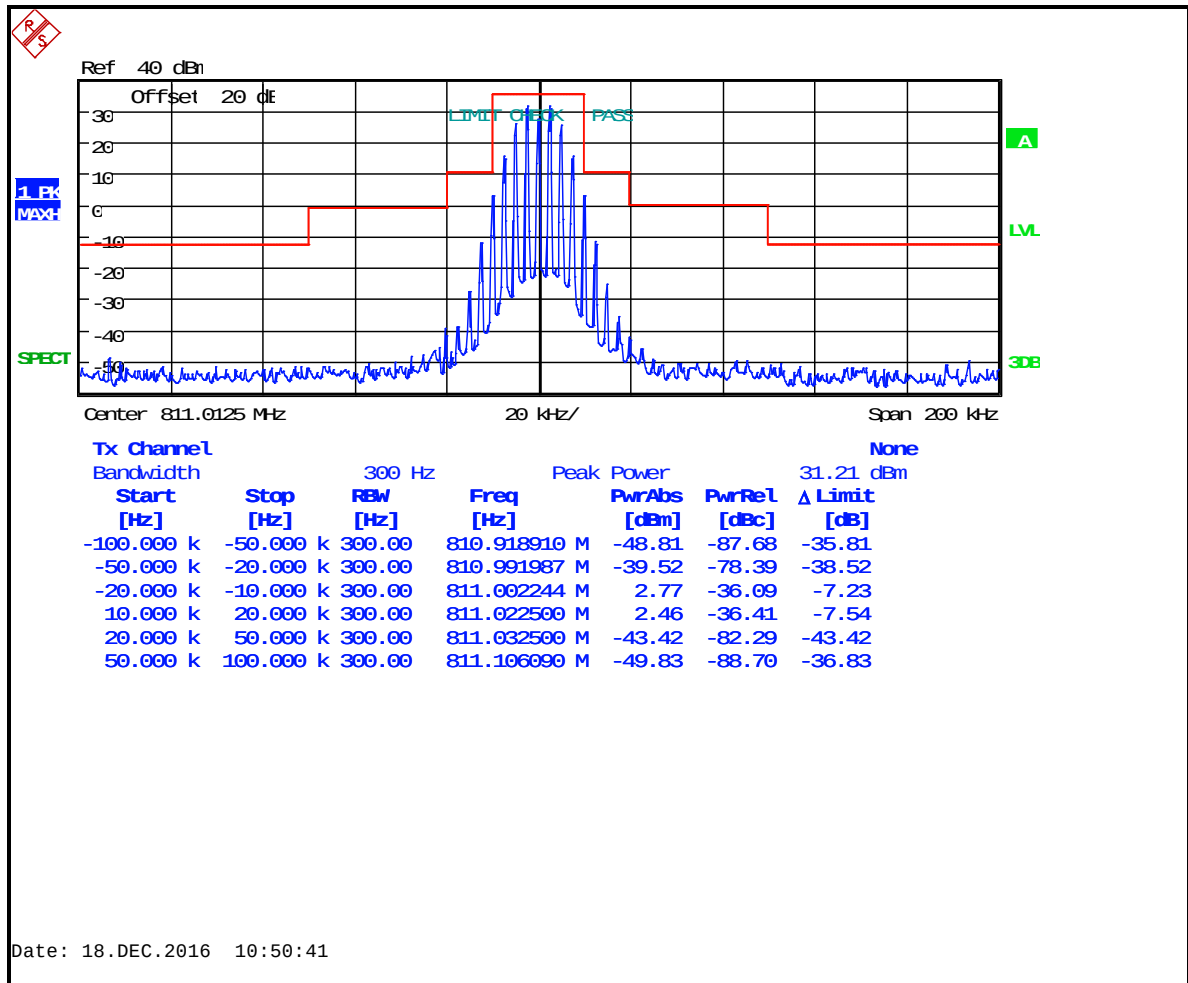
Plot 8-26: Occupied Bandwidth – 811.0125 MHz; WB Analog; Mask B
