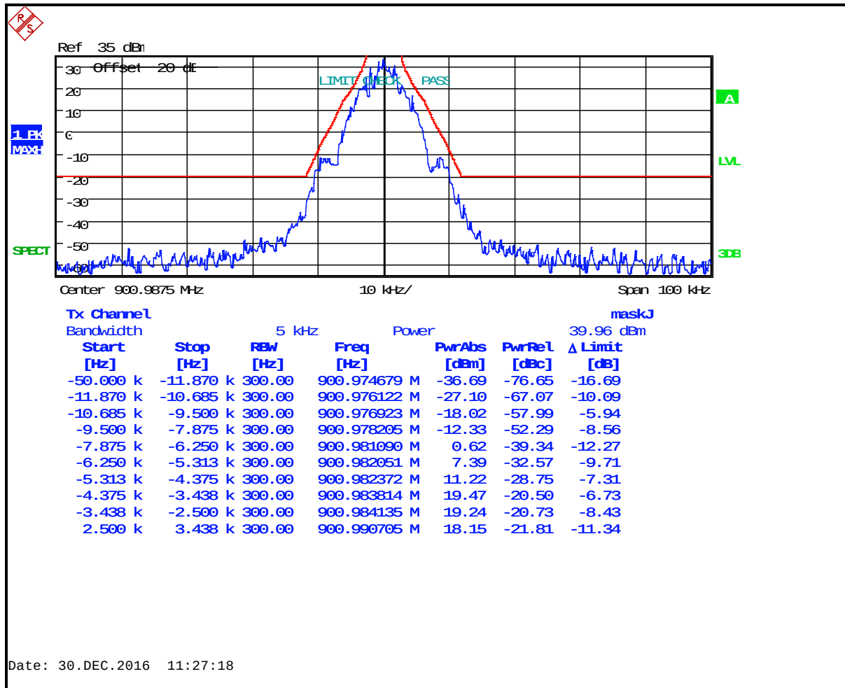
Plot 8-51: Occupied Bandwidth – 900.9875 MHz; 2-Level FSK 9600 NB; Mask J
