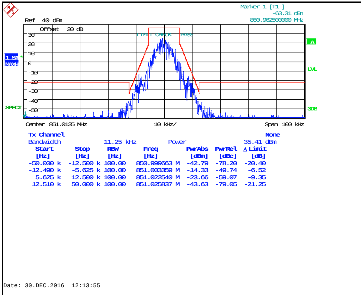
Plot 8-46: Occupied Bandwidth – 851.0125 MHz; 2-Level FSK 9600 NB; Mask D (IC)
