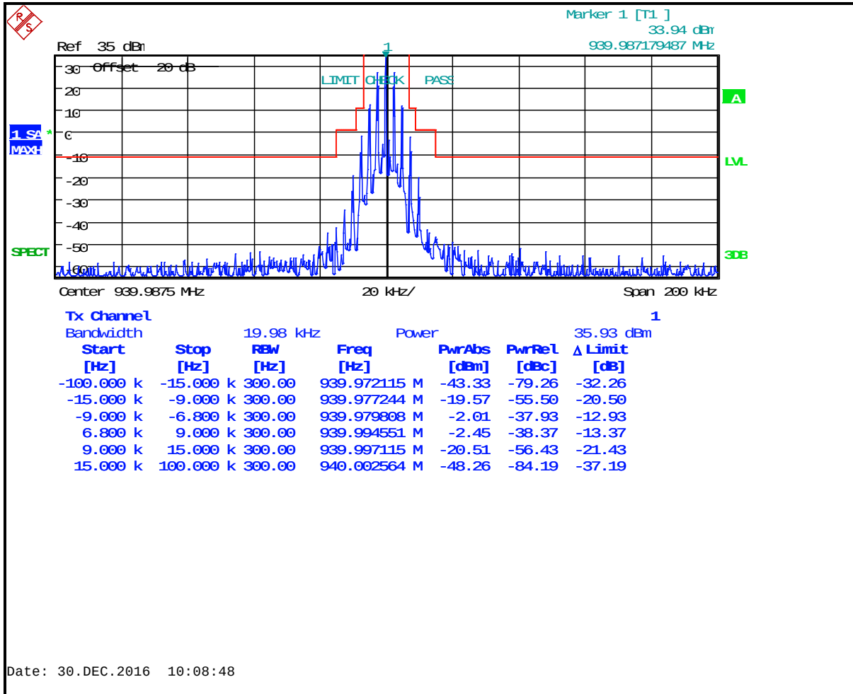
Plot 8-18: Occupied Bandwidth – 939.9875 MHz; NB Analog; Mask I
