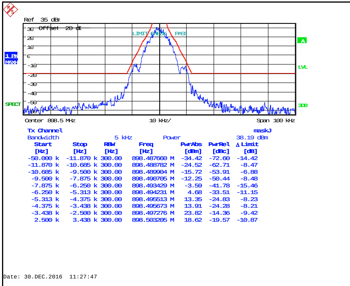
Plot 8-50: Occupied Bandwidth – 898.5 MHz; 2-Level FSK 9600 NB; Mask J
