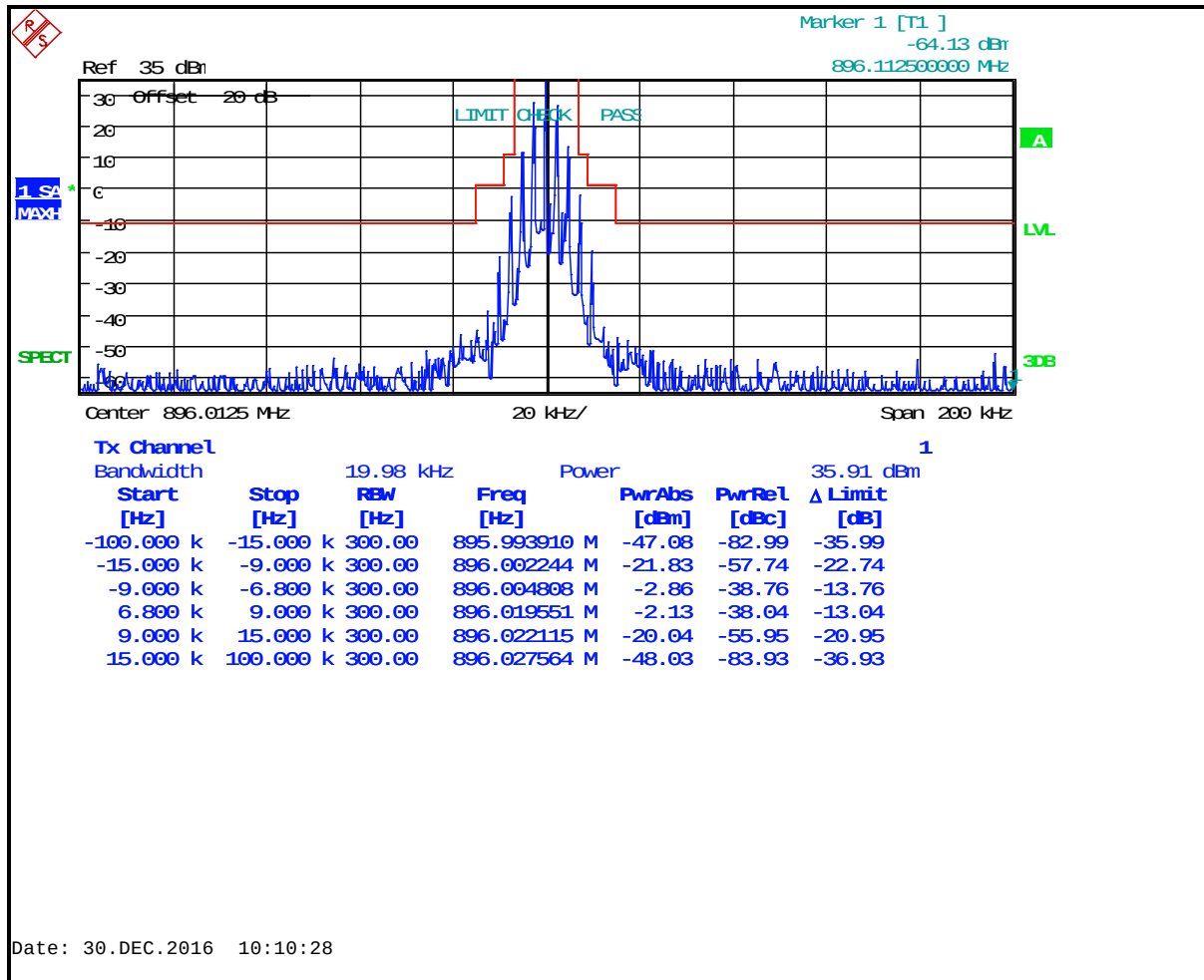
Plot 8-13: Occupied Bandwidth – 896.0125 MHz; NB Analog; Mask I
