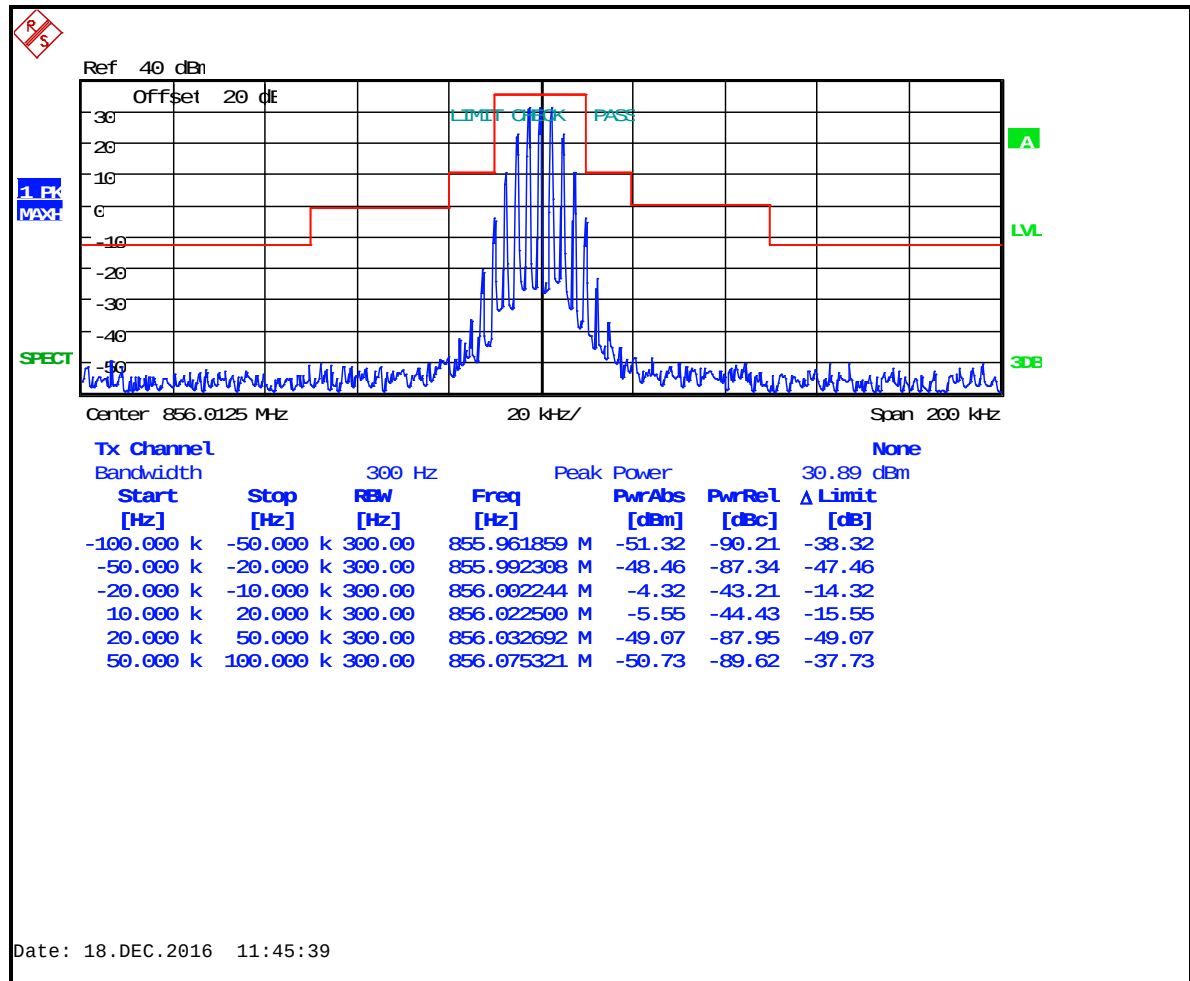
Plot 8-23: Occupied Bandwidth – 856.0125 MHz; Analog NPSPAC; Mask B
