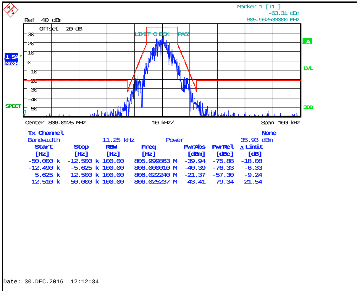
Plot 8-43: Occupied Bandwidth – 806.0125 MHz; 2-Level FSK 9600 NB; Mask D (IC)
