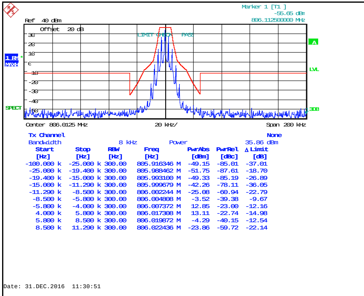
Plot 8-20: Occupied Bandwidth – 806.0125 MHz; Analog NPSPAC; Mask H
