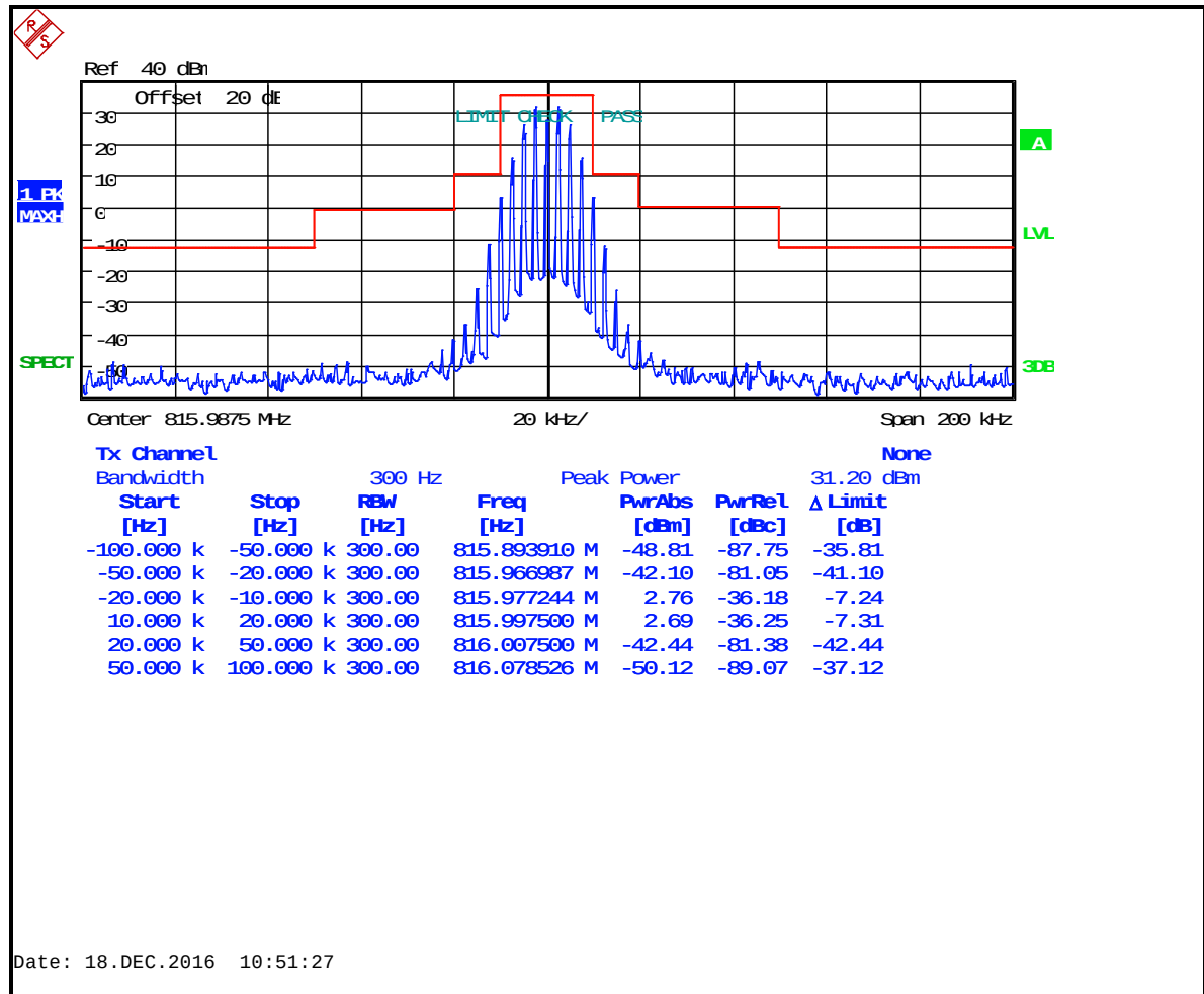
Plot 8-27: Occupied Bandwidth – 815.9875 MHz; WB Analog; Mask B
