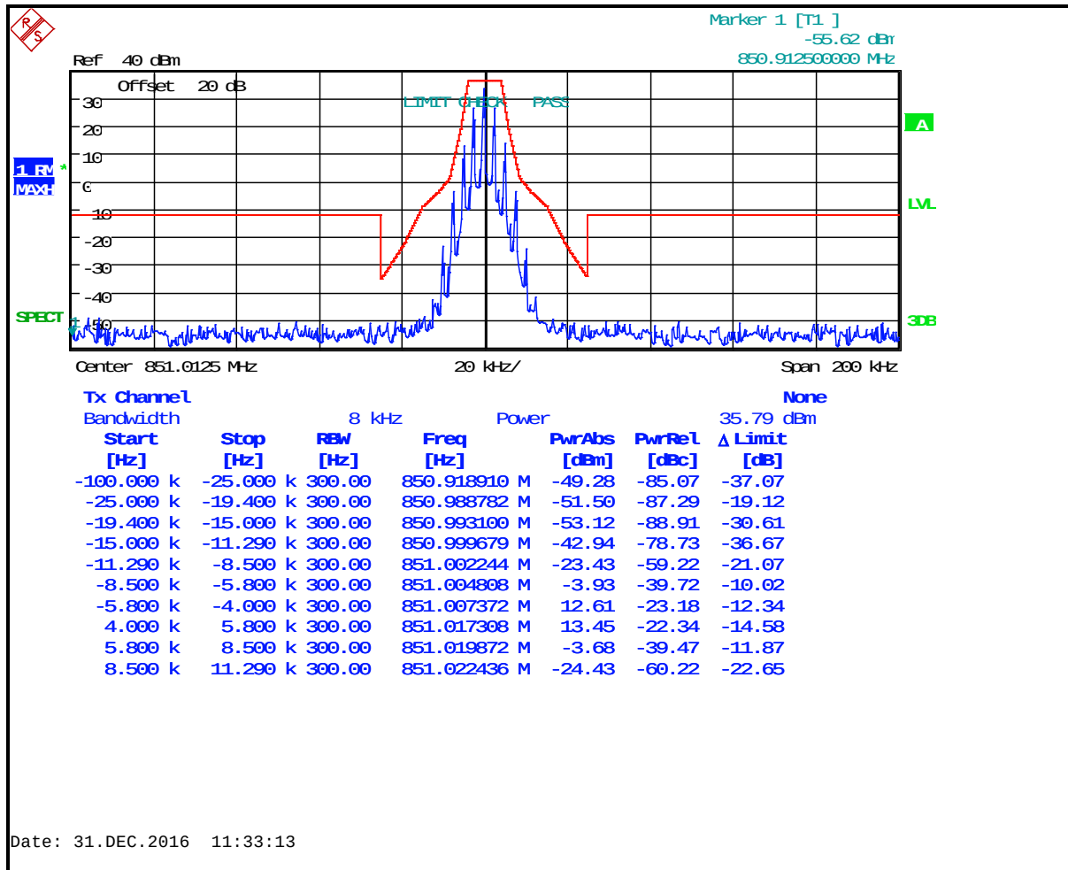
Plot 8-22: Occupied Bandwidth – 851.0125 MHz; Analog NPSPAC; Mask H
