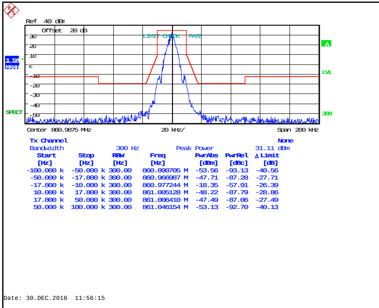
Plot 8-42: Occupied Bandwidth – 860.9875 MHz; 2-Level FSK 9600 NB; Mask G
