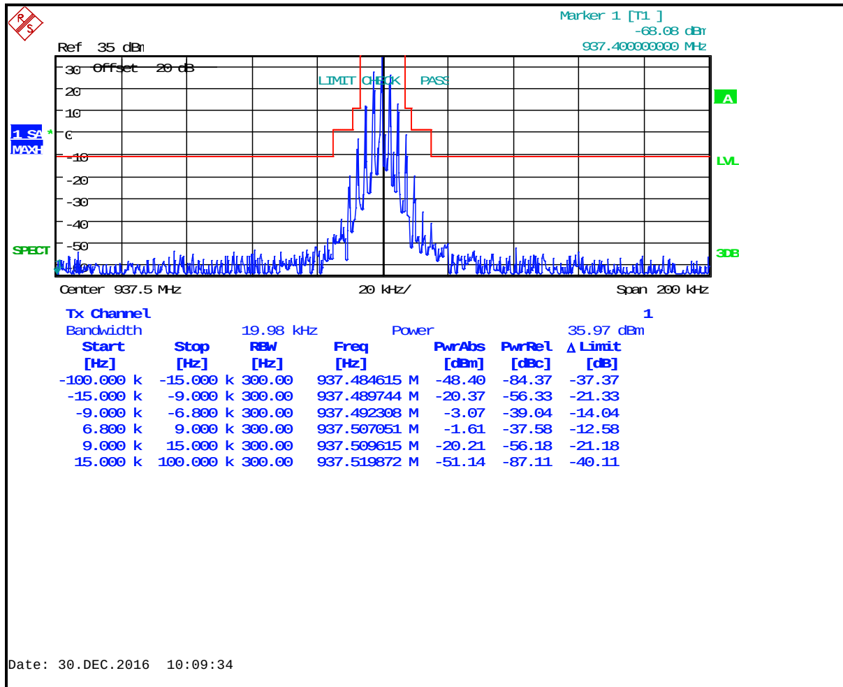
Plot 8-17: Occupied Bandwidth – 937.5 MHz; NB Analog; Mask I
