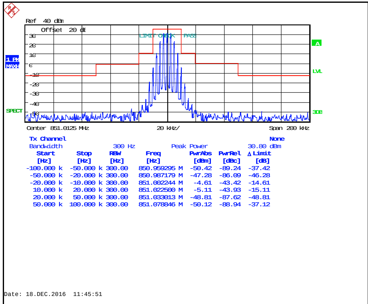
Plot 8-21: Occupied Bandwidth – 851.0125 MHz; Analog NPSPAC; Mask B
