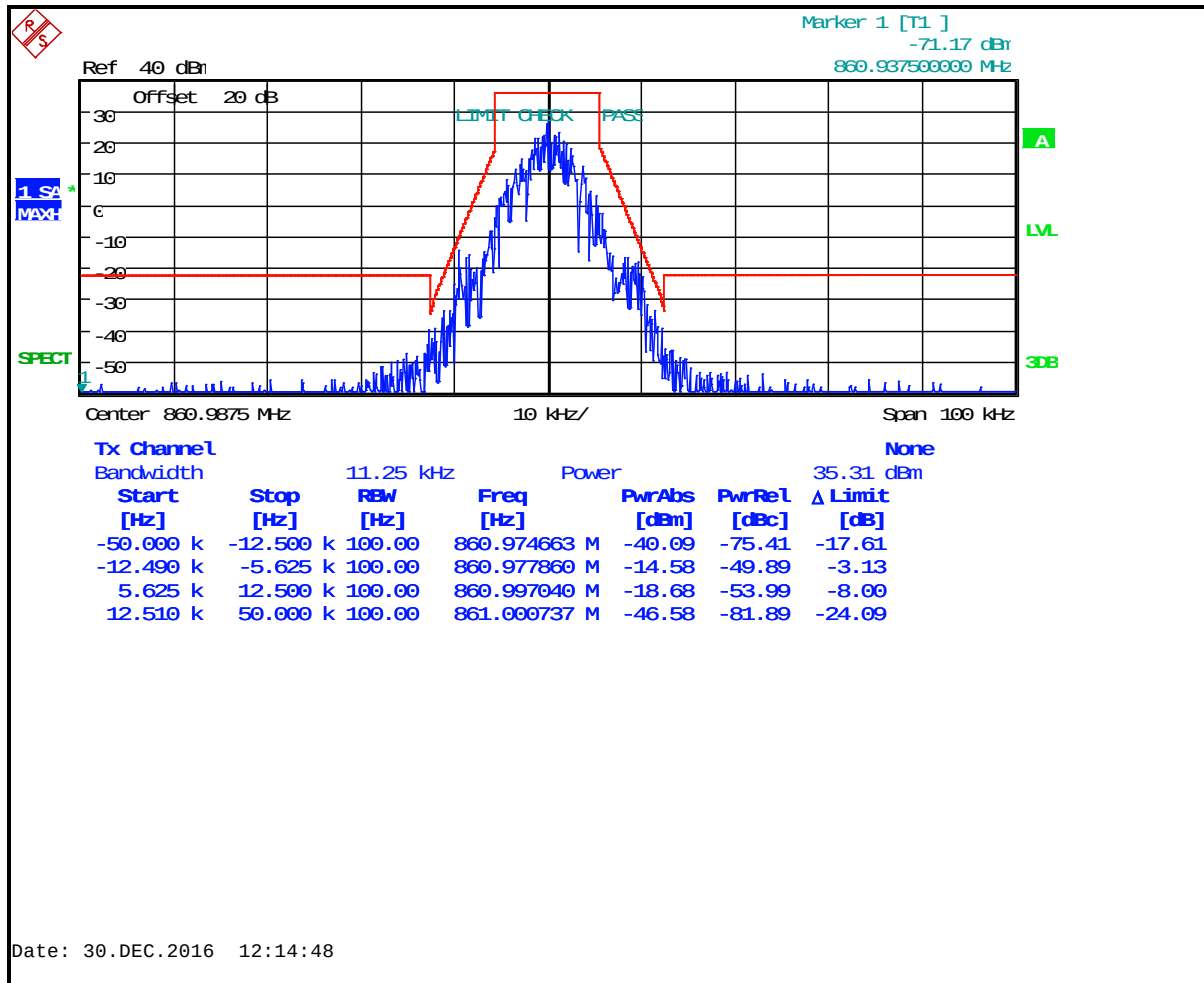
Plot 8-48: Occupied Bandwidth – 860.9875 MHz; 2-Level FSK 9600 NB; Mask D (IC)
