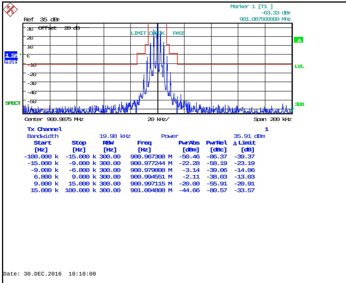
Plot 8-15: Occupied Bandwidth – 900.9875 MHz; NB Analog; Mask I
