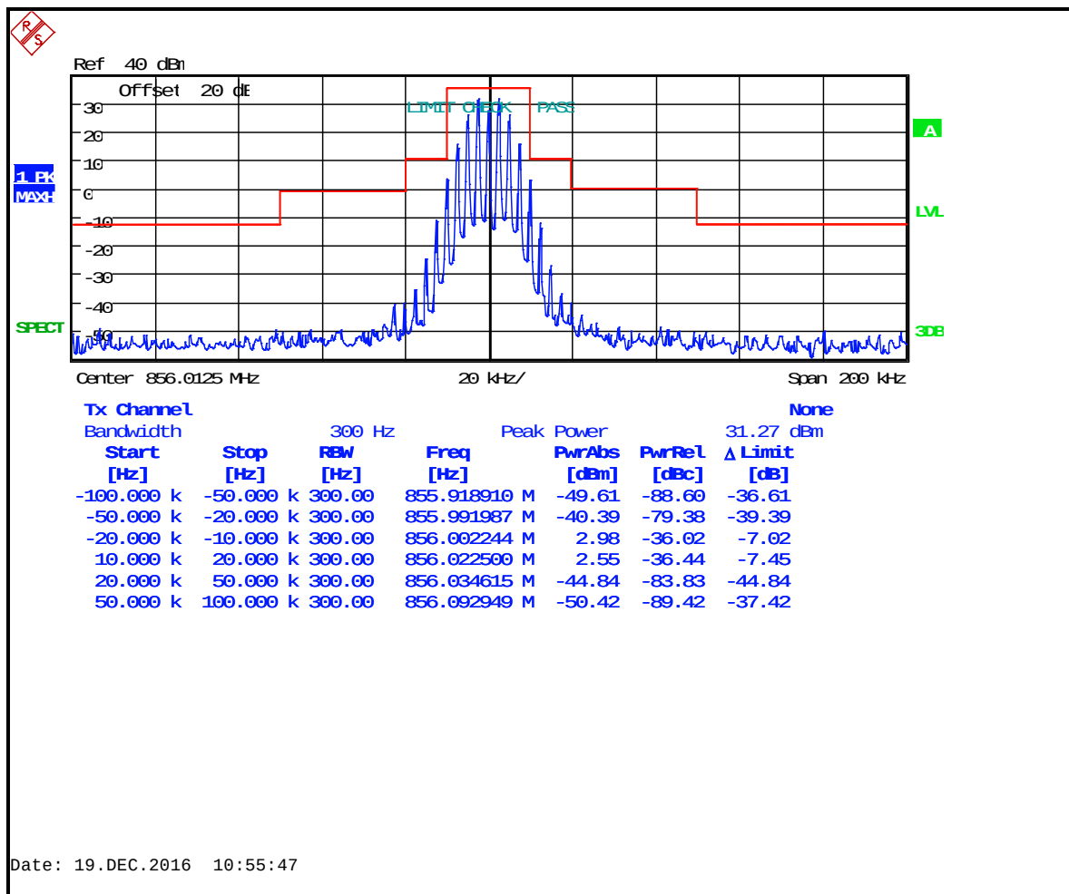
Plot 8-29: Occupied Bandwidth – 856.0125 MHz; WB Analog; Mask B
