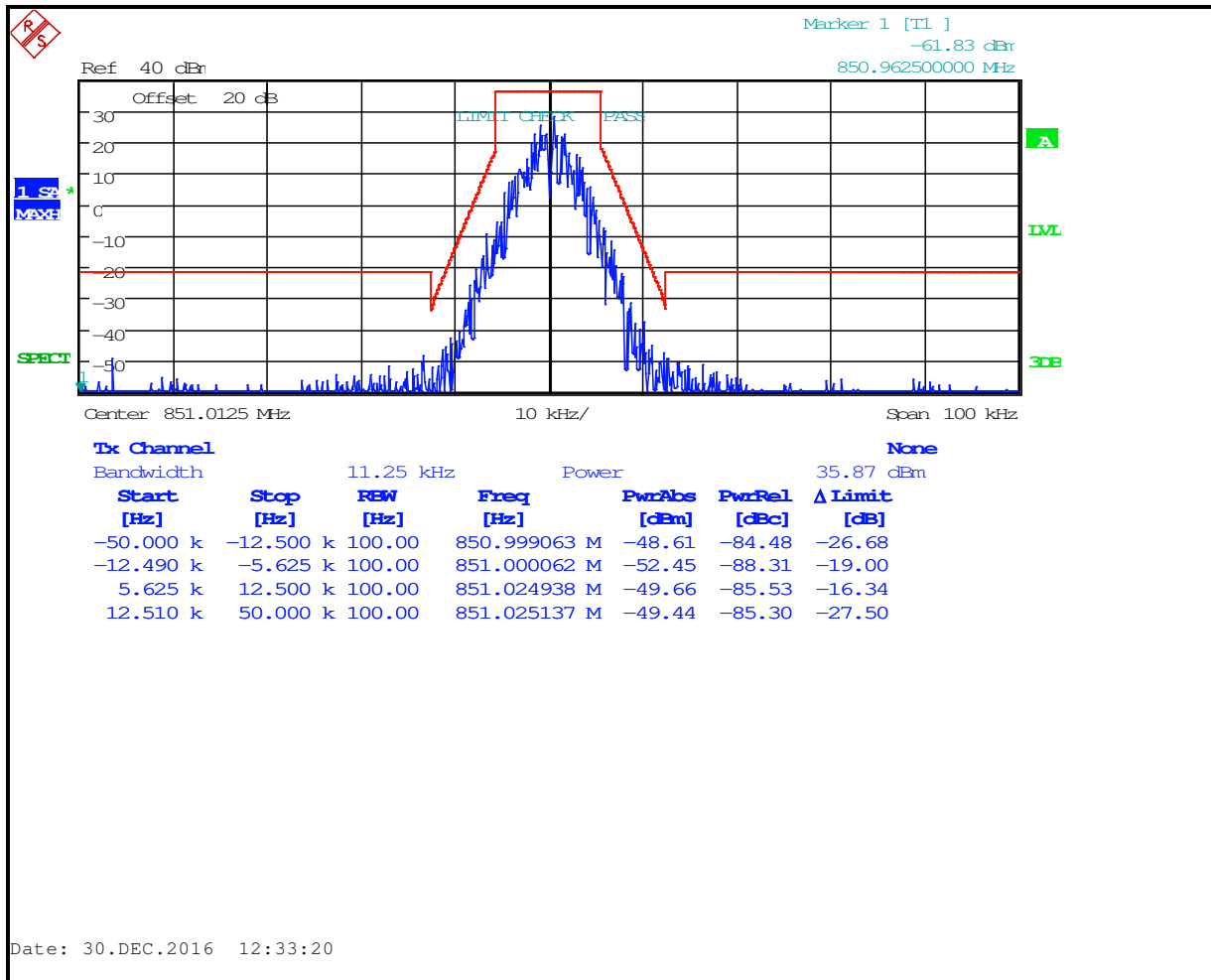
Plot 8-74: Occupied Bandwidth – 851.0125 MHz; P25; Mask D
