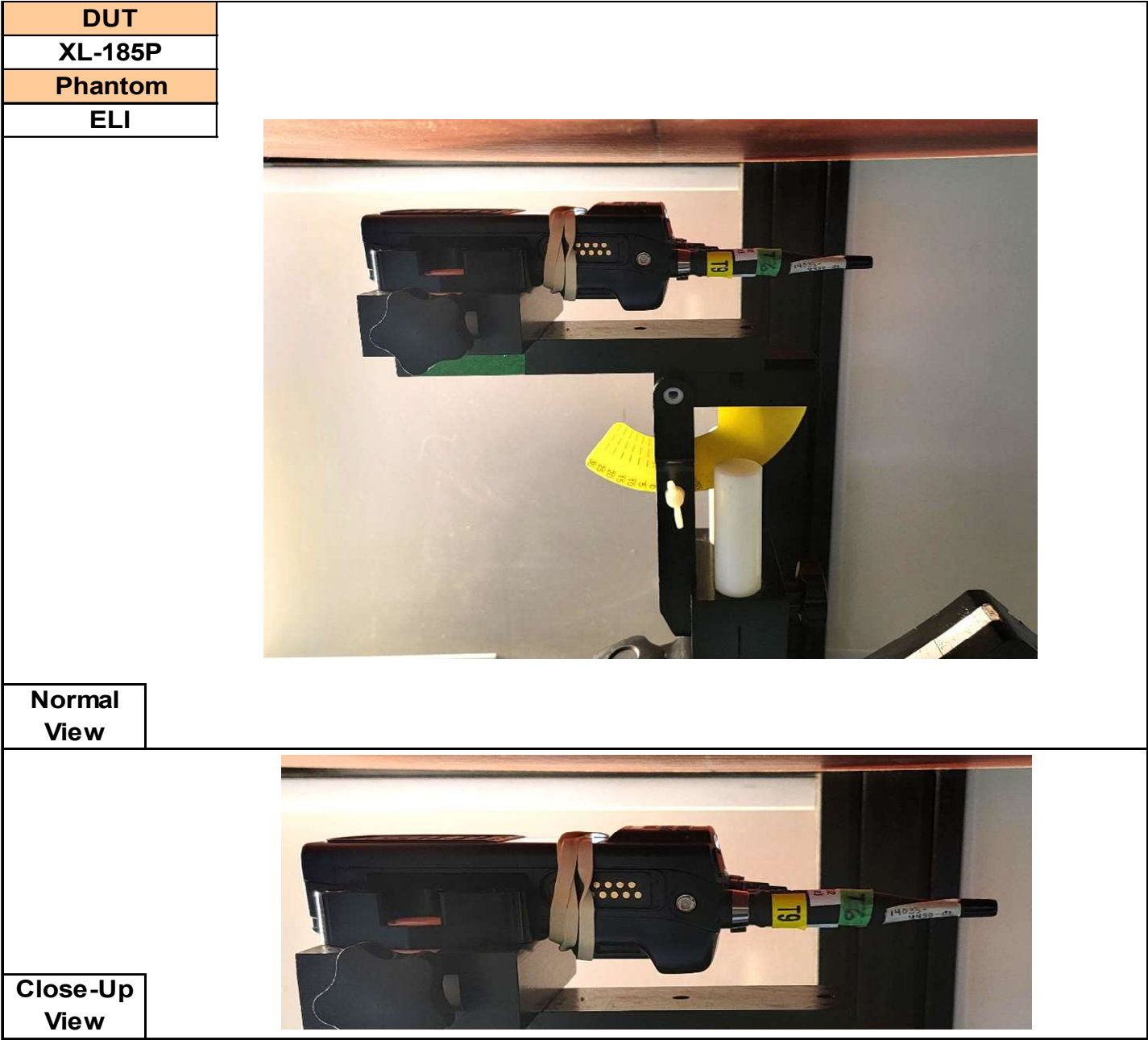
Figure 2: Photo – Setup, Face – P2, T9 (25mm)
