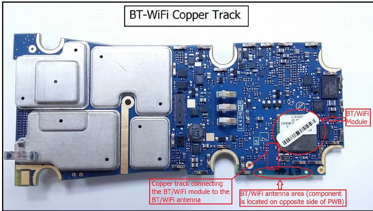
Bottom PWB with Shields
