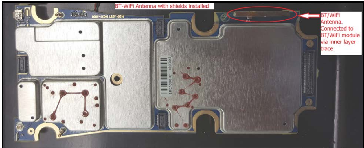
Top PWB with Shields
