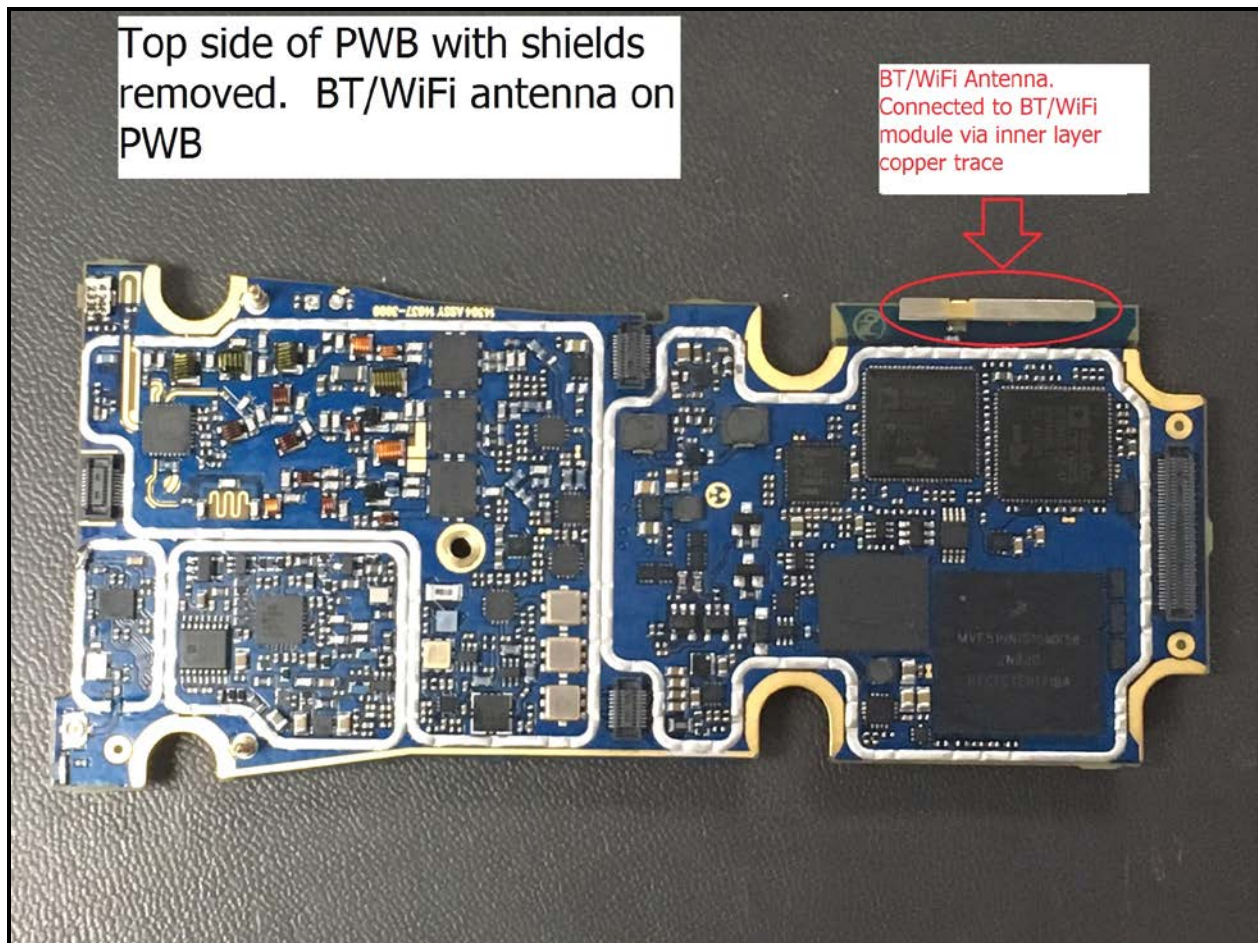
Top PWB without Shields
