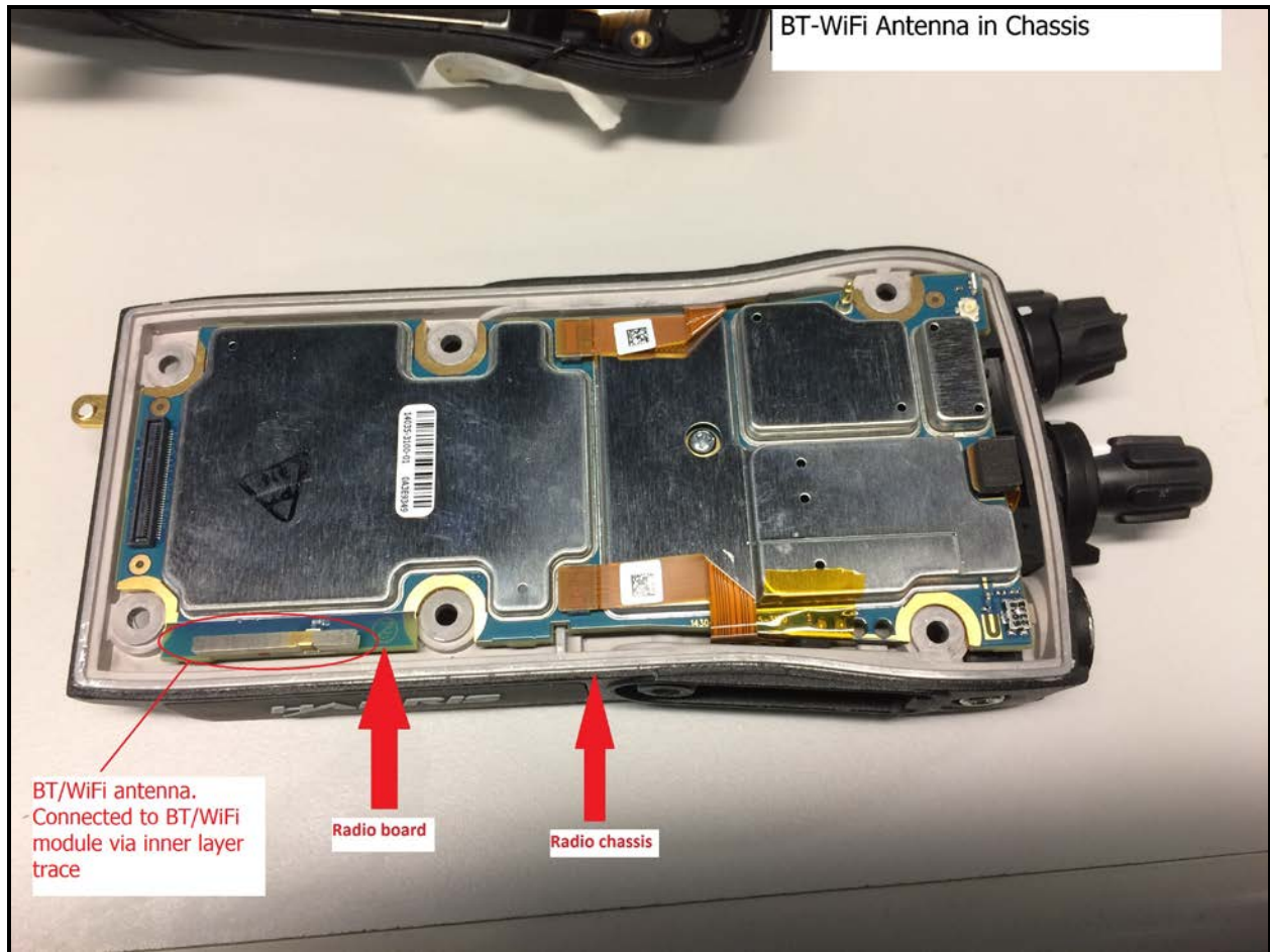
PWB in Chassis 2
