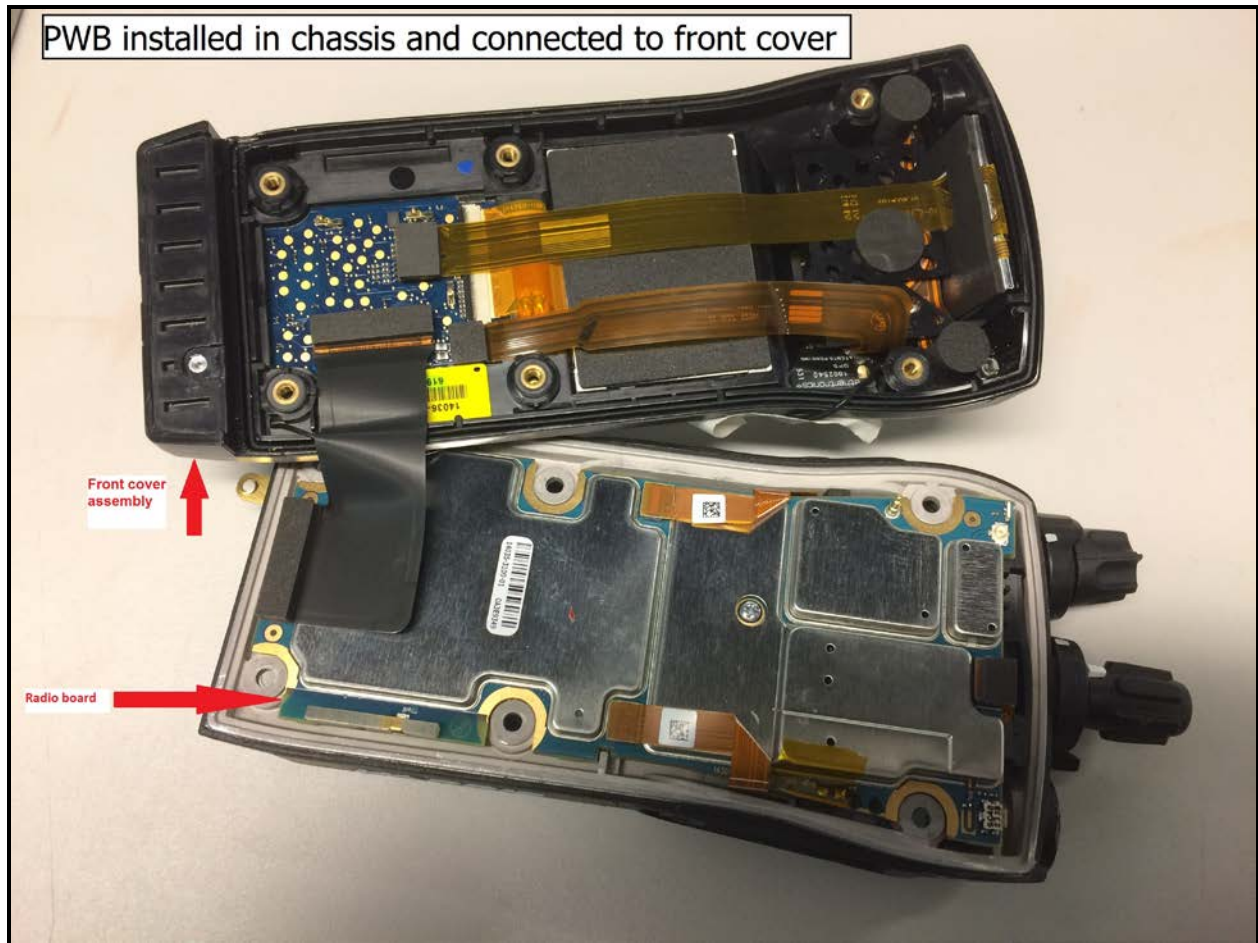
PWB in Chassis
