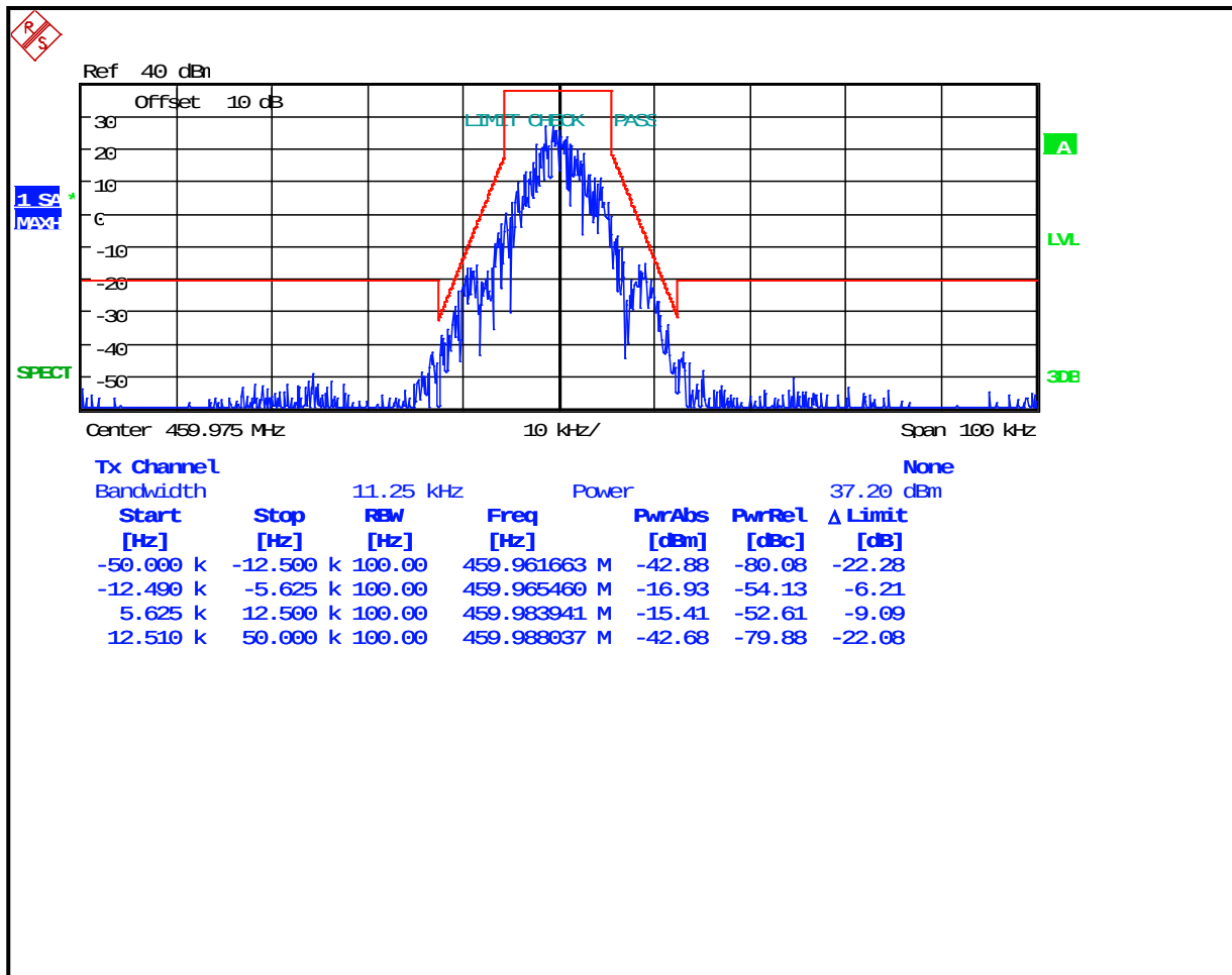
Plot 8-62: Occupied Bandwidth – 459.975 MHz; (2-level FSK 9600; NB) EDACS; Mask D
