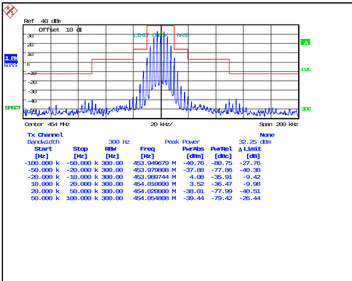
Plot 8-31: Occupied Bandwidth – 454 MHz; Wideband Analog; Mask B
