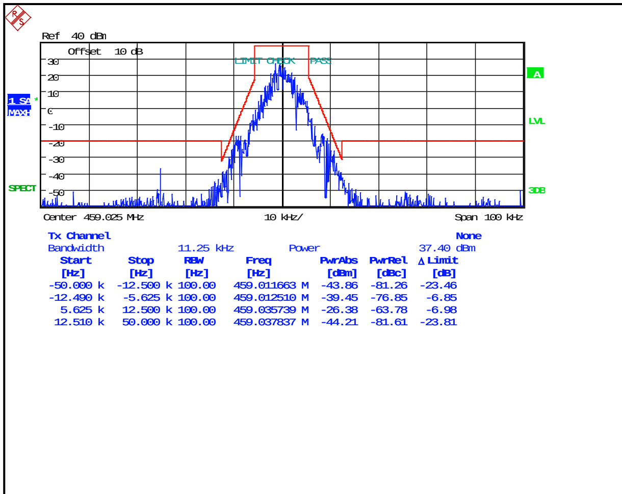
Plot 8-61: Occupied Bandwidth – 459.025 MHz; (2-level FSK 9600; NB) EDACS; Mask D
