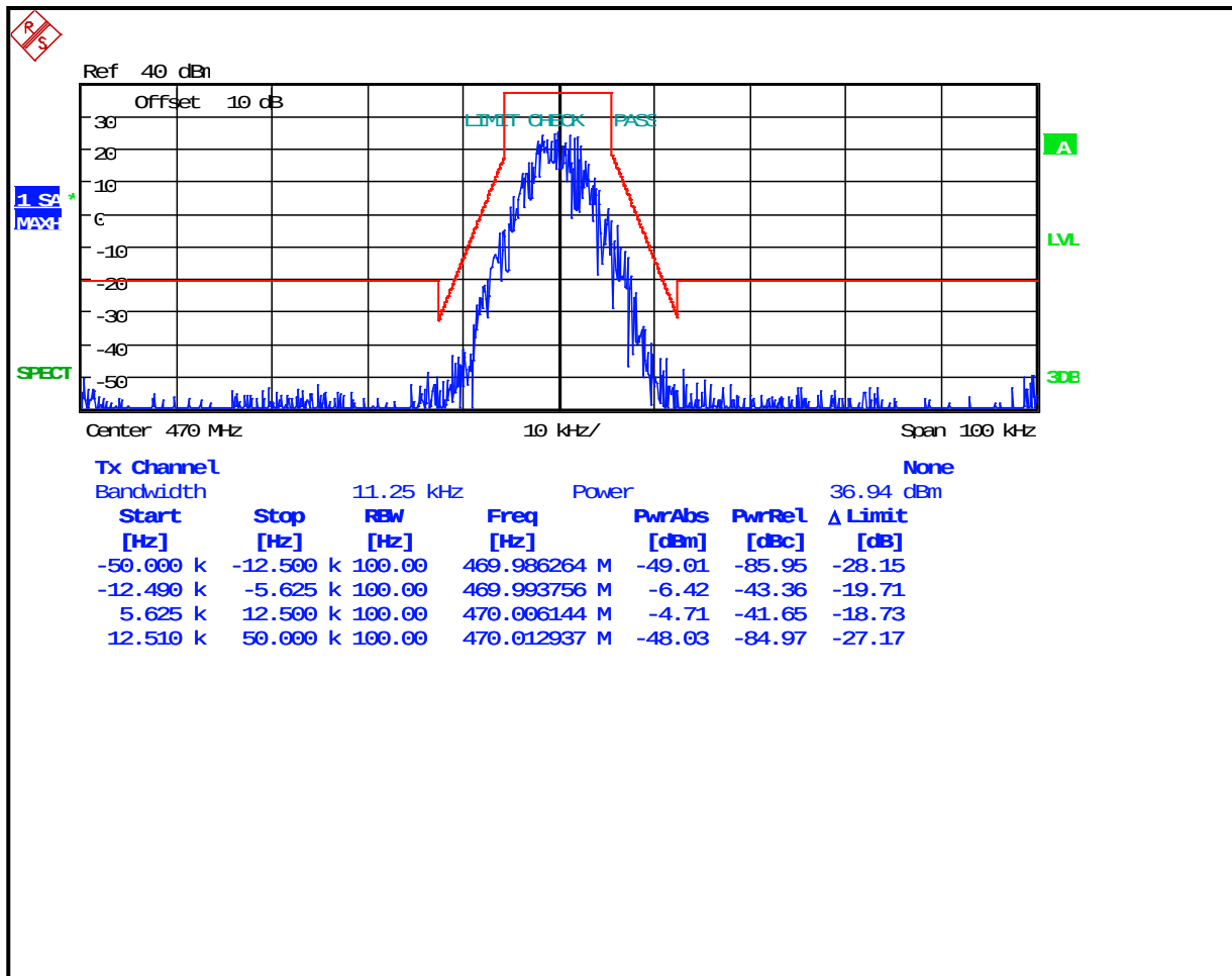
Plot 8-56: Occupied Bandwidth – 470 MHz; CPM TDMA; Mask D
