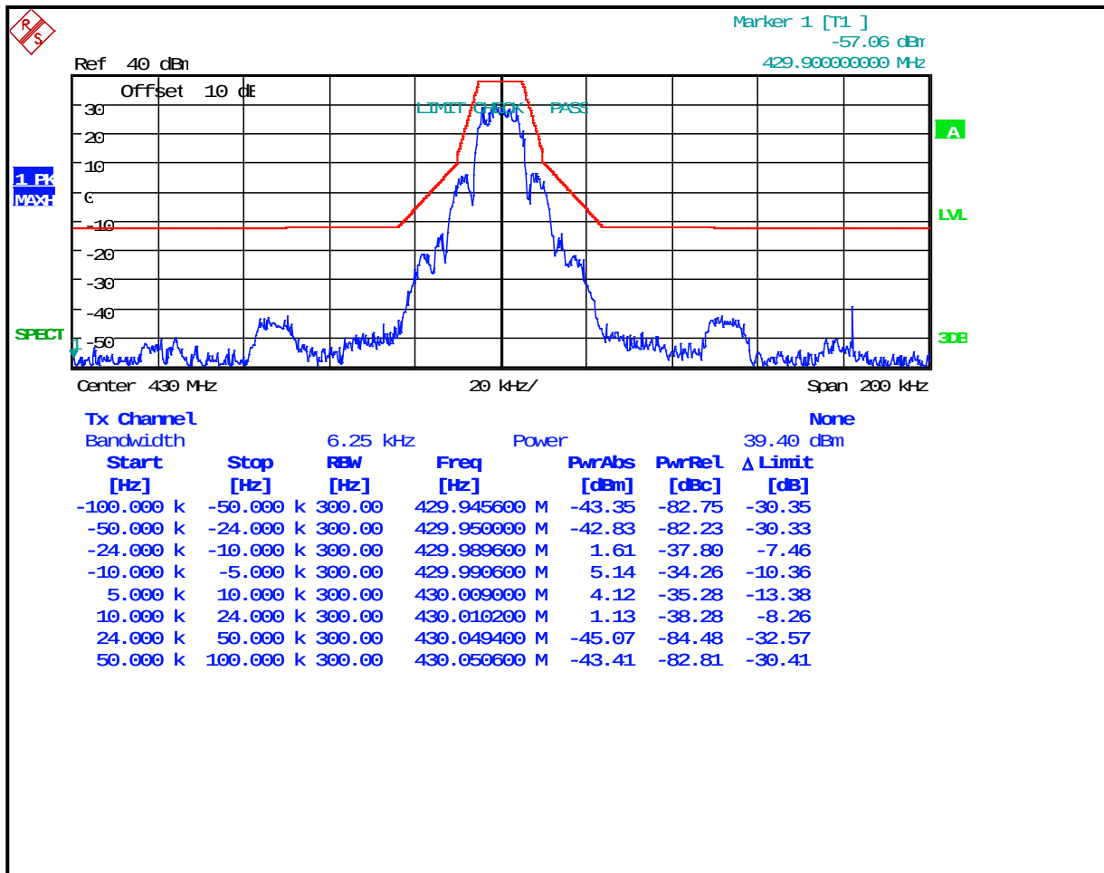
Plot 8-64: Occupied Bandwidth – 430 MHz; (2-level FSK 9600; WB) EDACS; Mask C
