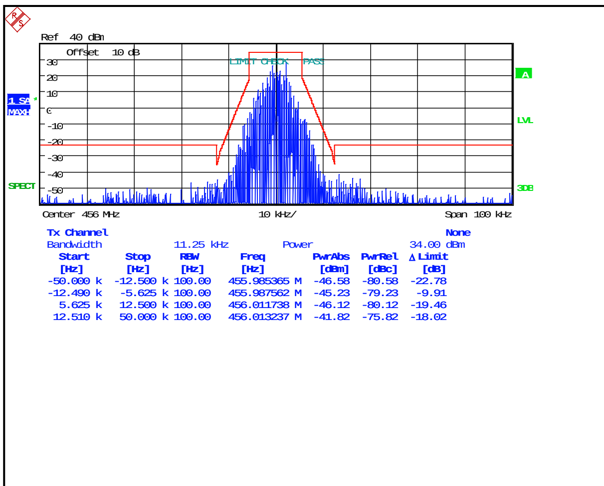
Plot 8-53: Occupied Bandwidth – 456MHz; CPM TDMA; Mask D
