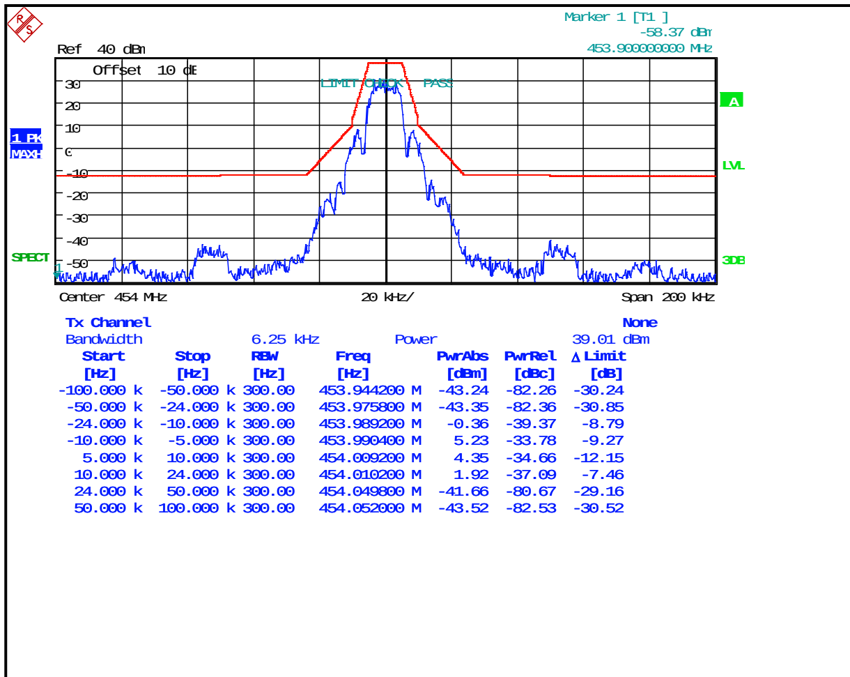
Plot 8-66: Occupied Bandwidth – 454 MHz; (2-level FSK 9600; WB) EDACS; Mask C
