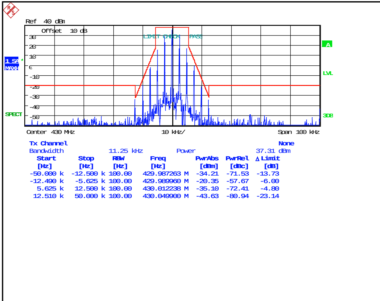
Plot 8-36: Occupied Bandwidth – 430 MHz; Narrowband Analog; Mask D
