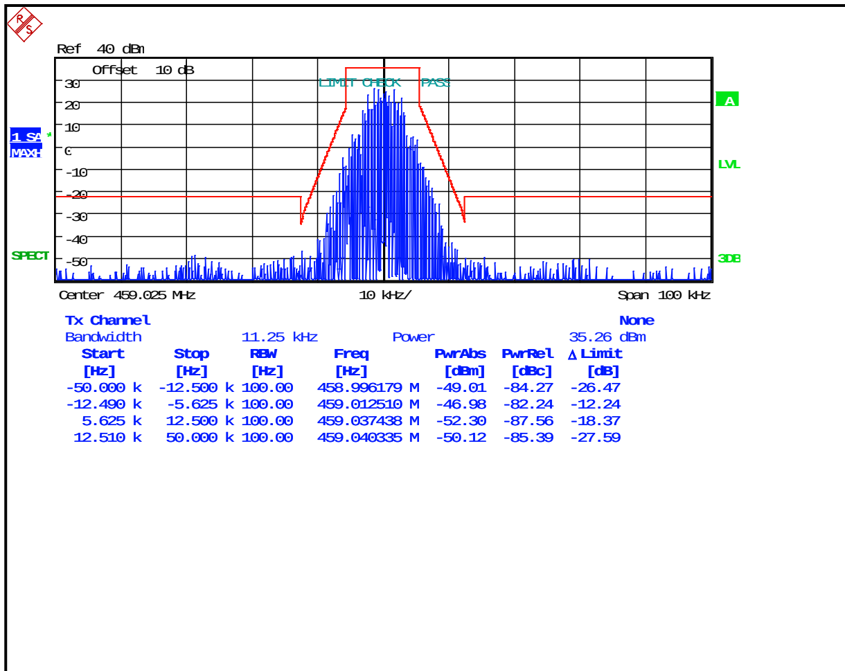
Plot 8-54: Occupied Bandwidth – 459.025 MHz; CPM TDMA; Mask D
