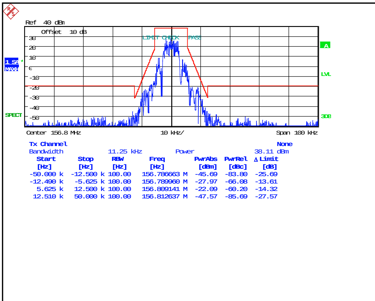
Plot 8-18: Occupied Bandwidth – 156.8 MHz; 2-Level FSK 4800; XNB EDACS; (Mask D)
