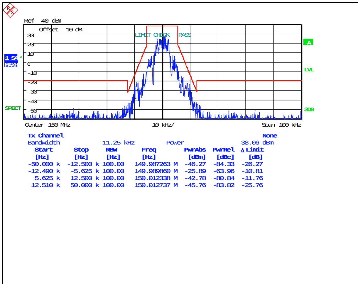
Plot 8-17: Occupied Bandwidth – 150 MHz; 2-Level FSK 4800; XNB EDACS; (Mask D)
