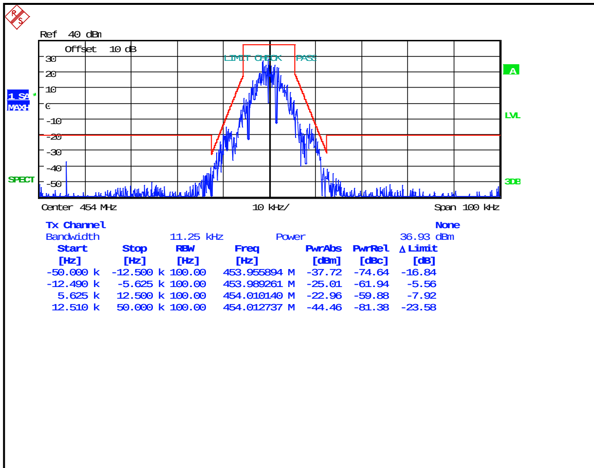
Plot 8-59: Occupied Bandwidth – 454 MHz; (2-level FSK 9600; NB) EDACS; Mask D
