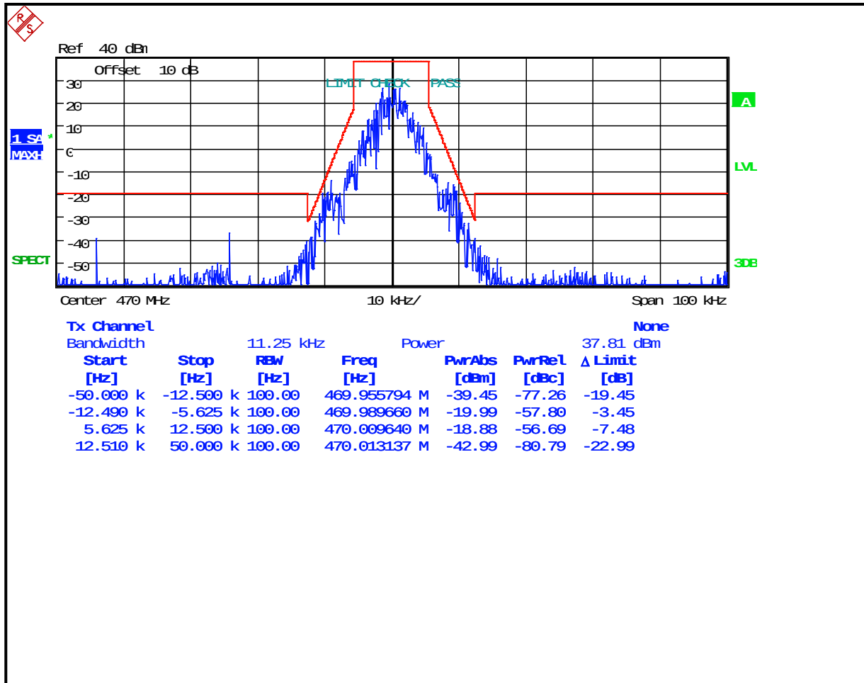
Plot 8-63: Occupied Bandwidth – 470 MHz; (2-level FSK 9600; NB) EDACS; Mask D
