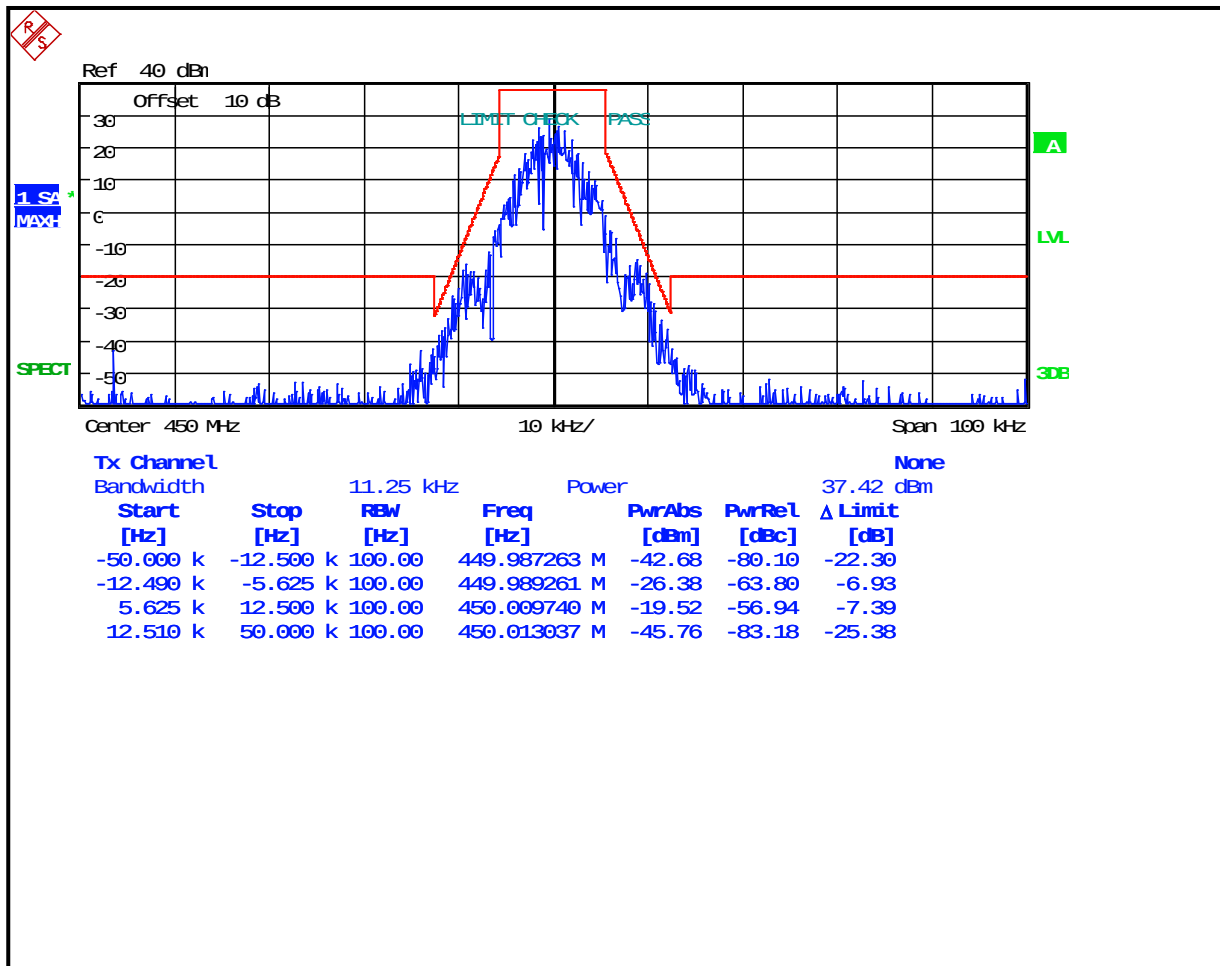
Plot 8-58: Occupied Bandwidth – 450 MHz; (2-level FSK 9600; NB) EDACS; Mask D
