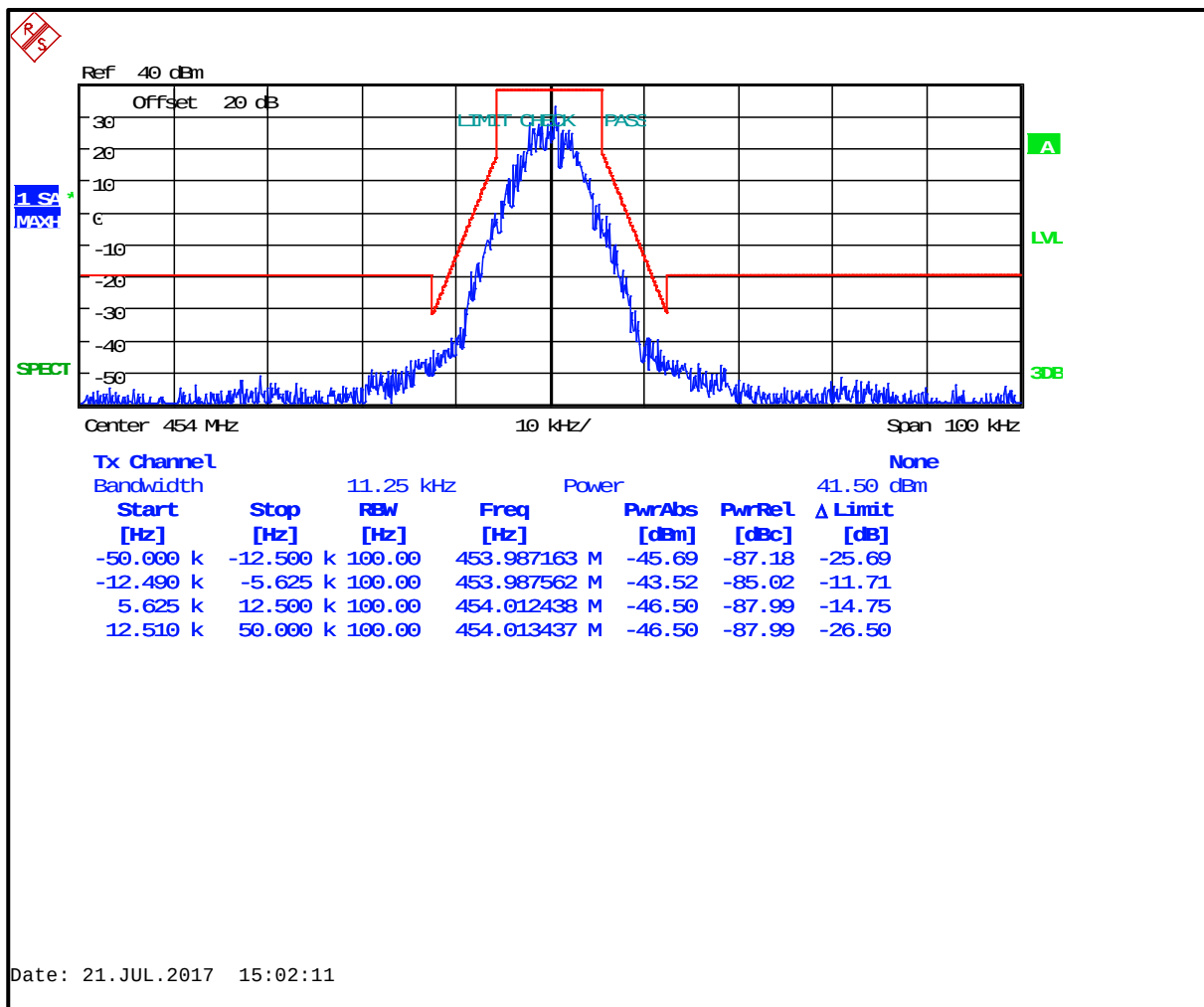
Plot 8-45: Occupied Bandwidth – 454 MHz; P25; Mask D
