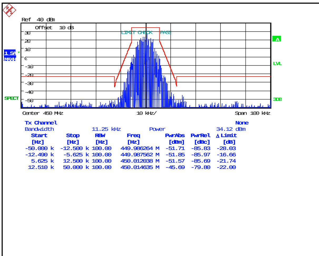
Plot 8-51: Occupied Bandwidth – 450 MHz; CPM TDMA; Mask D
