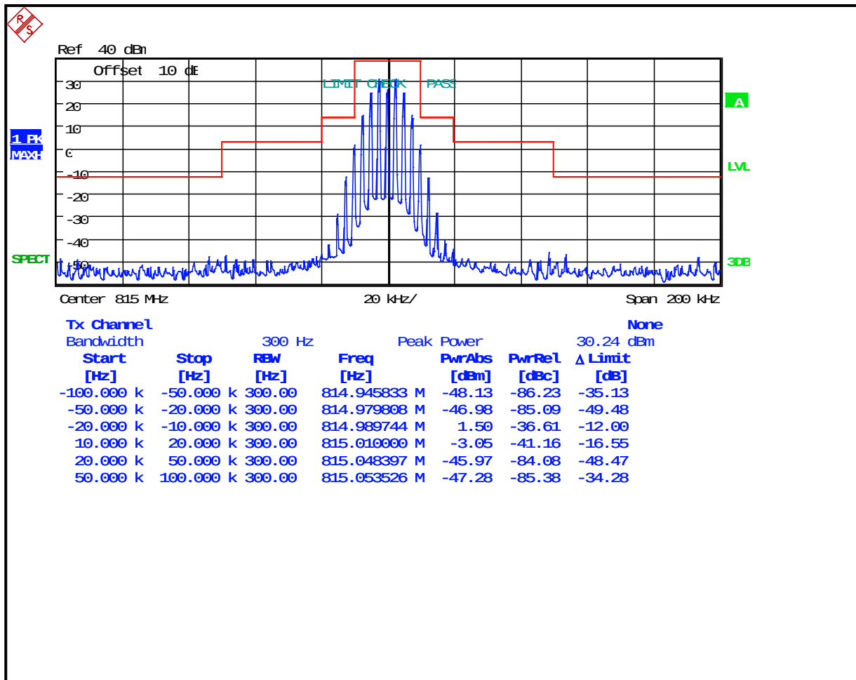
Plot 8-82: Occupied Bandwidth – 815 MHz; Wideband Analog; Mask B
