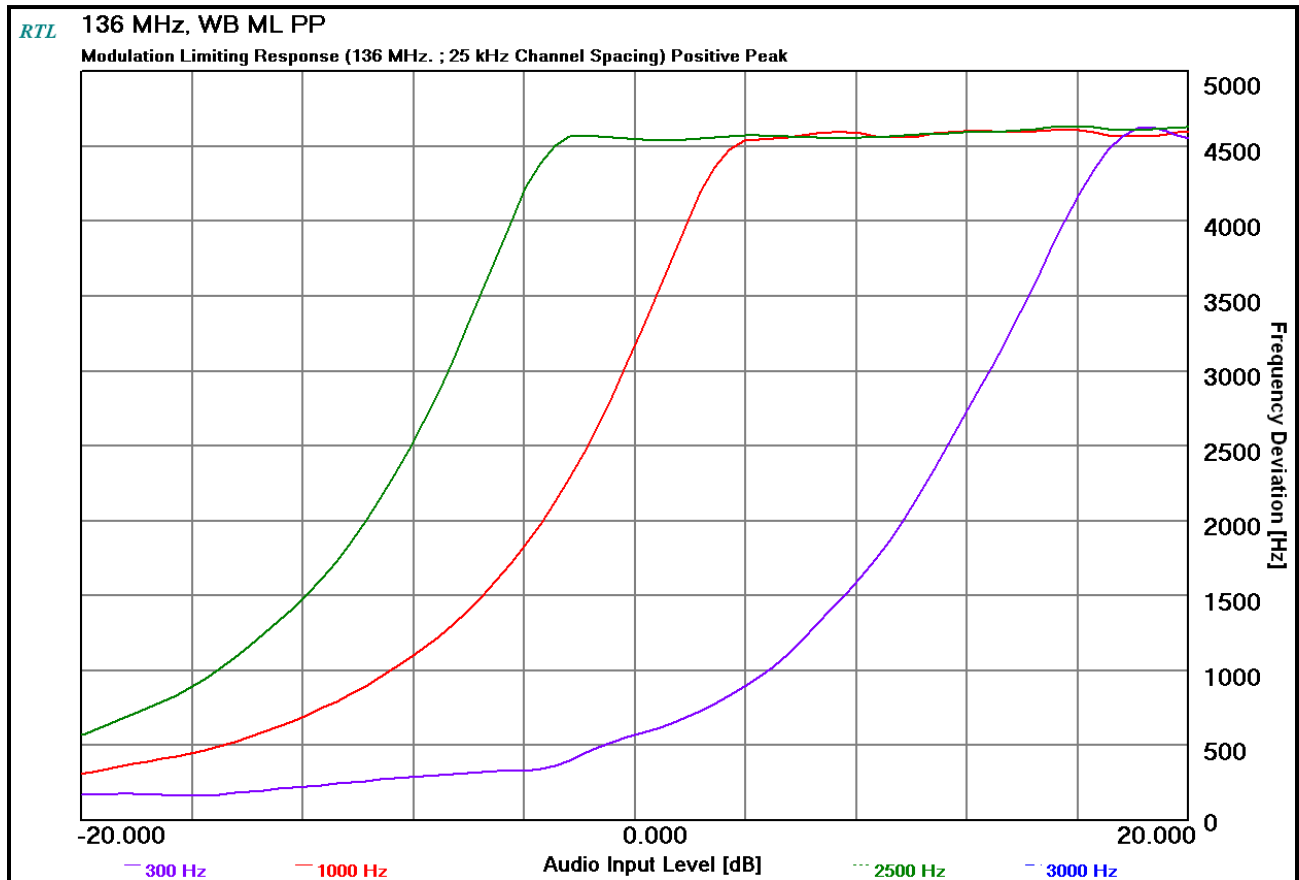
Plot 10-20: Modulation Characteristics – Modulation Limiting - 136 MHz; Positive Peak; WB
