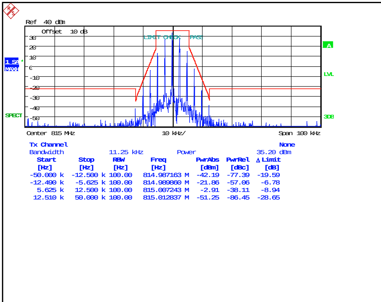
Plot 8-78: Occupied Bandwidth – 815 MHz; Narrowband Analog; Mask D
