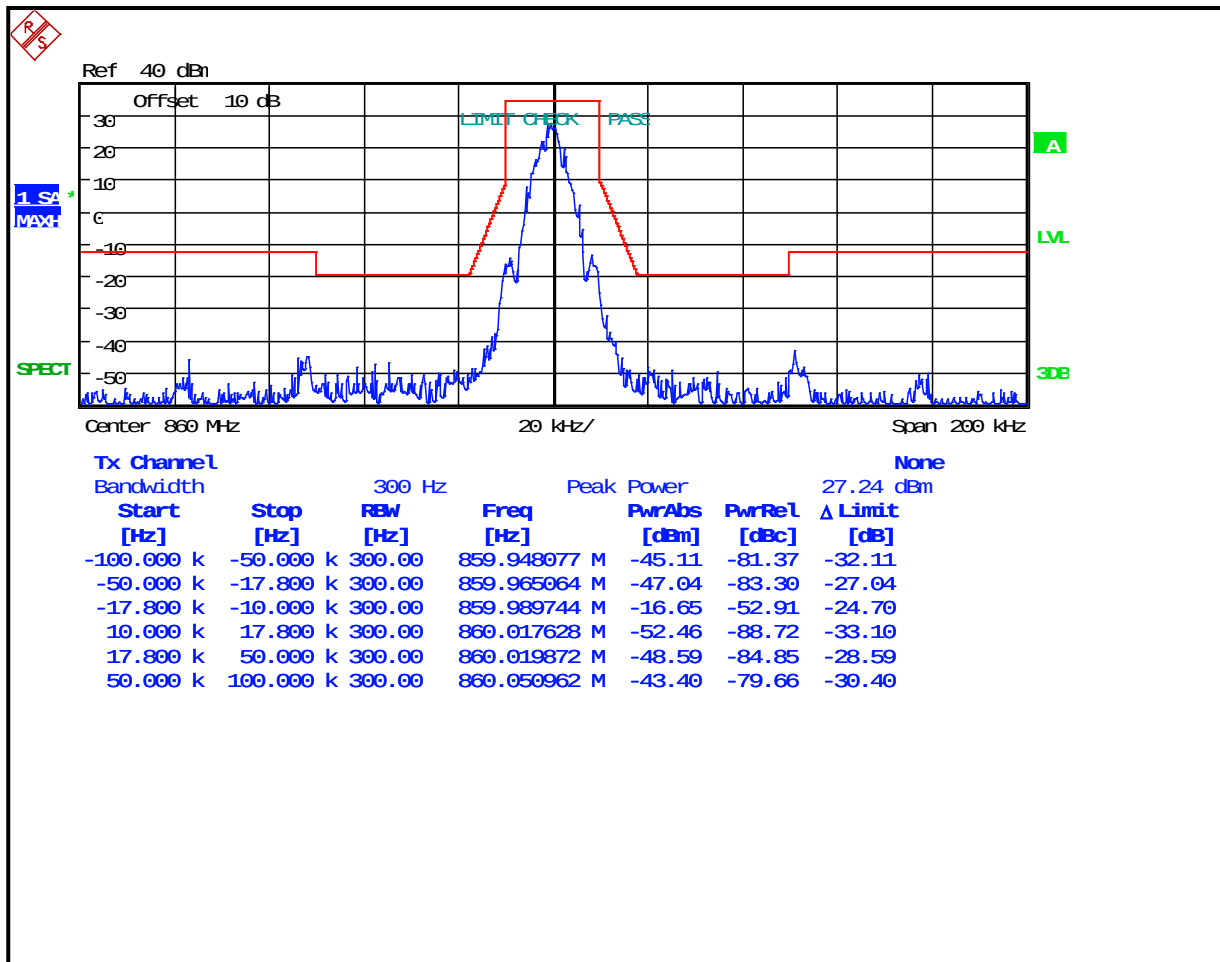
Plot 8-99: Occupied Bandwidth – 860 MHz; 2-level FSK 9600; NB EDACS; Mask G
