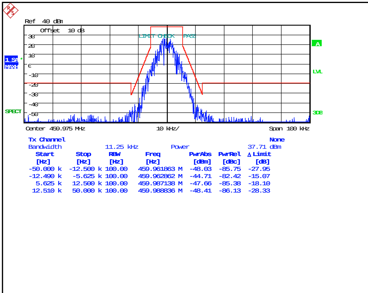
Plot 8-76: Occupied Bandwidth – 459.975MHz; (4-level FSK Data/Voice; NB) OpenSky; Mask D
