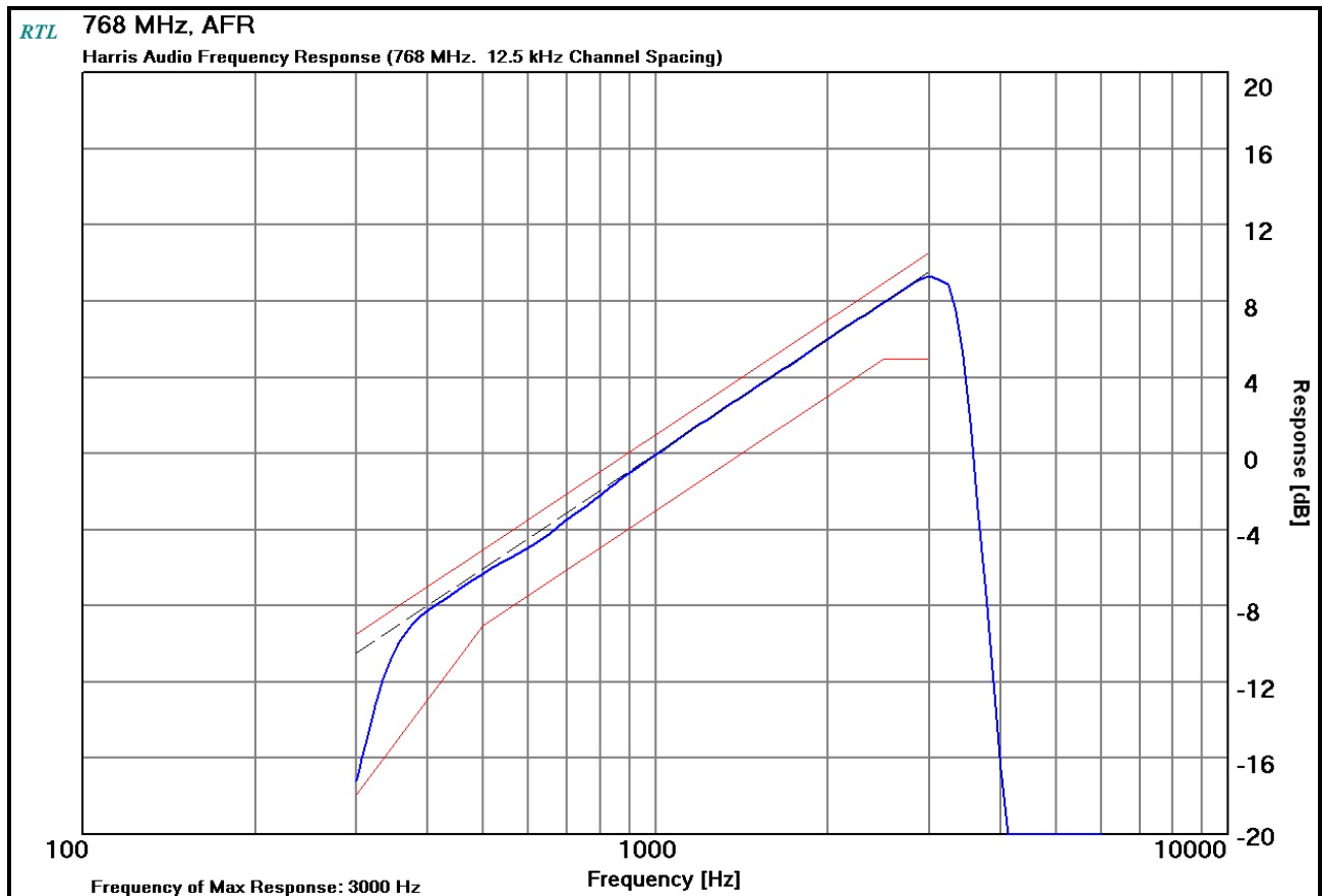
Plot 10-4: Modulation Characteristics - Audio Frequency Response - 768 MHz
