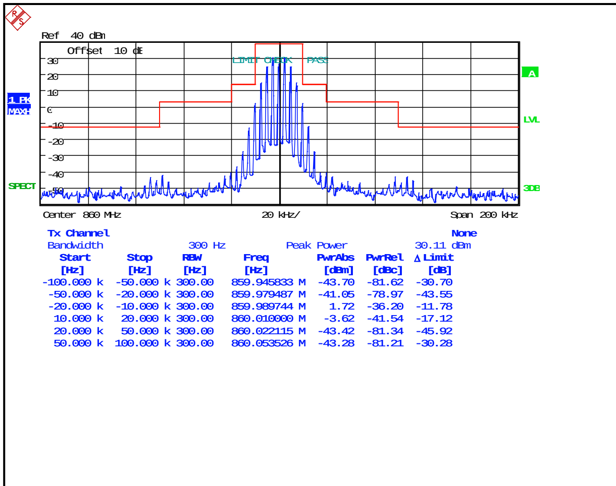
Plot 8-83: Occupied Bandwidth – 860 MHz; Wideband Analog; Mask B
