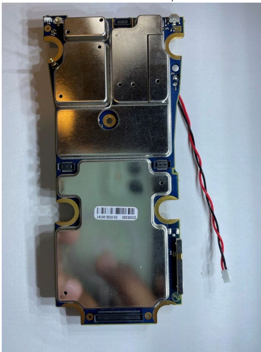
Main Board with Shields – Top View
