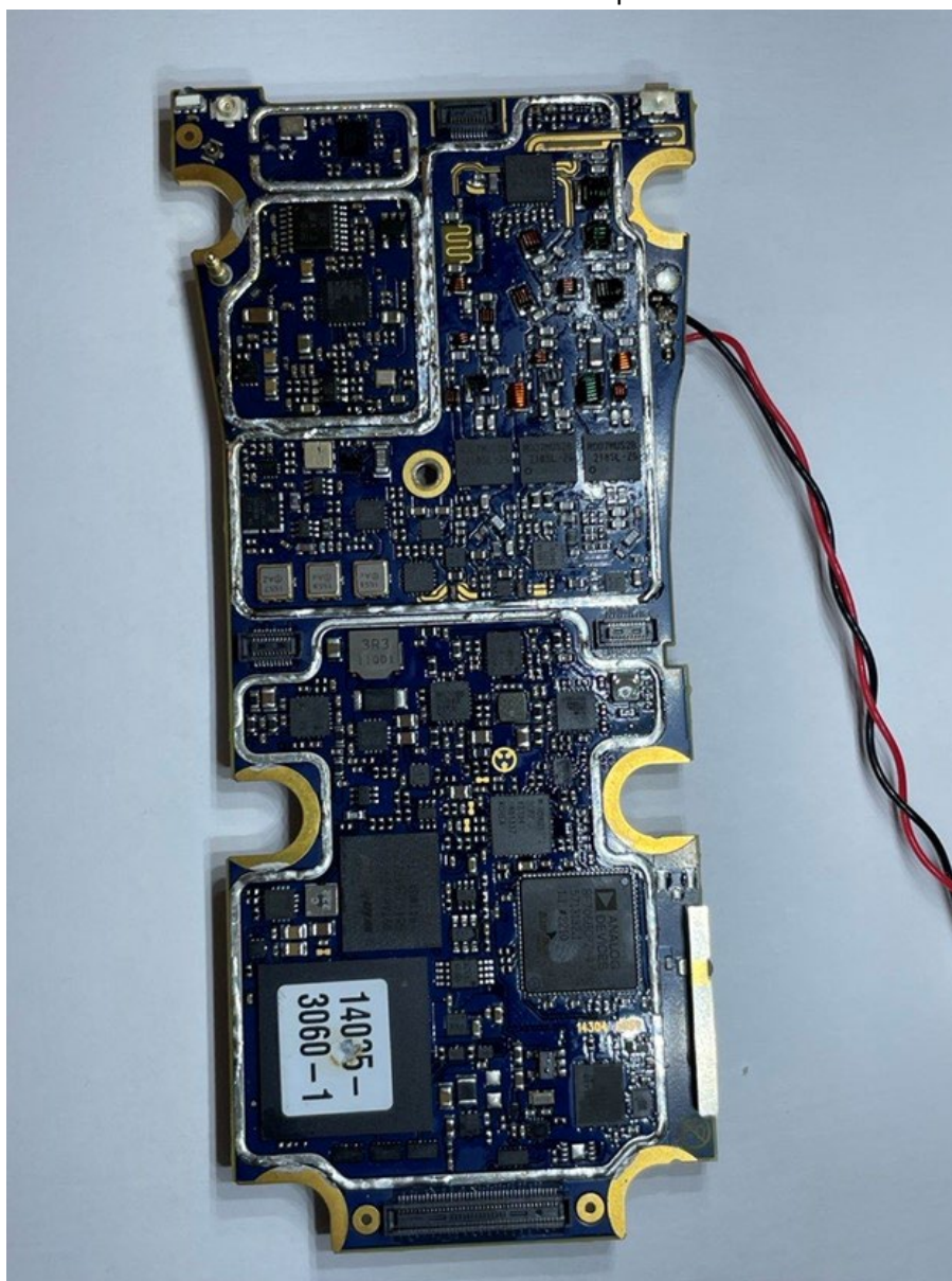
Main Board No Shields – Top View
