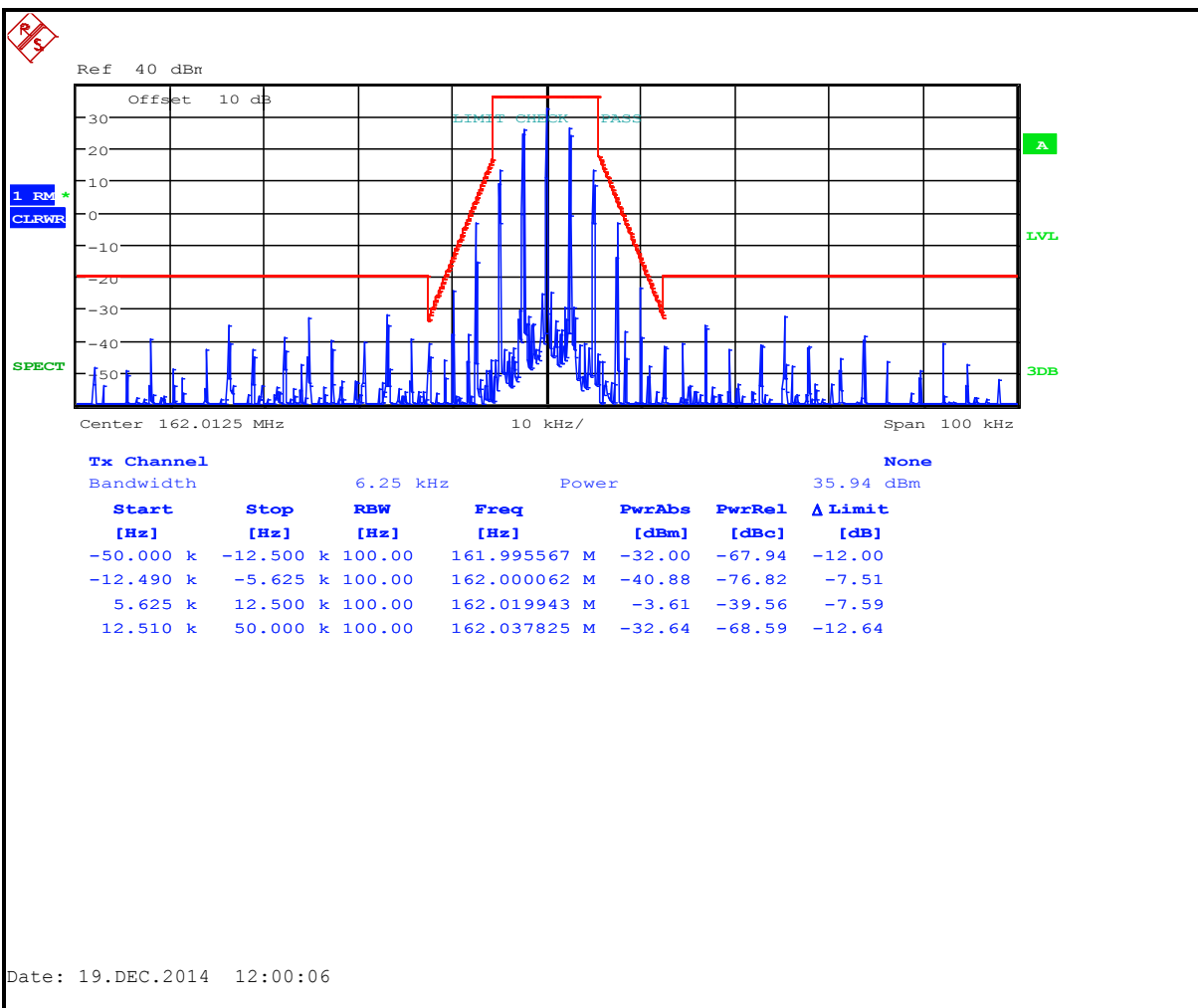
Plot 8-8: Occupied Bandwidth – 162.0125 MHz; Narrowband Analog (Mask D)
