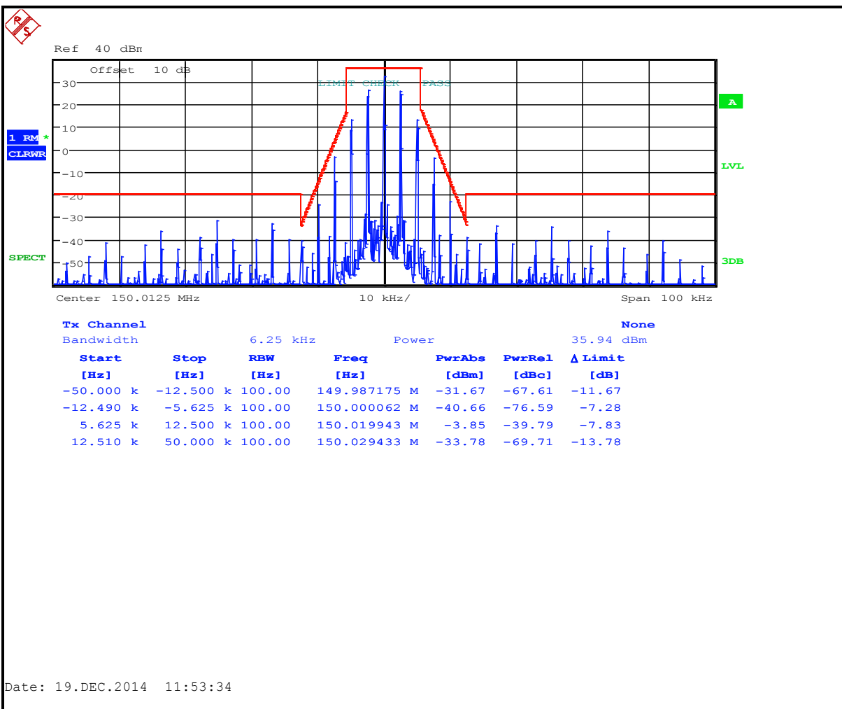
Plot 8-6: Occupied Bandwidth – 150.0125 MHz; Narrowband Analog (Mask D)
