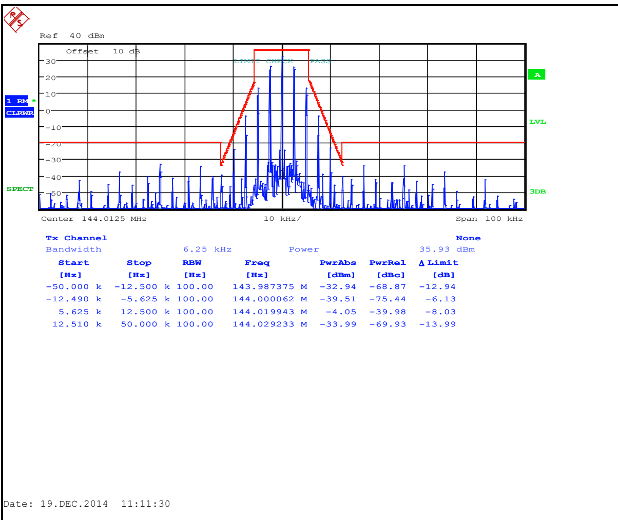
Plot 8-4: Occupied Bandwidth – 144.0125 MHz; Narrowband Analog (Mask D)
