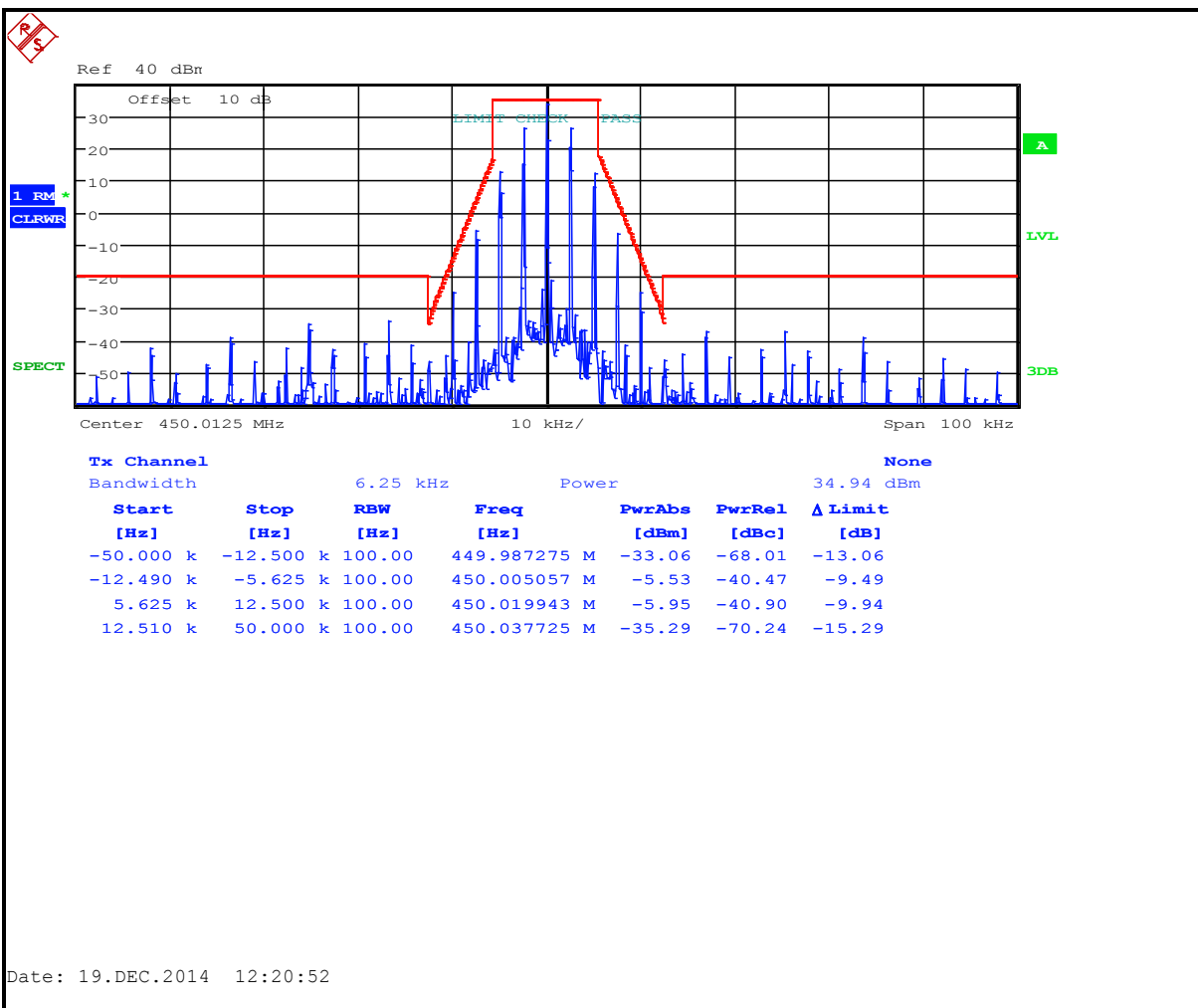
Plot 8-13: Occupied Bandwidth – 450.0125 MHz; Narrowband Analog (Mask D)
