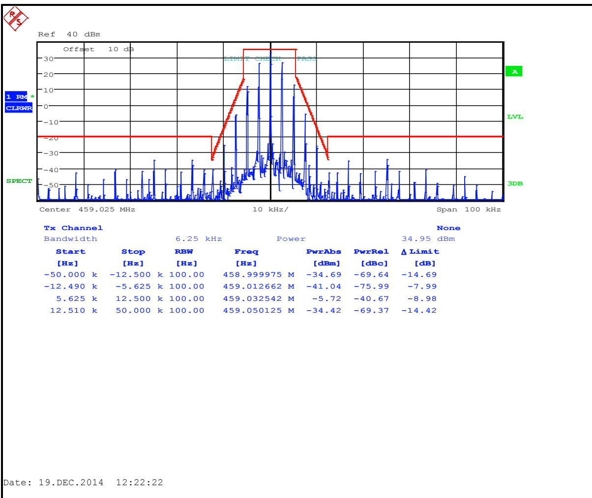
Plot 8-16: Occupied Bandwidth – 459.0250 MHz; Narrowband Analog (Mask D)
