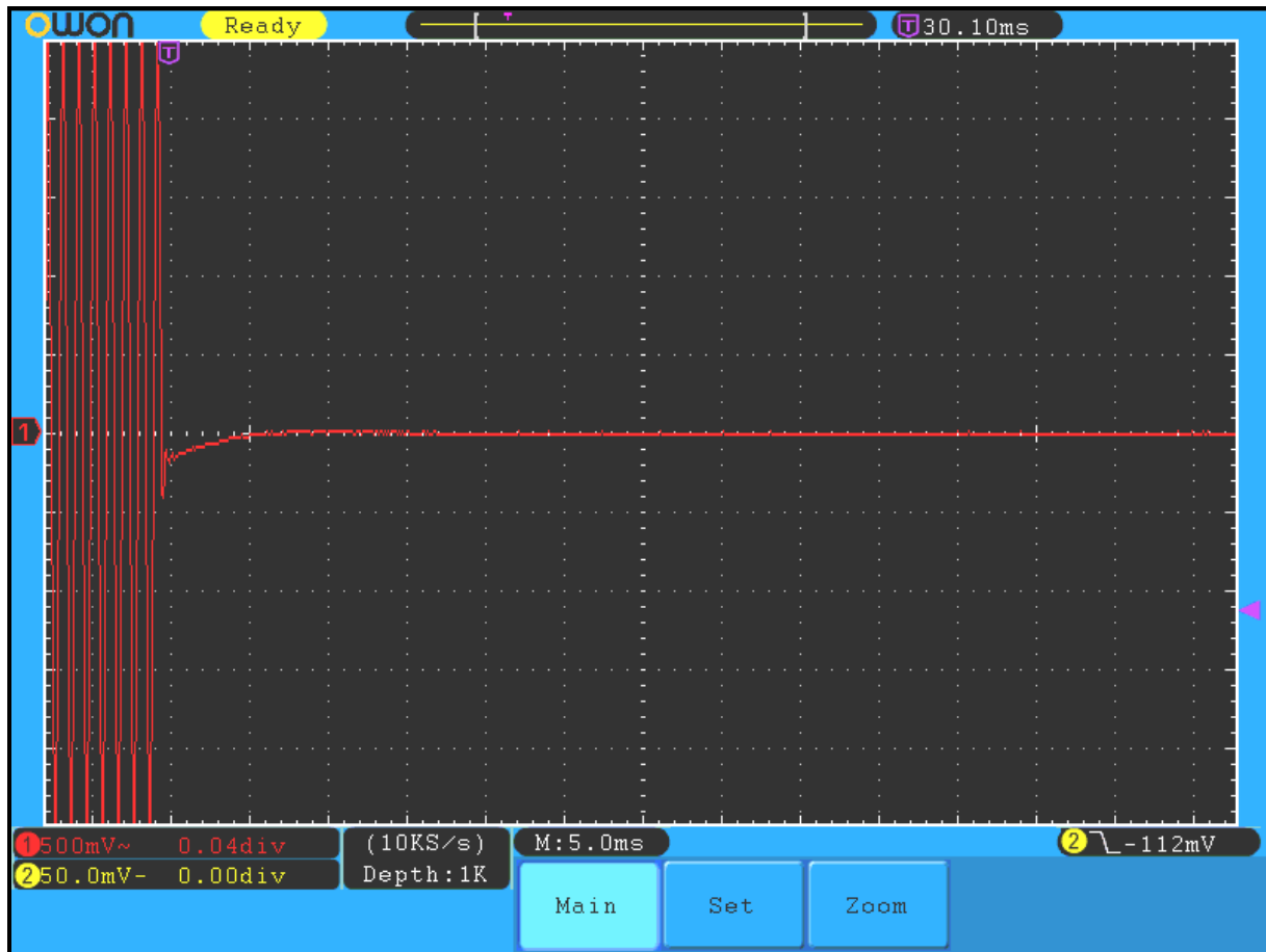
Plot 11-13: Transient Frequency Behavior – 173.9875 MHz; Wide Band; Carrier ON Time
