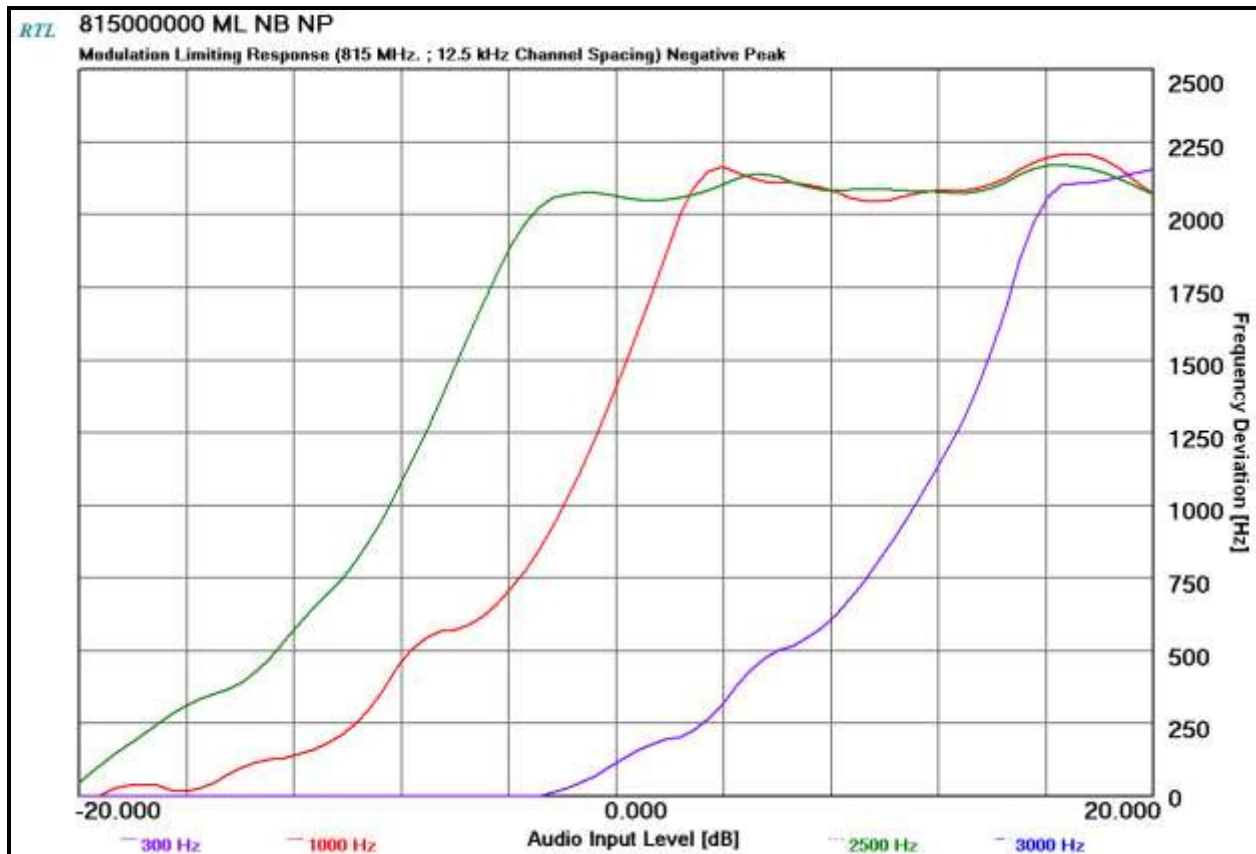
Plot 10-46: Modulation Characteristics – Modulation Limiting – 815 MHz; Negative Peak; NB
