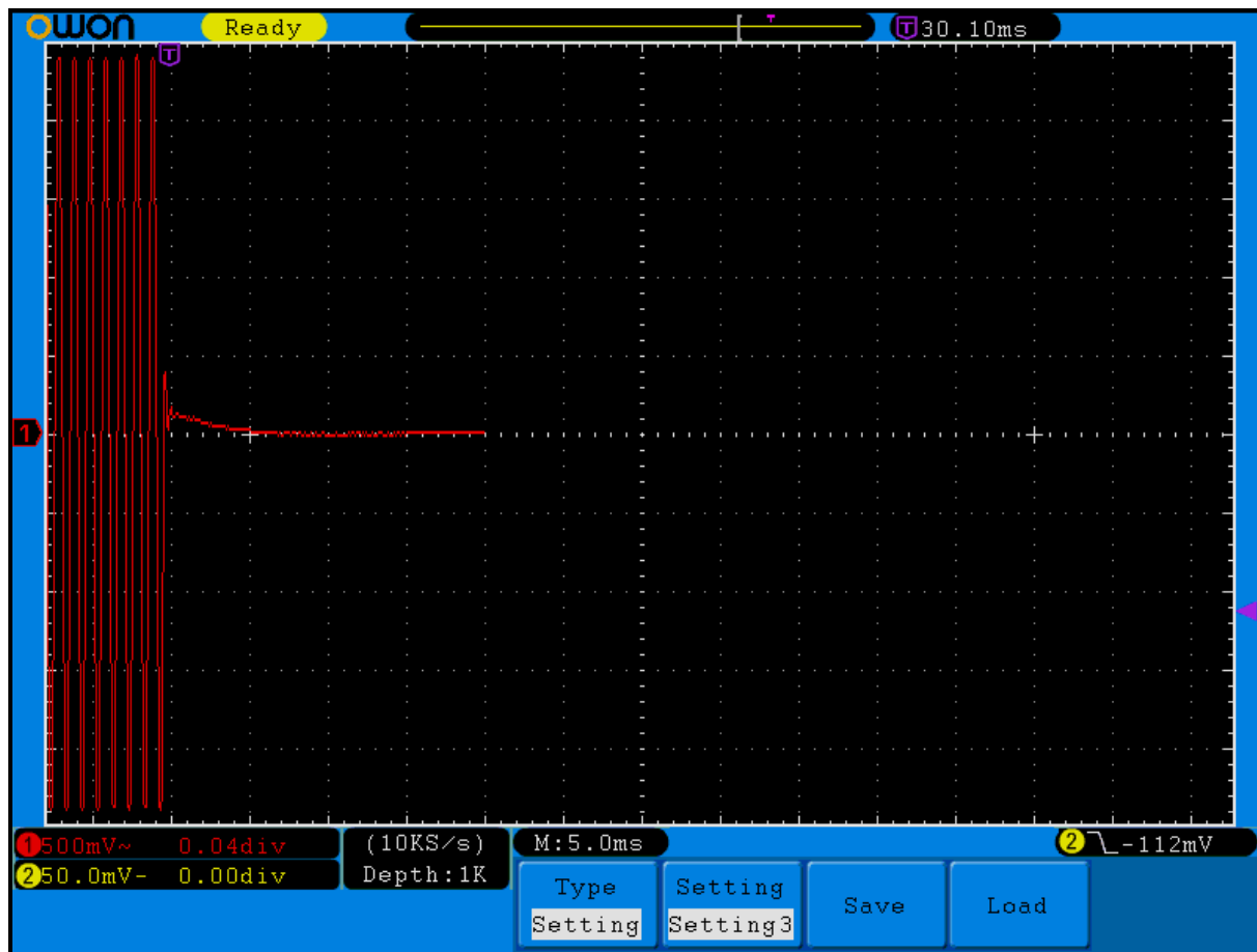
Plot 11-5: Transient Frequency Behavior – 156.8000 MHz; Wide Band; Carrier ON Time
