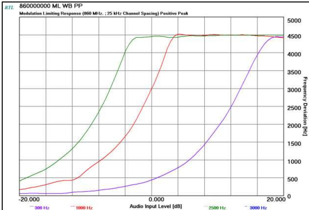
Plot 10-63: Modulation Characteristics – Modulation Limiting - 860 MHz; Positive Peak; WB
