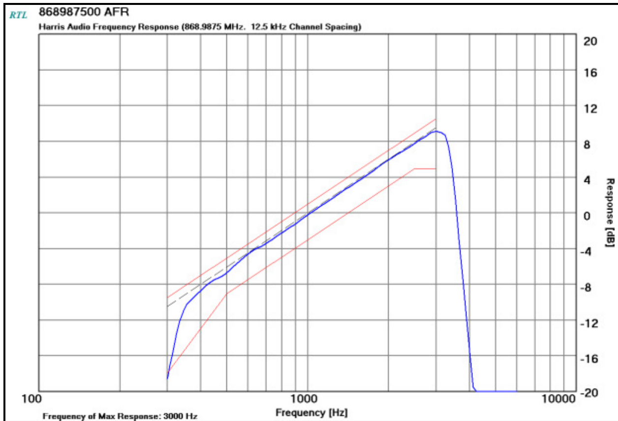
Plot 10-15: Modulation Characteristics - Audio Frequency Response – 868.9875 MHz
