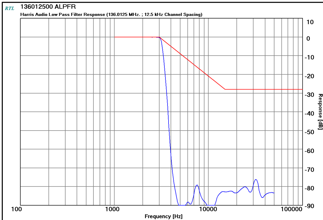
Plot 10-16: Modulation Characteristics – Audio Low Pass Filter – 136.0125 MHz
