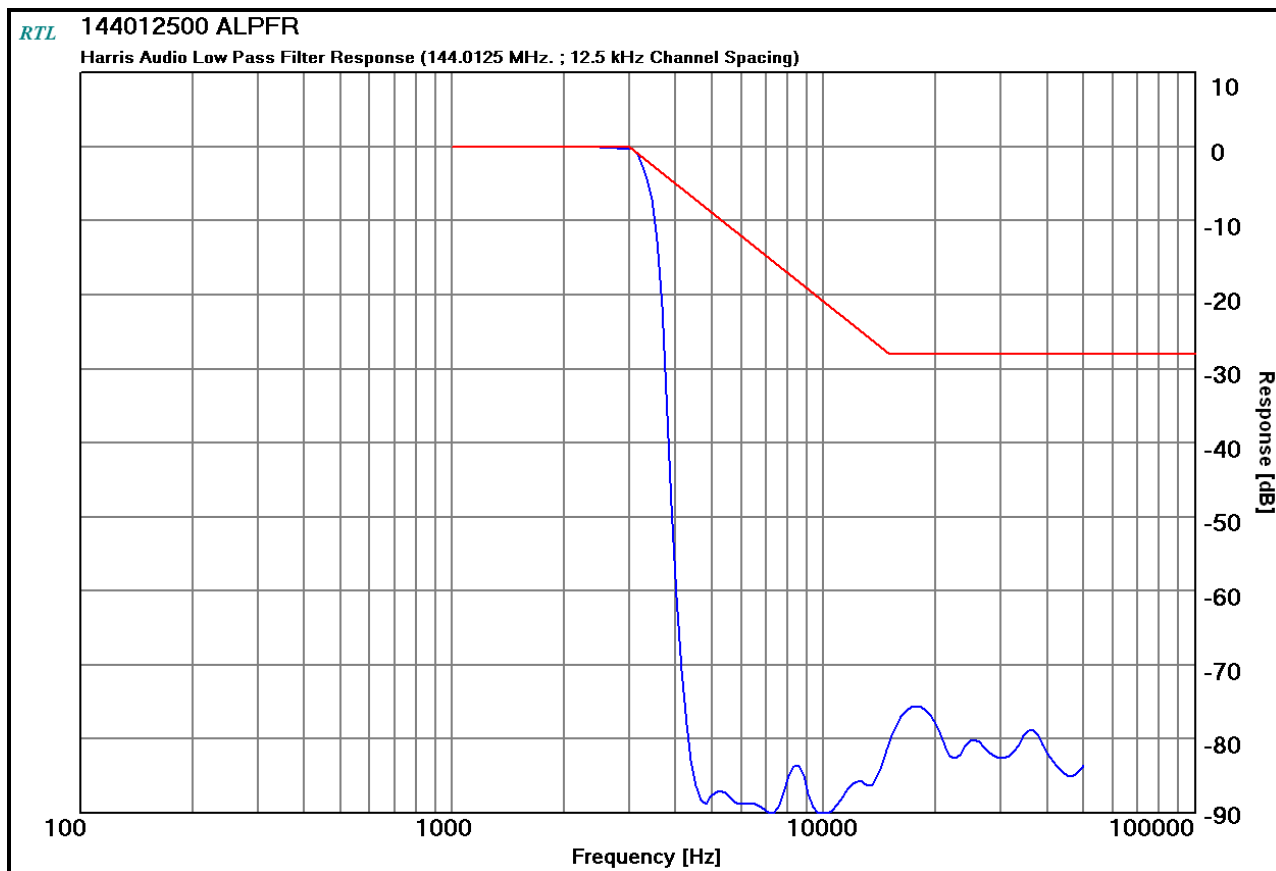
Plot 10-17: Modulation Characteristics – Audio Low Pass Filter – 144.0125 MHz
