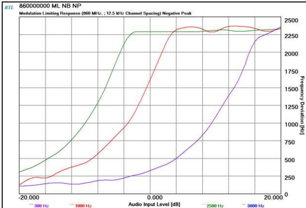
Plot 10-48: Modulation Characteristics – Modulation Limiting - 860 MHz; Negative Peak; NB
