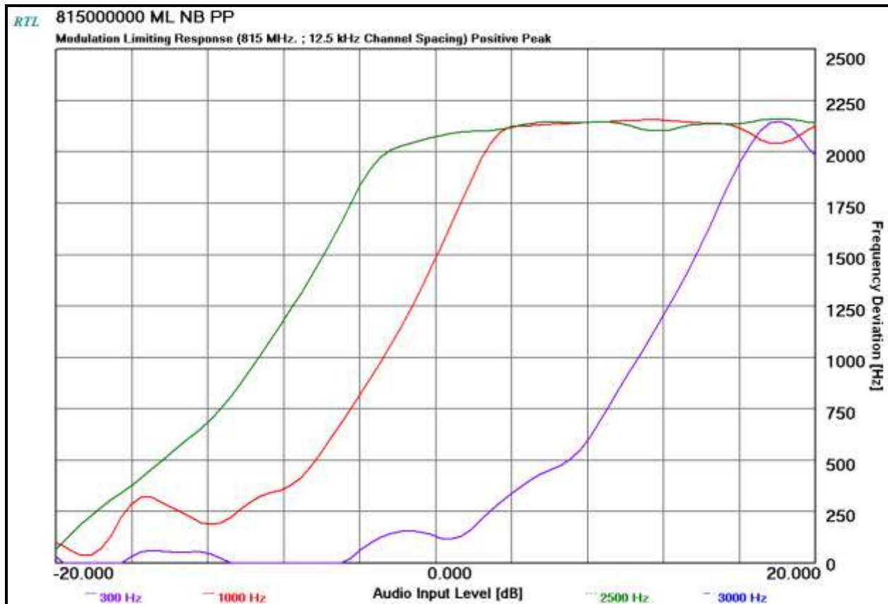
Plot 10-45: Modulation Characteristics – Modulation Limiting – 815 MHz; Positive Peak; NB
