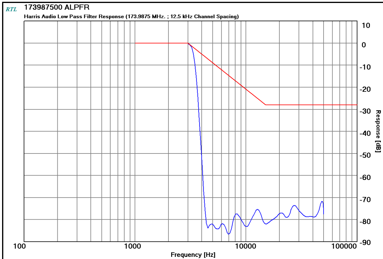
Plot 10-18: Modulation Characteristics – Audio Low Pass Filter – 173.9875 MHz
