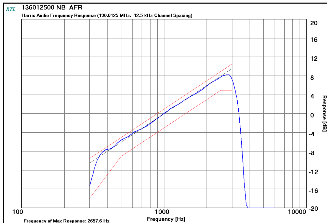
Plot 10-1: Modulation Characteristics - Audio Frequency Response – 136.0125 MHz
