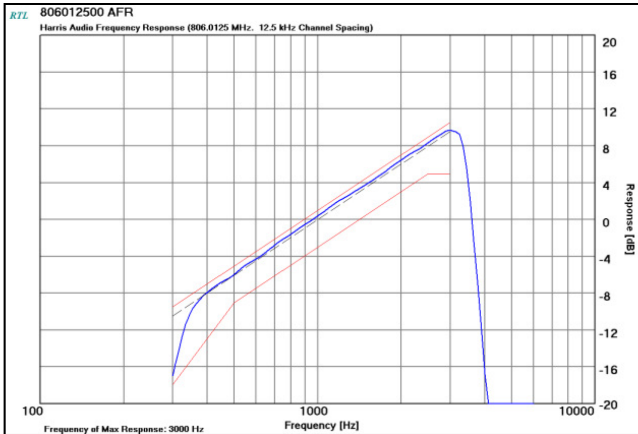
Plot 10-10: Modulation Characteristics - Audio Frequency Response – 806.0125 MHz
