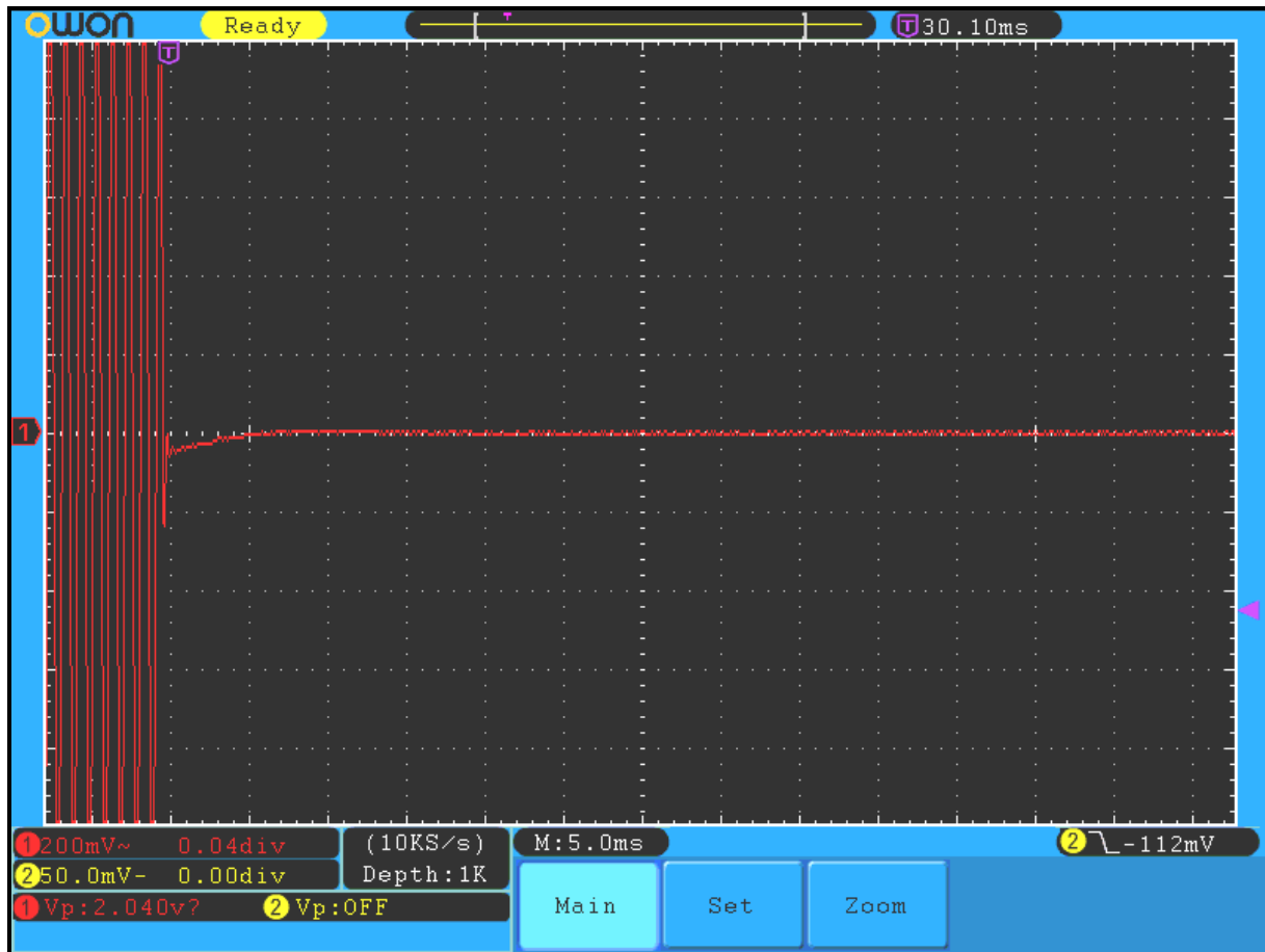
Plot 11-15: Transient Frequency Behavior – 173.9875 MHz; Narrow Band; Carrier ON Time
