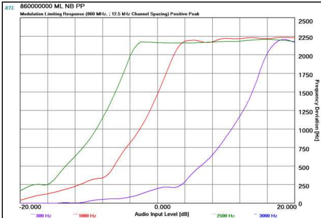
Plot 10-47: Modulation Characteristics – Modulation Limiting - 860 MHz; Positive Peak; NB
