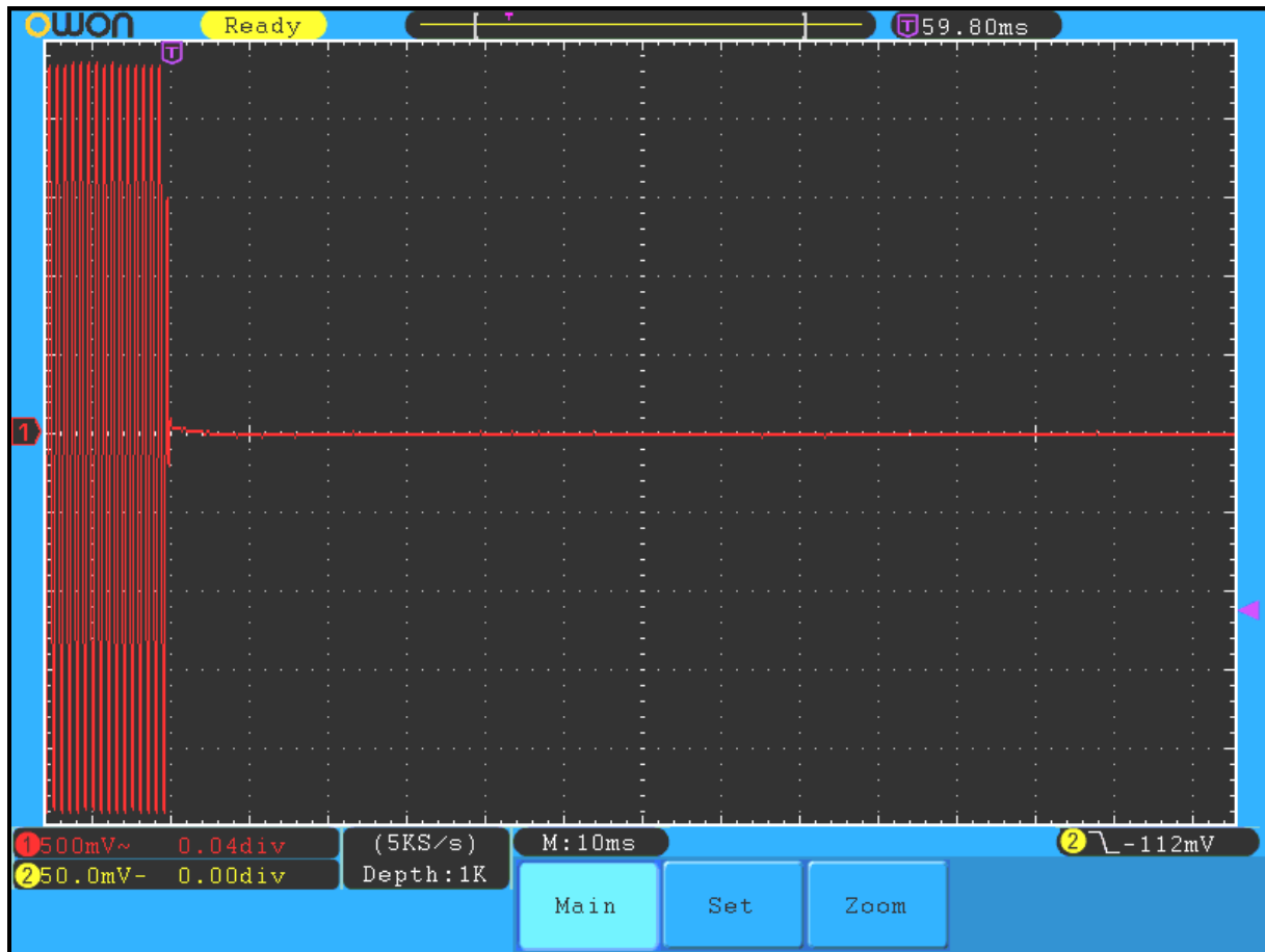
Plot 11-17: Transient Frequency Behavior – 430.0125 MHz; Wide Band; Carrier ON Time
