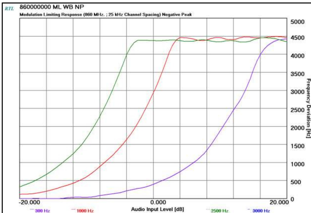
Plot 10-64: Modulation Characteristics – Modulation Limiting - 860 MHz; Negative Peak; WB
