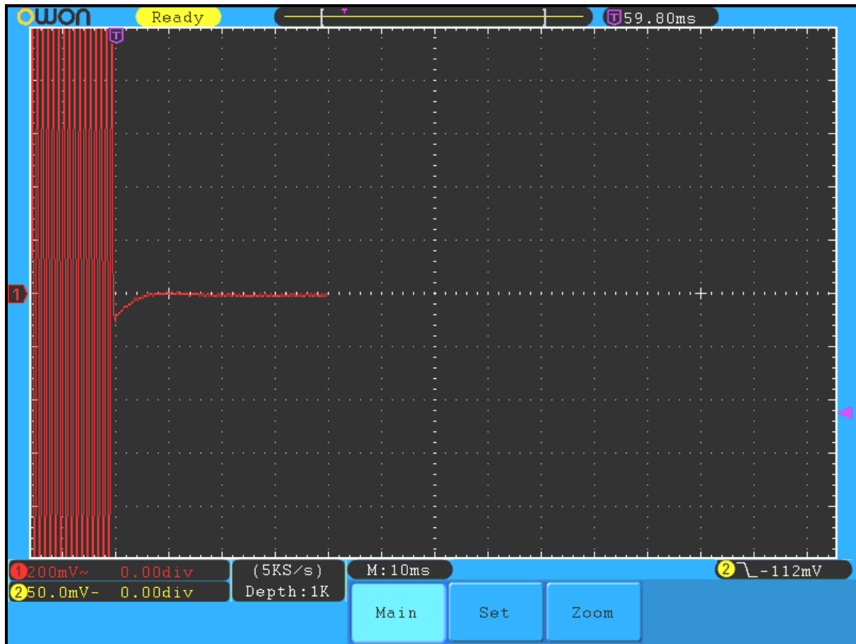
Plot 11-19: Transient Frequency Behavior – 430.0125 MHz; Narrow Band; Carrier ON Time
