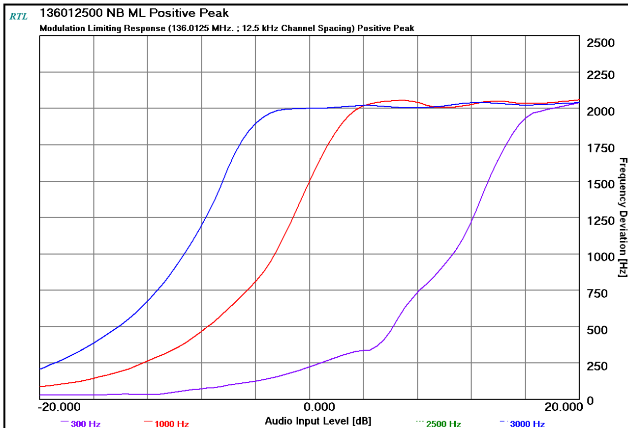
Plot 10-27: Modulation Characteristics – Modulation Limiting – 136.0125 MHz; Positive Peak; NB
