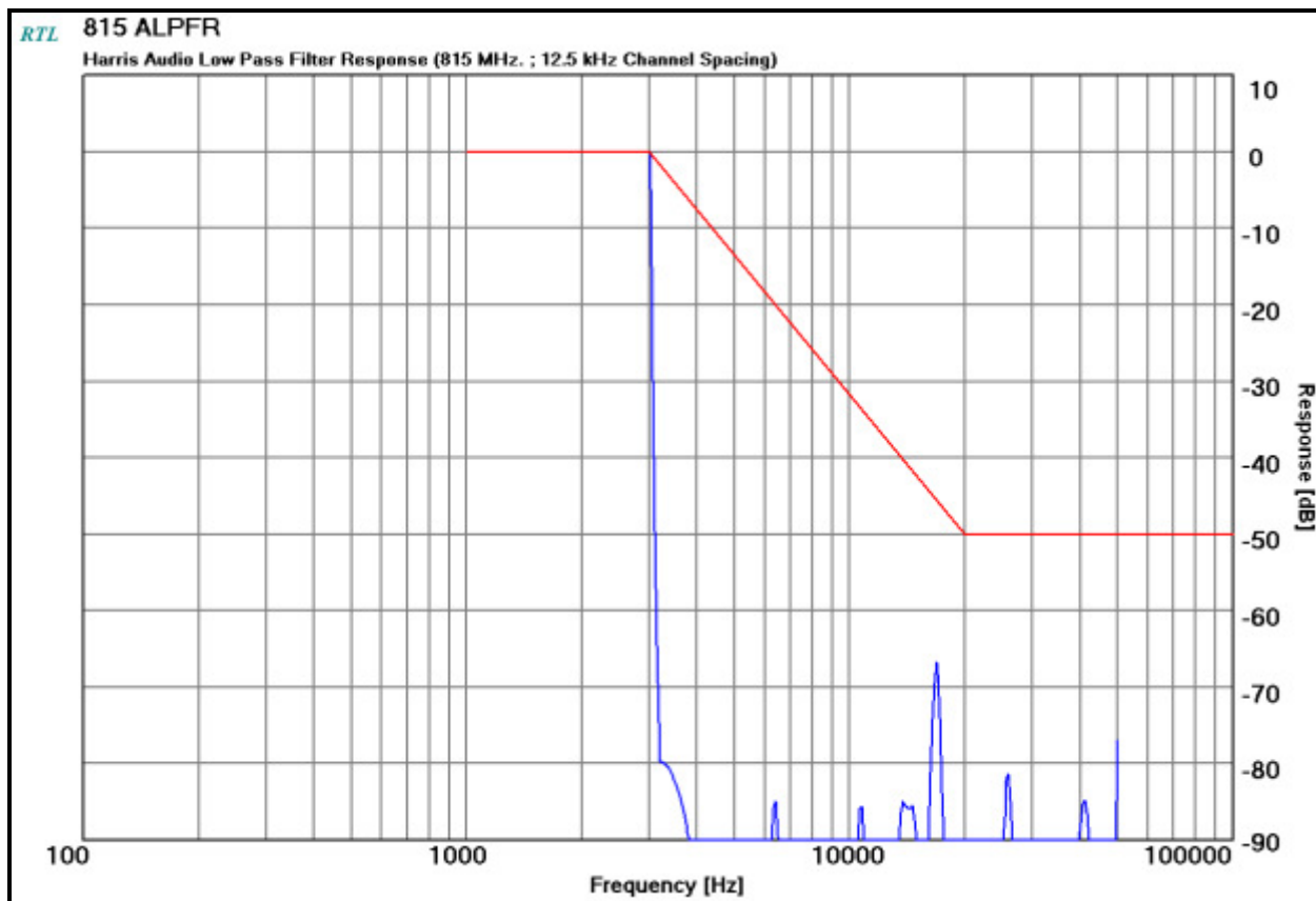
Plot 10-25: Modulation Characteristics – Audio Low Pass Filter – 815.0000 MHz
