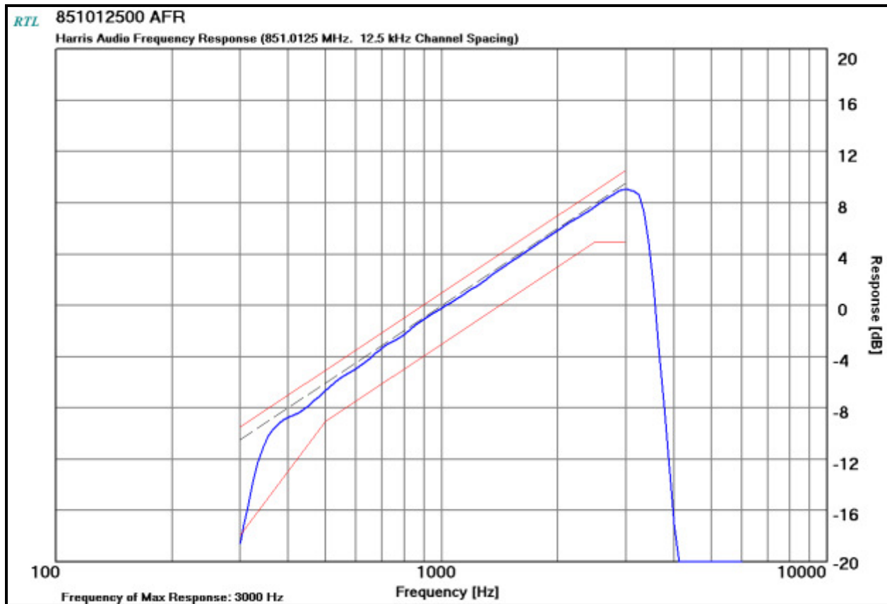
Plot 10-13: Modulation Characteristics - Audio Frequency Response – 851.0125 MHz
