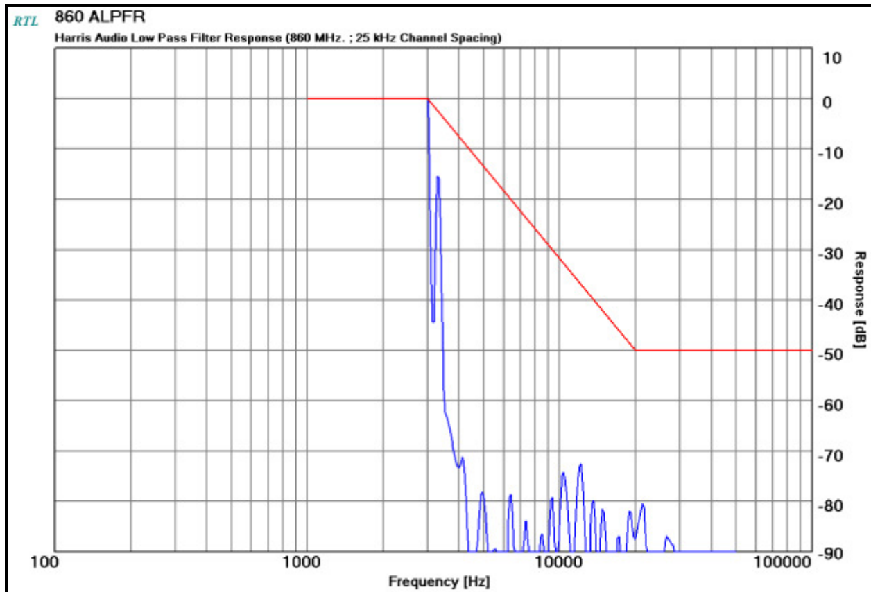
Plot 10-26: Modulation Characteristics – Audio Low Pass Filter – 860.0000 MHz
