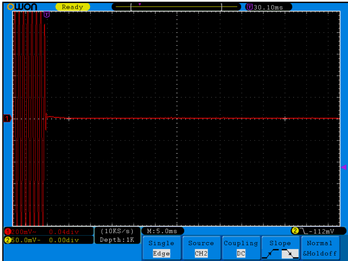
Plot 11-7: Transient Frequency Behavior – 156.8000 MHz; Narrow Band; Carrier ON Time
