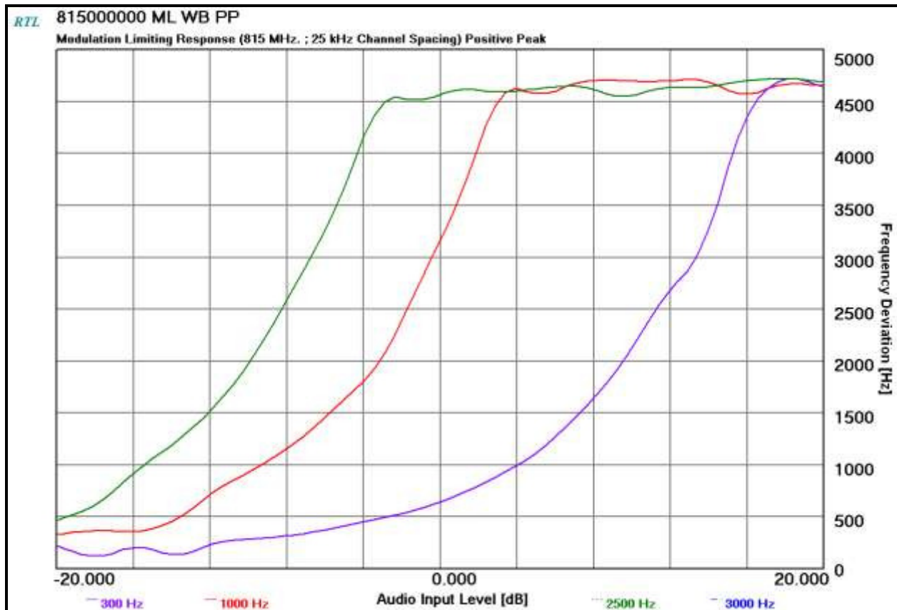
Plot 10-61: Modulation Characteristics – Modulation Limiting – 815 MHz; Positive Peak; WB
