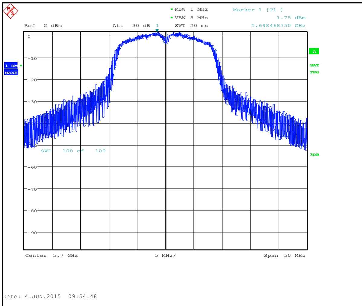
Plot 4-100: Peak Power Spectral Density: Channel 140 (5700 MHz) 802.11a 54 Mbps
