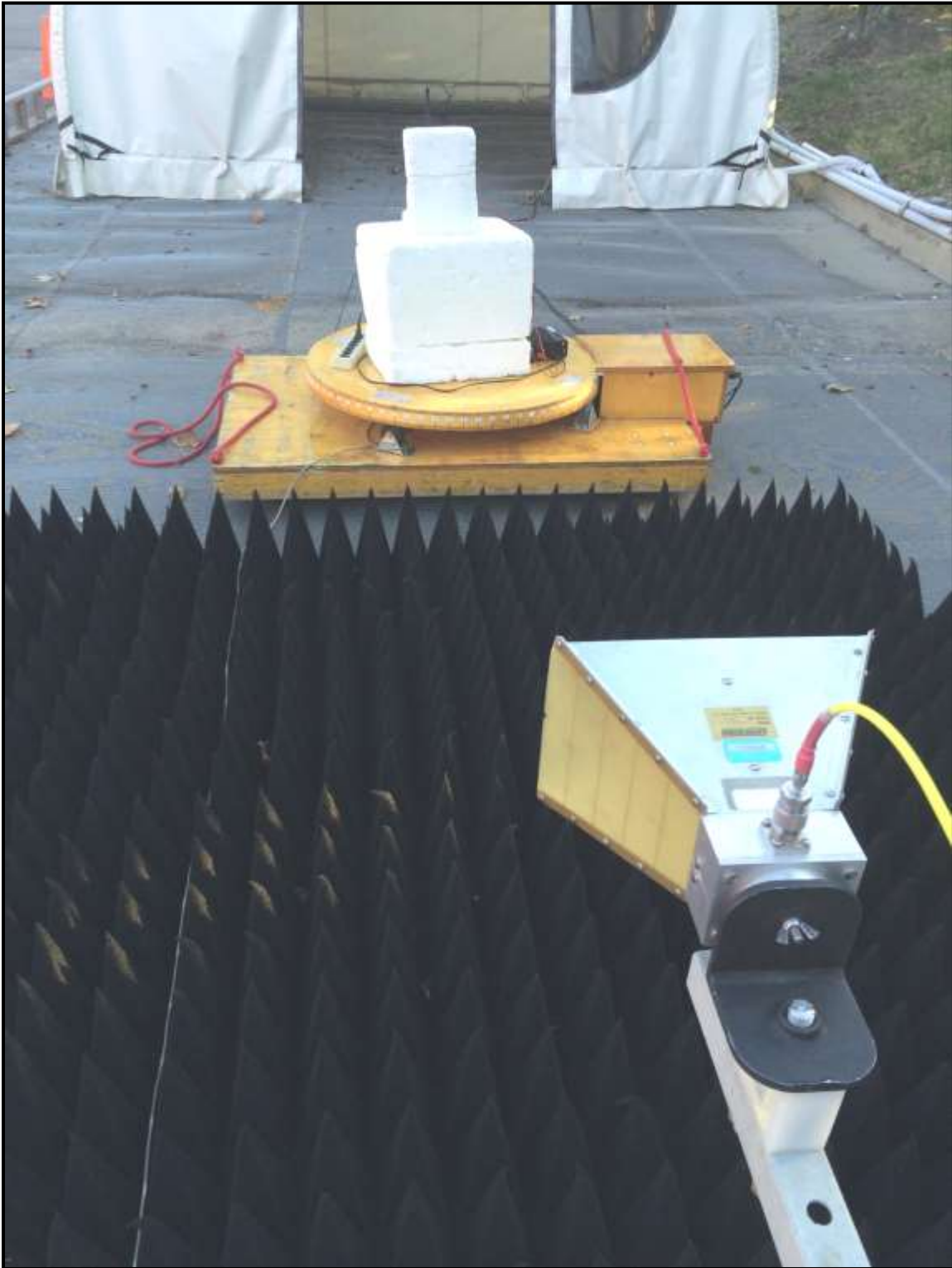
Photograph 2: Radiated Emissions – Back View
