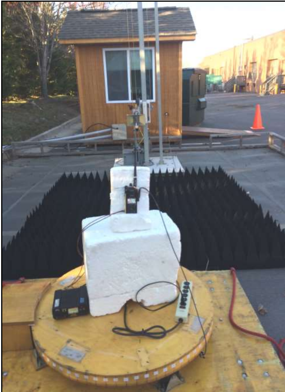
Photograph 1: Radiated Emissions – Front View
