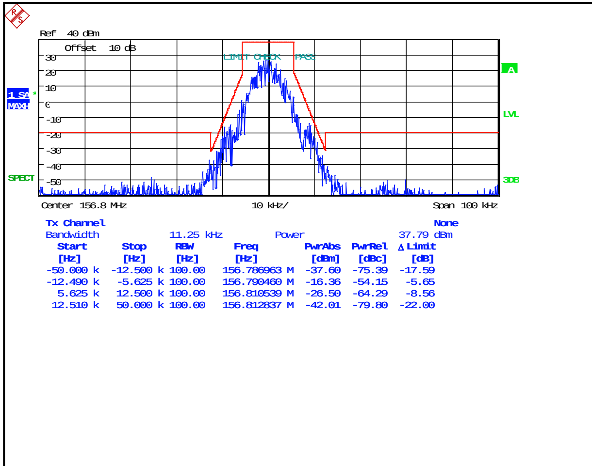
Plot 8-26: Occupied Bandwidth – 156.8 MHz; 2-Level FSK 9600; NB EDACS; (Mask D)
