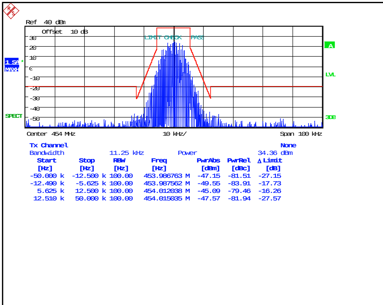
Plot 8-52: Occupied Bandwidth – 454 MHz; CPM TDMA; Mask D
