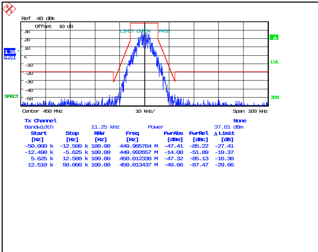
Plot 8-44: Occupied Bandwidth – 450 MHz; P25; Mask D
