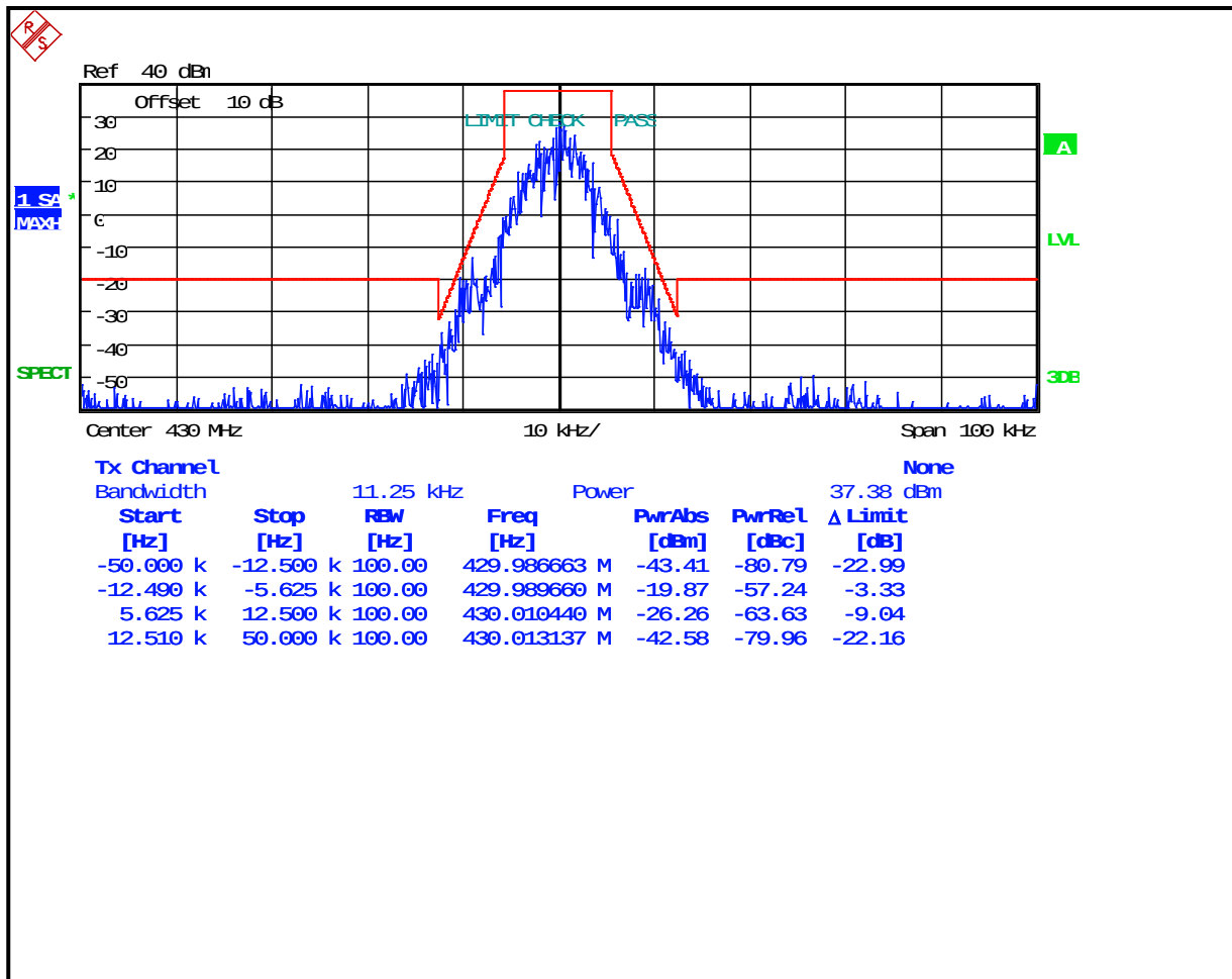
Plot 8-57: Occupied Bandwidth – 430 MHz; (2-level FSK 9600; NB) EDACS; Mask D
