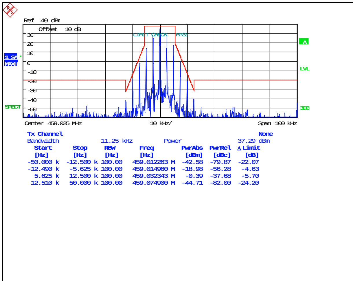
Plot 8-40: Occupied Bandwidth – 459.025 MHz; Narrowband Analog; Mask D
