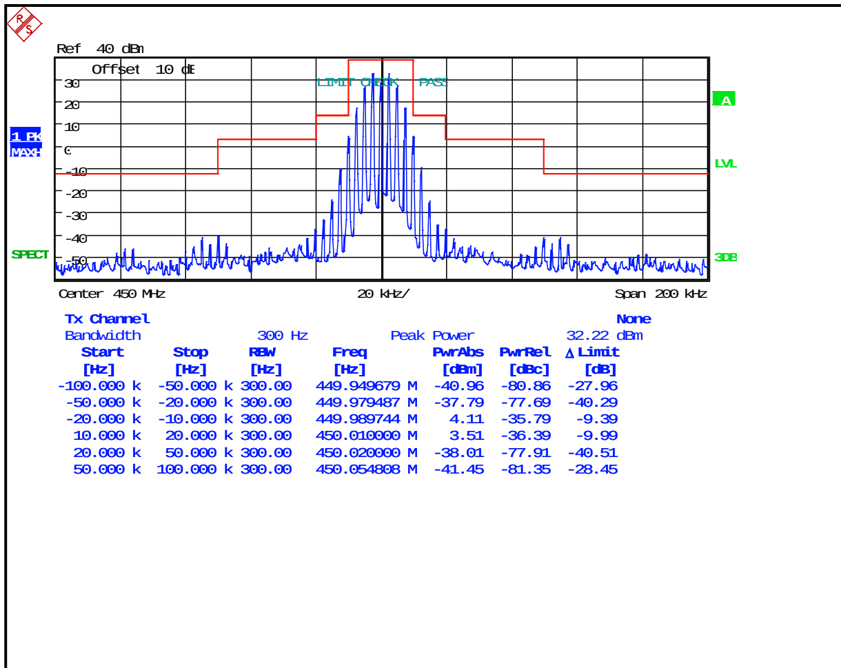
Plot 8-30: Occupied Bandwidth – 450 MHz; Wideband Analog; Mask B
