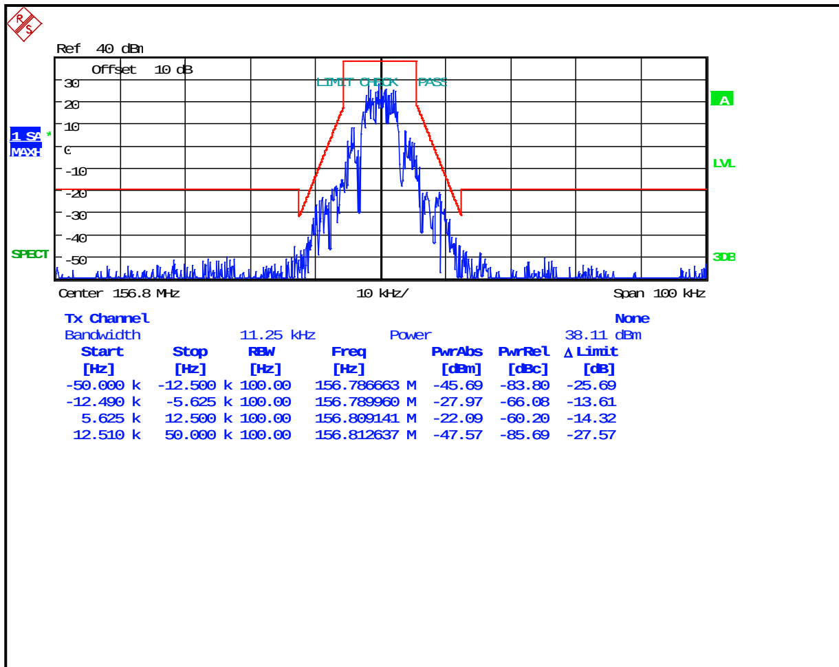
Plot 8-18: Occupied Bandwidth – 156.8 MHz; 2-Level FSK 4800; XNB EDACS; (Mask D)
