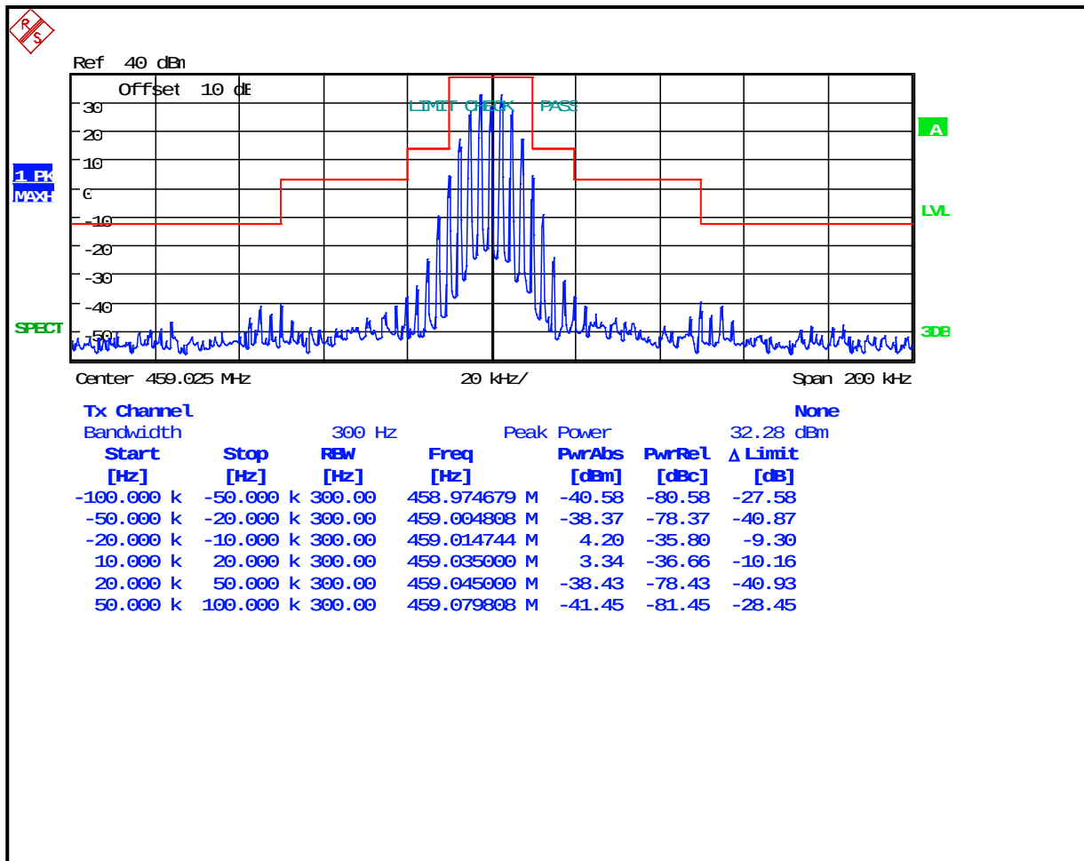
Plot 8-33: Occupied Bandwidth – 459.025 MHz; Wideband Analog; Mask B
