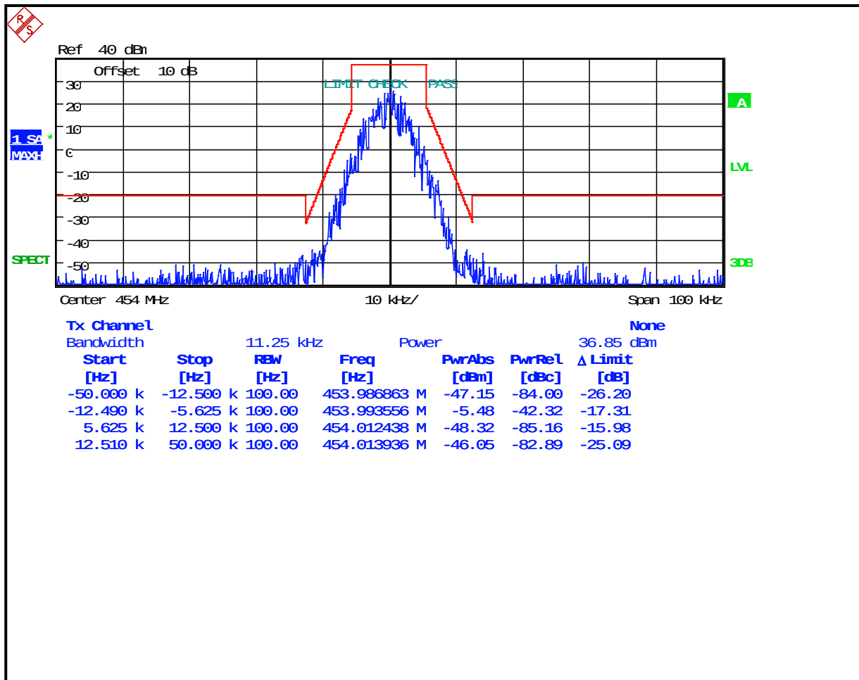
Plot 8-73: Occupied Bandwidth – 454 MHz; (4-level FSK Data/Voice; NB) OpenSky; Mask D
