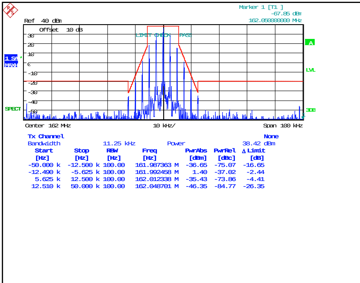
Plot 8-7: Occupied Bandwidth – 162 MHz; Analog NB (Mask D)
