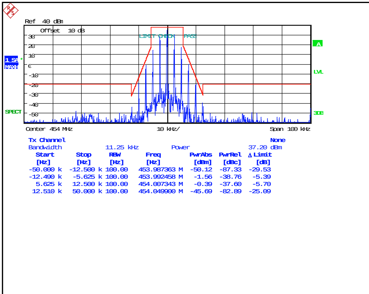
Plot 8-38: Occupied Bandwidth – 454 MHz; Narrowband Analog; Mask D
