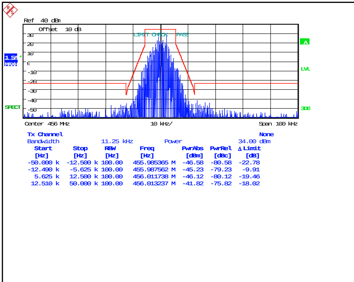
Plot 8-53: Occupied Bandwidth – 456MHz; CPM TDMA; Mask D
