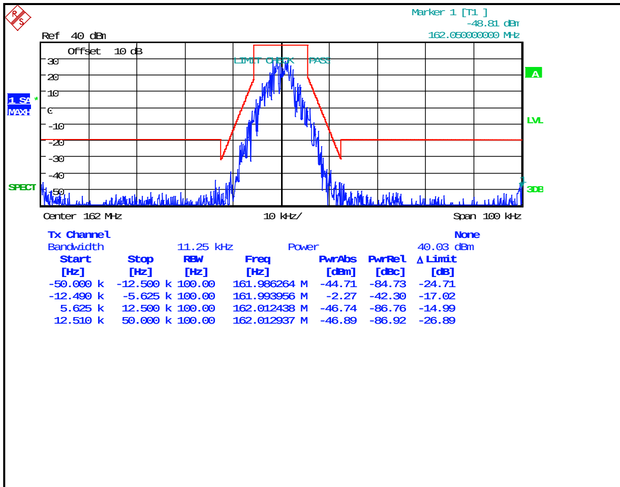
Plot 8-15: Occupied Bandwidth – 162 MHz; CPM TDMA TDMA; (Mask D)
