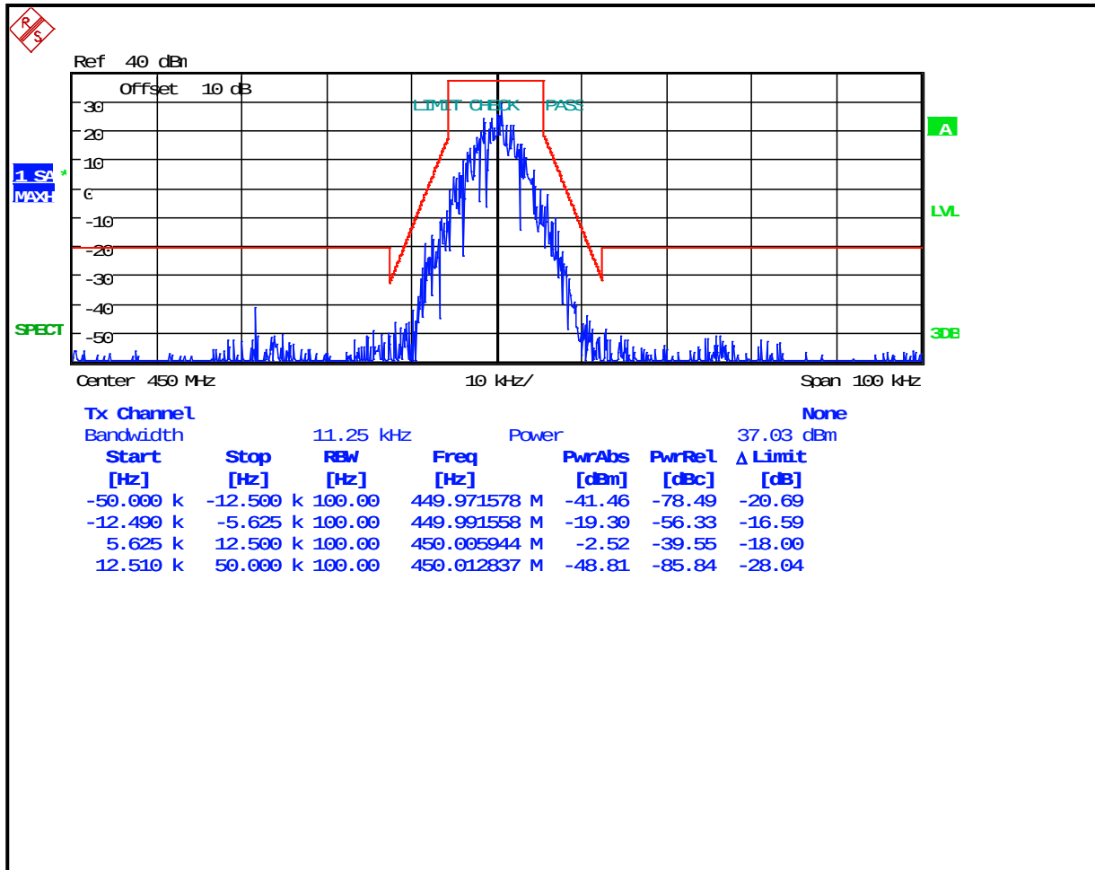
Plot 8-72: Occupied Bandwidth – 450 MHz; (4-level FSK Data/Voice; NB) OpenSky; Mask D
