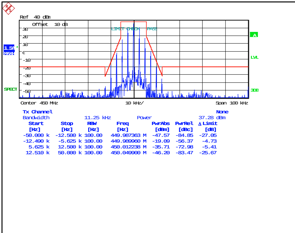
Plot 8-37: Occupied Bandwidth – 450 MHz; Narrowband Analog; Mask D
