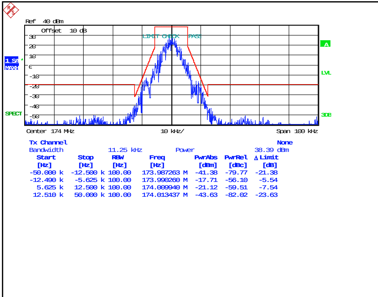
Plot 8-28: Occupied Bandwidth – 174 MHz; 2-Level FSK 9600; NB EDACS; (Mask D)
