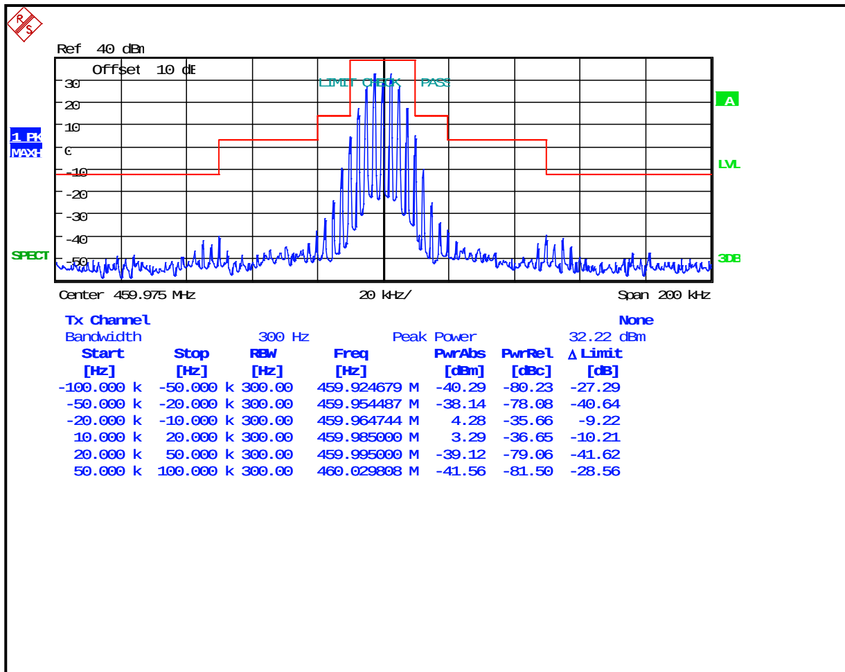
Plot 8-34: Occupied Bandwidth – 459.975MHz; Wideband Analog; Mask B
