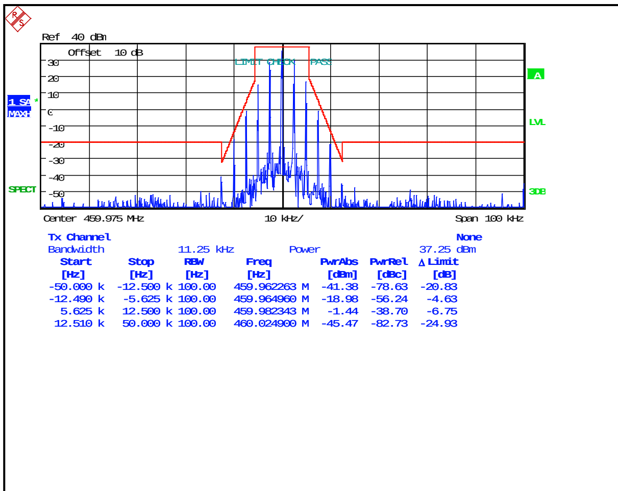
Plot 8-41: Occupied Bandwidth – 459.975 MHz; Narrowband Analog; Mask D
