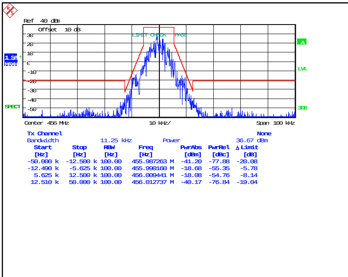
Plot 8-60: Occupied Bandwidth – 456 MHz; (2-level FSK 9600; NB) EDACS; Mask D
