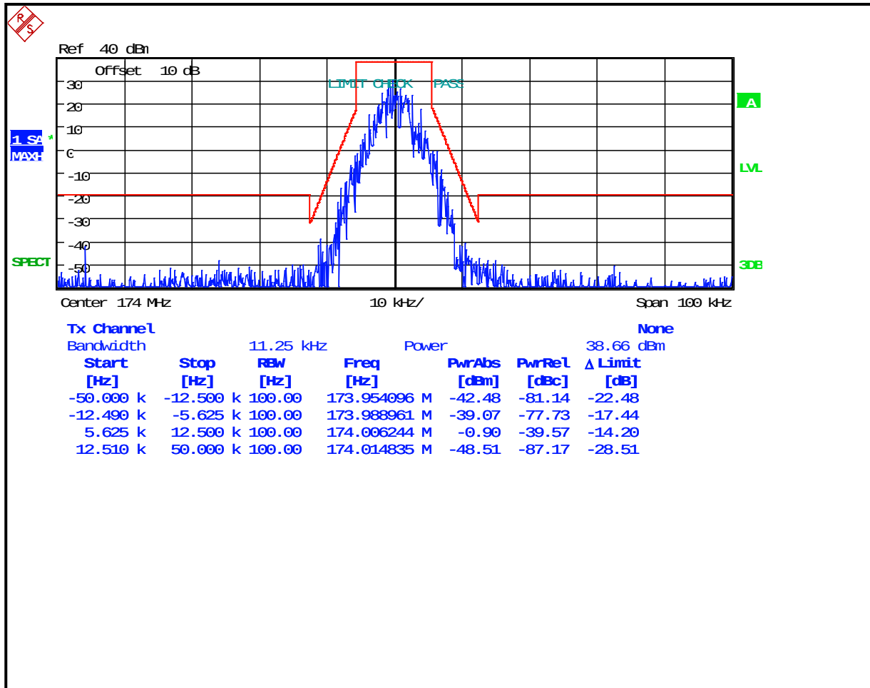
Plot 8-12: Occupied Bandwidth – 174 MHz; P25; (Mask D)
