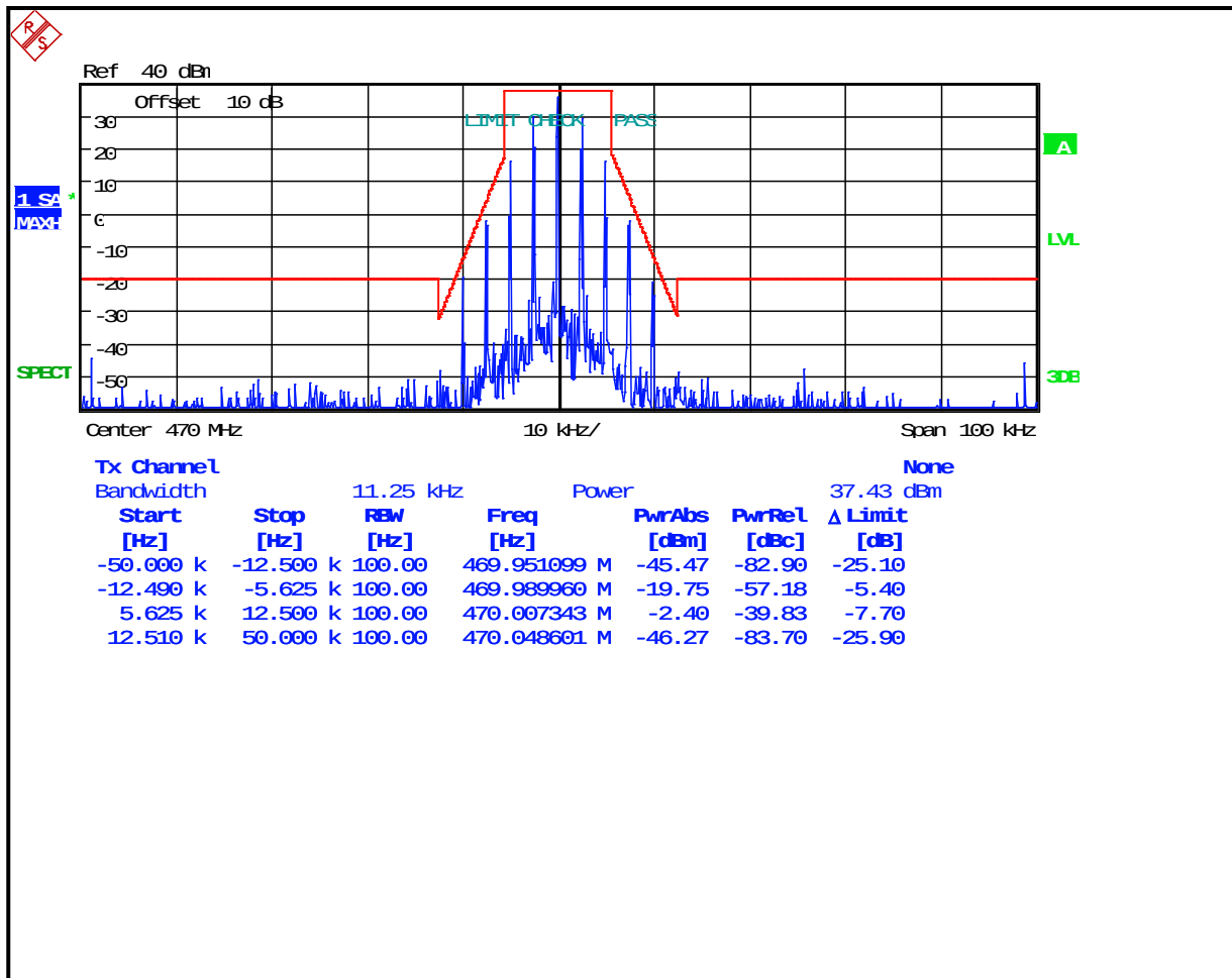
Plot 8-42: Occupied Bandwidth – 470 MHz; Narrowband Analog; Mask D
