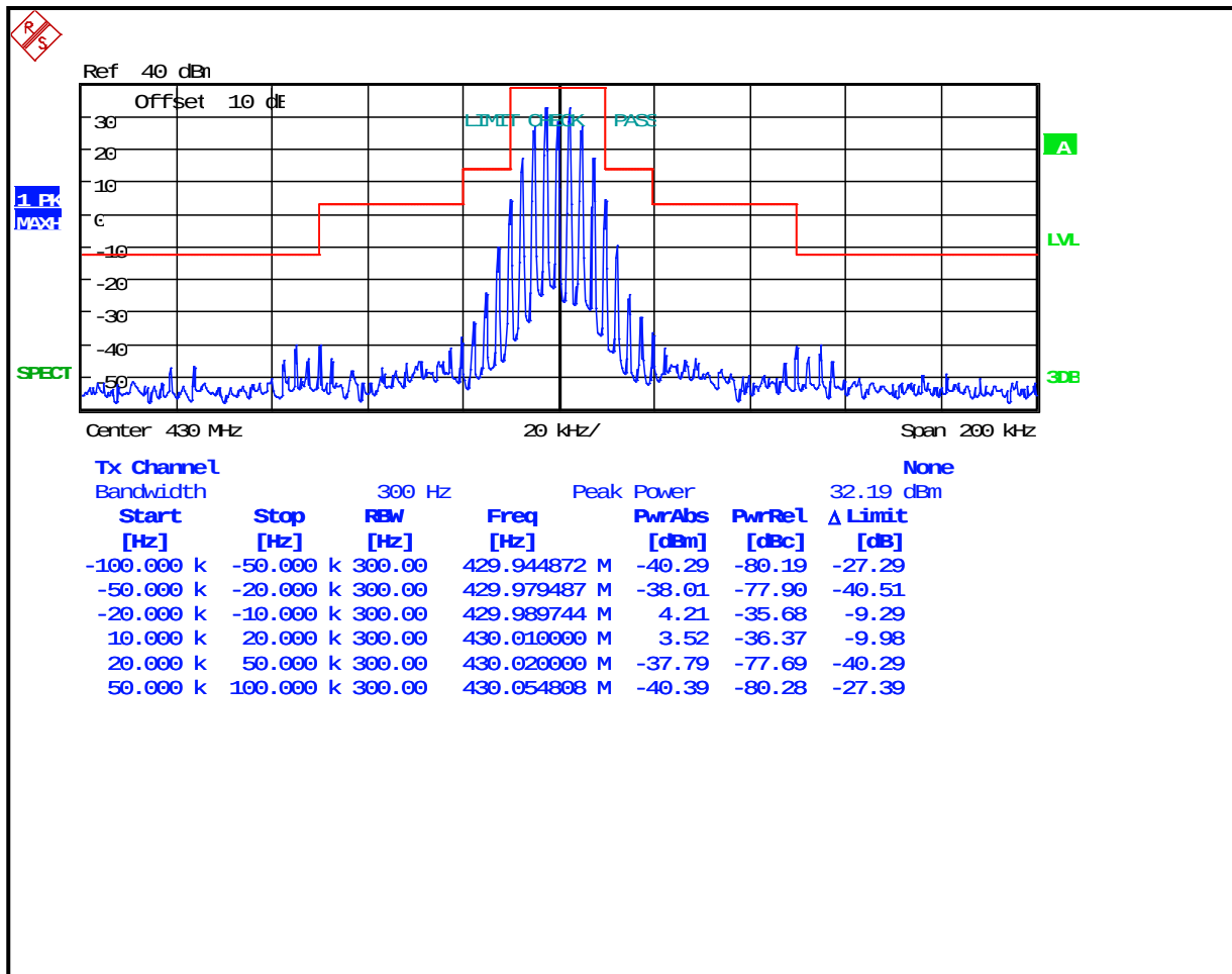
Plot 8-29: Occupied Bandwidth – 430 MHz; Wideband Analog; Mask B
