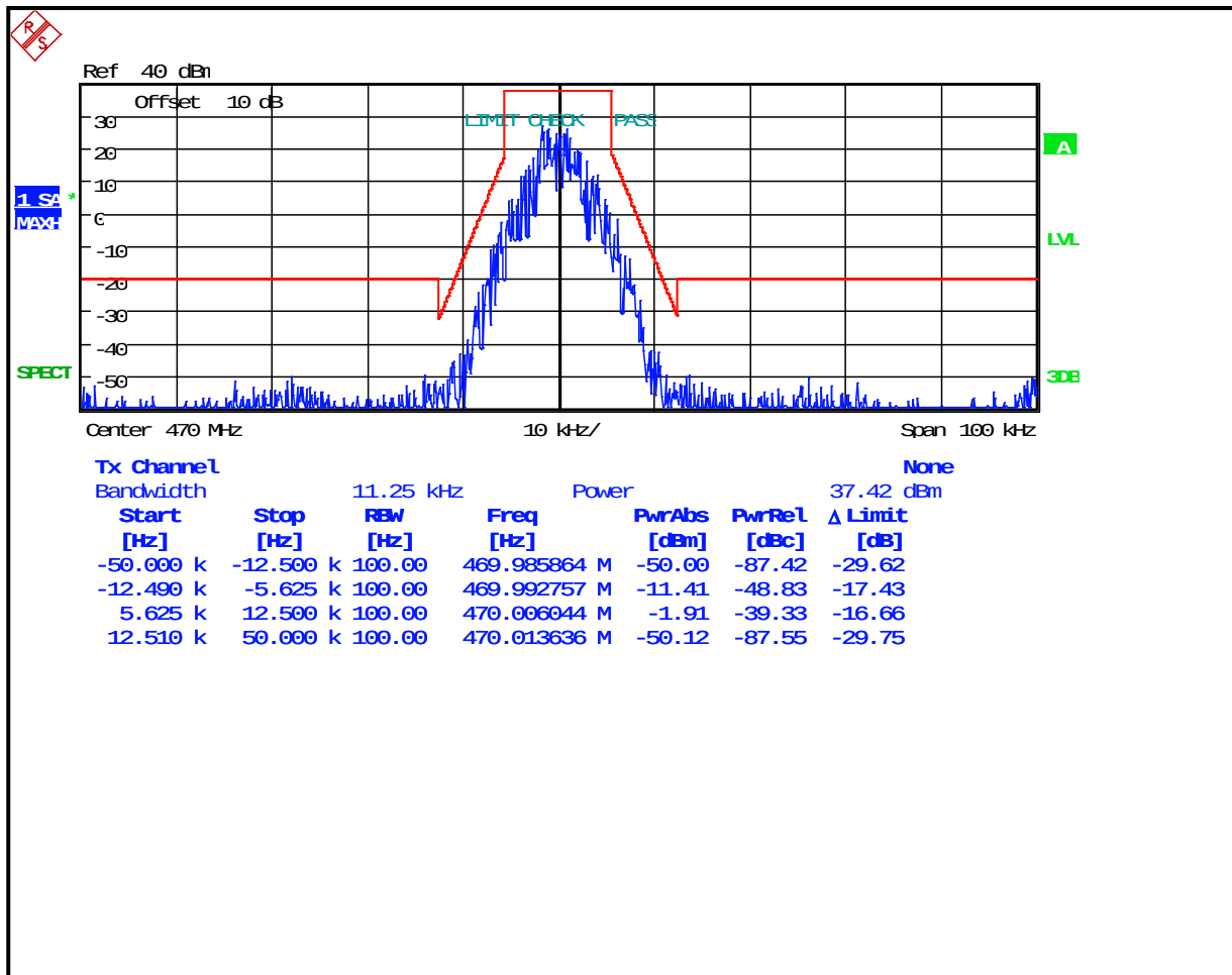
Plot 8-49: Occupied Bandwidth – 470 MHz; P25; Mask D
