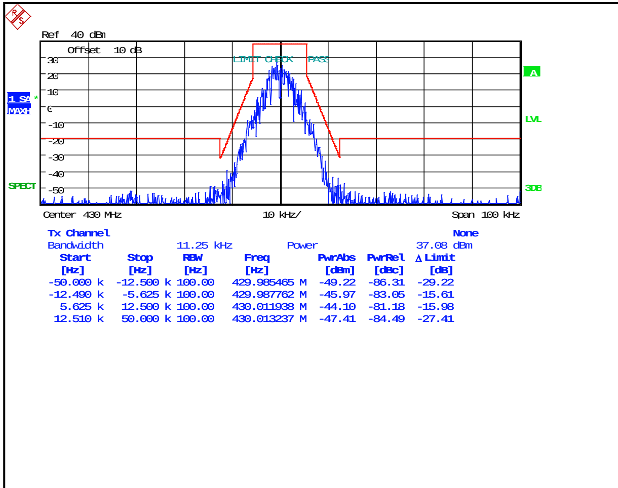
Plot 8-71: Occupied Bandwidth – 430 MHz; (4-level FSK Data/Voice; NB) OpenSky; Mask D
