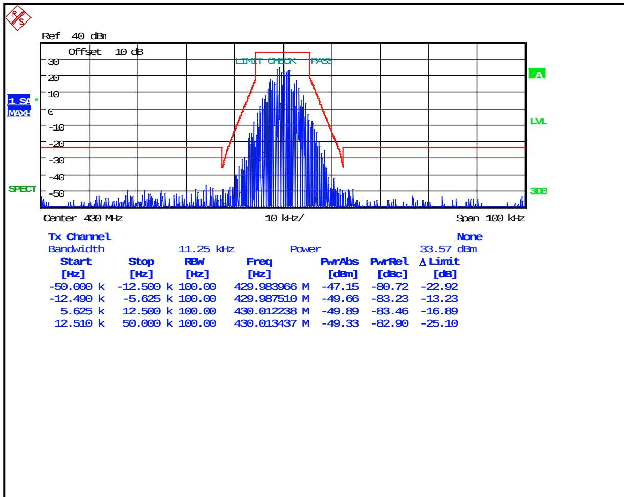
Plot 8-50: Occupied Bandwidth – 430 MHz; CPM TDMA; Mask D
