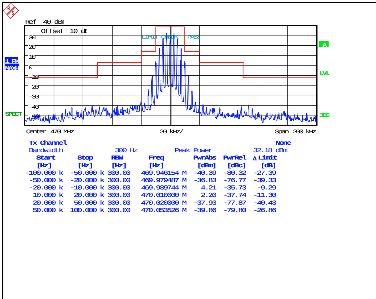
Plot 8-35: Occupied Bandwidth – 470 MHz; Wideband Analog; Mask B
