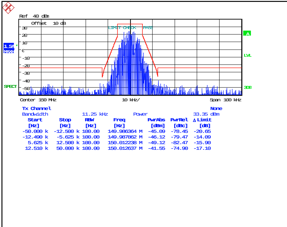
Plot 8-13: Occupied Bandwidth – 150 MHz; CPM TDMA TDMA; (Mask D)
