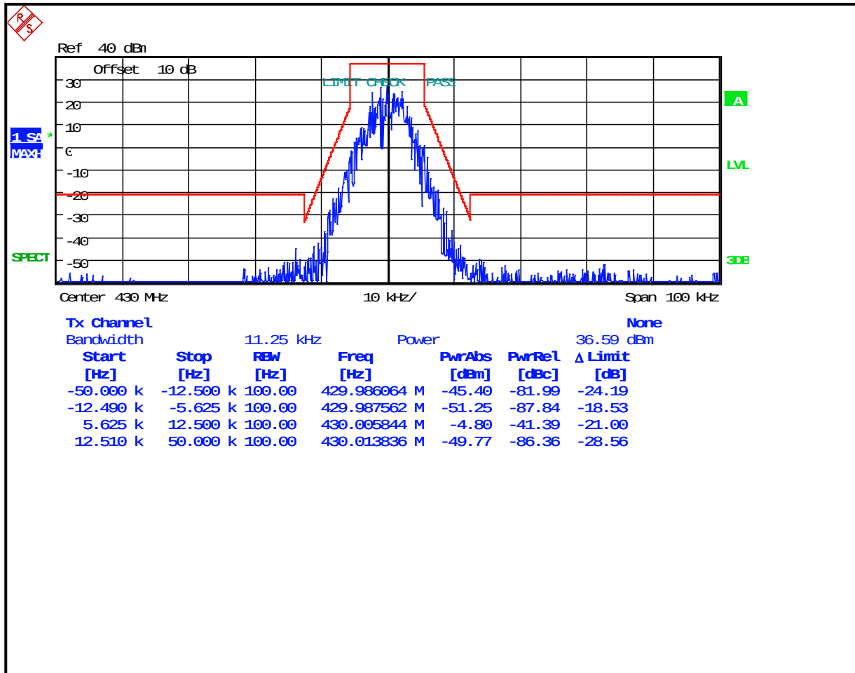
Plot 8-43: Occupied Bandwidth – 430 MHz; P25; Mask D
