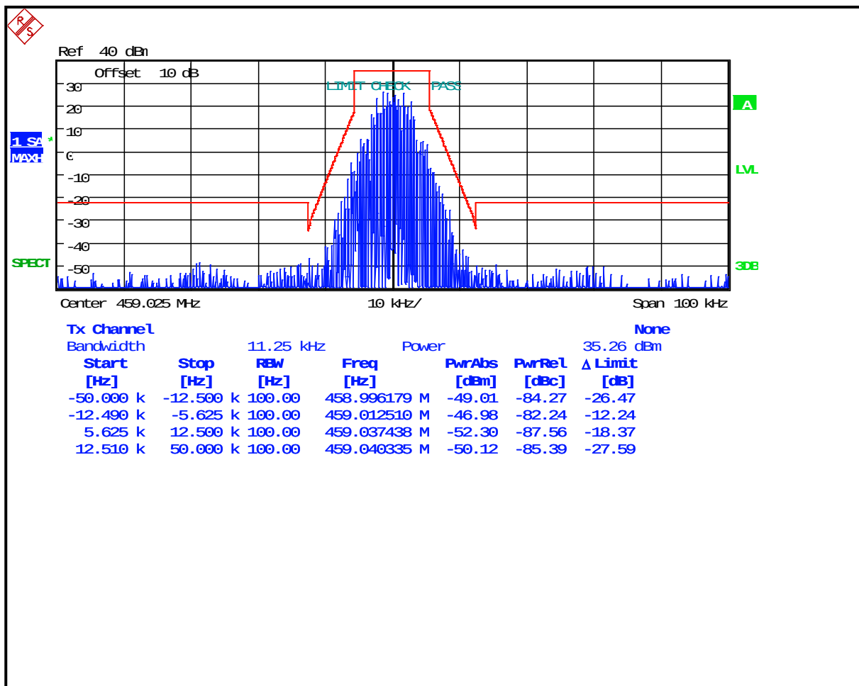
Plot 8-54: Occupied Bandwidth – 459.025 MHz; CPM TDMA; Mask D
