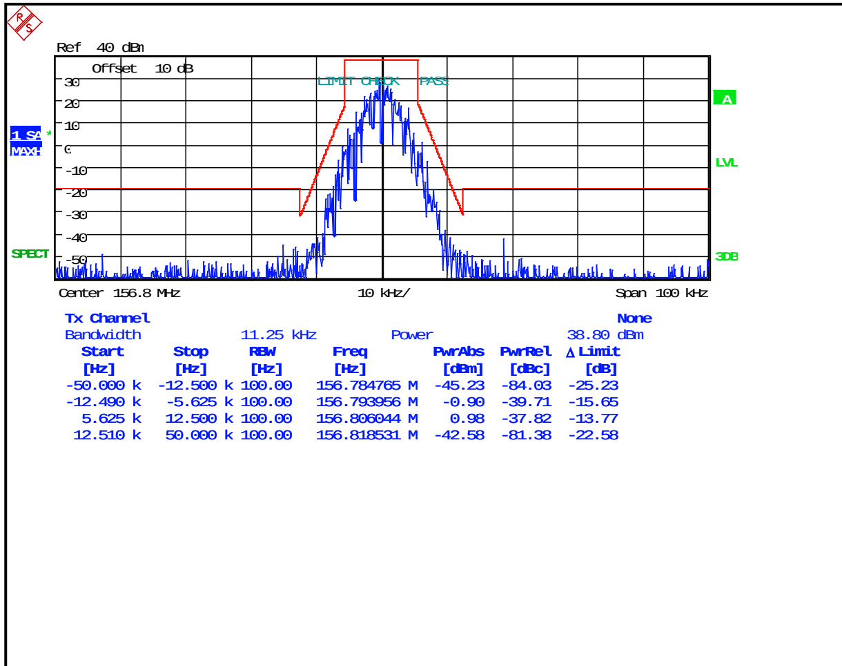
Plot 8-10: Occupied Bandwidth – 156.8 MHz; P25; (Mask D)
