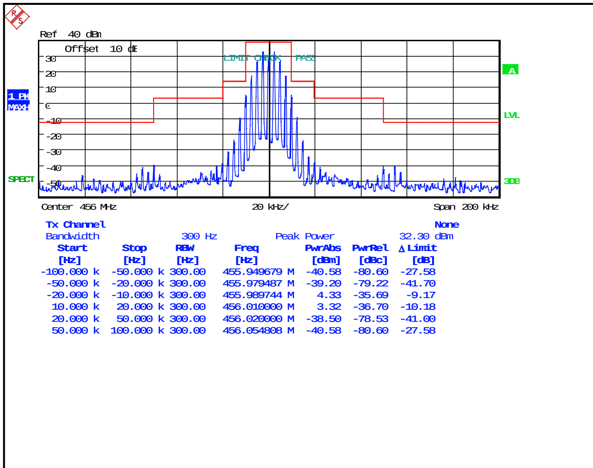
Plot 8-32: Occupied Bandwidth – 456 MHz; Wideband Analog; Mask B
