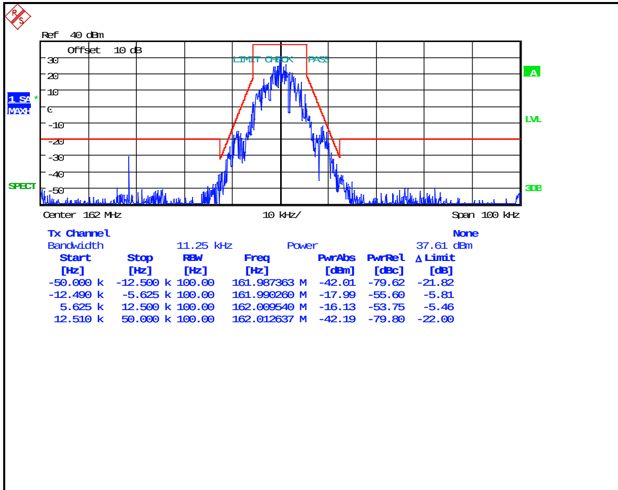
Plot 8-27: Occupied Bandwidth – 162 MHz; 2-Level FSK 49600; NB EDACS; (Mask D)
