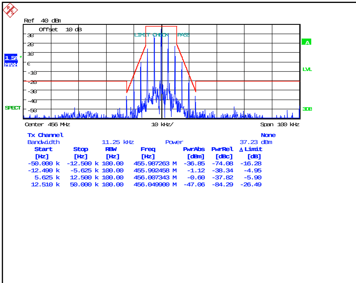
Plot 8-39: Occupied Bandwidth – 456 MHz; Narrowband Analog; Mask D
