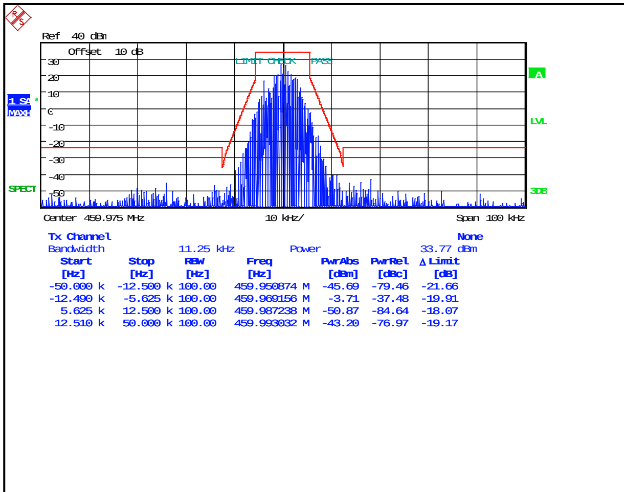
Plot 8-55: Occupied Bandwidth – 459.975 MHz; CPM TDMA; Mask D
