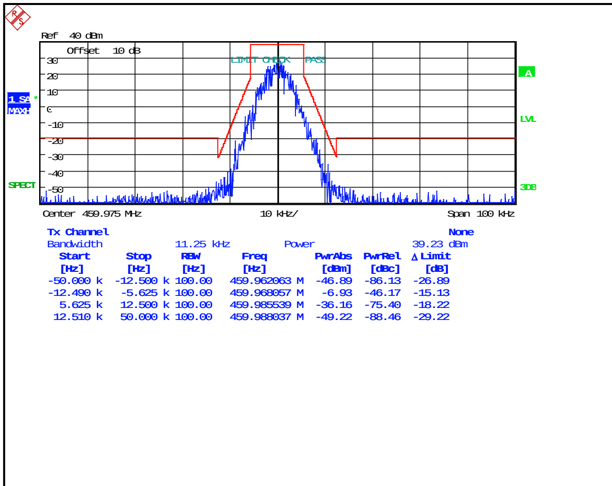
Plot 8-48: Occupied Bandwidth – 459.975 MHz; P25; Mask D
