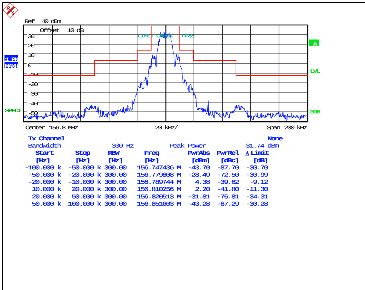
Plot 8-22: Occupied Bandwidth – 156.8 MHz; 2-Level FSK 9600; WB EDACS; (Mask B)
