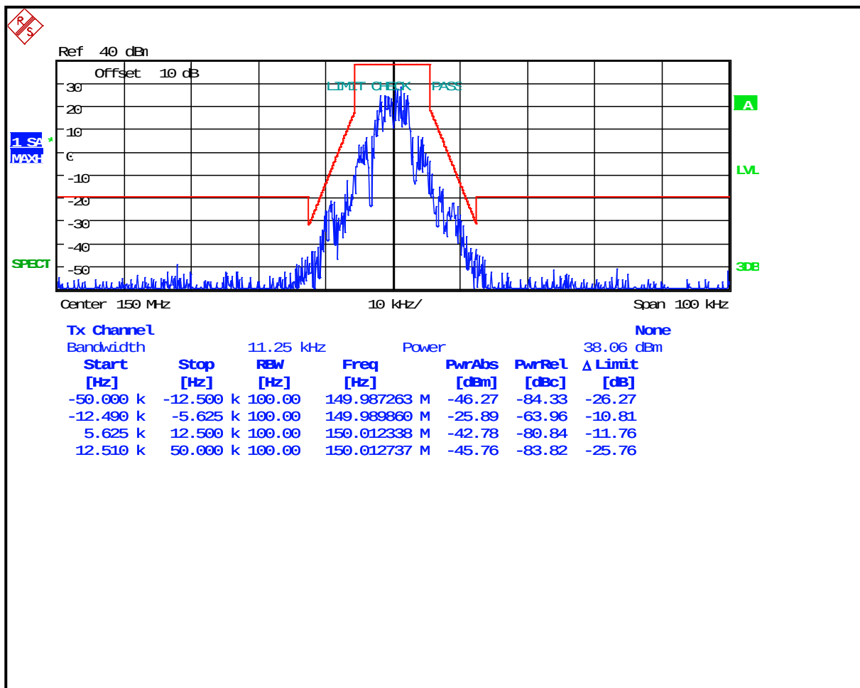
Plot 8-17: Occupied Bandwidth – 150 MHz; 2-Level FSK 4800; XNB EDACS; (Mask D)
