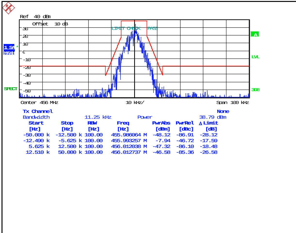
Plot 8-74: Occupied Bandwidth – 456 MHz; (4-level FSK Data/Voice; NB) OpenSky; Mask D
