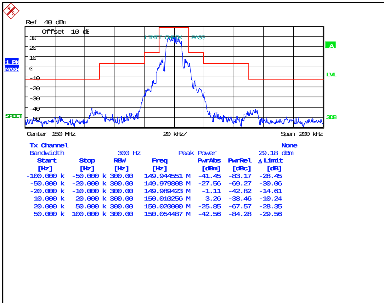
Plot 8-21: Occupied Bandwidth – 150 MHz; 2-Level FSK 9600; WB EDACS; (Mask B)
