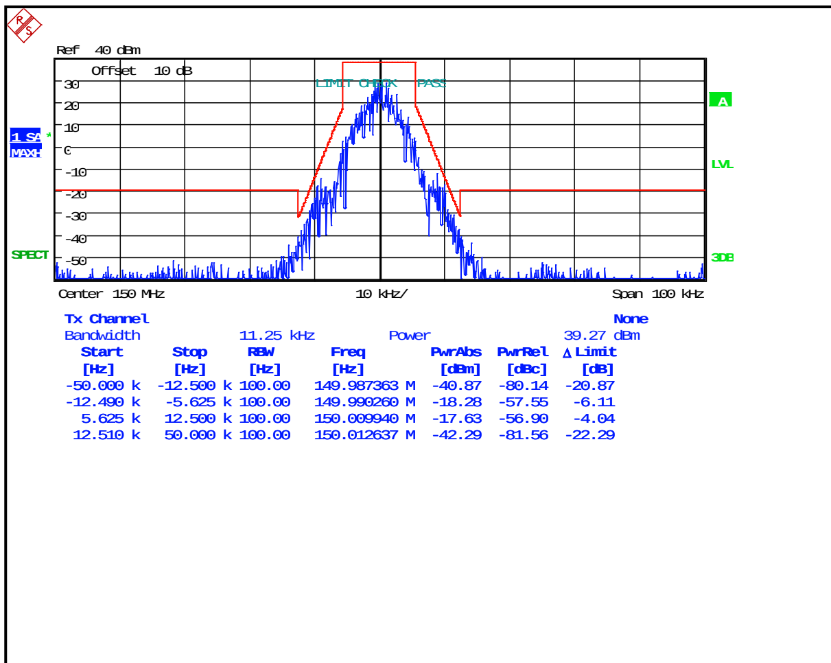
Plot 8-25: Occupied Bandwidth – 150 MHz; 2-Level FSK 9600; NB EDACS; (Mask D)
