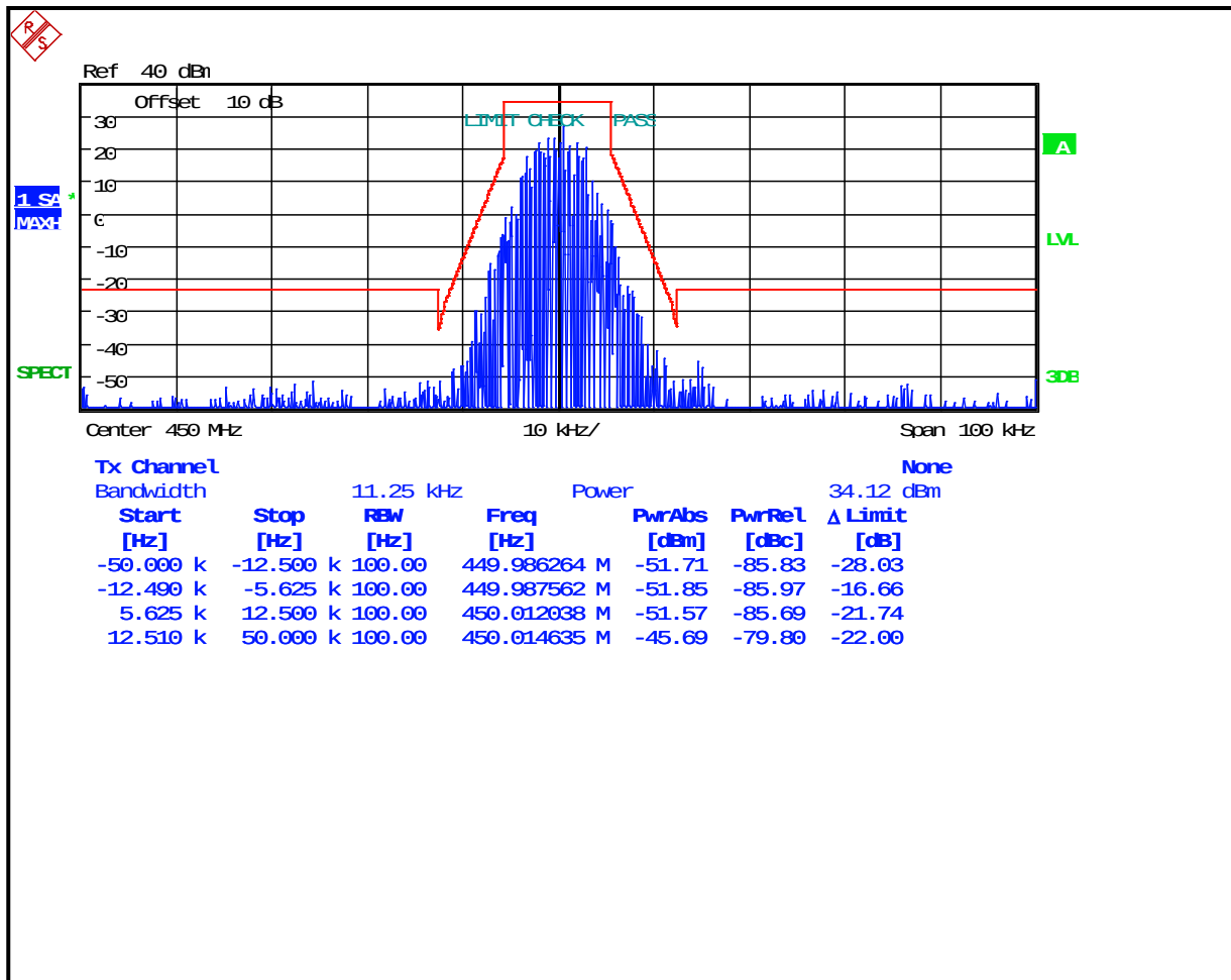
Plot 8-51: Occupied Bandwidth – 450 MHz; CPM TDMA; Mask D
