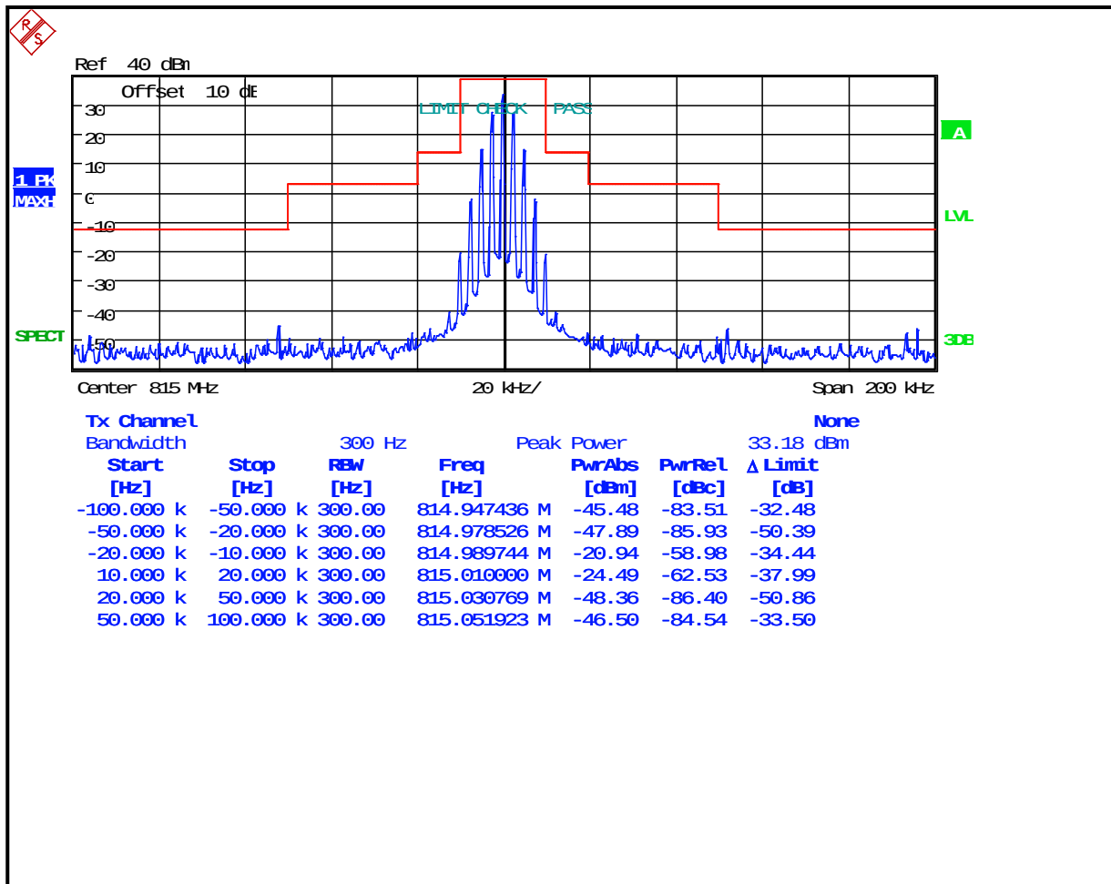
Plot 8-79: Occupied Bandwidth – 815 MHz; Narrowband Analog; Mask B
