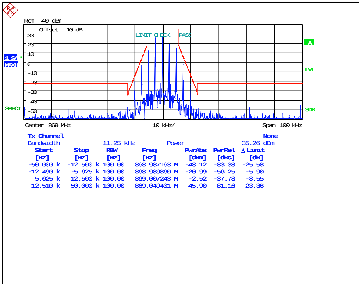
Plot 8-84: Occupied Bandwidth – 869 MHz; Narrowband Analog; Mask D
