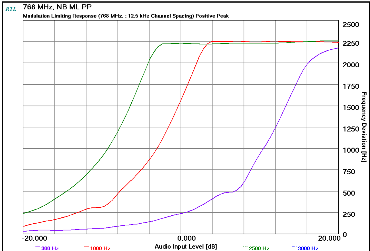
Plot 10-34: Modulation Characteristics – Modulation Limiting - 768 MHz; Positive Peak; NB
